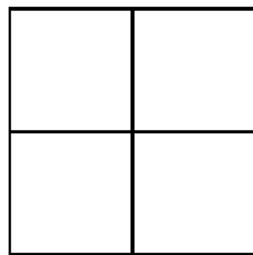
QUADTREE SPLIT
