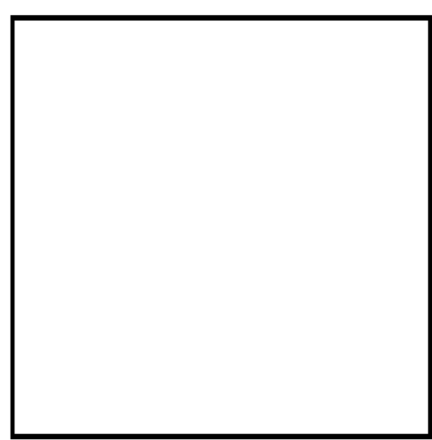
NO SPLIT
