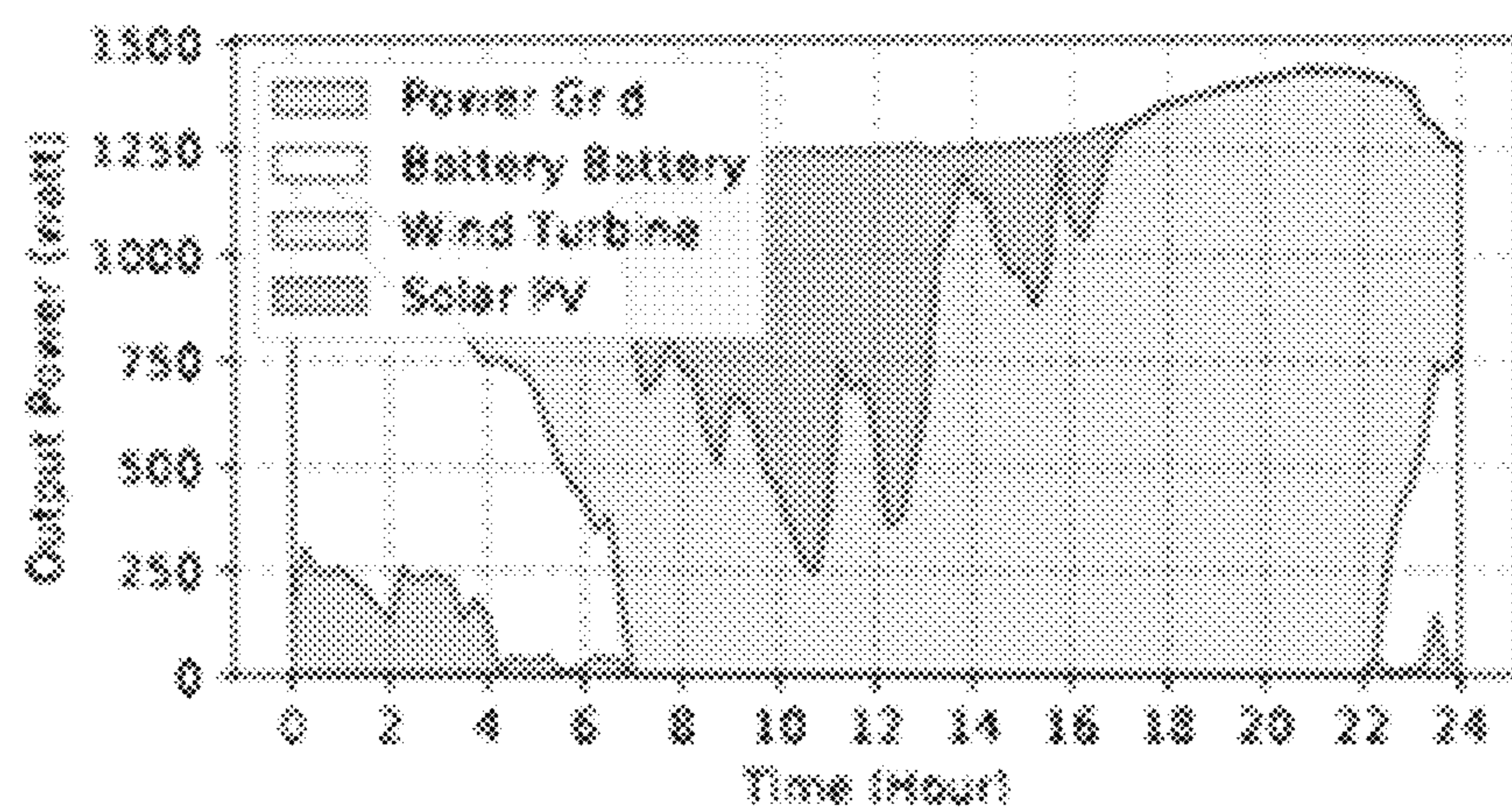
(e) The power supply pattern under the partial cloudy & middle-wind day
