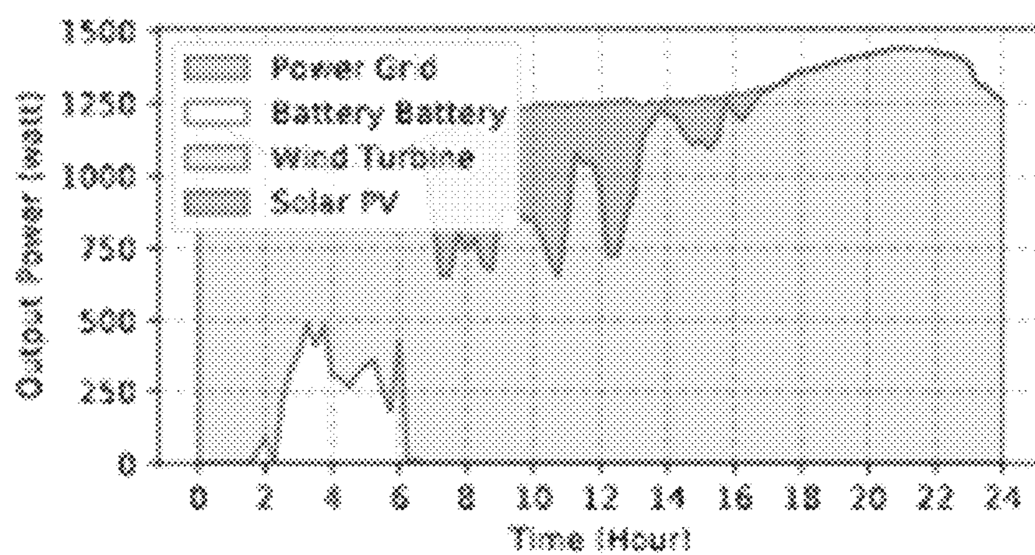
(d) The power supply pattern under the partial cloudy & high-wind day
