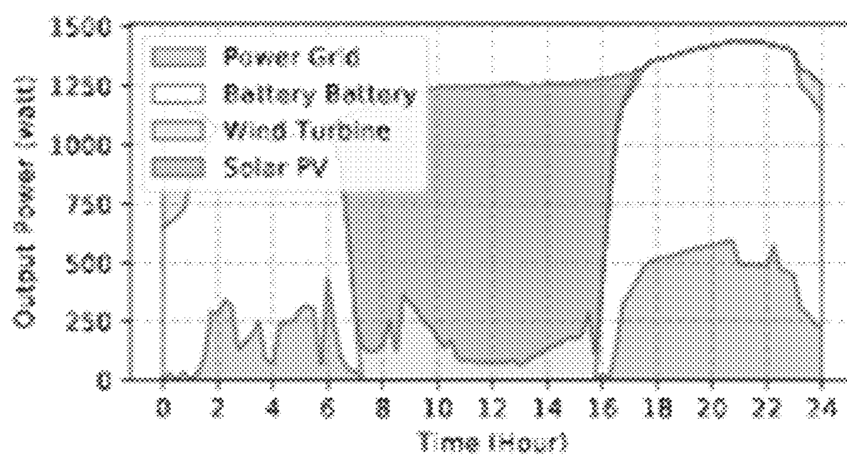
(c) The power supply pattern under the clear & low-wind day
