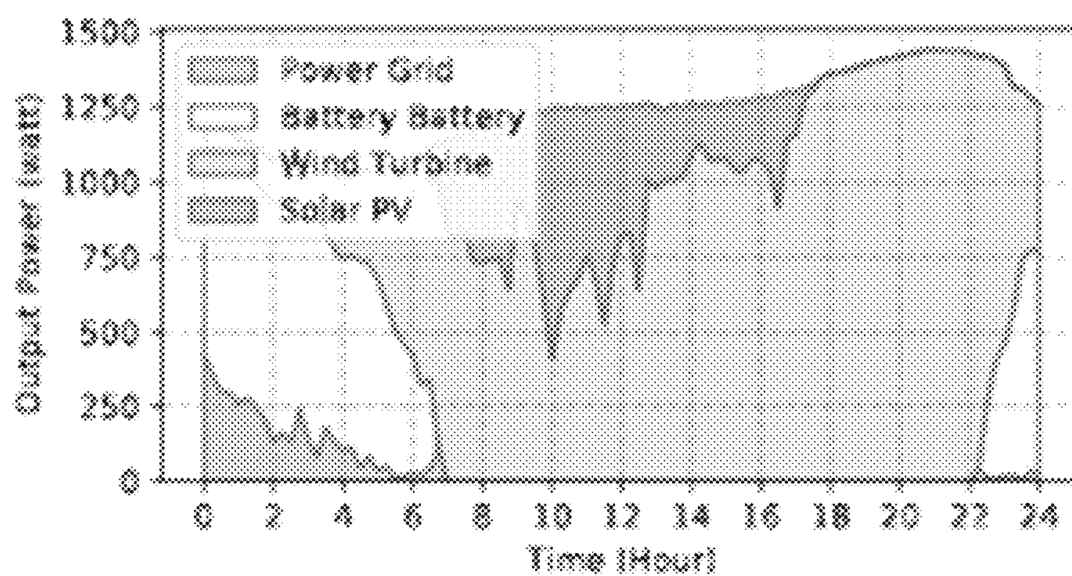
(h) The power supply pattern under the cloudy & middle-wind day
