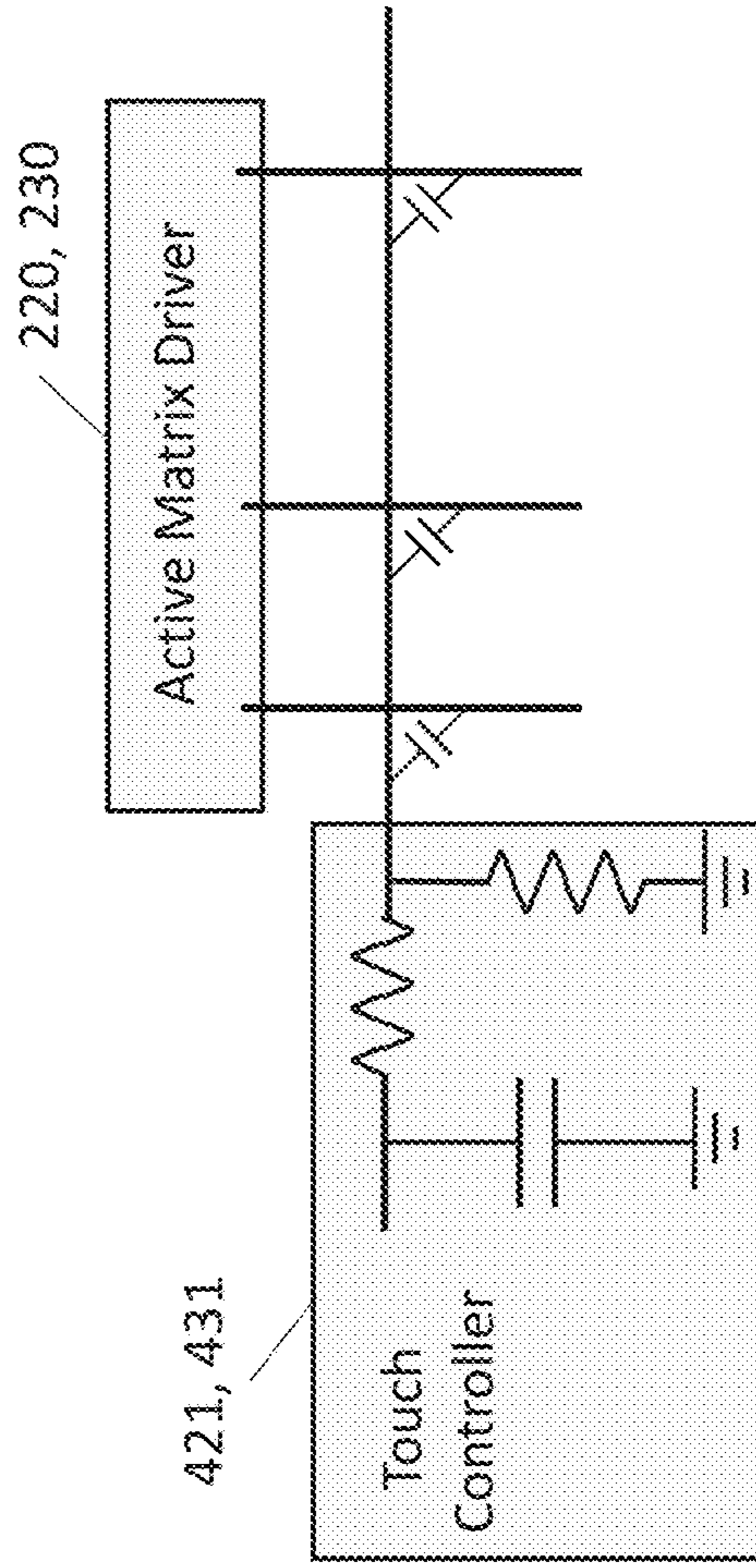
FIG. 14C: Use of a Band-Pass Filter on a Touch Controller channel connected to multiple Active Matrix conductors.
