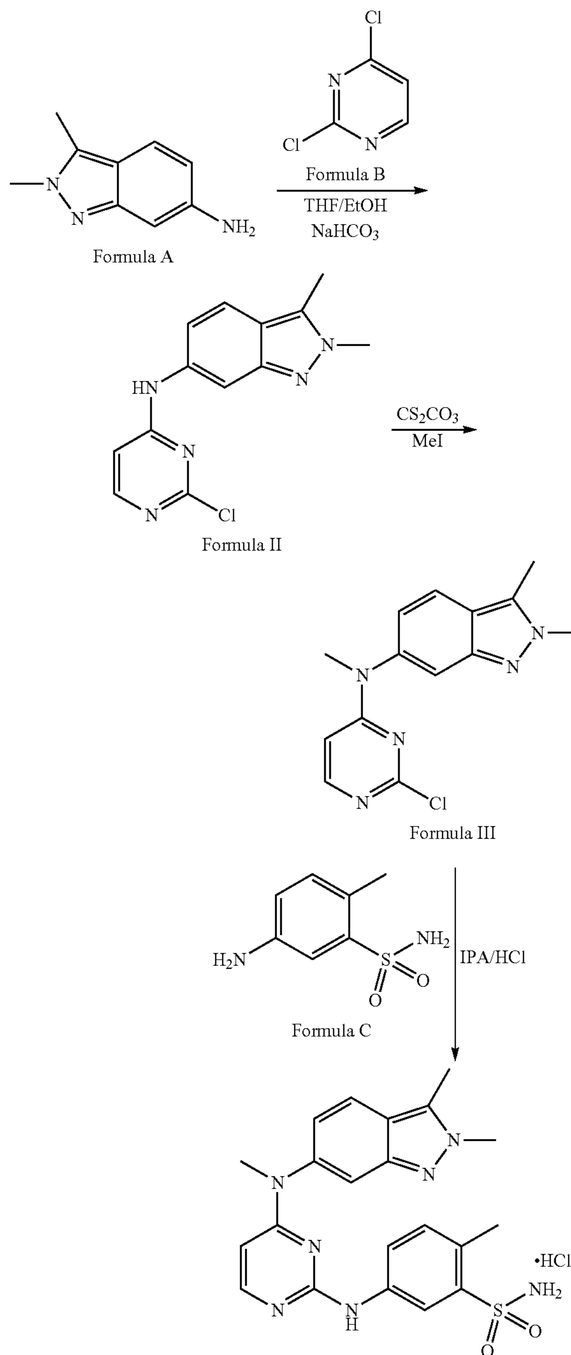
Formula I
