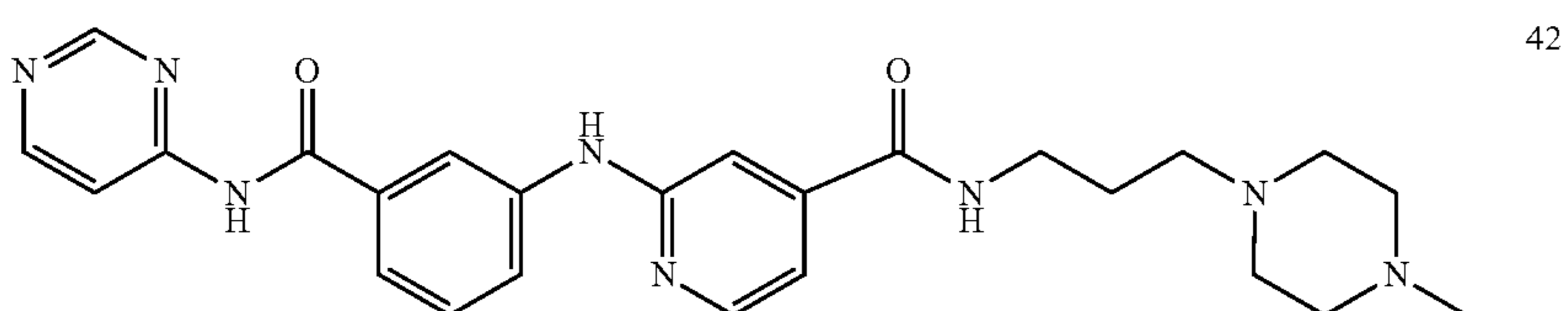
Formula (Id)
