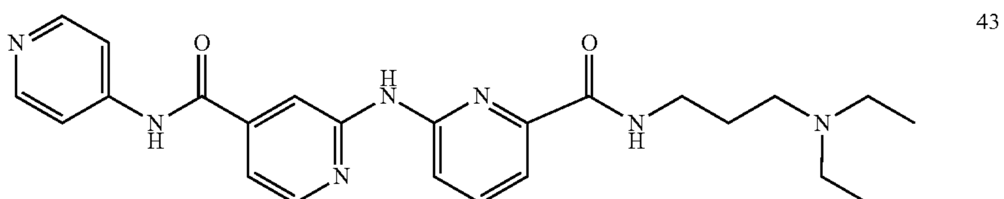
Formula (Id)
