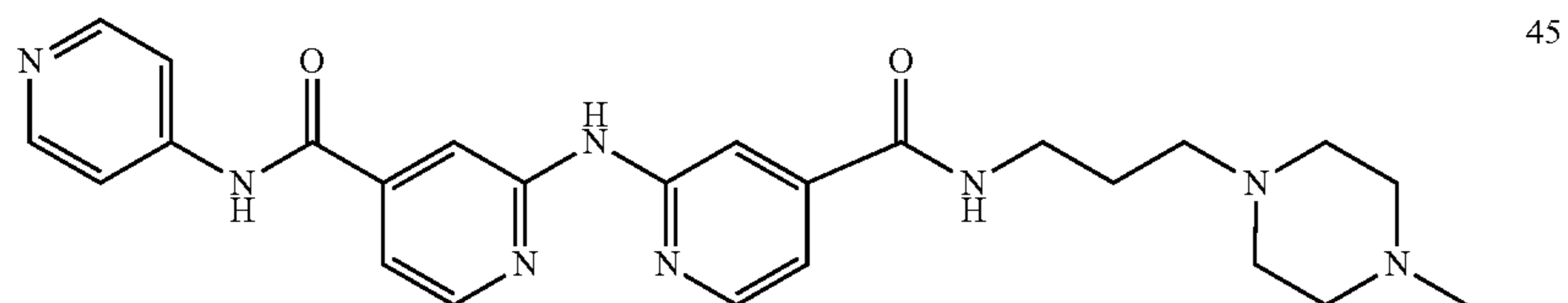
Formula (Ie)
