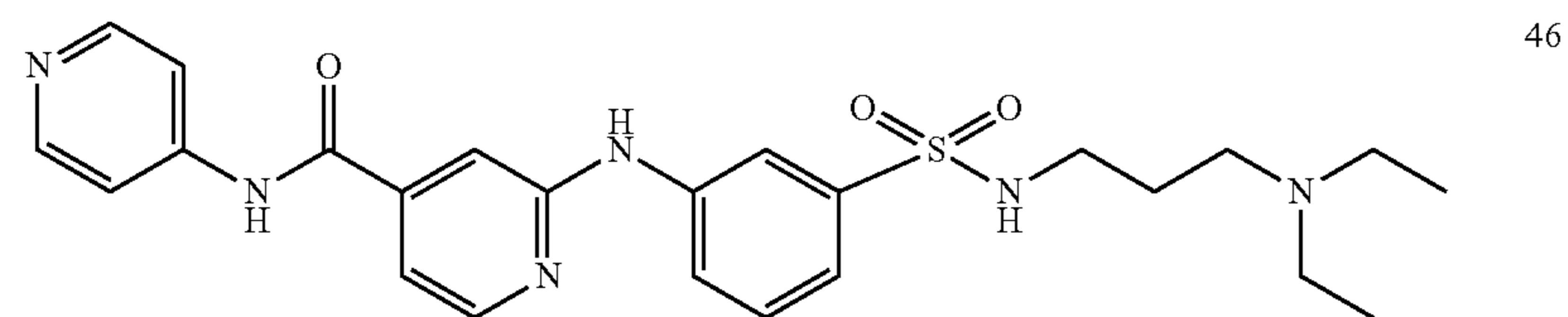
Formula (Ie)
