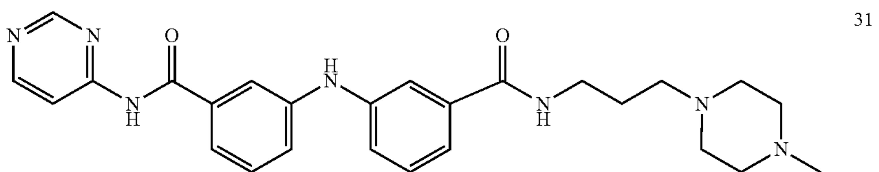
Formula (Ib)
