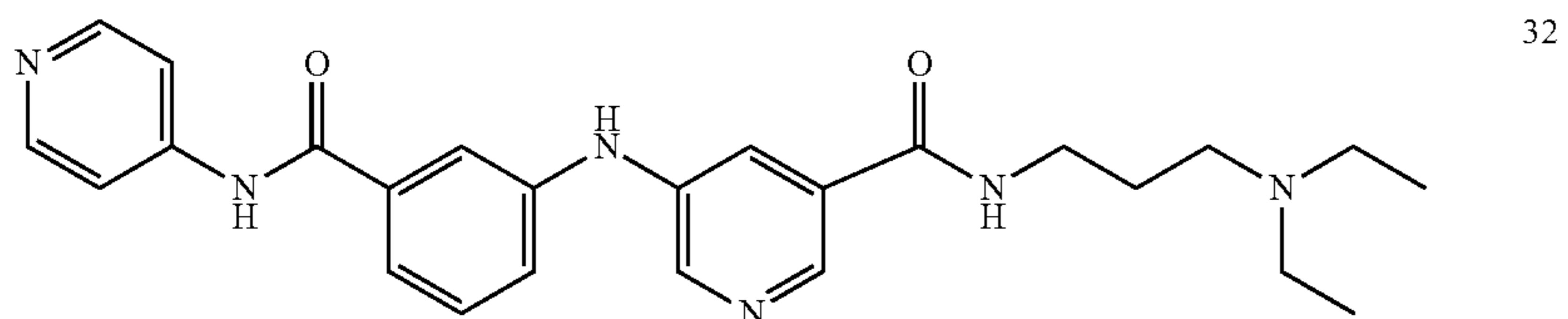
Formula (Ic)
