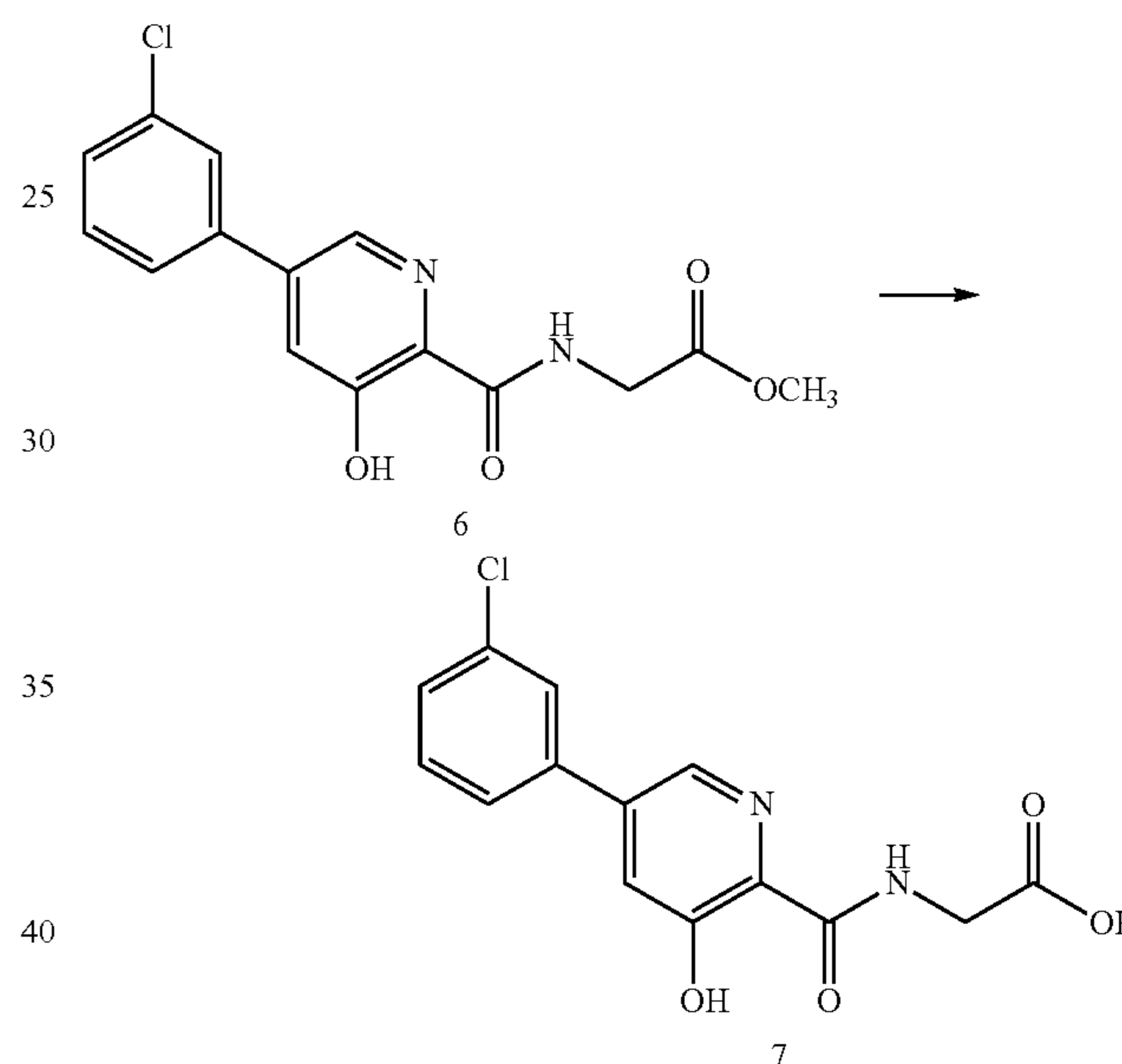
Scheme II
