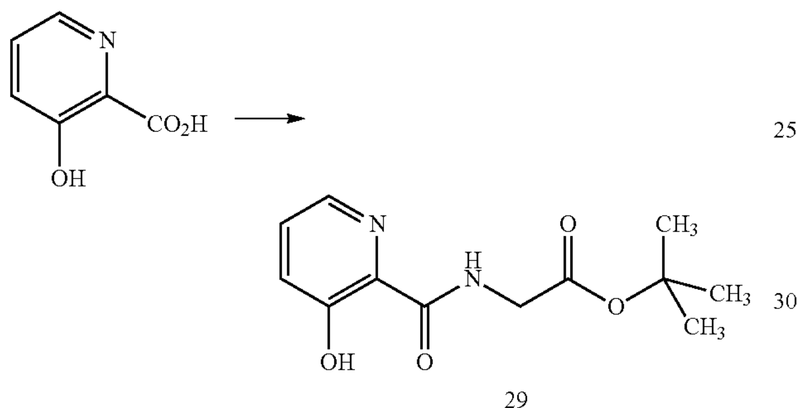
Scheme XVI
