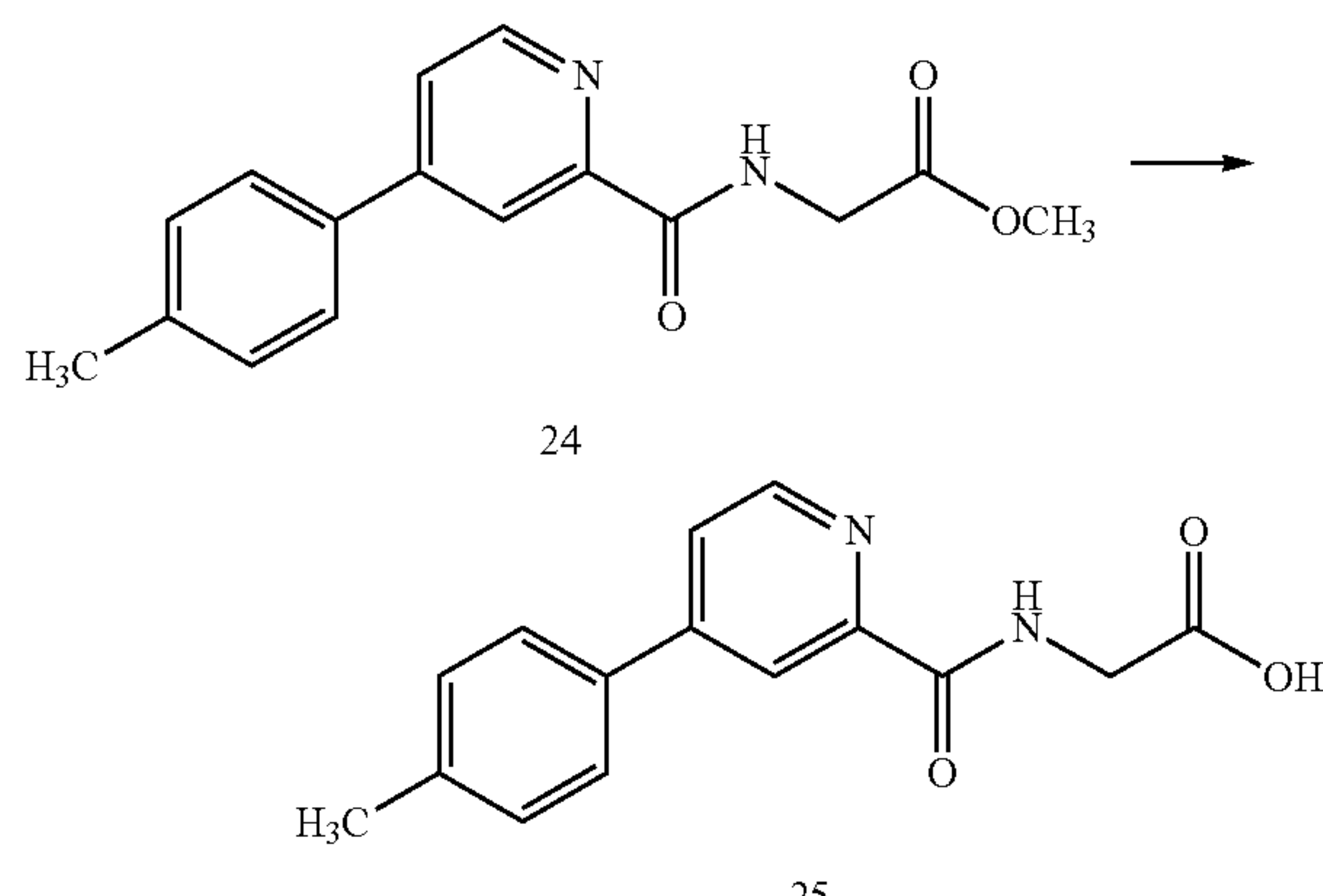
Scheme XIII
