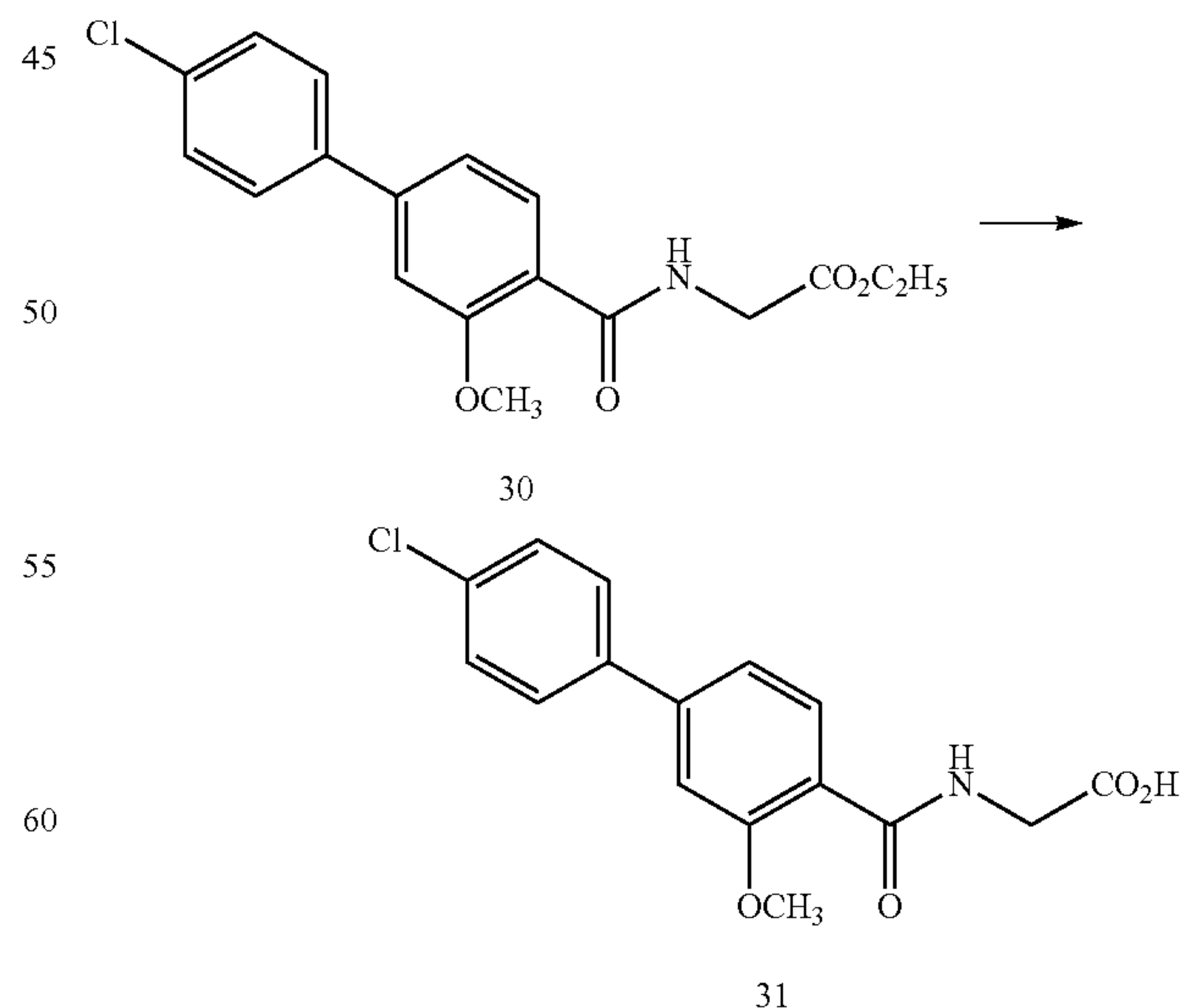
Scheme XVIII
