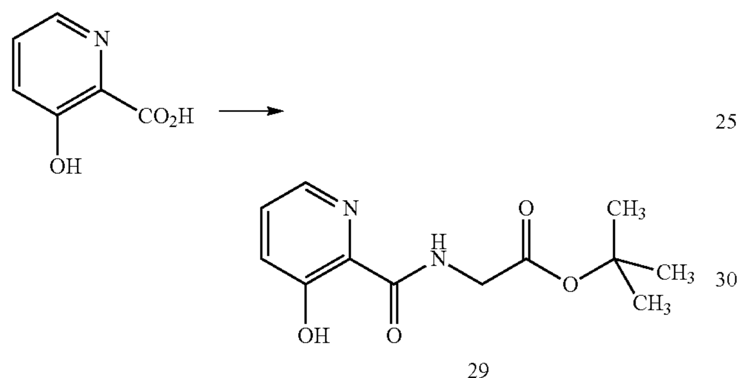
Scheme XVI
