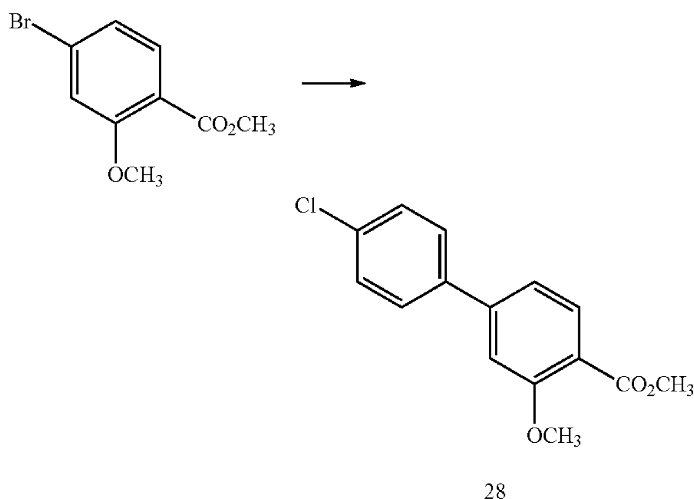
Scheme XVII
