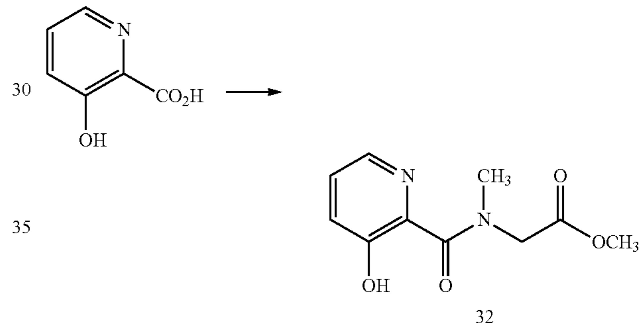
Scheme XIX
