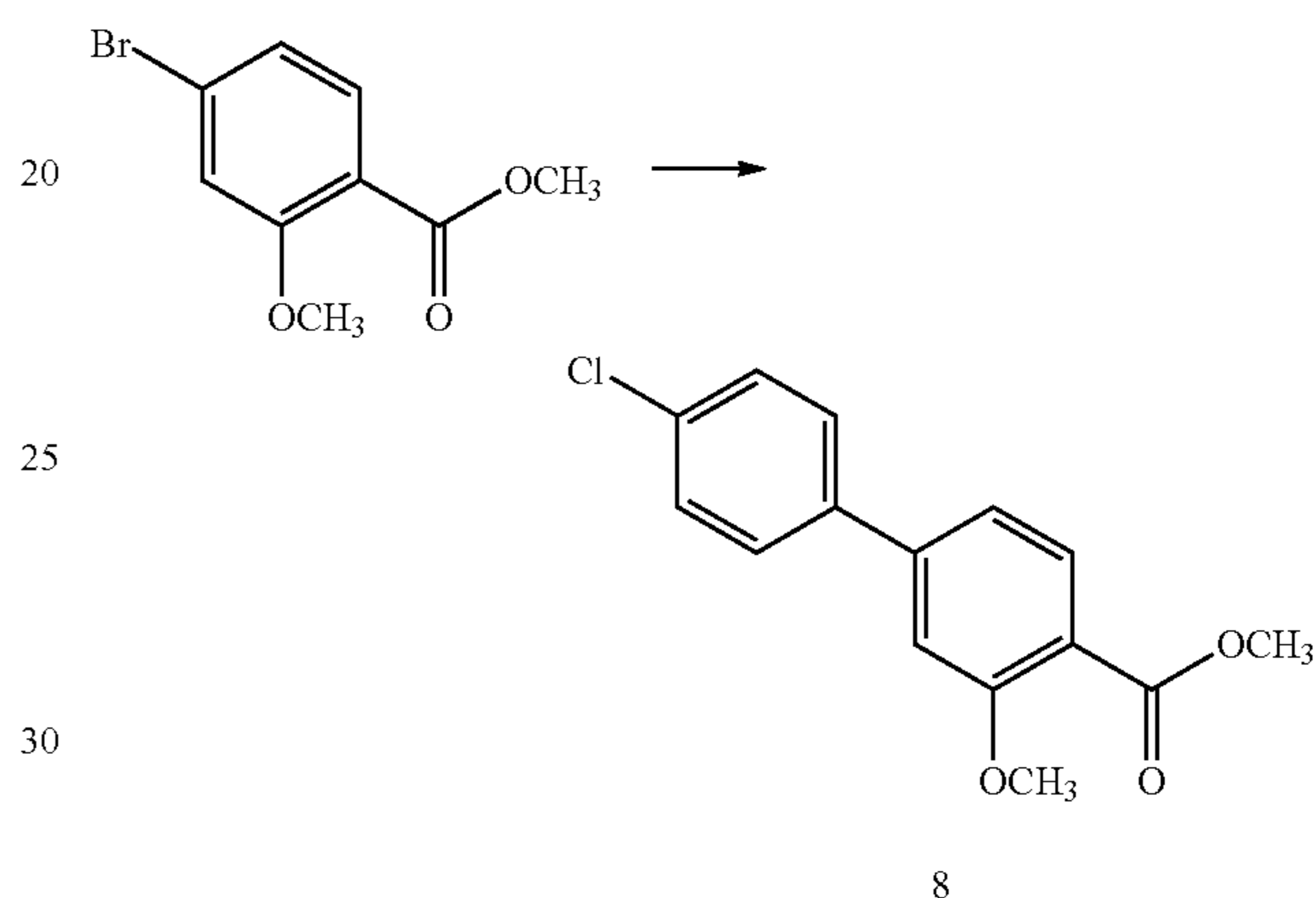
Scheme V
