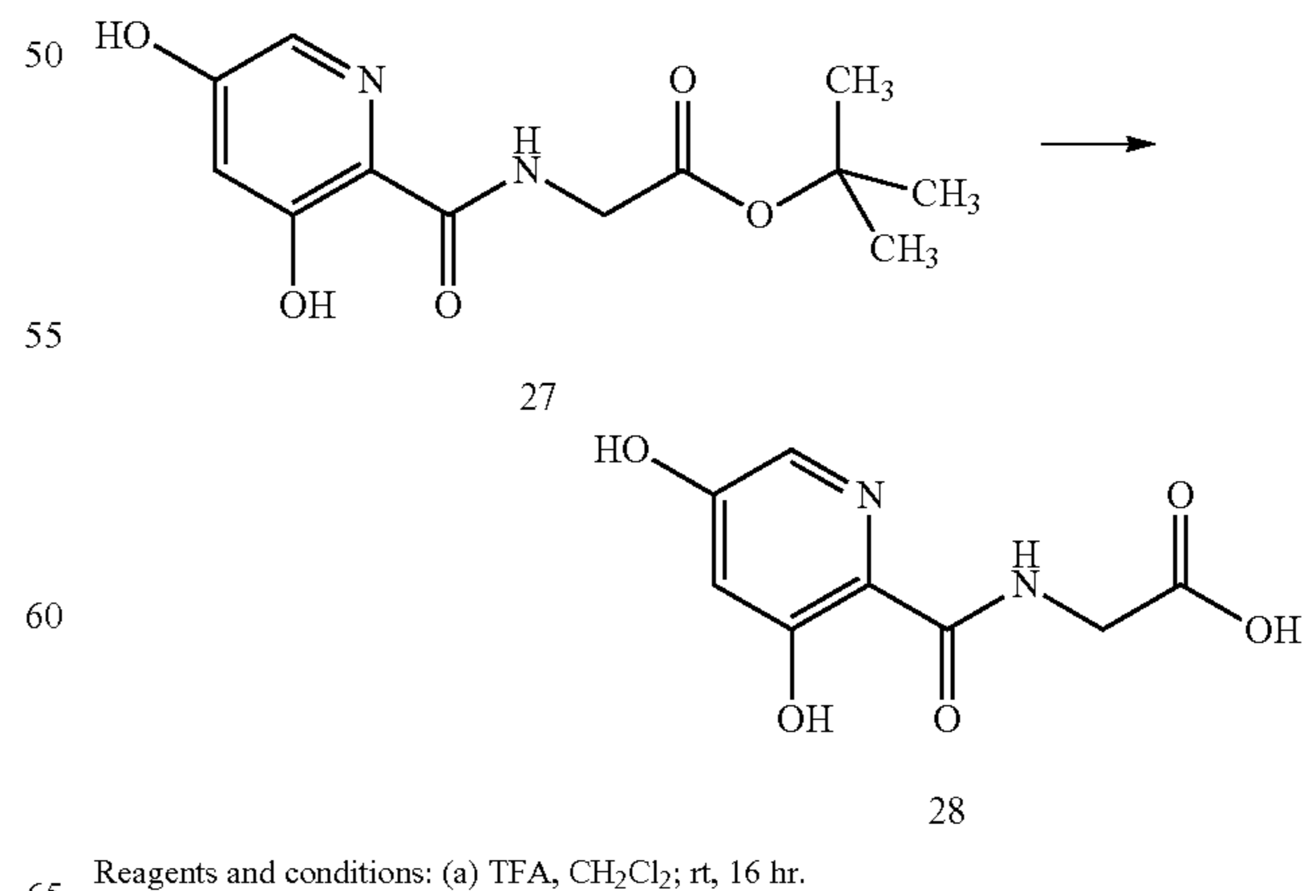
Scheme XV
