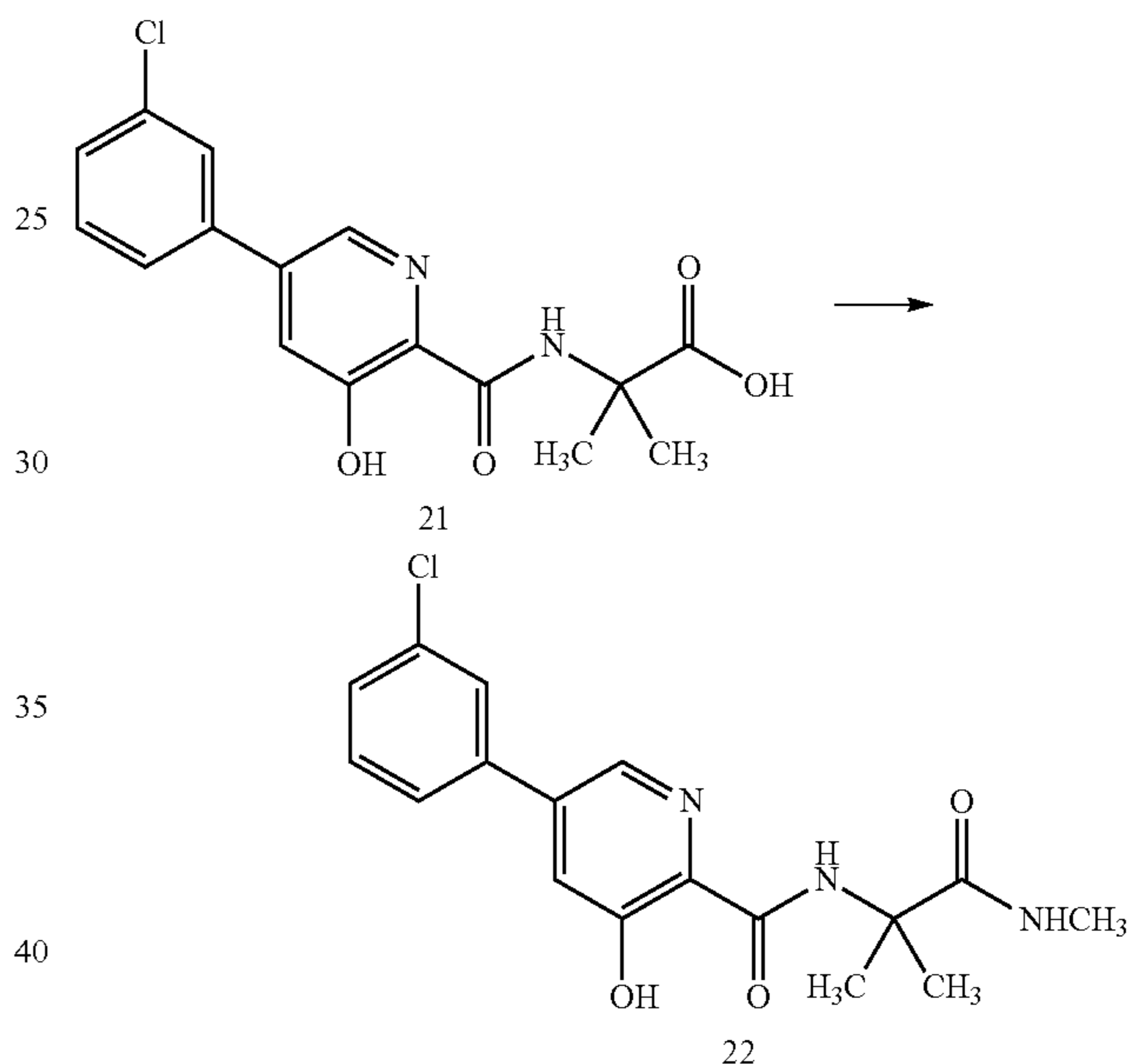
Scheme XI
