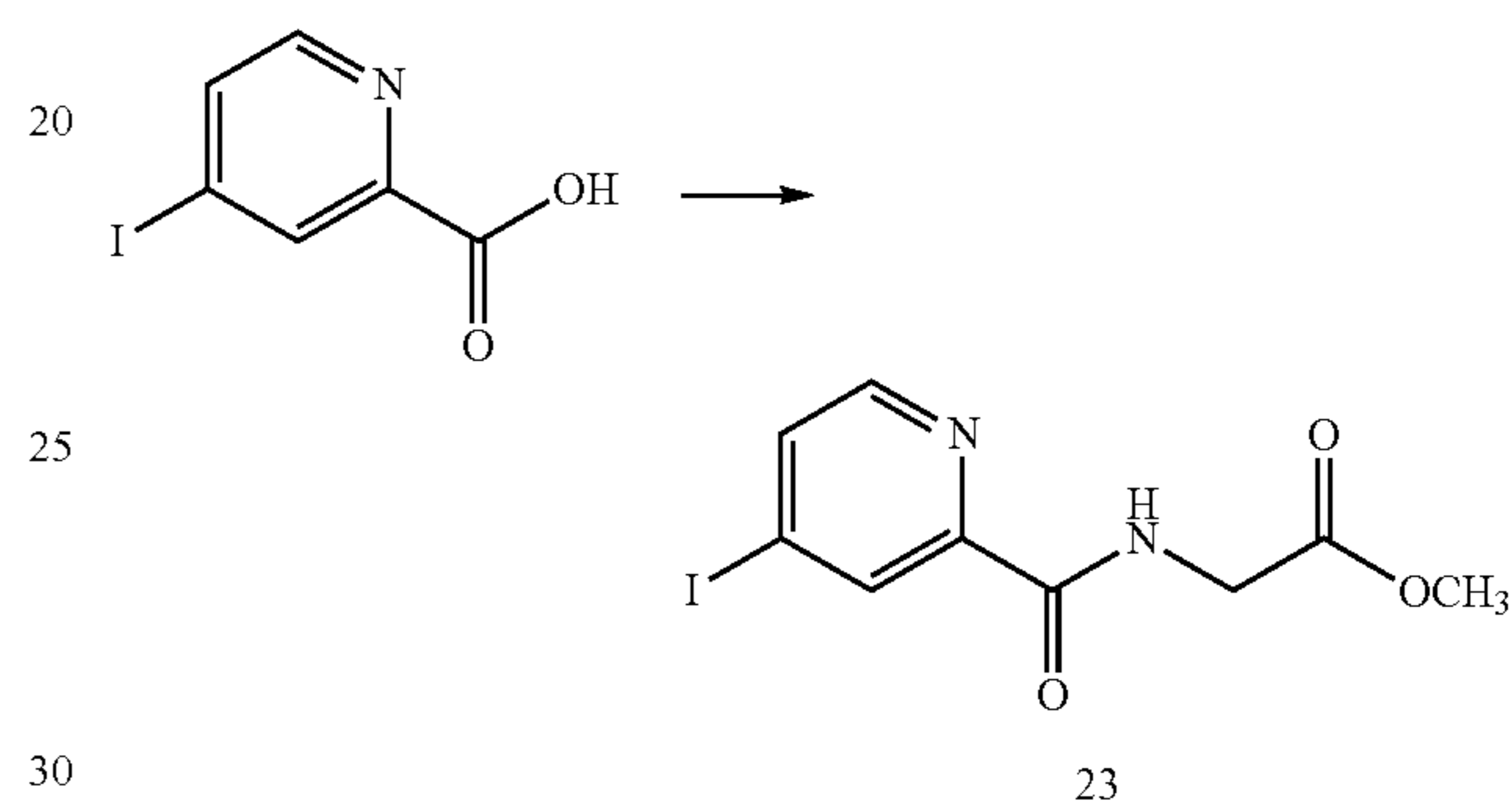
Scheme XII
