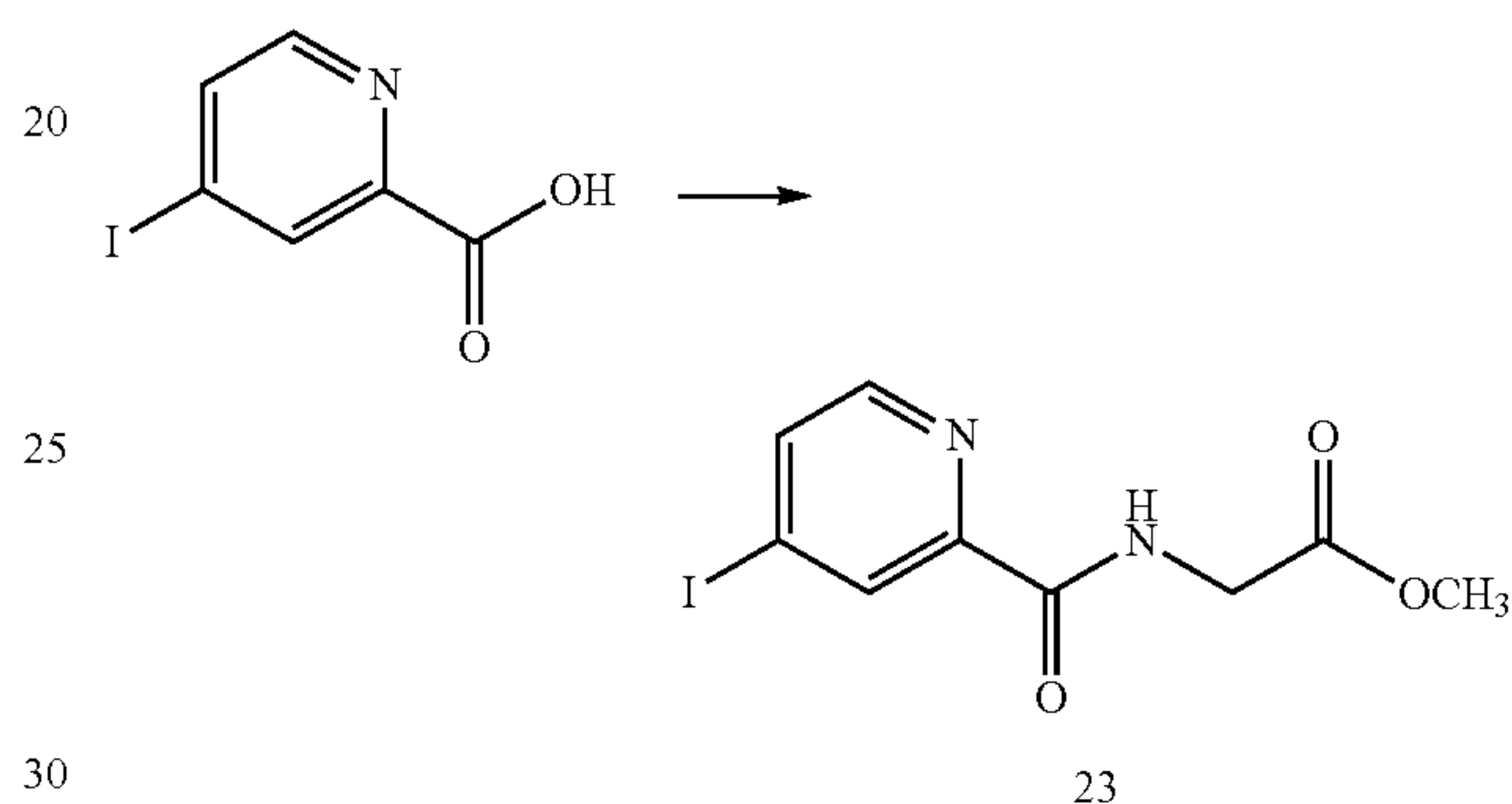
Scheme XII
