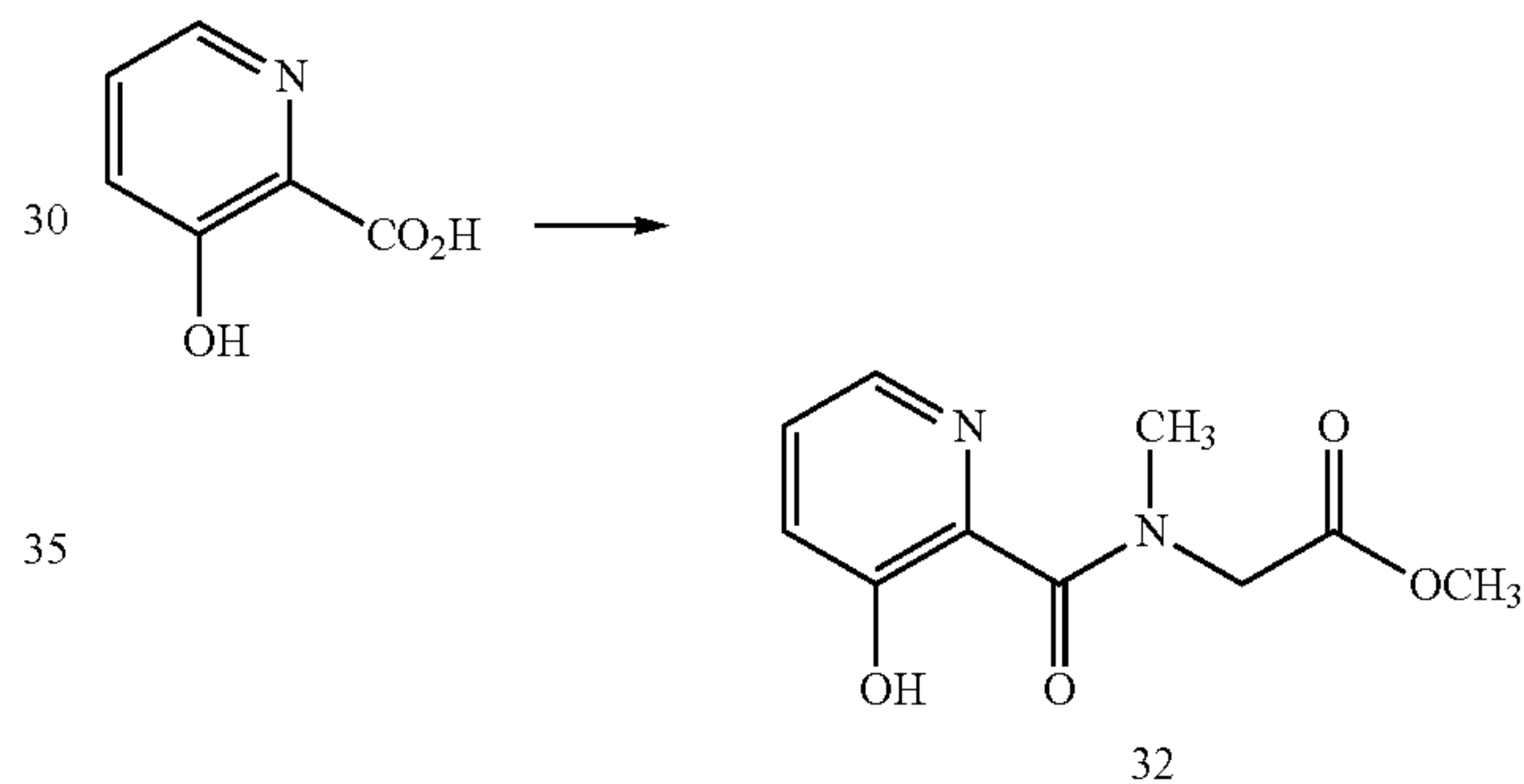
Scheme XIX
