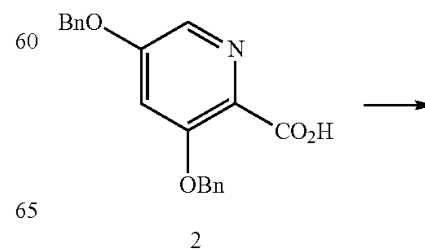
Scheme IX
