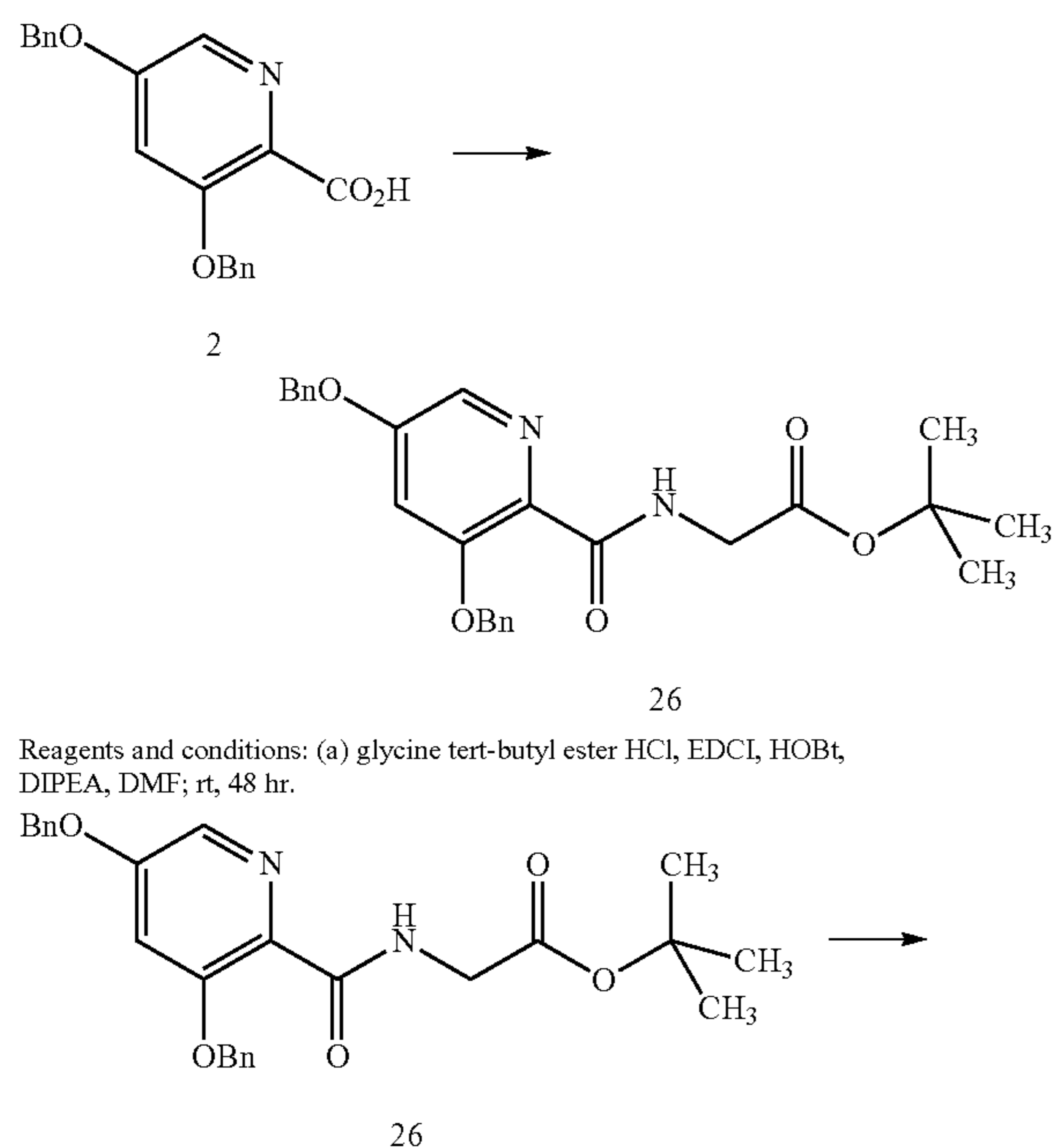
Scheme XIV
