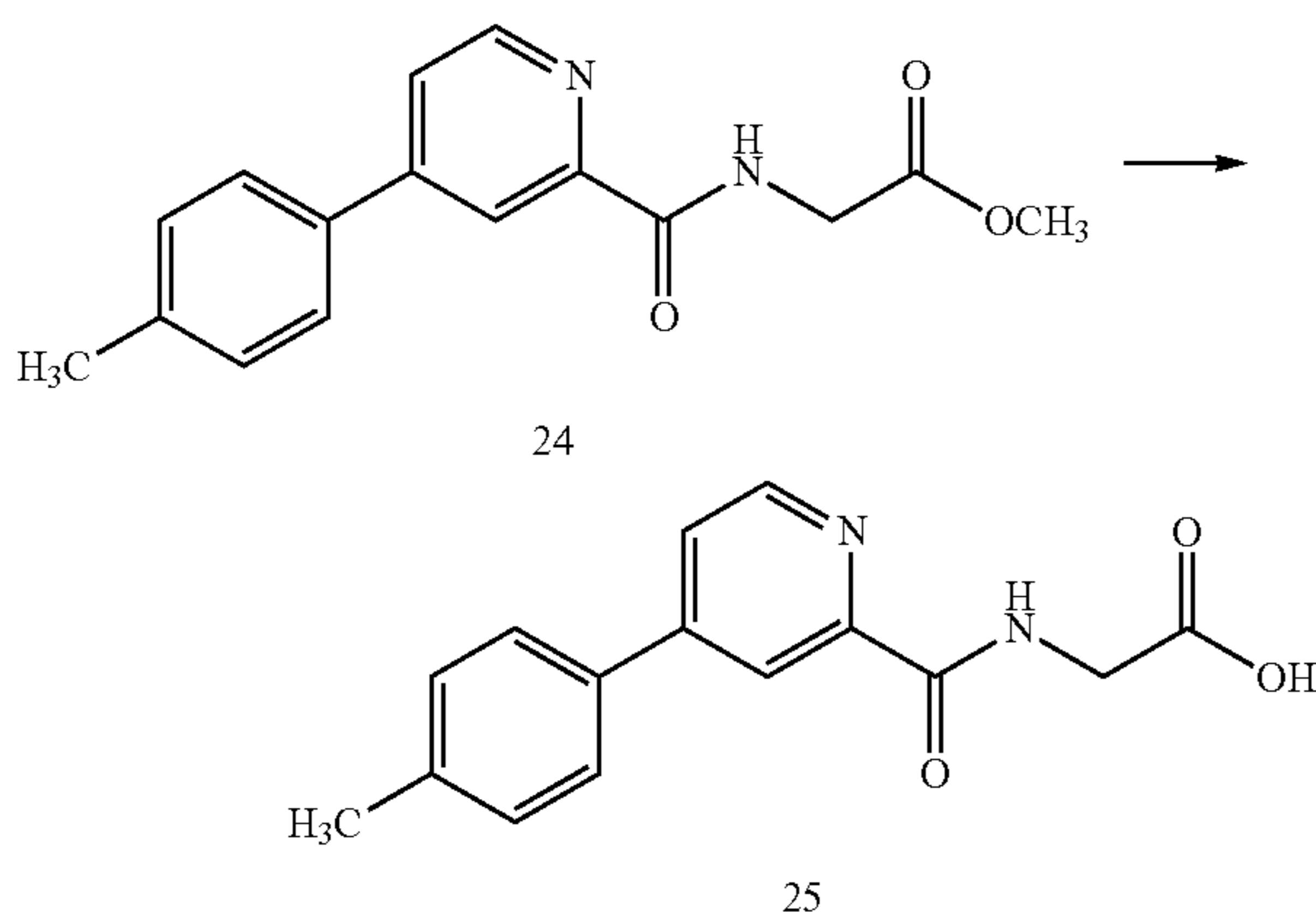
Scheme XIII
