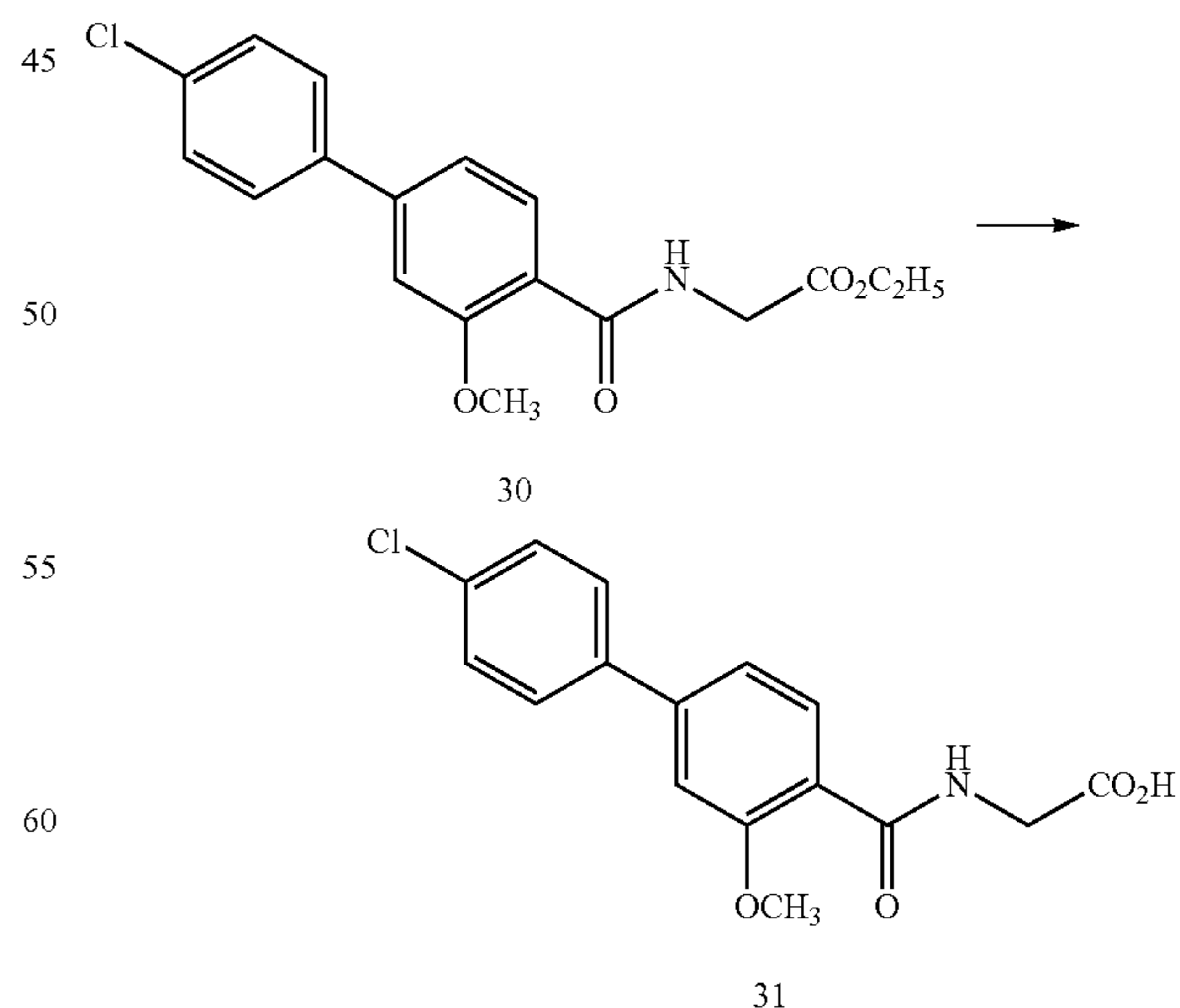
Scheme XVIII
