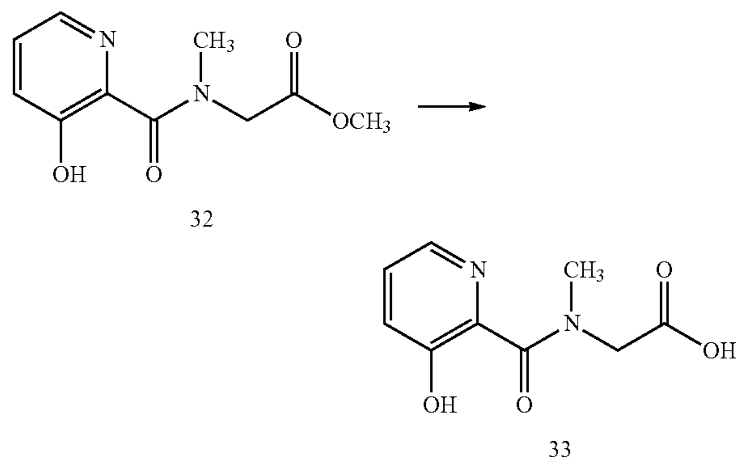
Scheme XX
