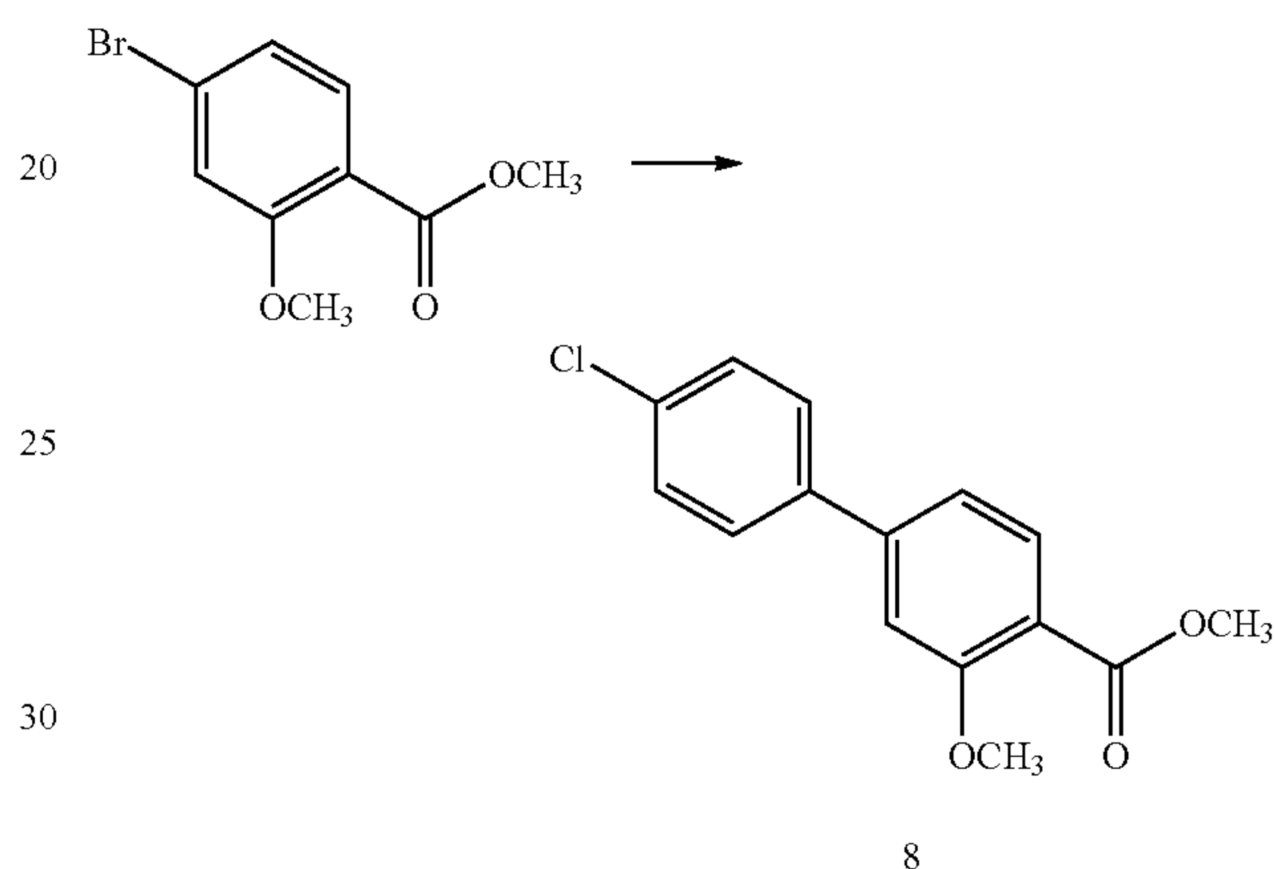
Scheme V
