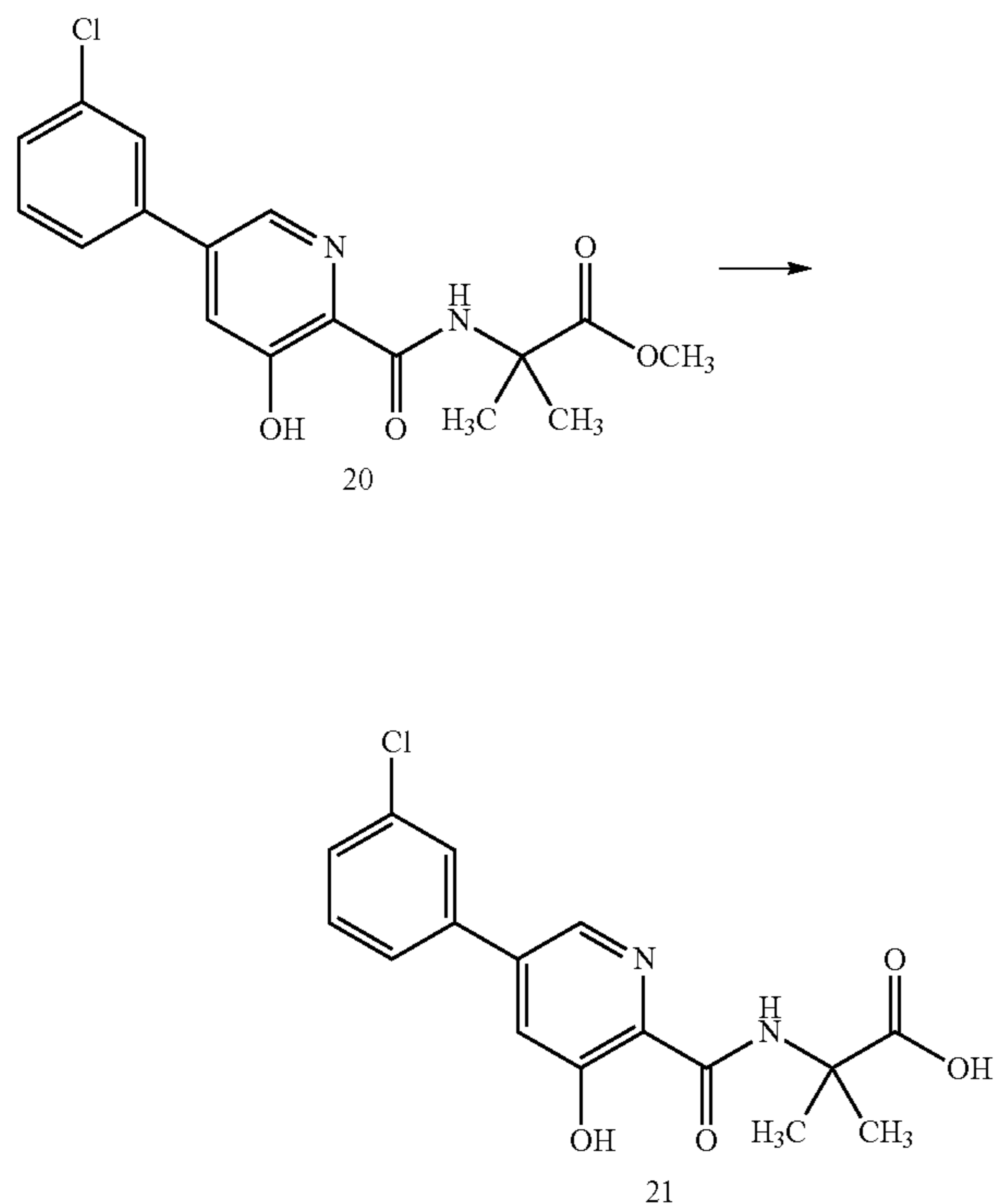
Scheme X
