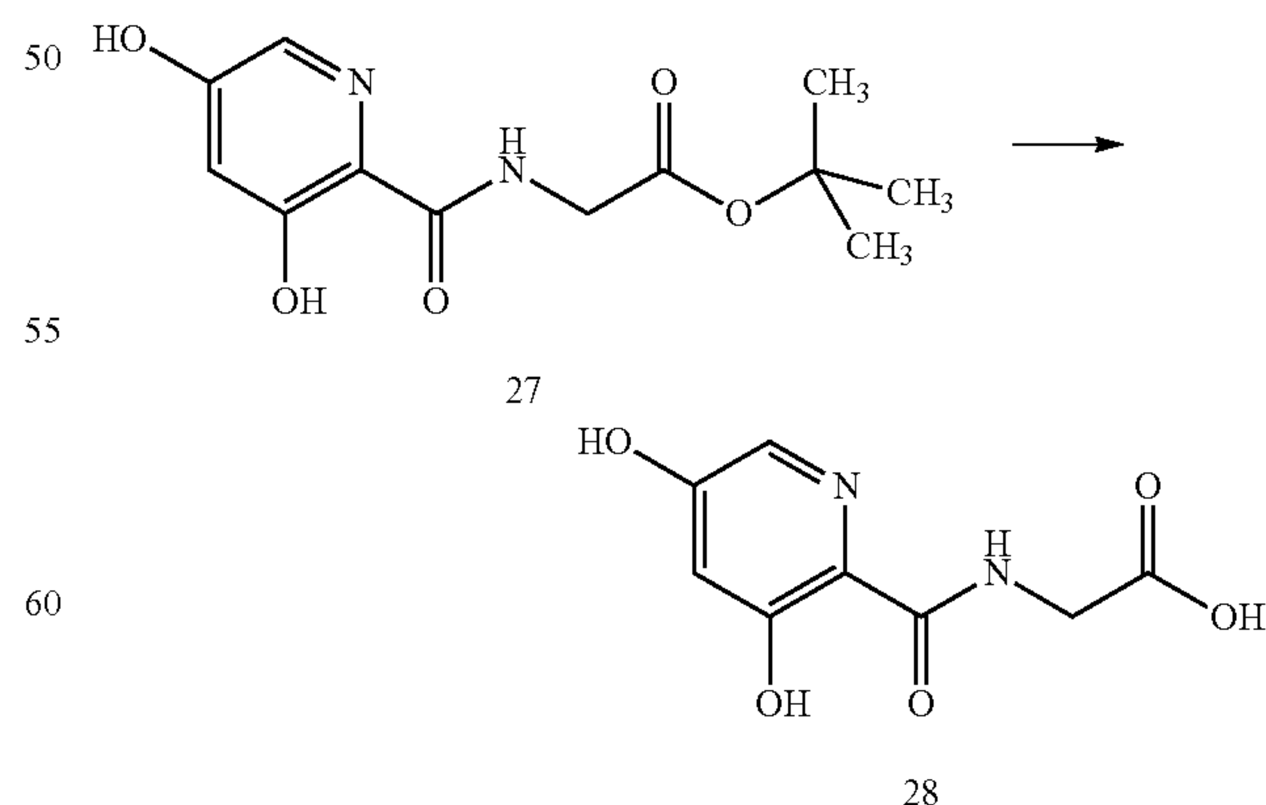
Scheme XV
