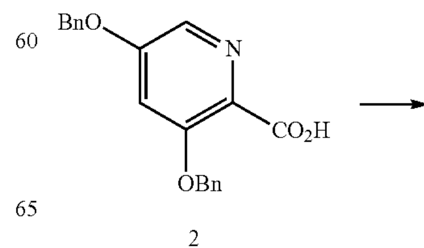
Scheme IX
