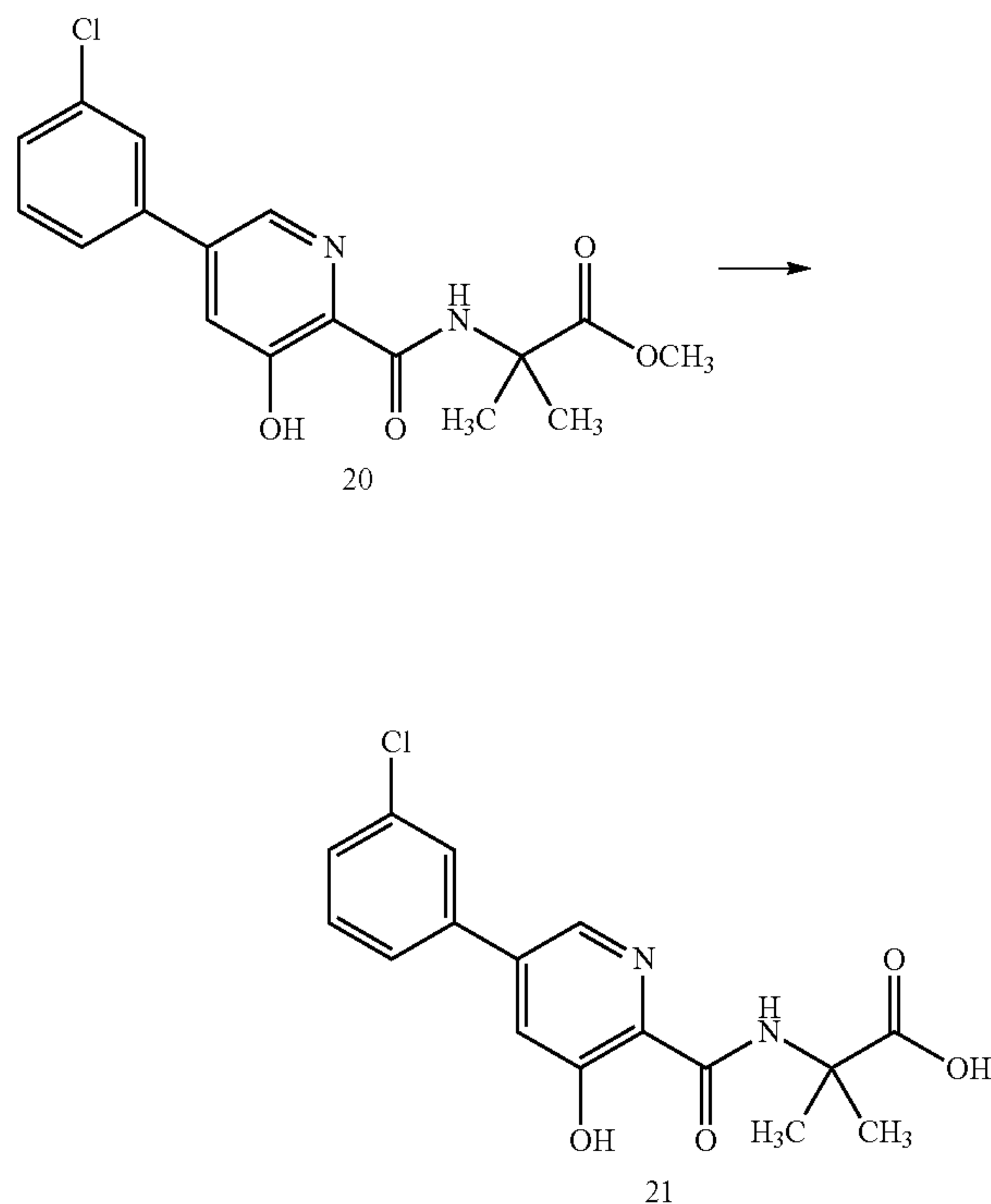
Scheme X
