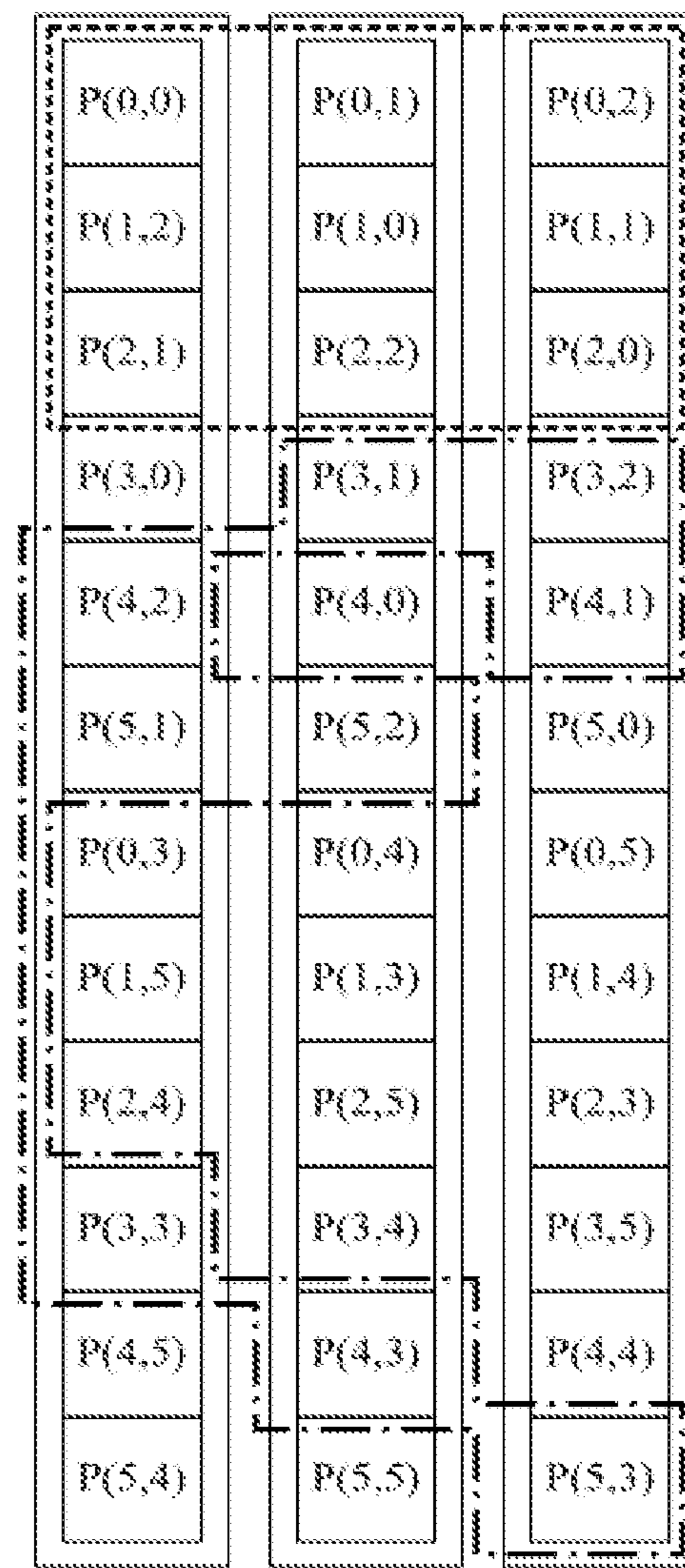
RAM-1 RAM-2 RAM-3 Physical View of Pixel Array
