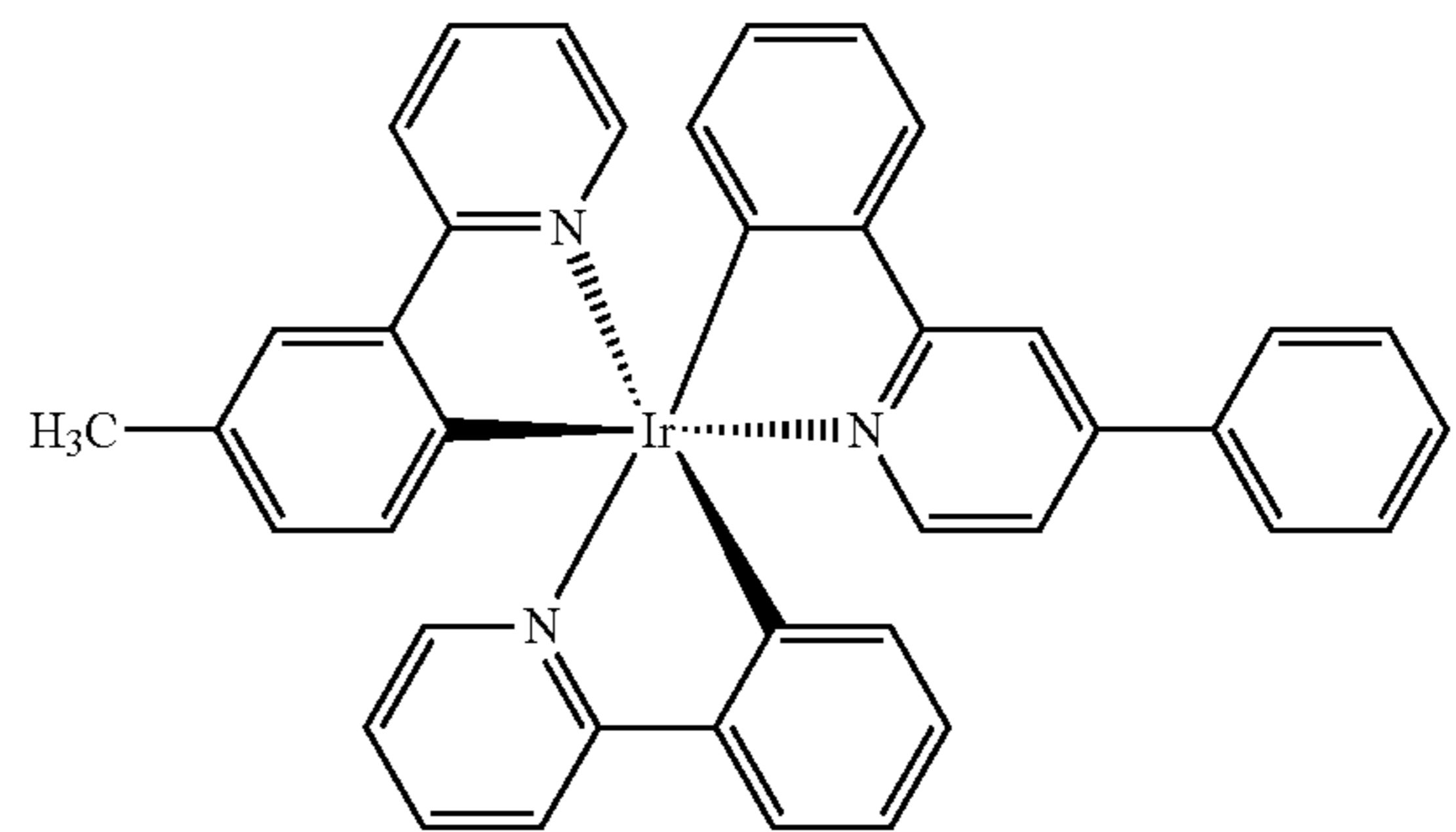
Compound 6
