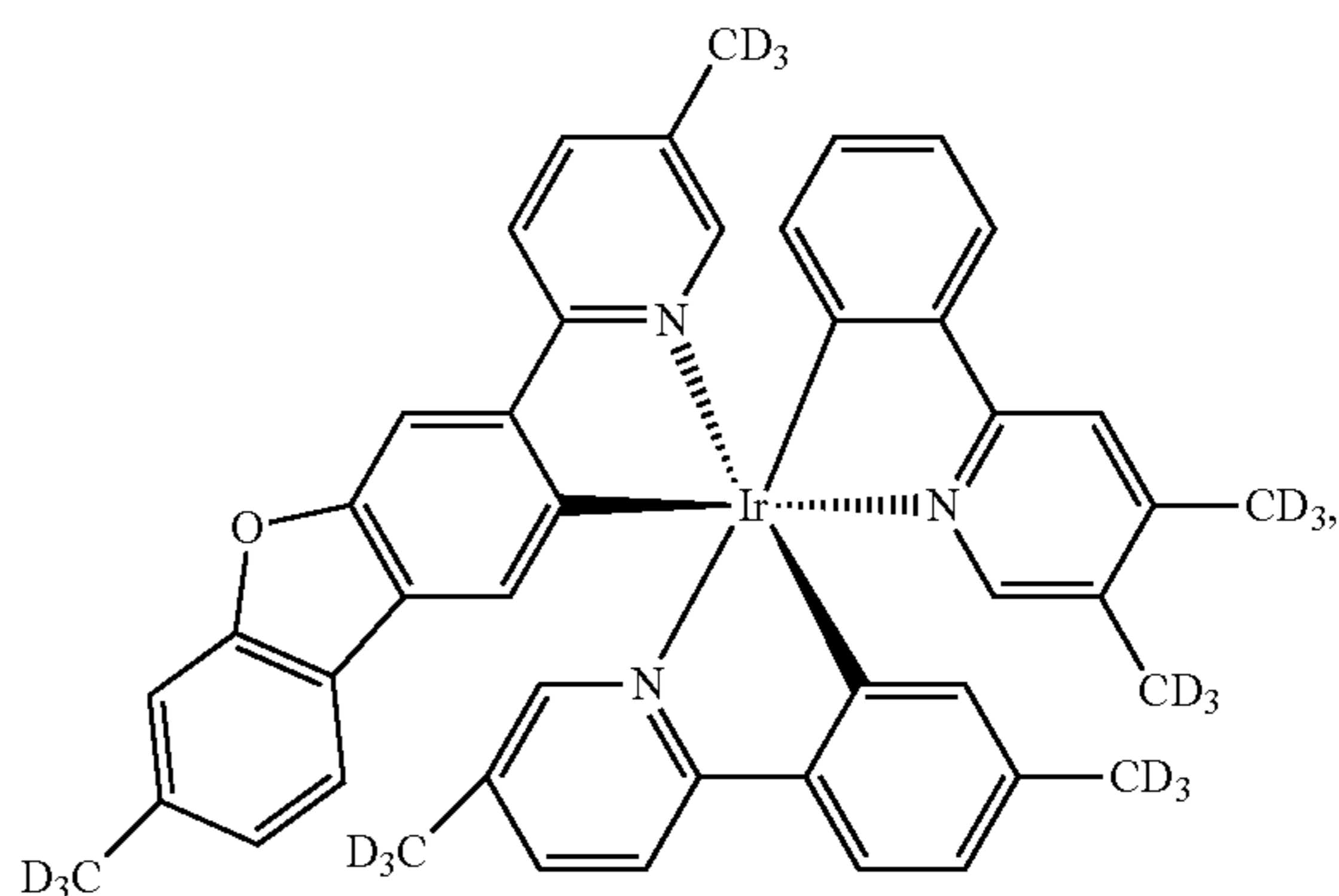
Compound 67
