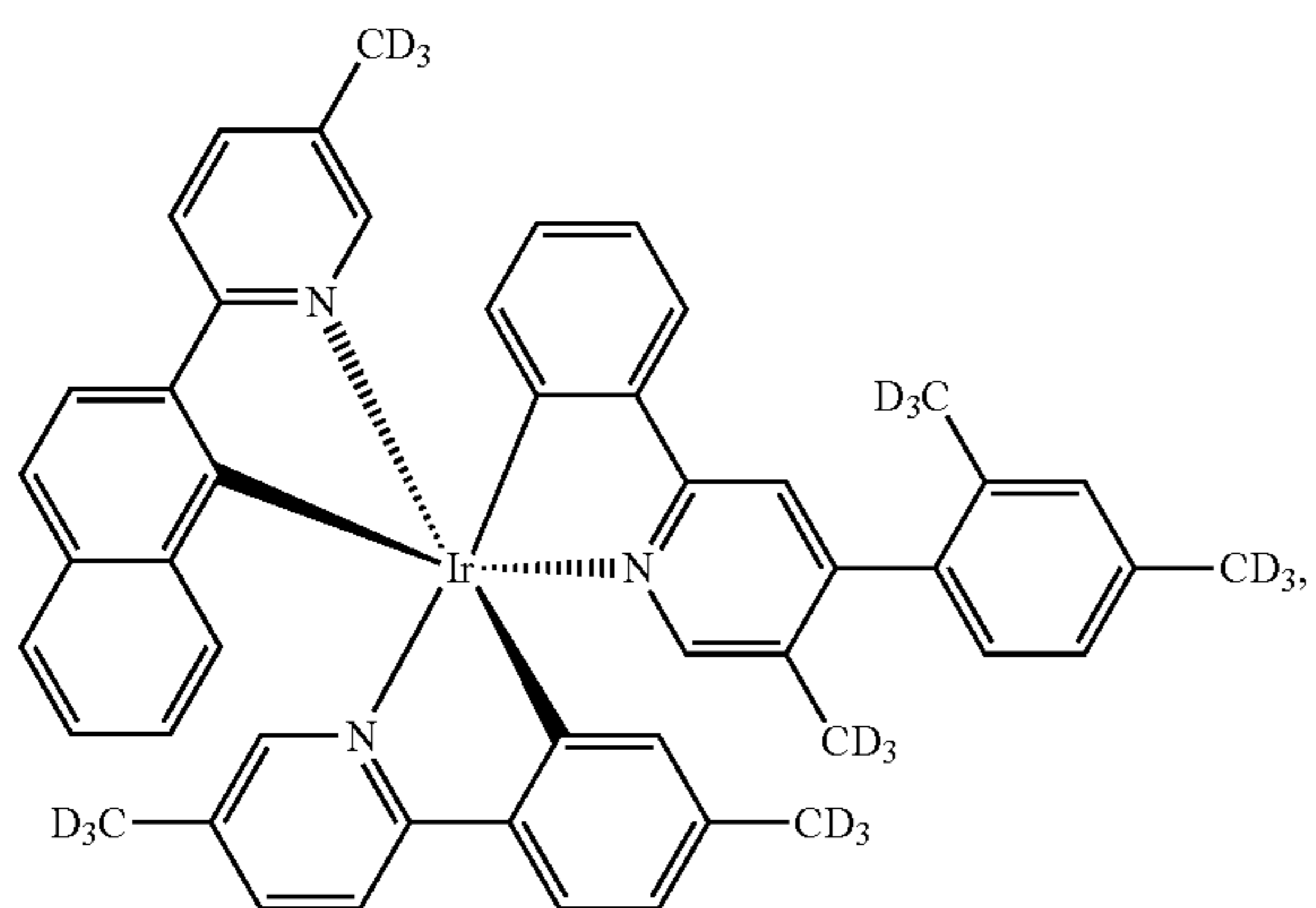
Compound 66
