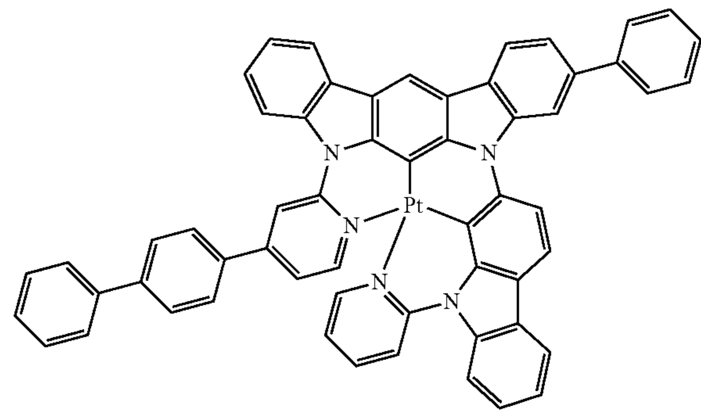
Compound 88
