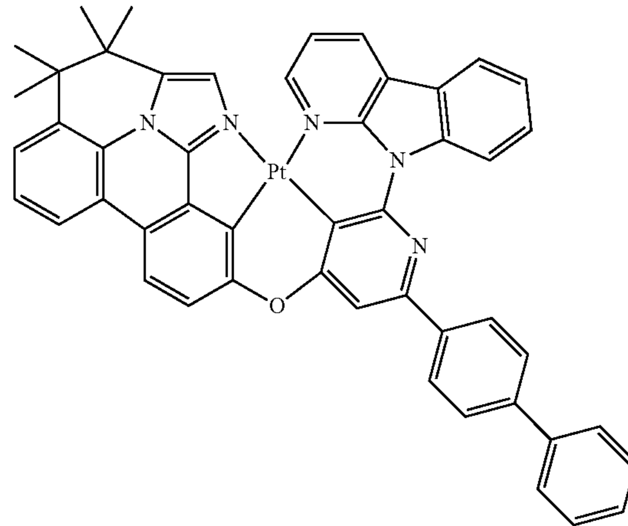
Compound 88
