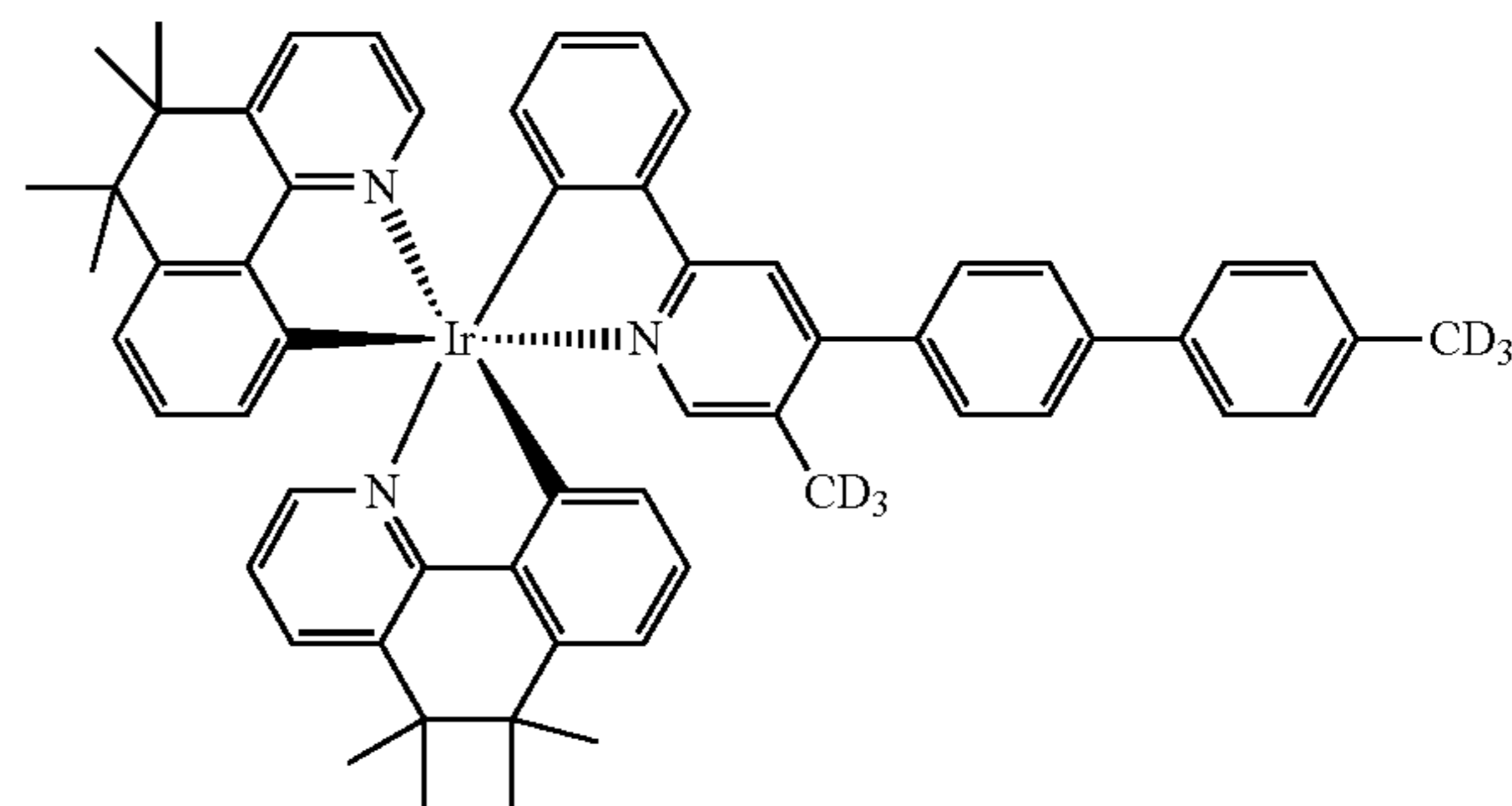
Compound 129
