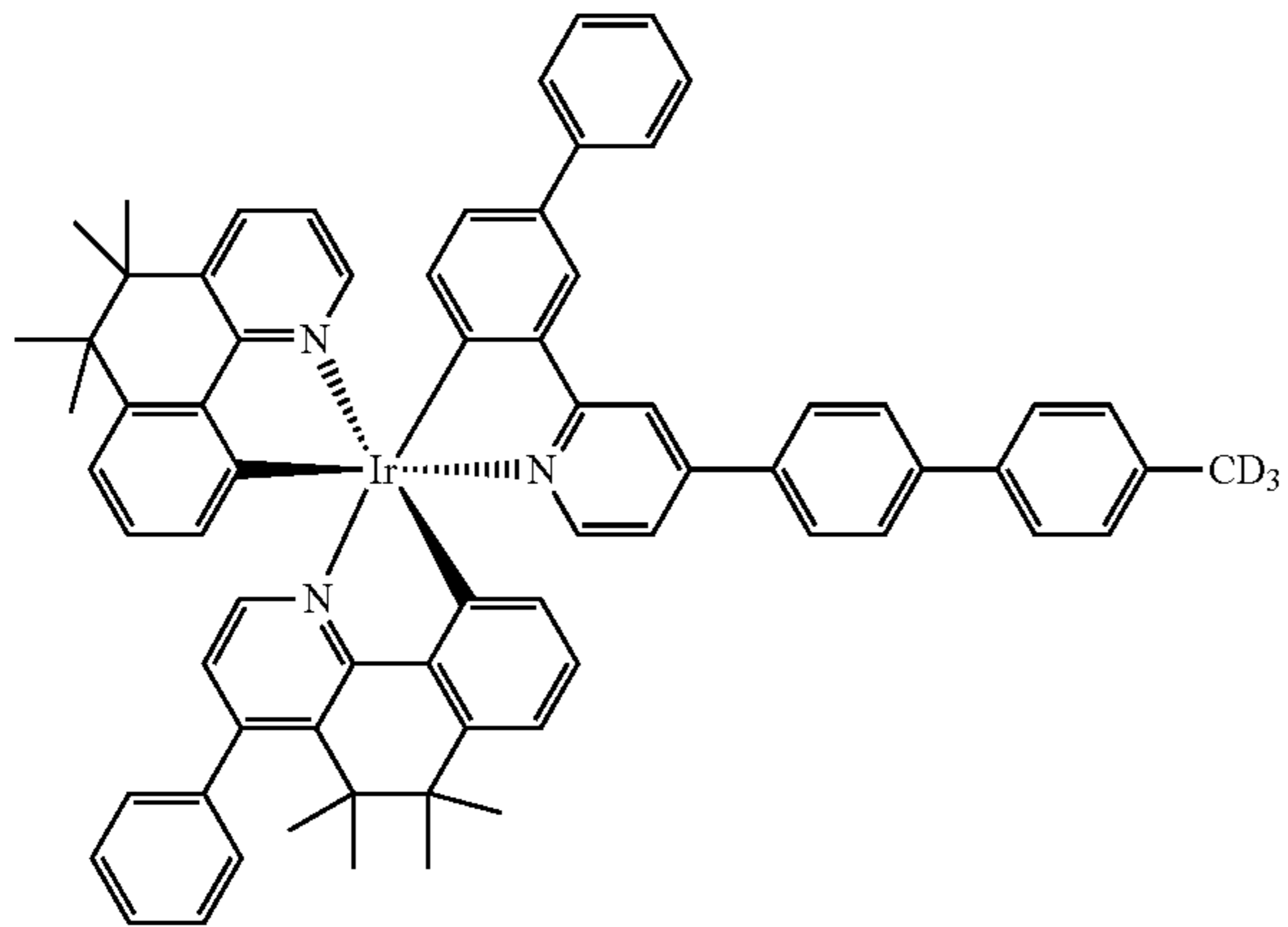
Compound 128
