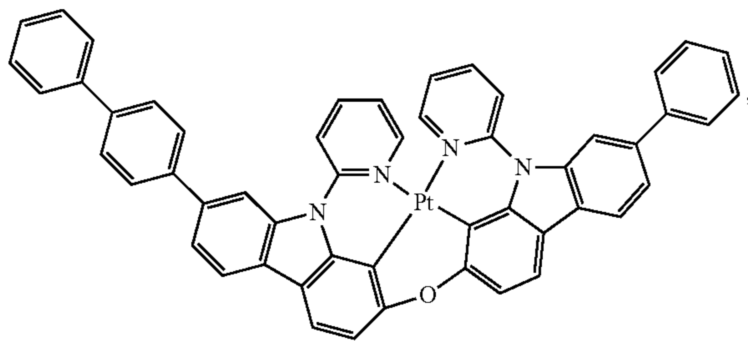
Compound 87
