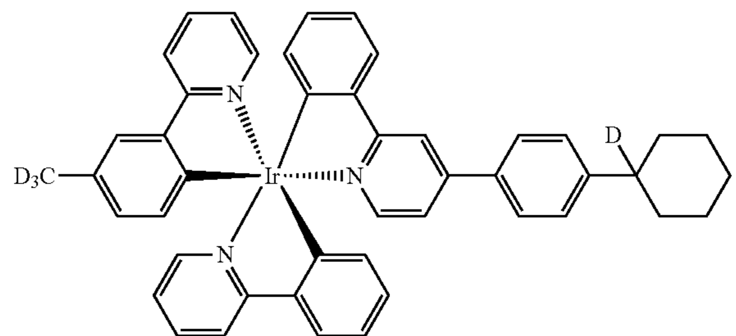
Compound 10
