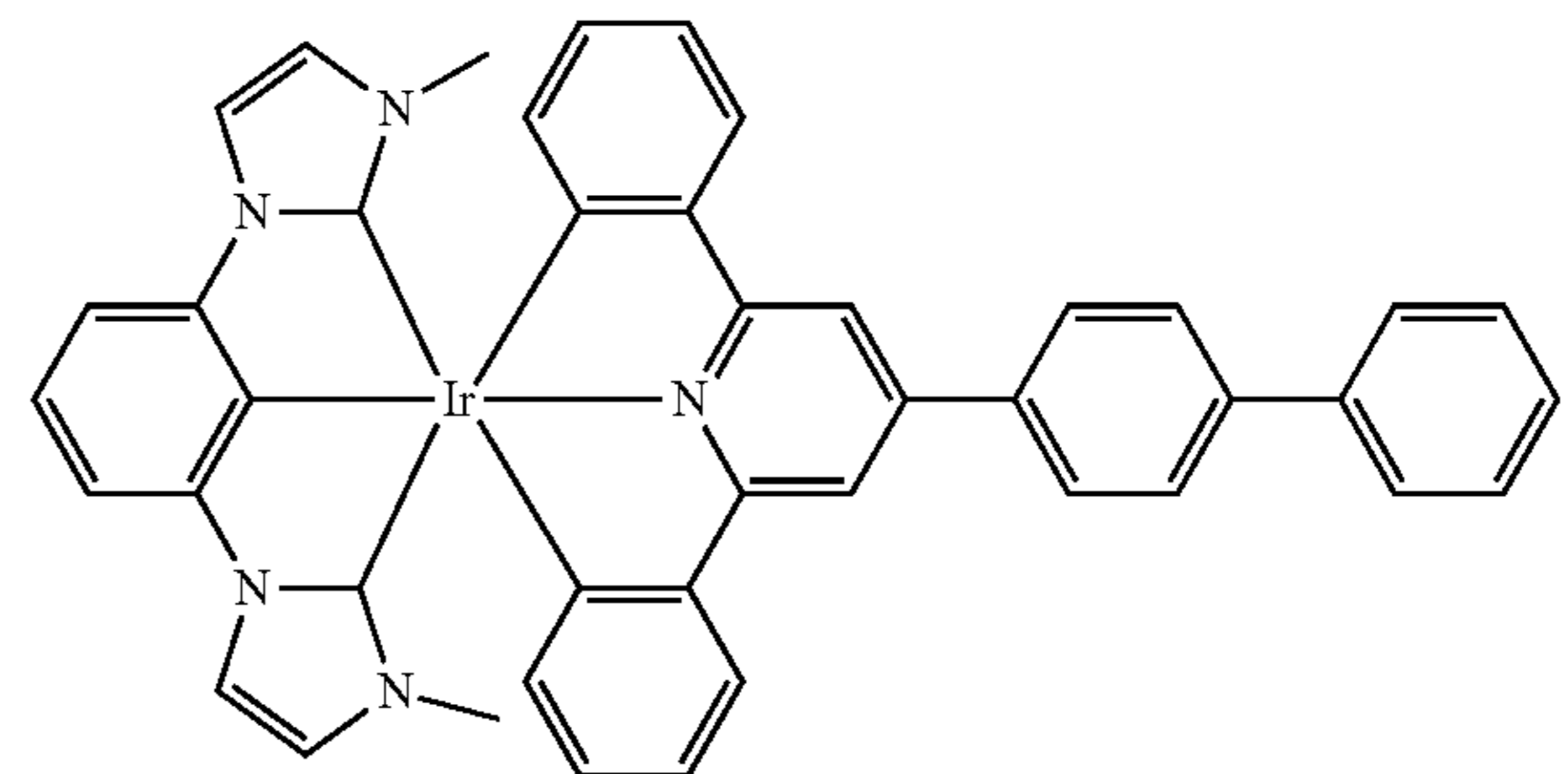
Compound 92
