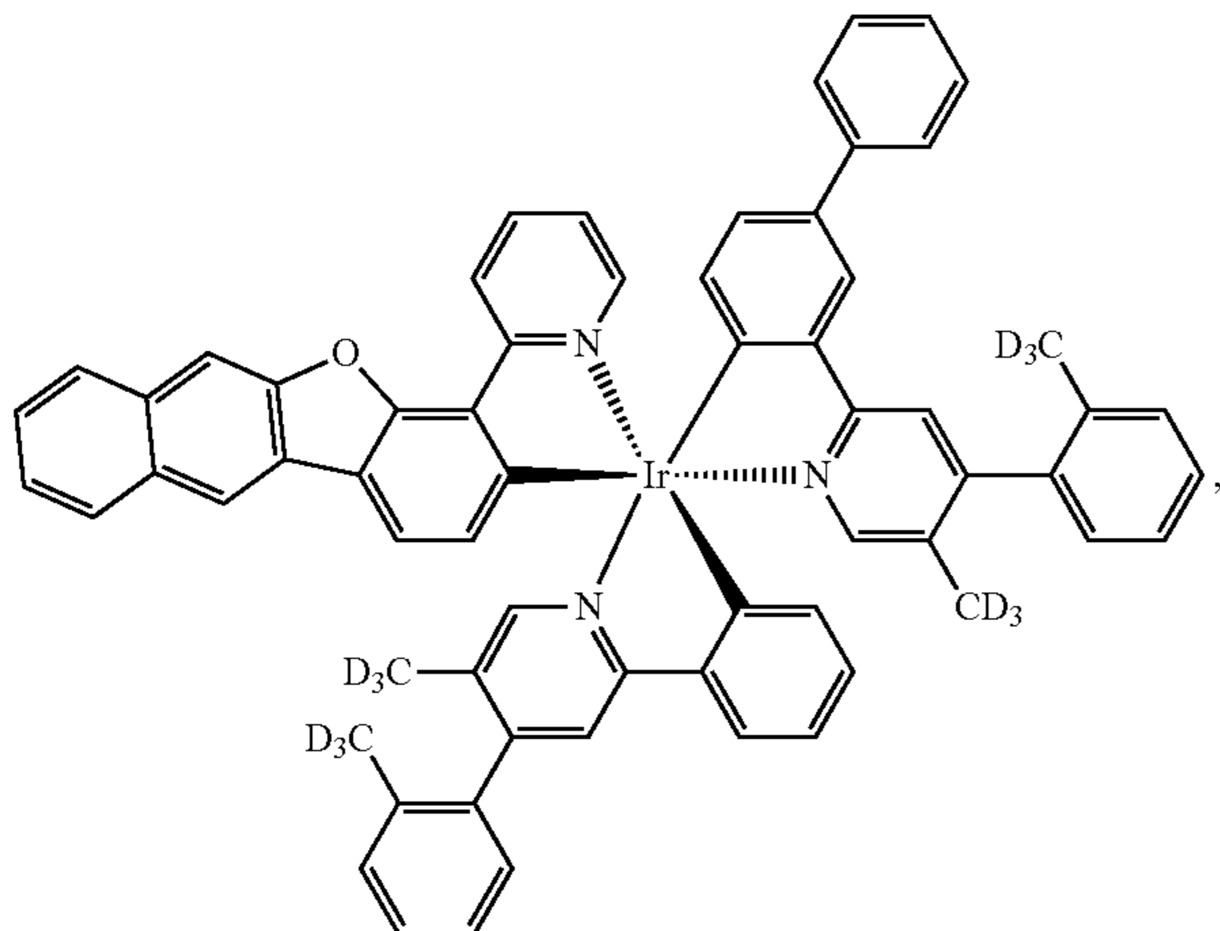
Compound 126
