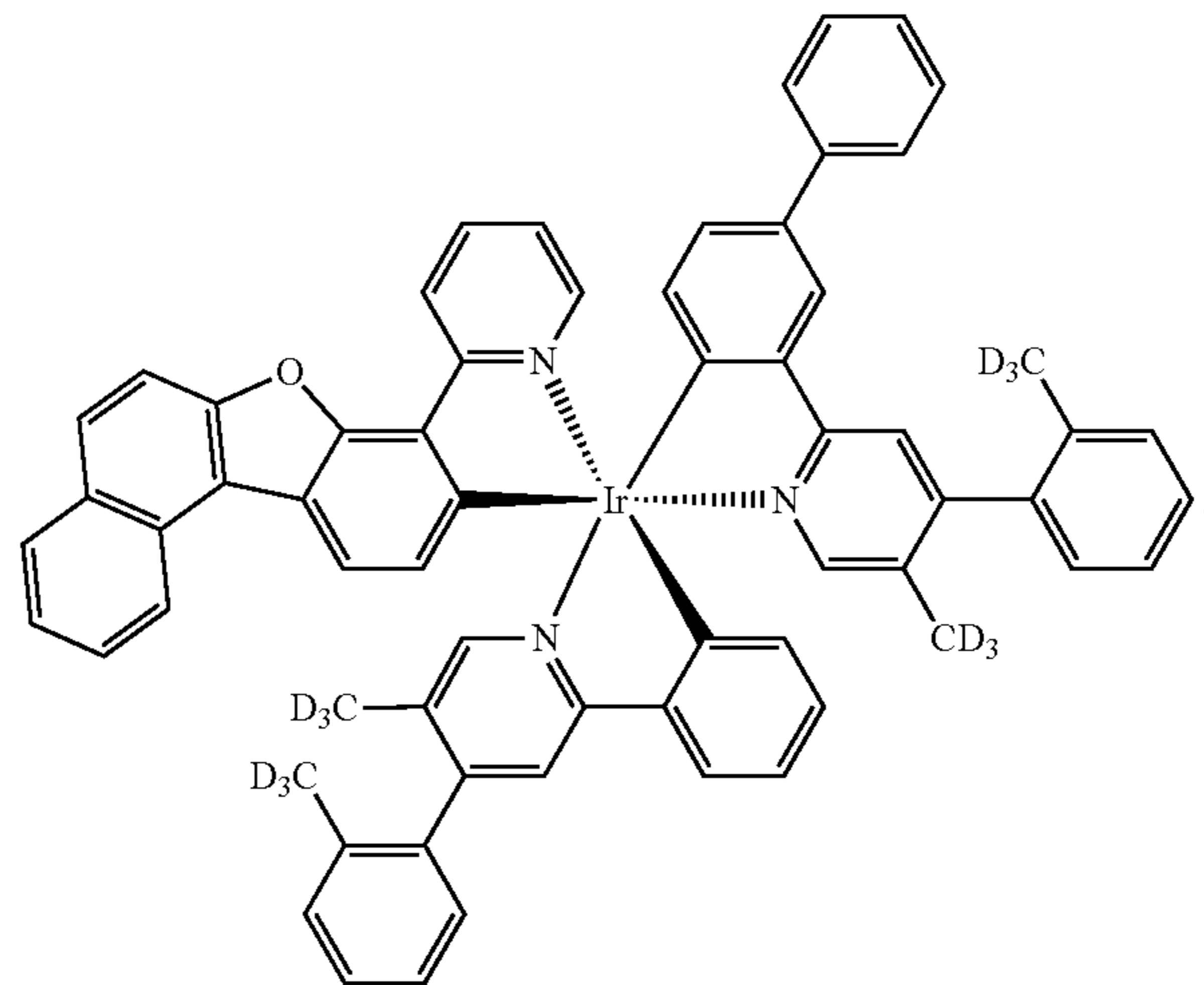
Compound 127
