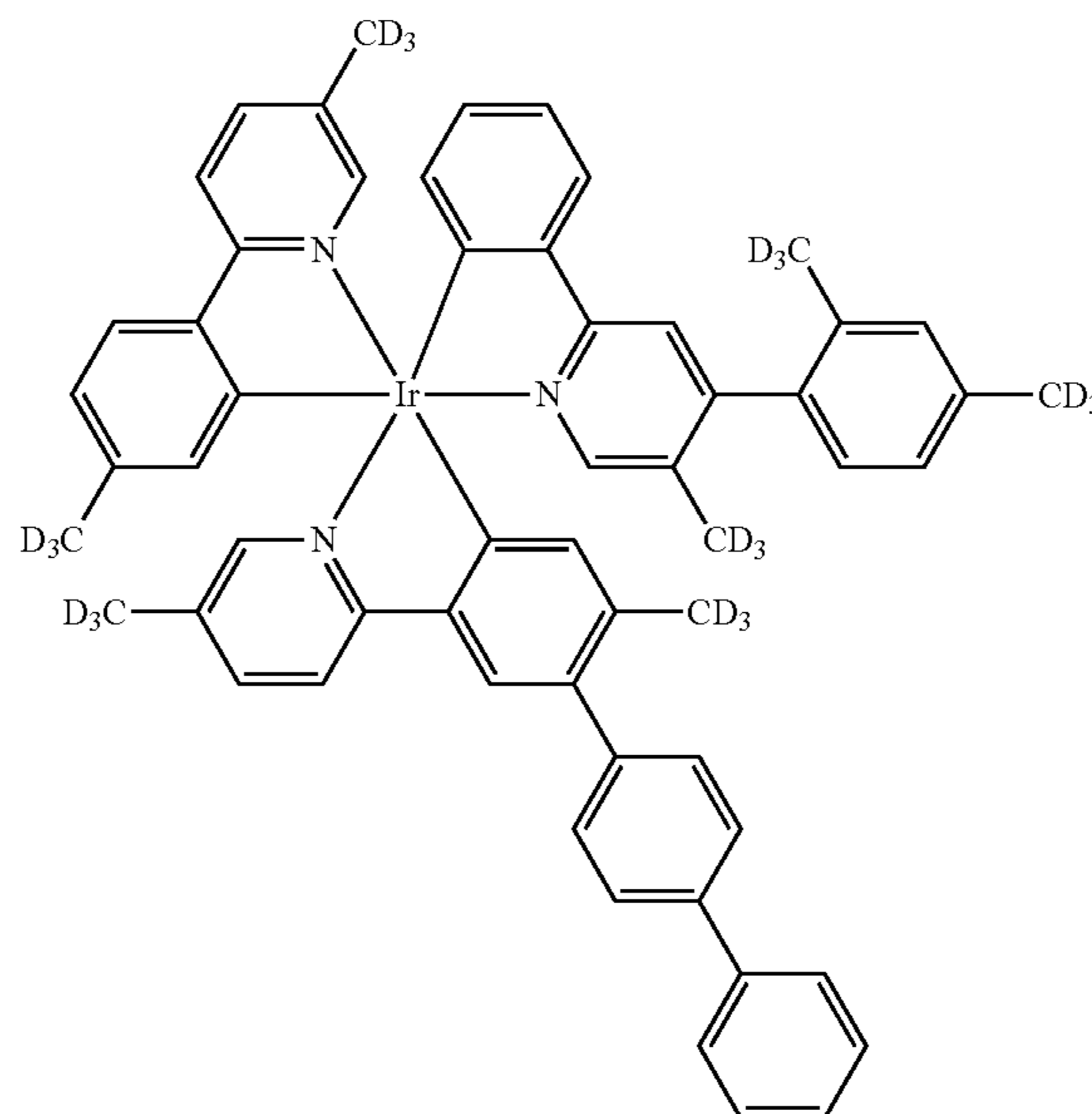
Compound 153
