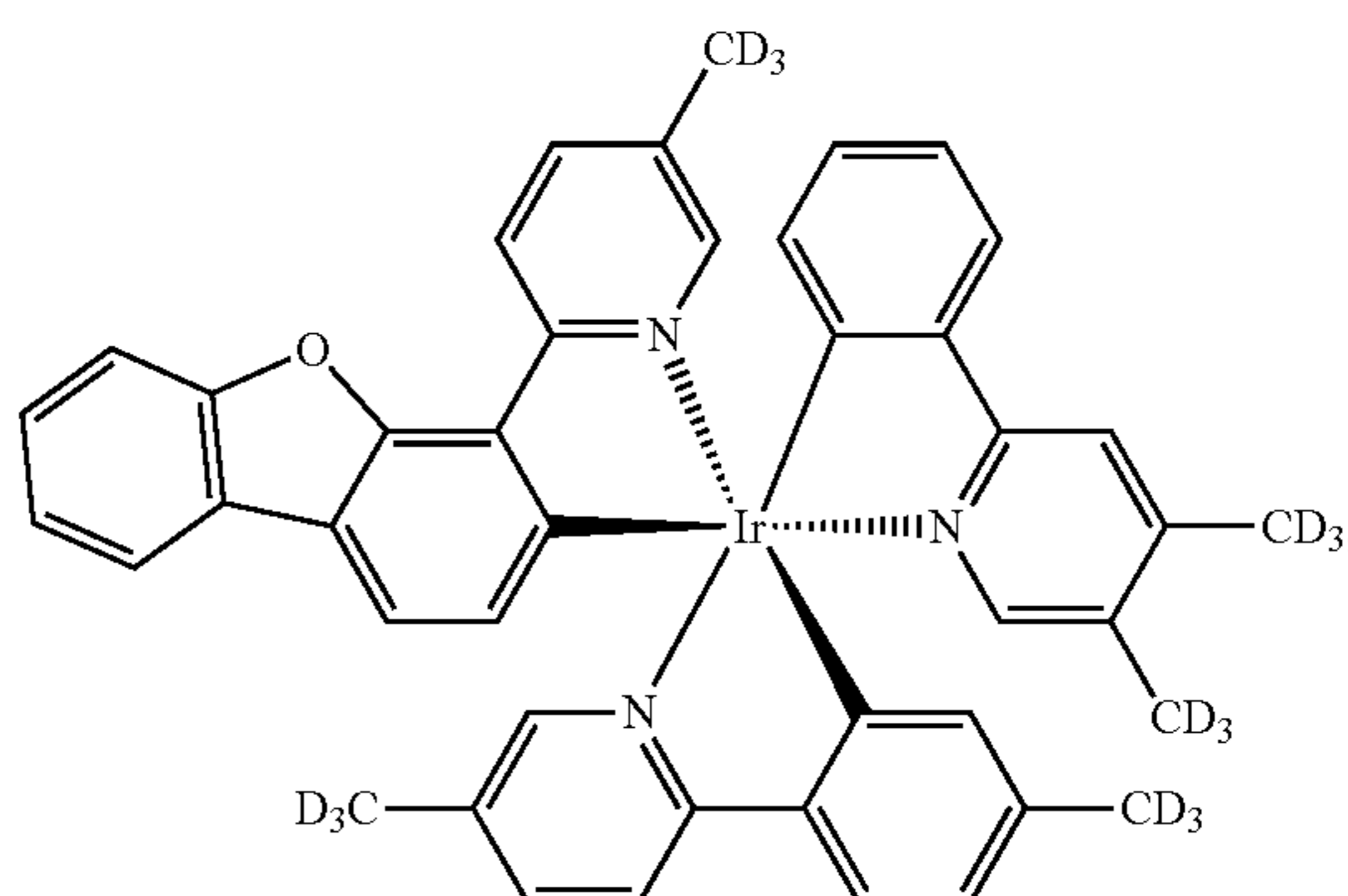
Compound 65
