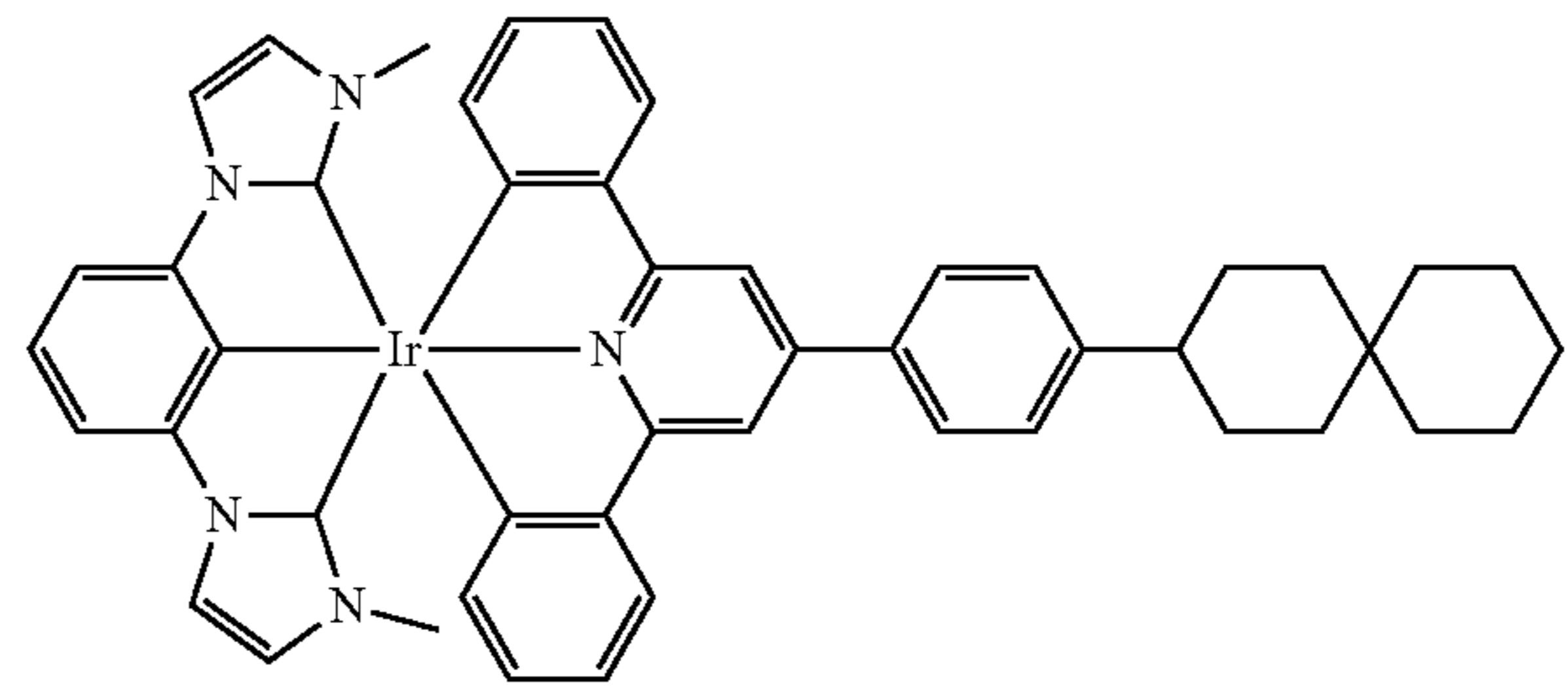
Compound 95
