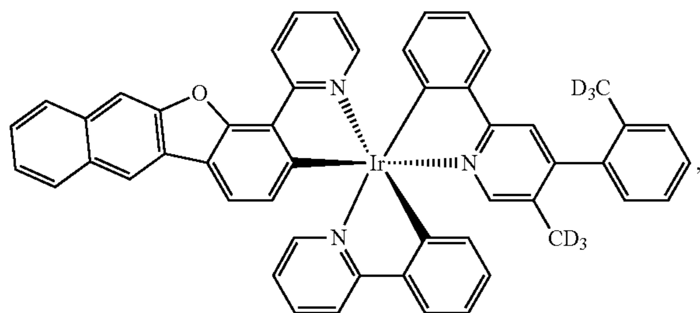
Compound 126
