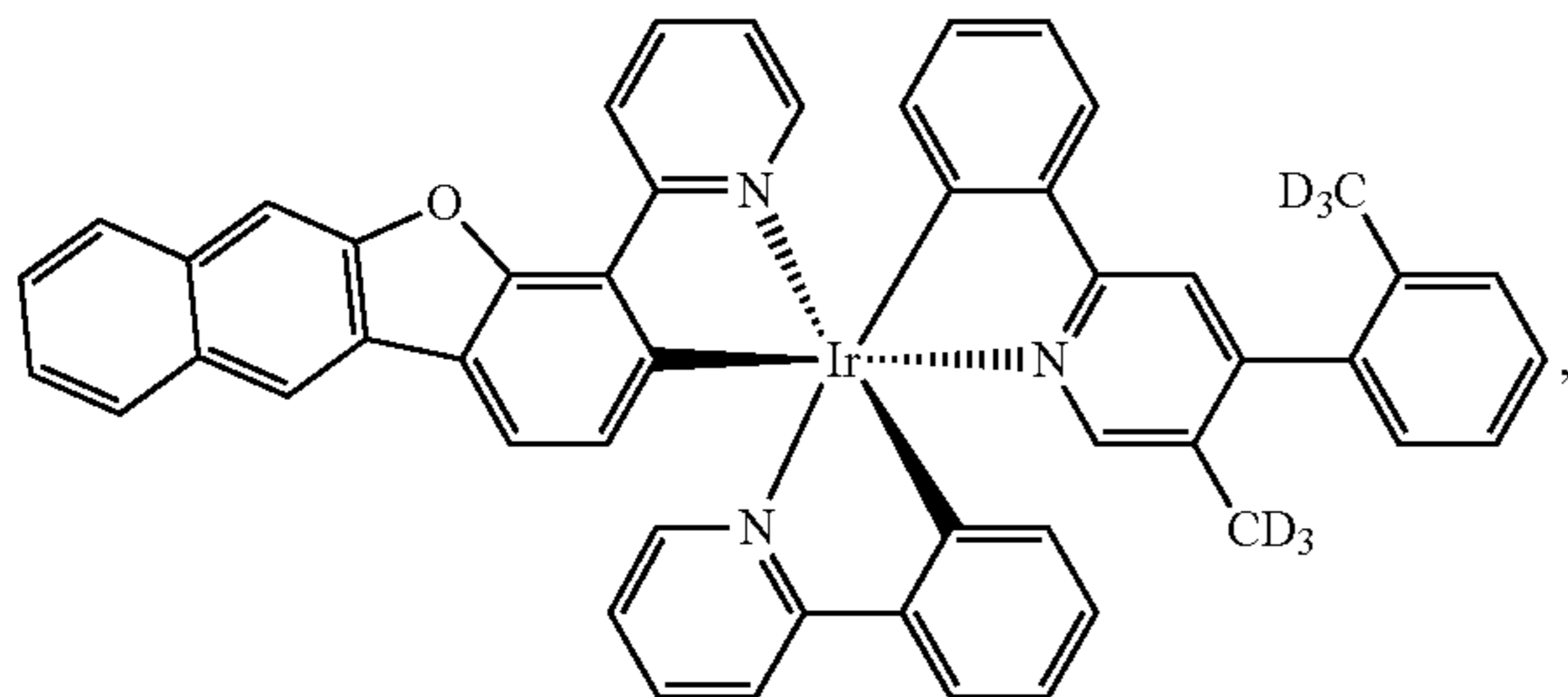
Compound 126
