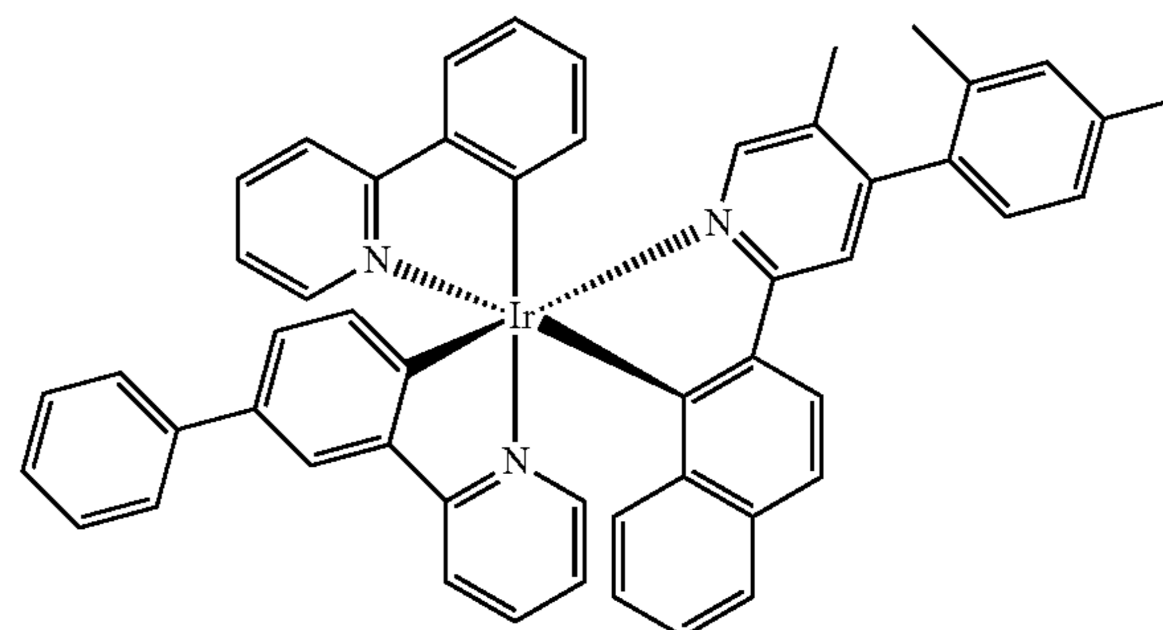
Compound 71
