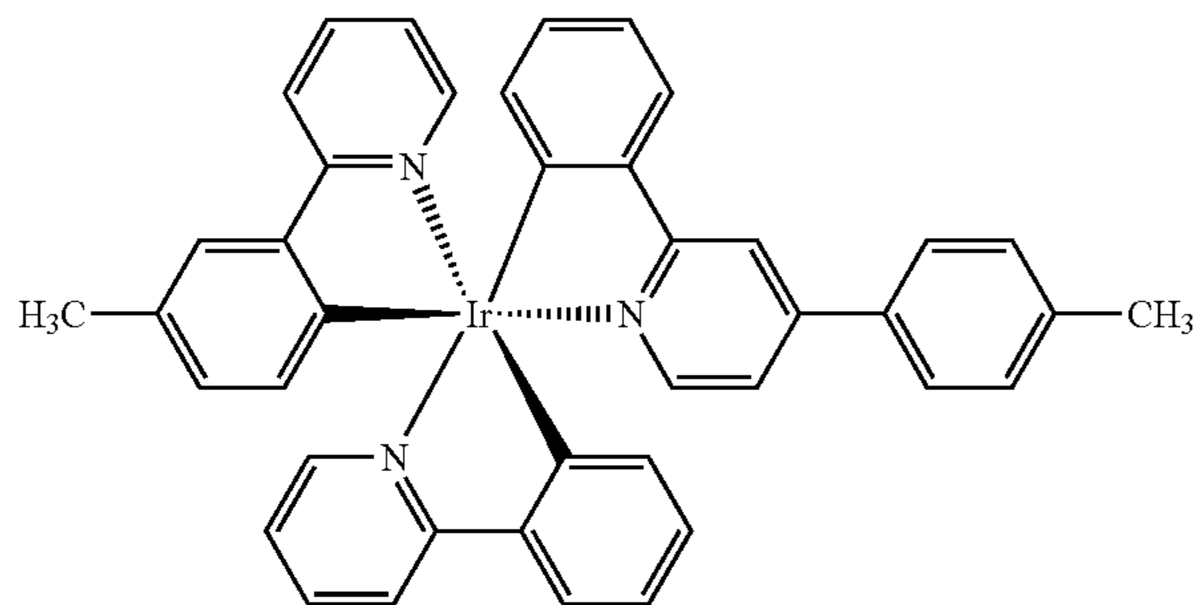
Compound 5
