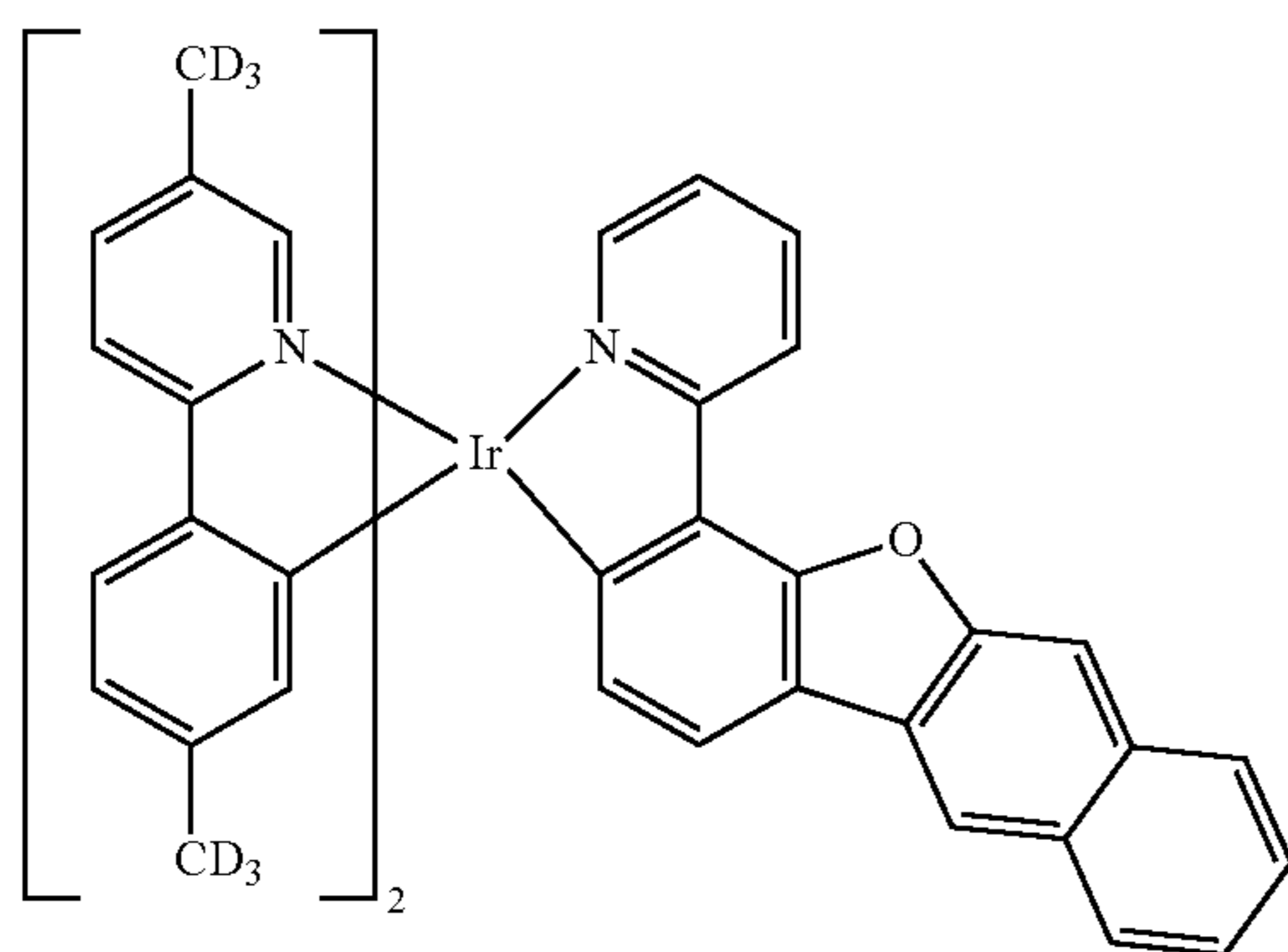
Compound B
