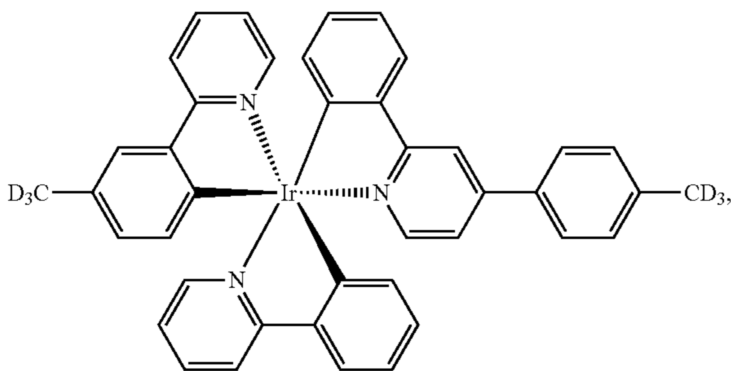
Compound 9
