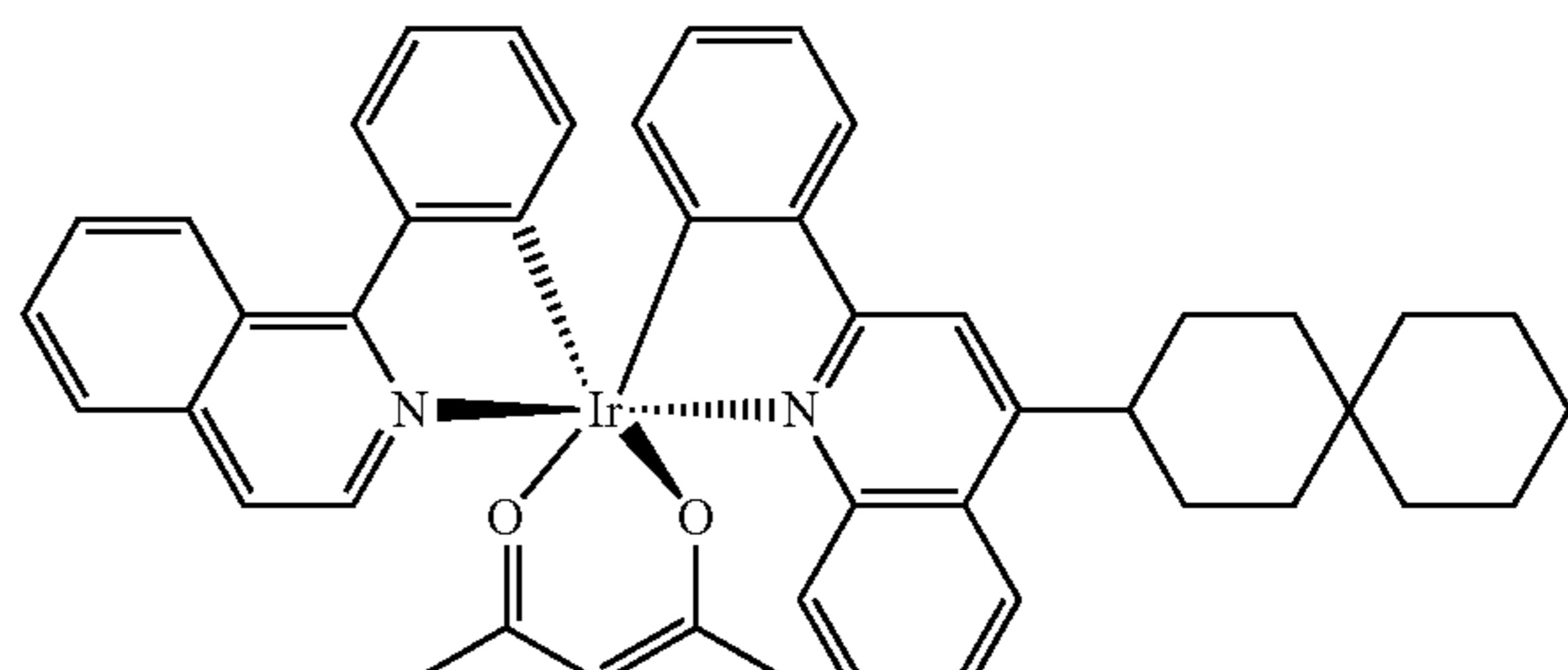
Compound 57
