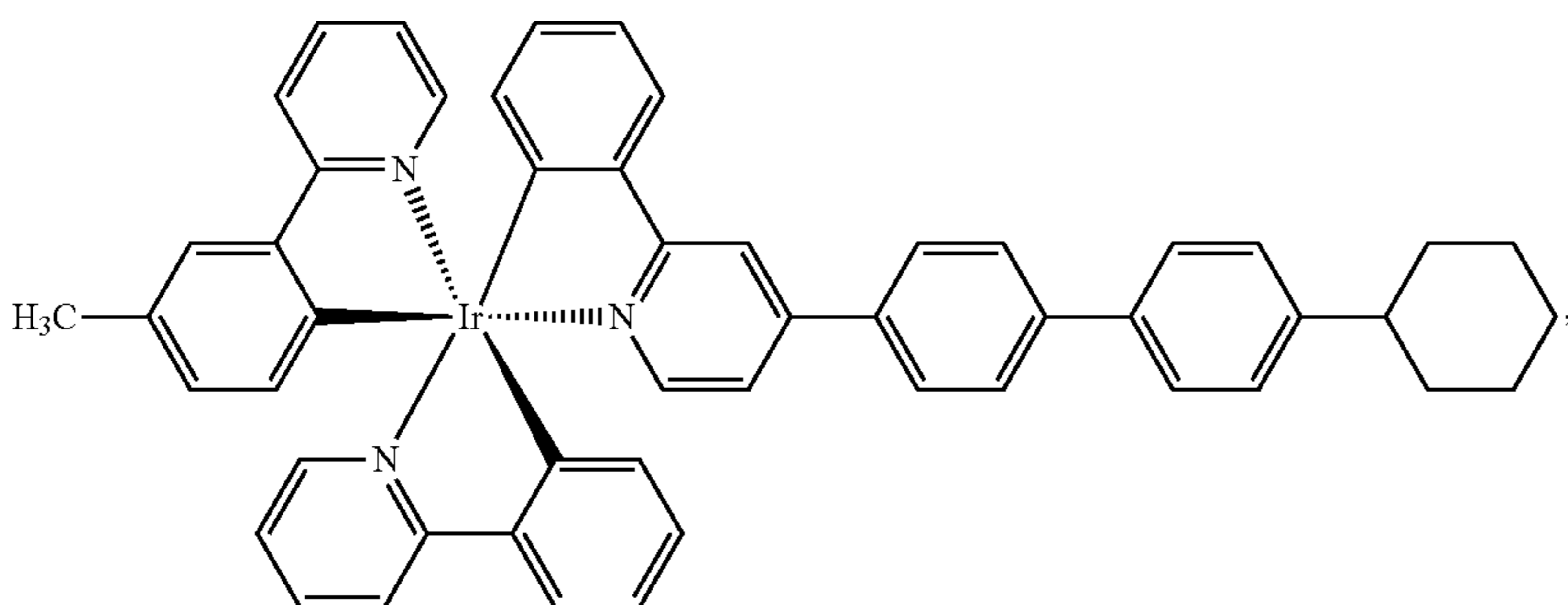
Compound 9
