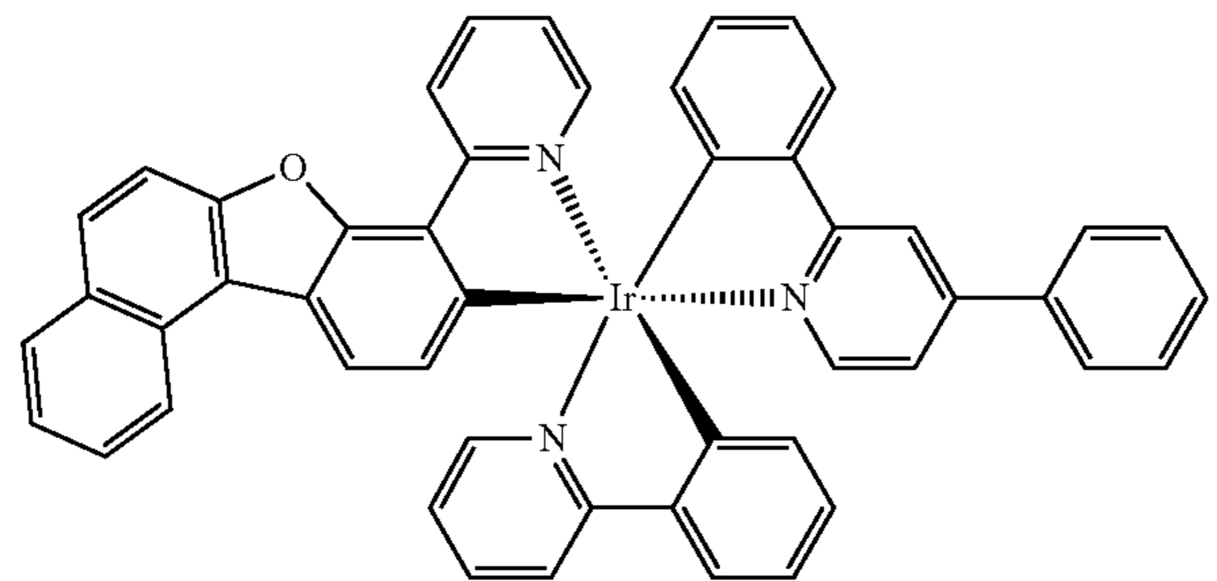
Compound 125
