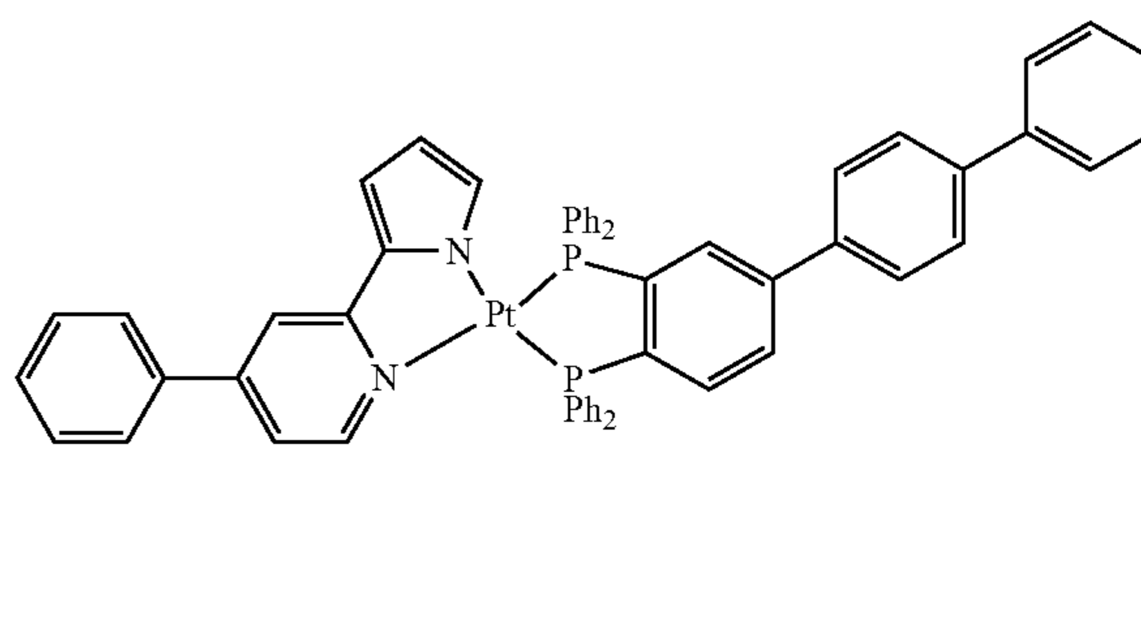
Compound 140
