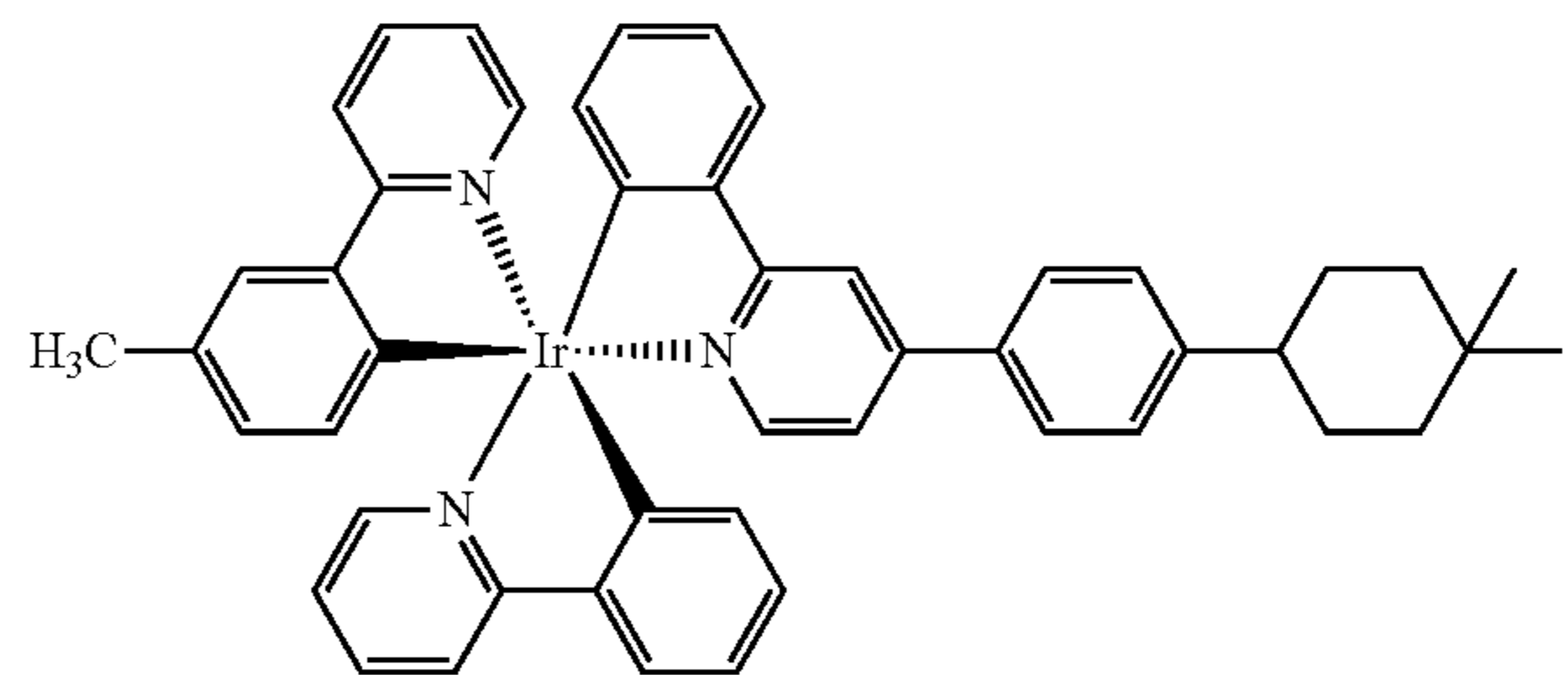
Compound 6
