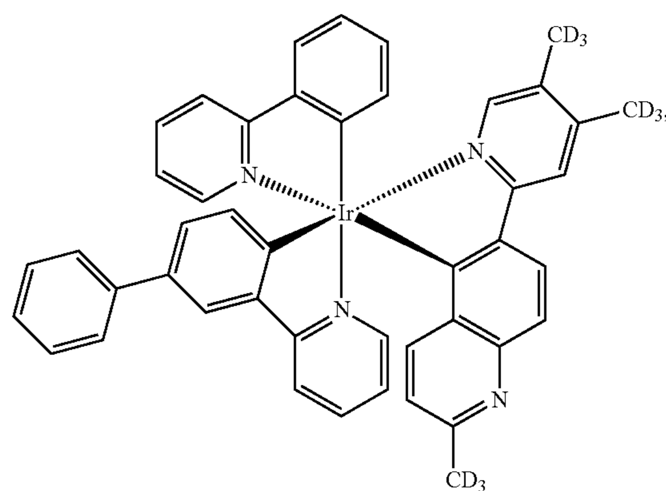
Compound 75
