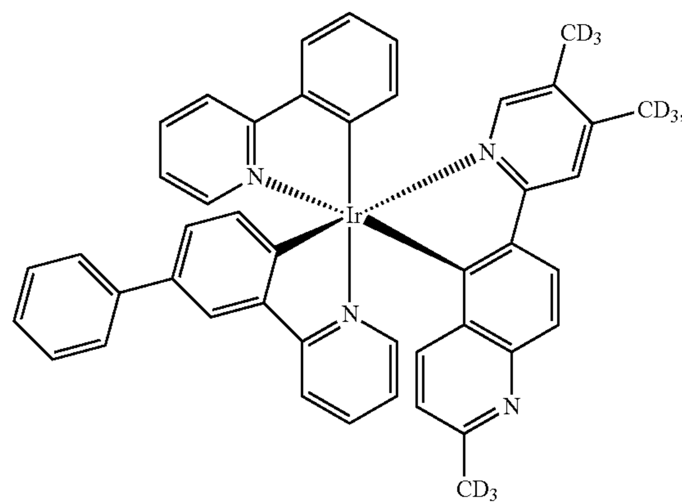
Compound 75
