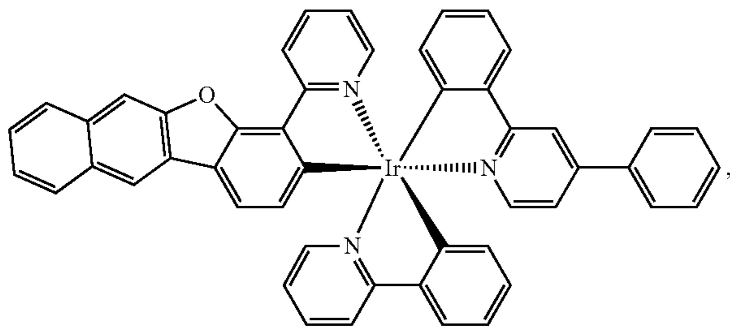
Compound 124
