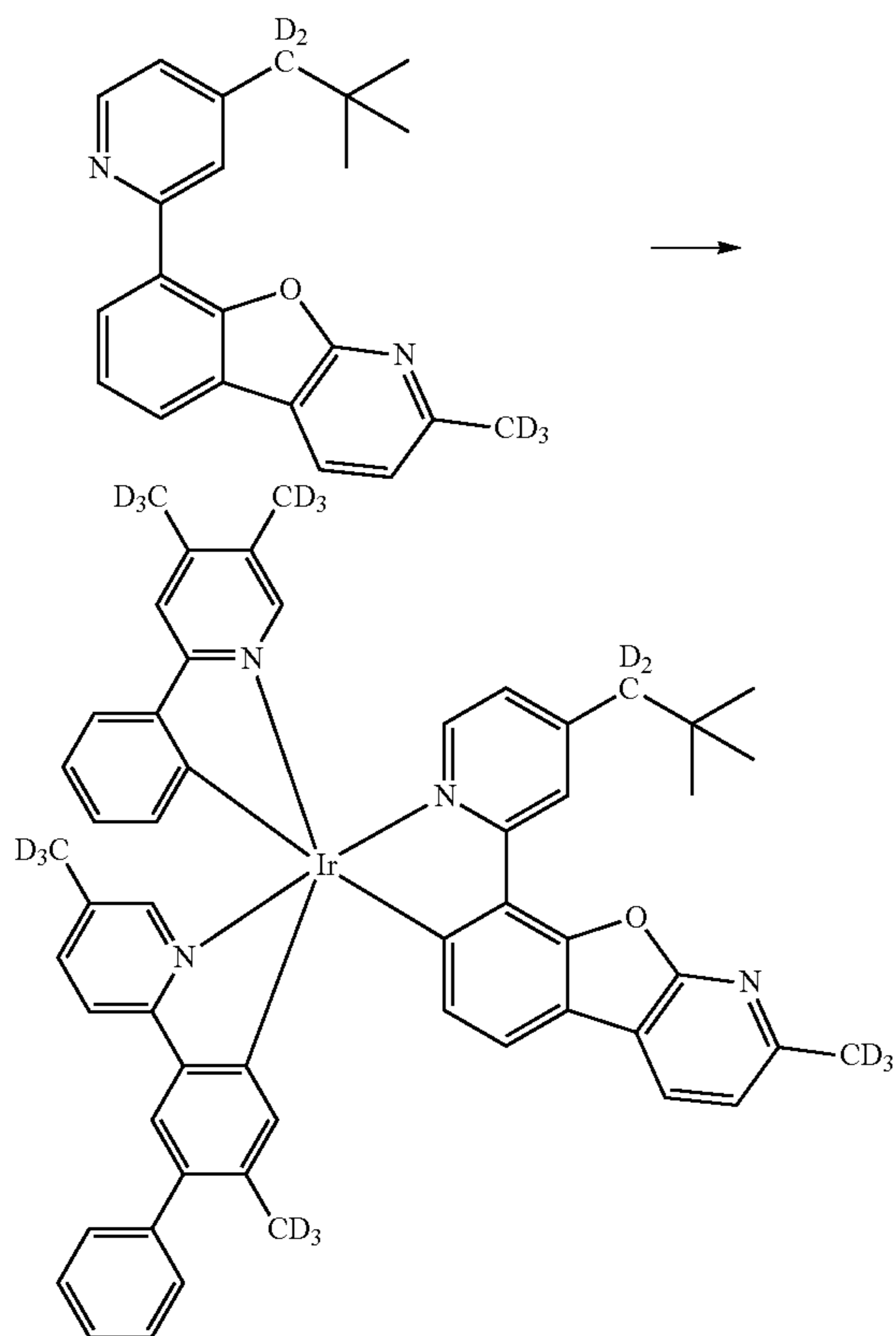
Compound 155
