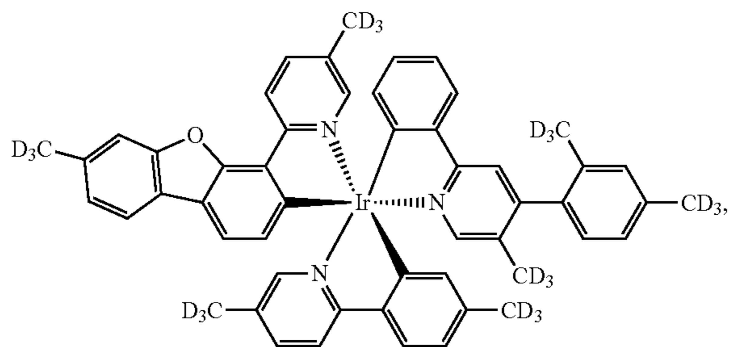
Compound 62
