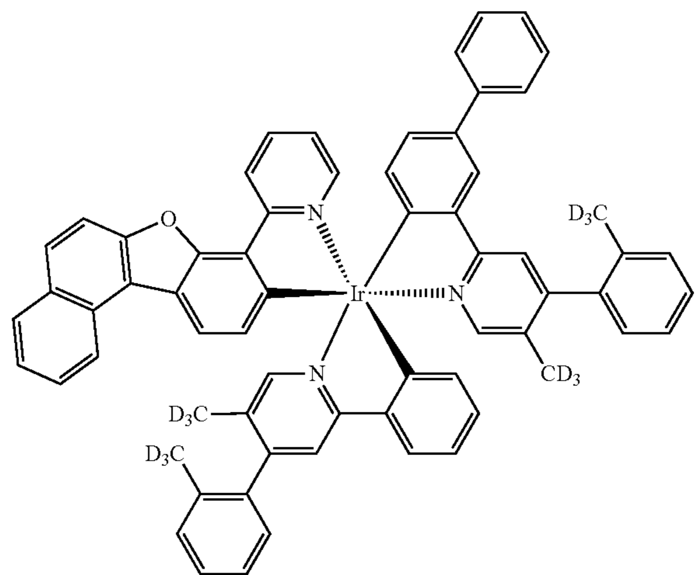
Compound 127
