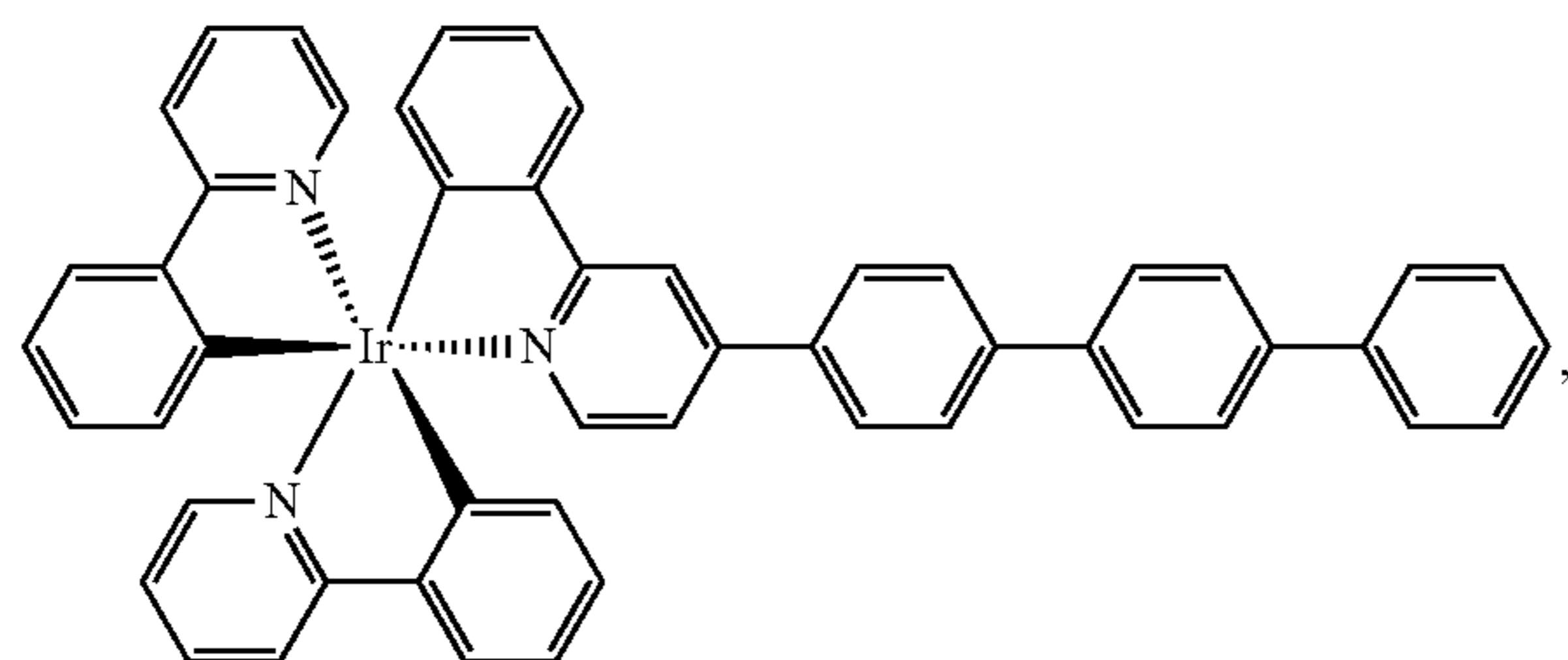
Compound 56
