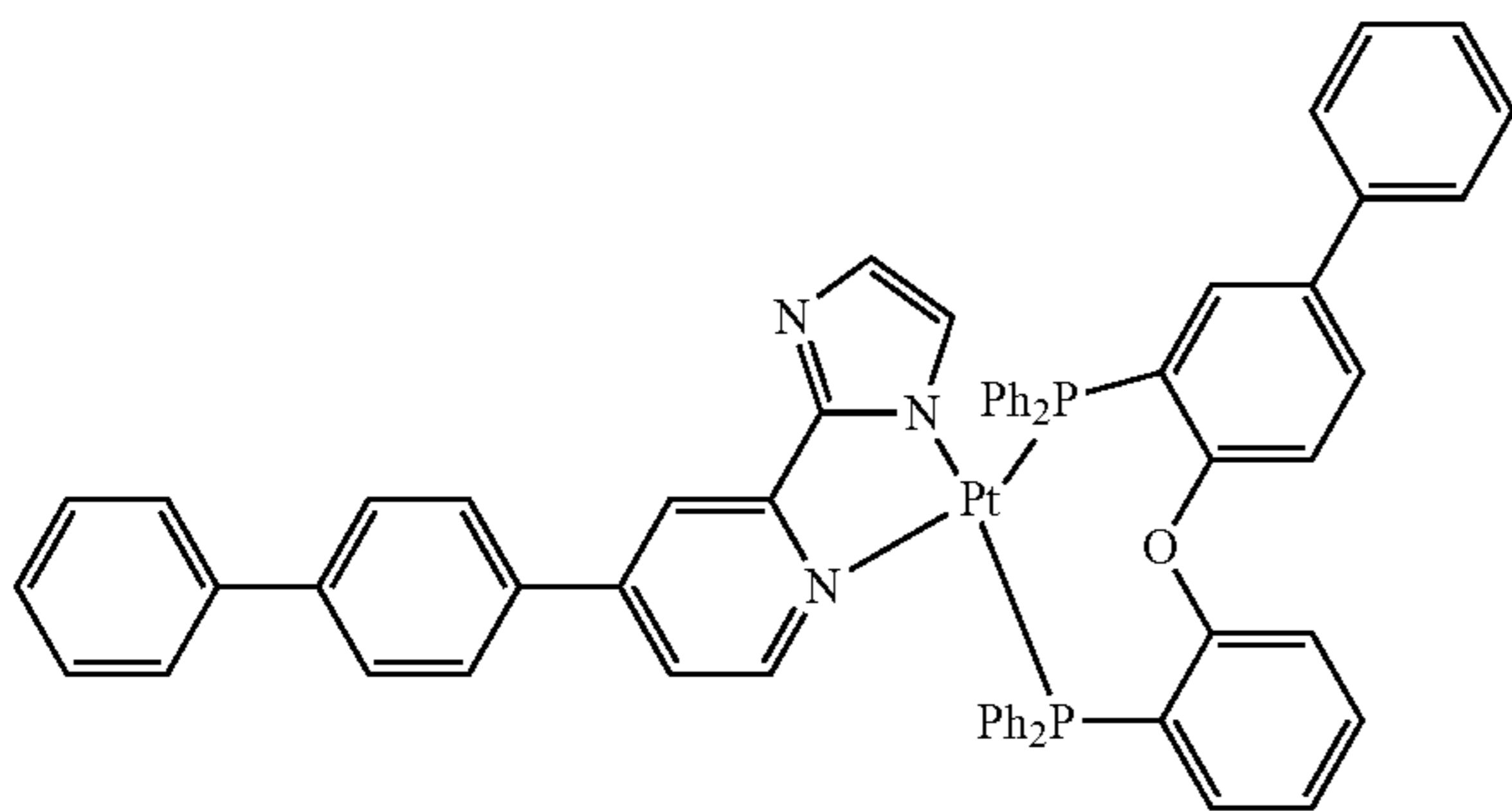
Compound 143
