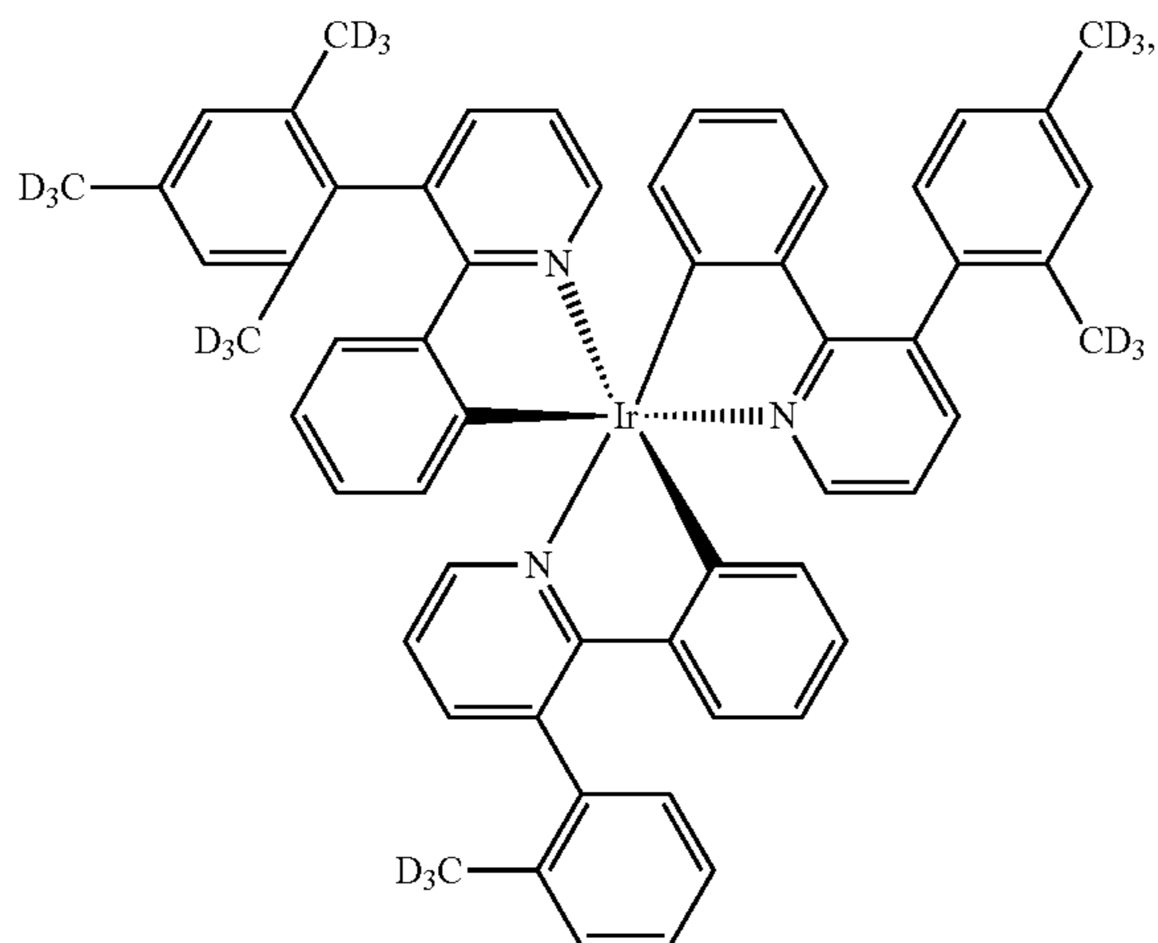
Compound 56
