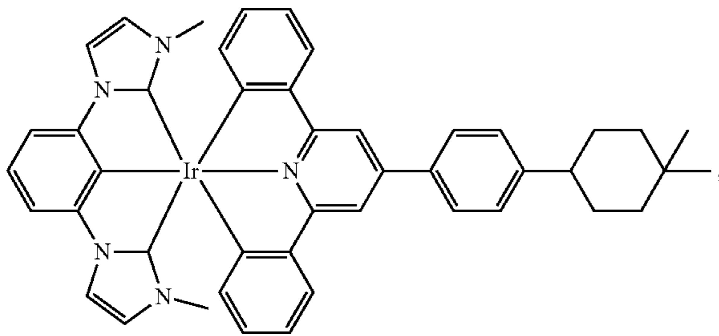
Compound 93
