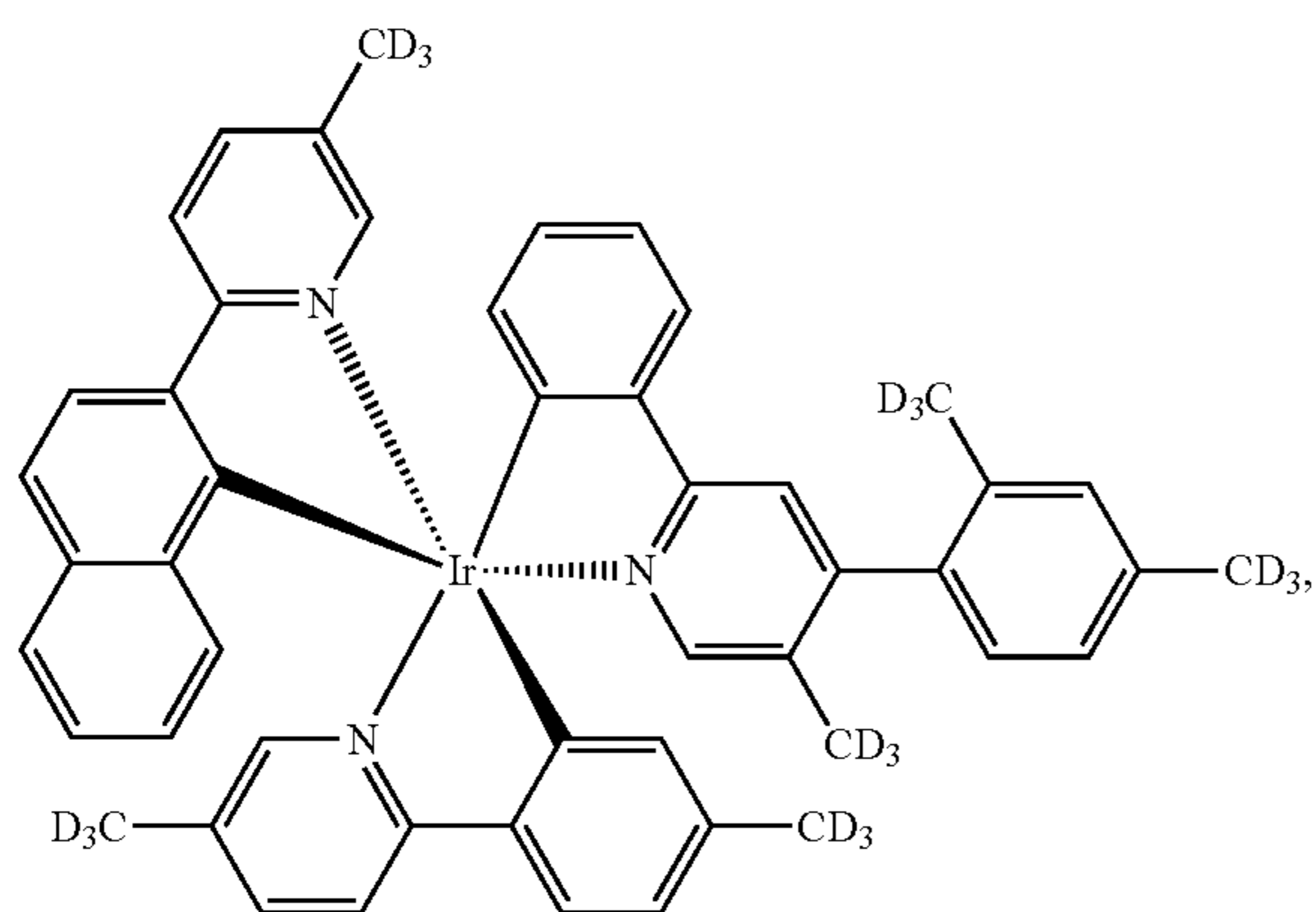
Compound 66
