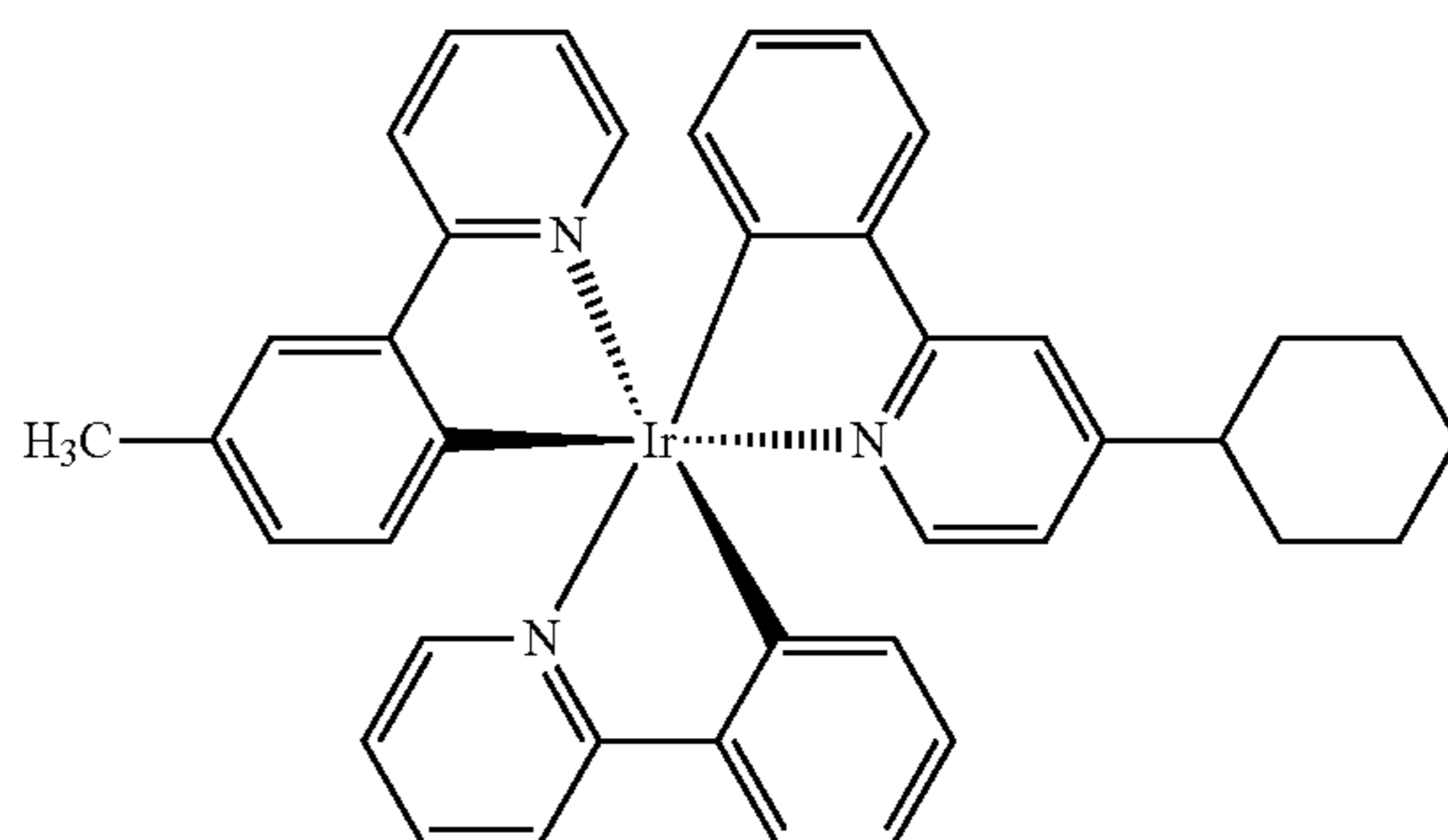
Compound 2
