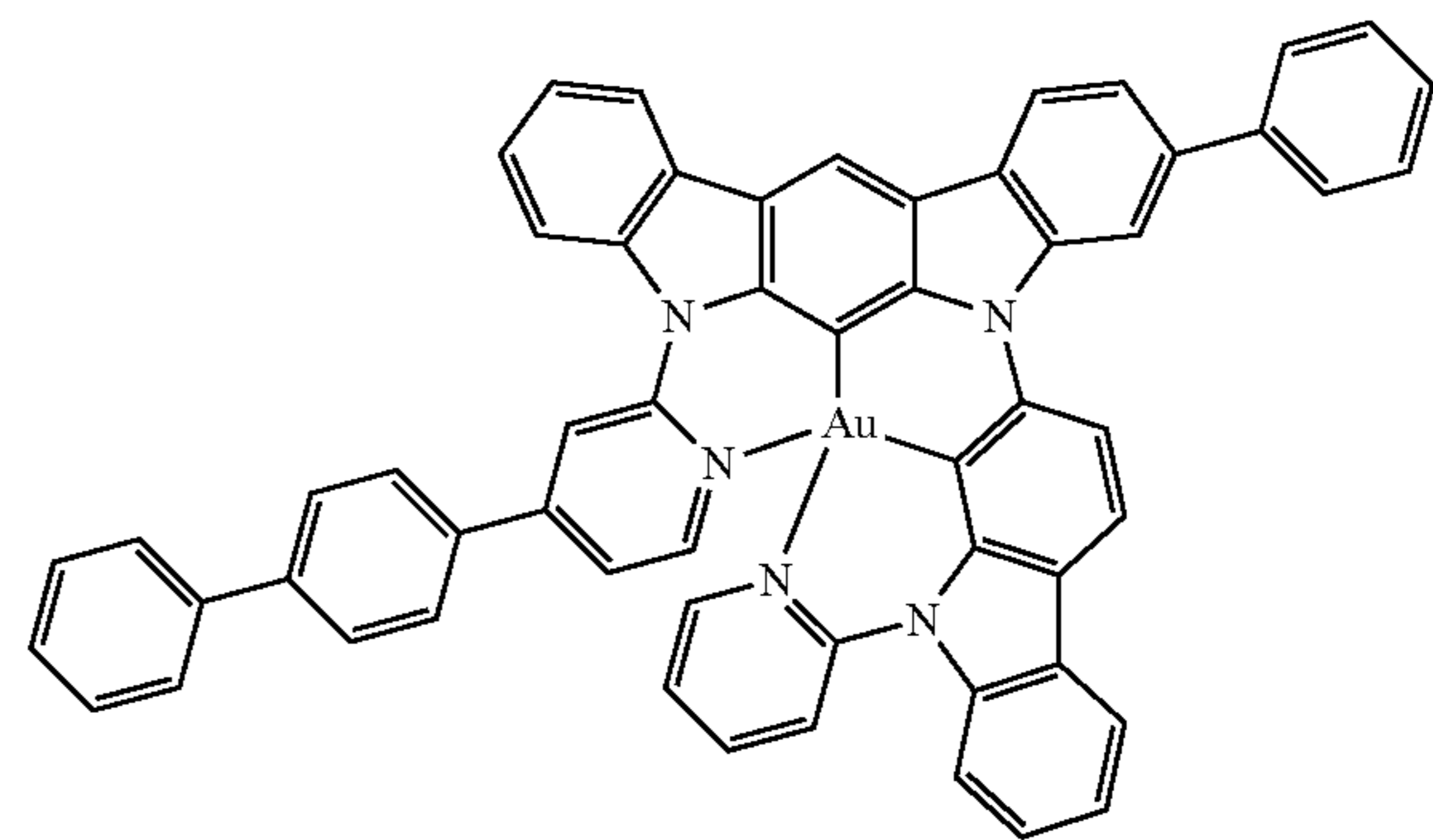
Compound 92
