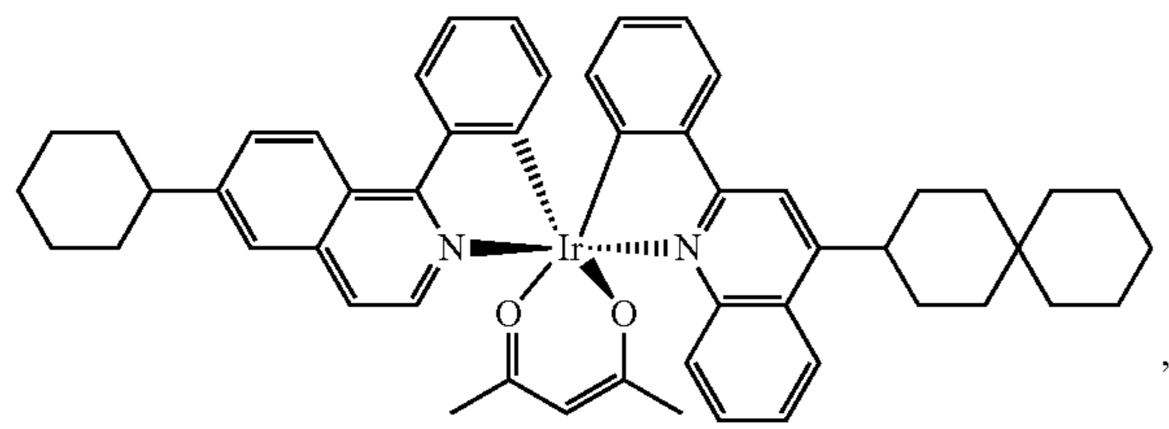
Compound 58
