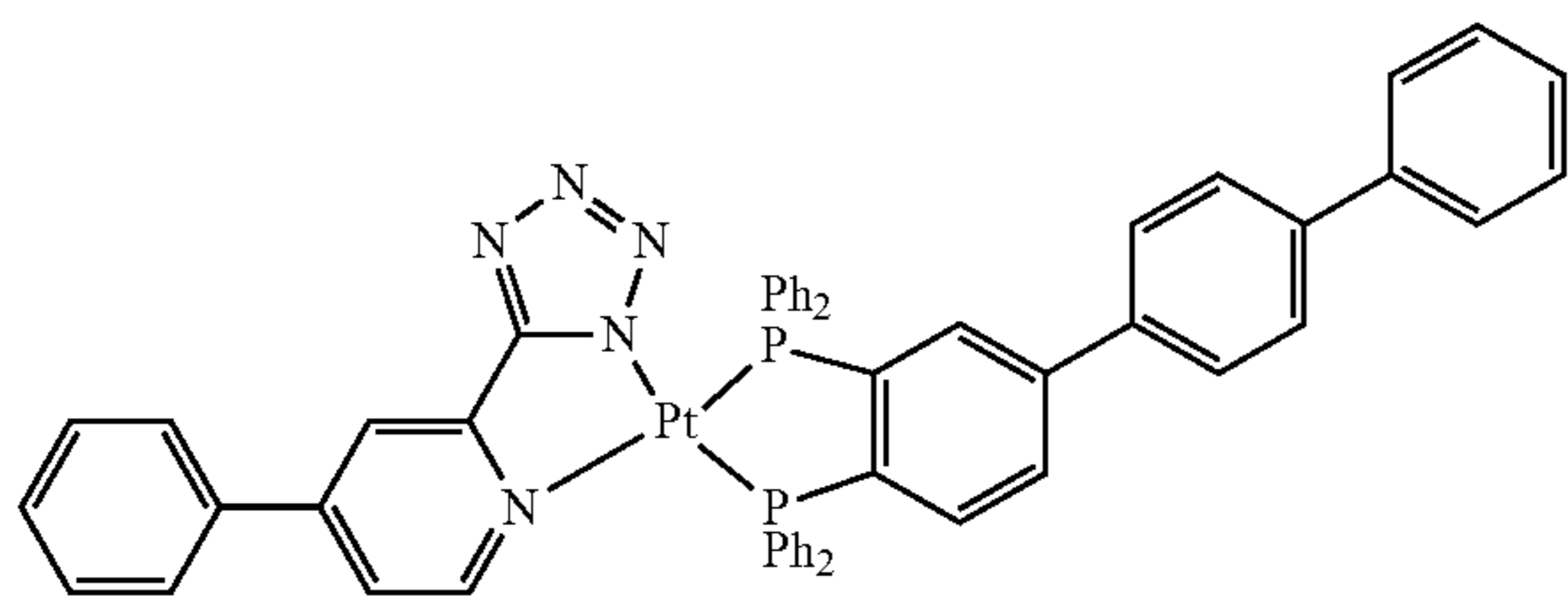
Compound 137
