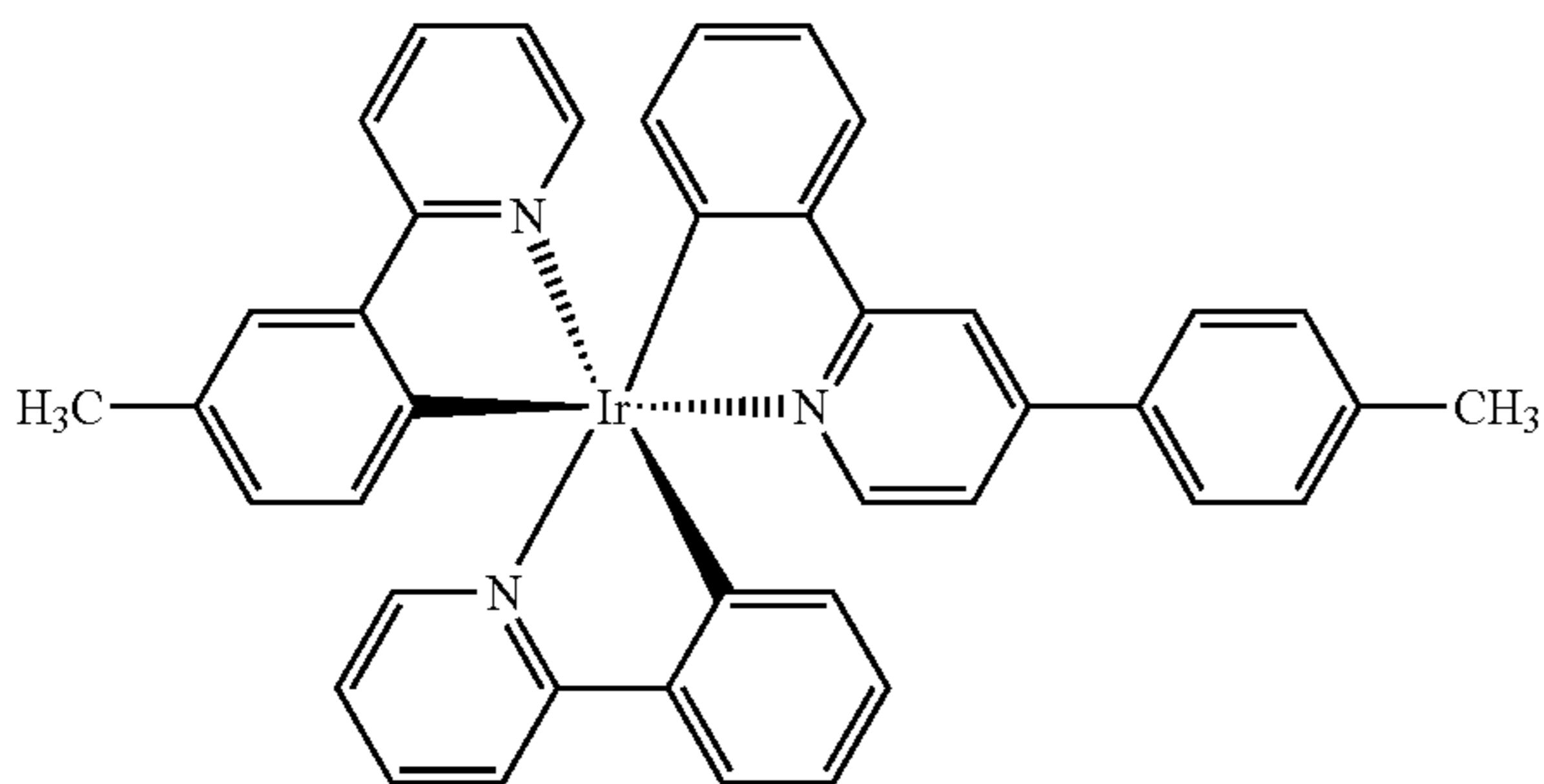
Compound 5
