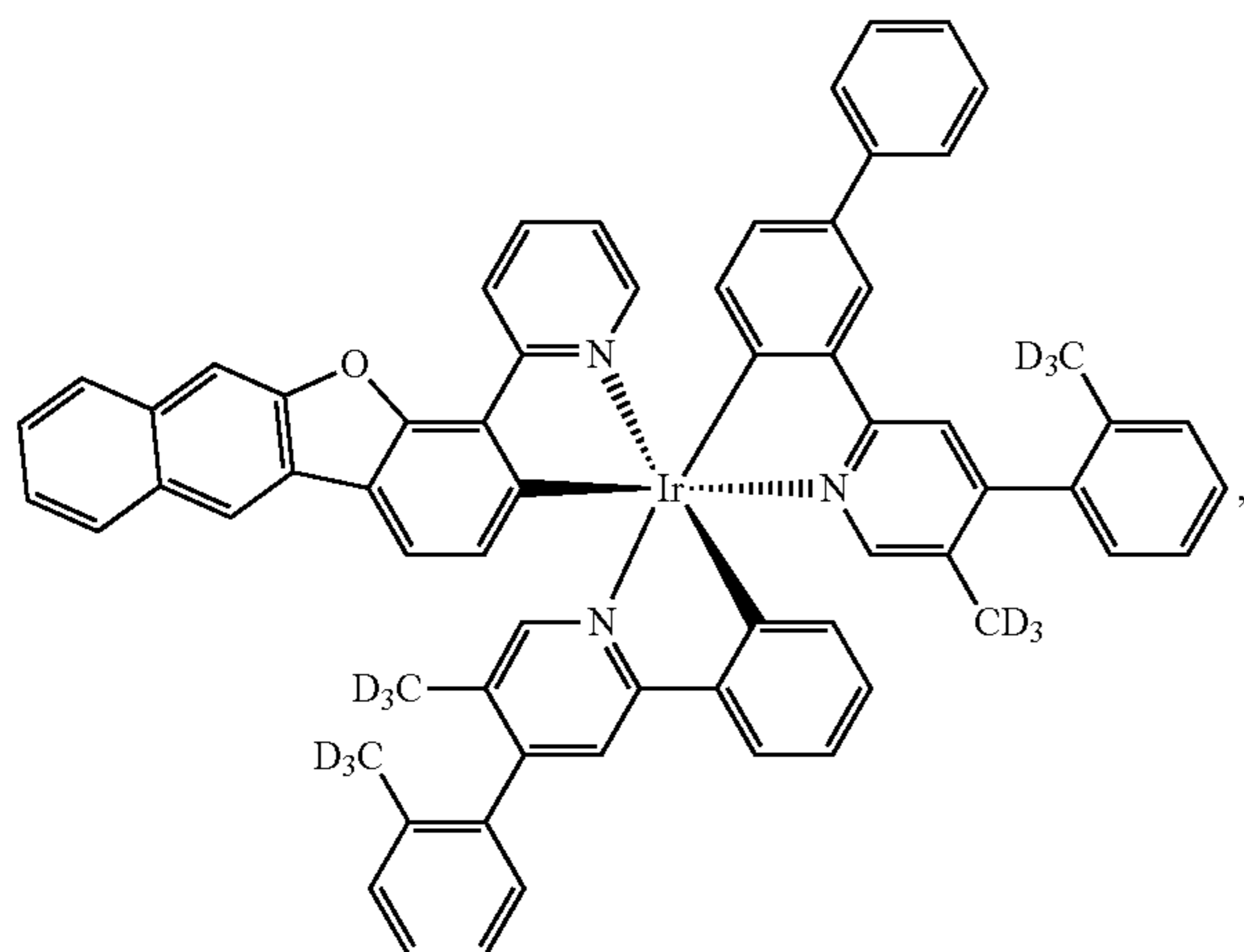
Compound 126
