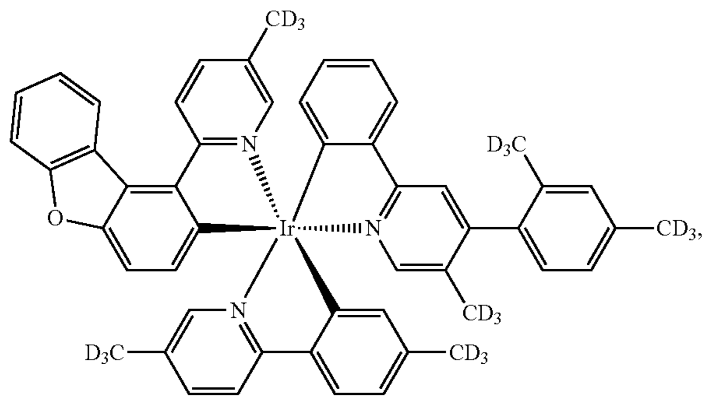
Compound 60
