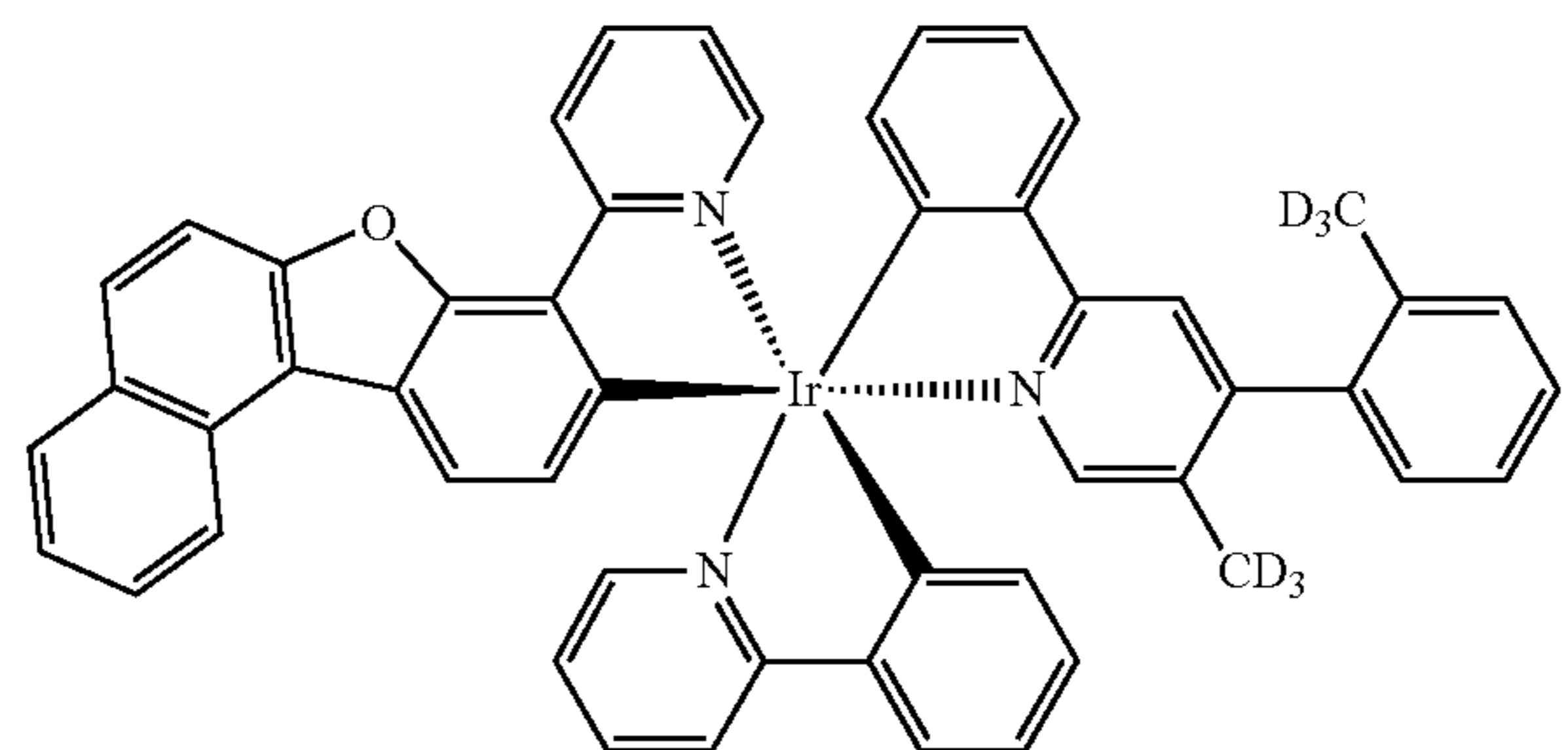
Compound 127
