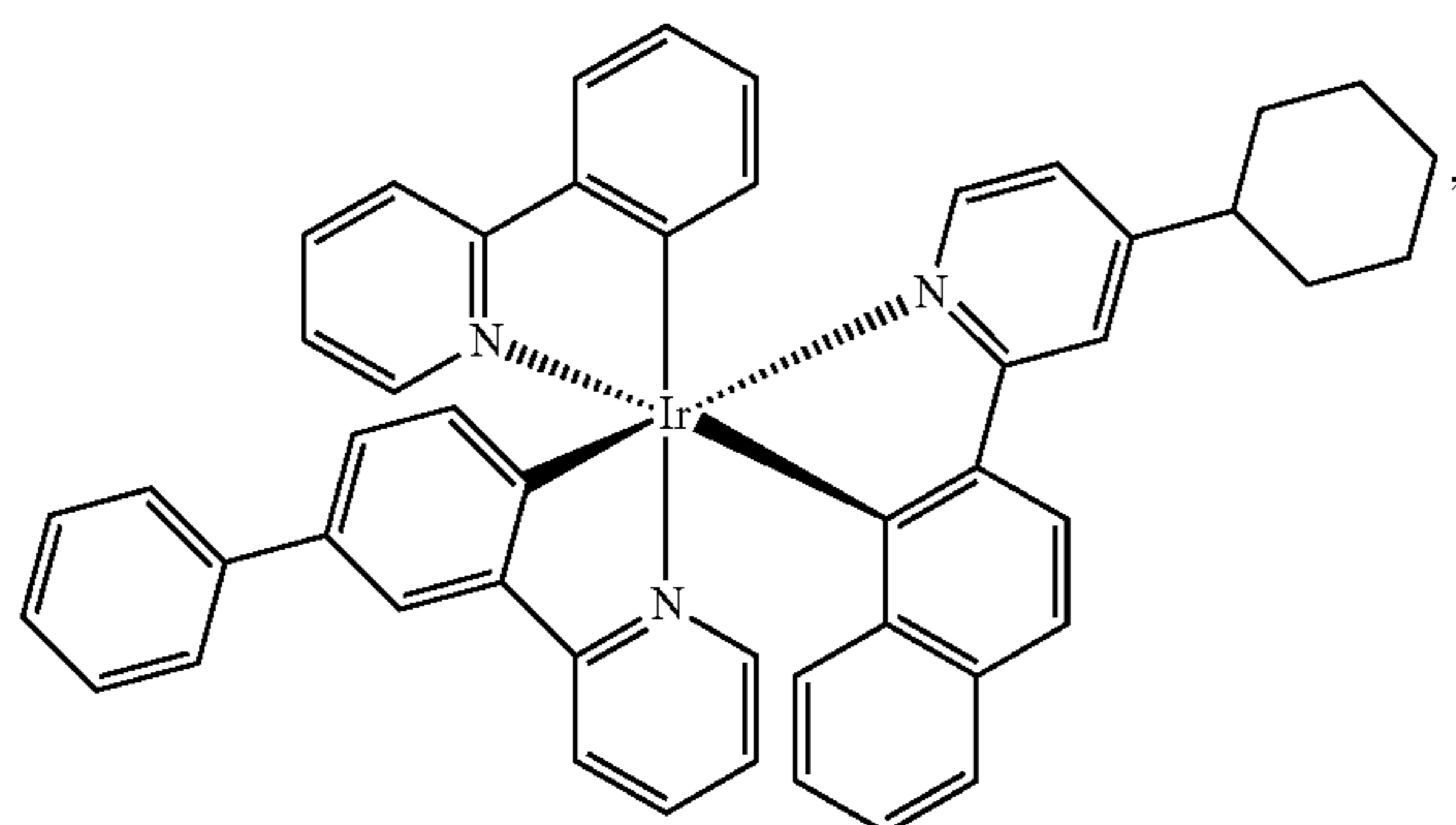
Compound 72
