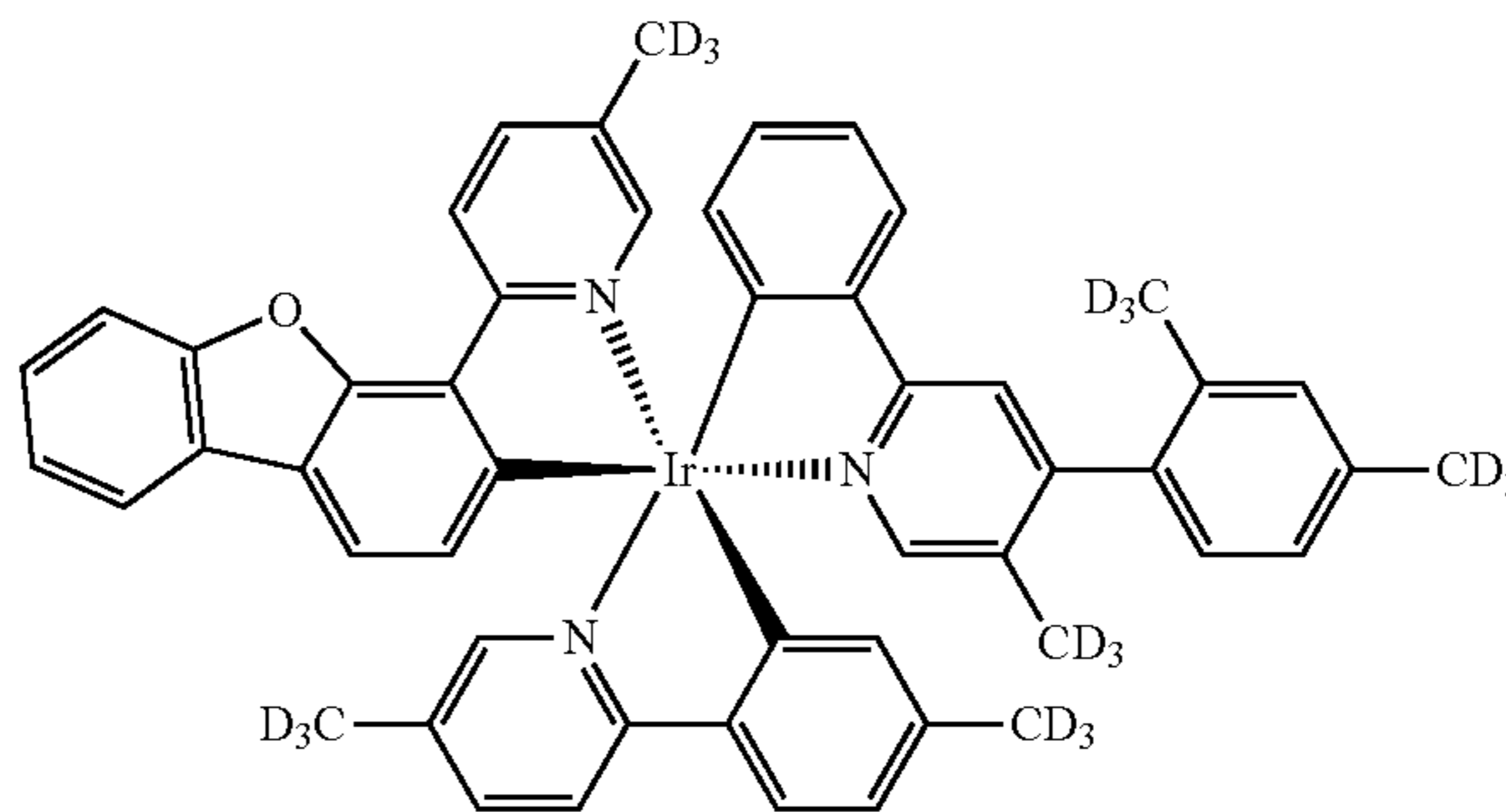
Compound 59
