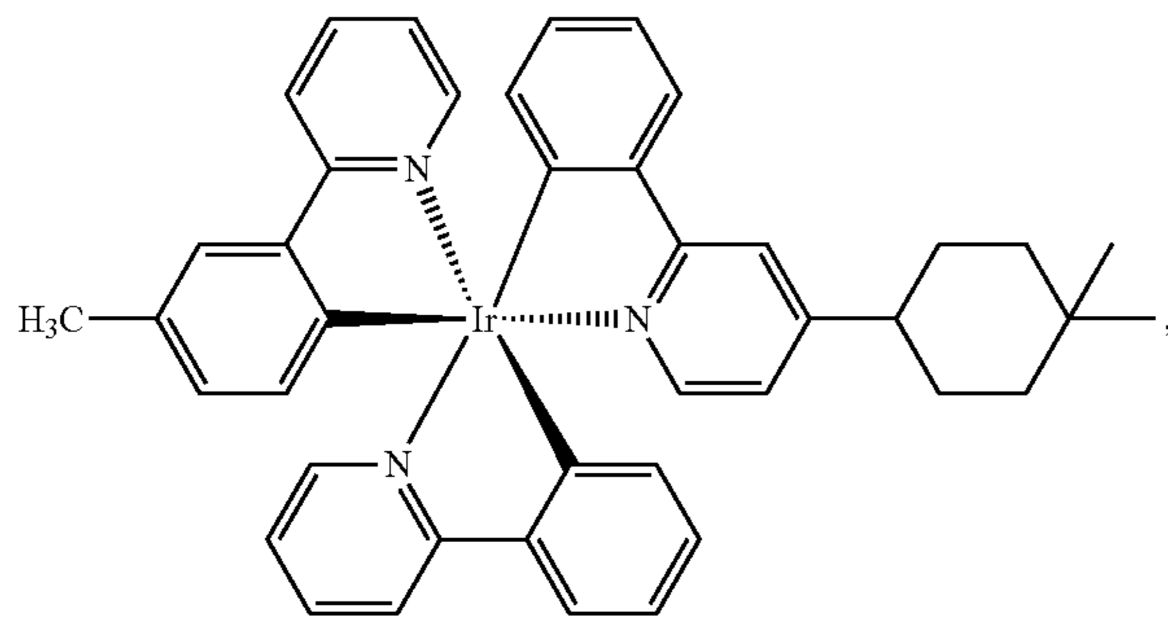
Compound 5
