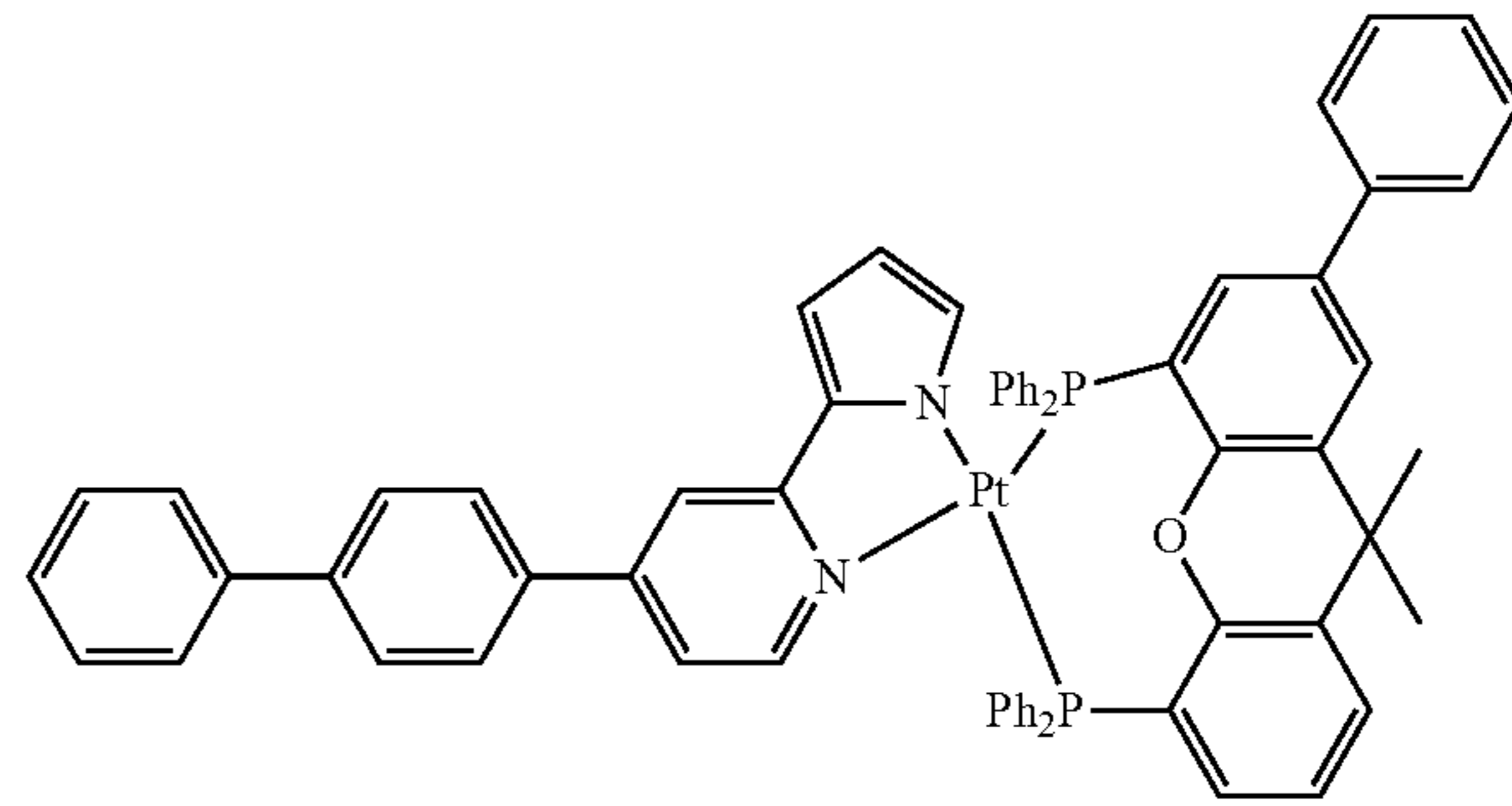
Compound 142
