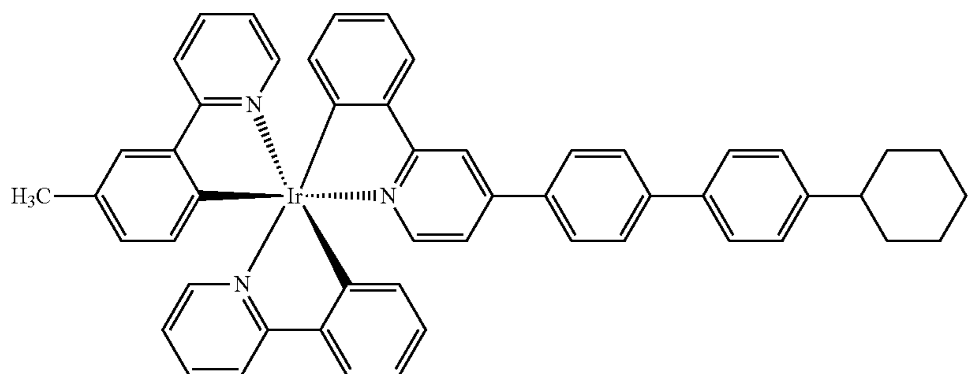
Compound 9
