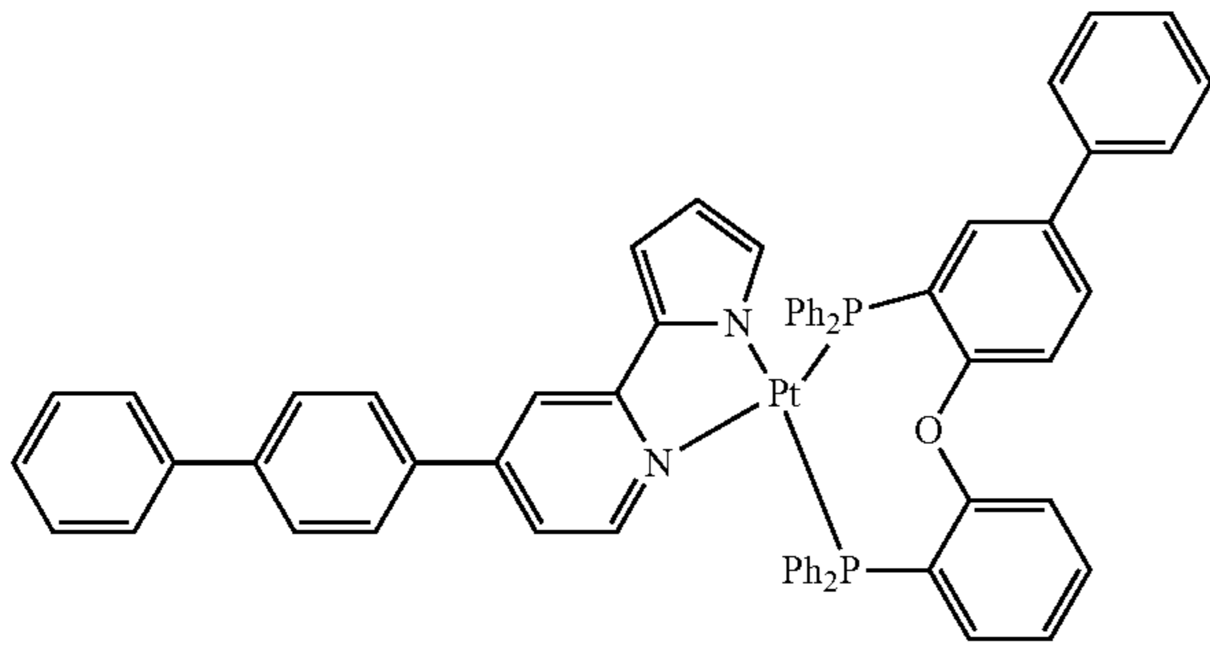
Compound 141
