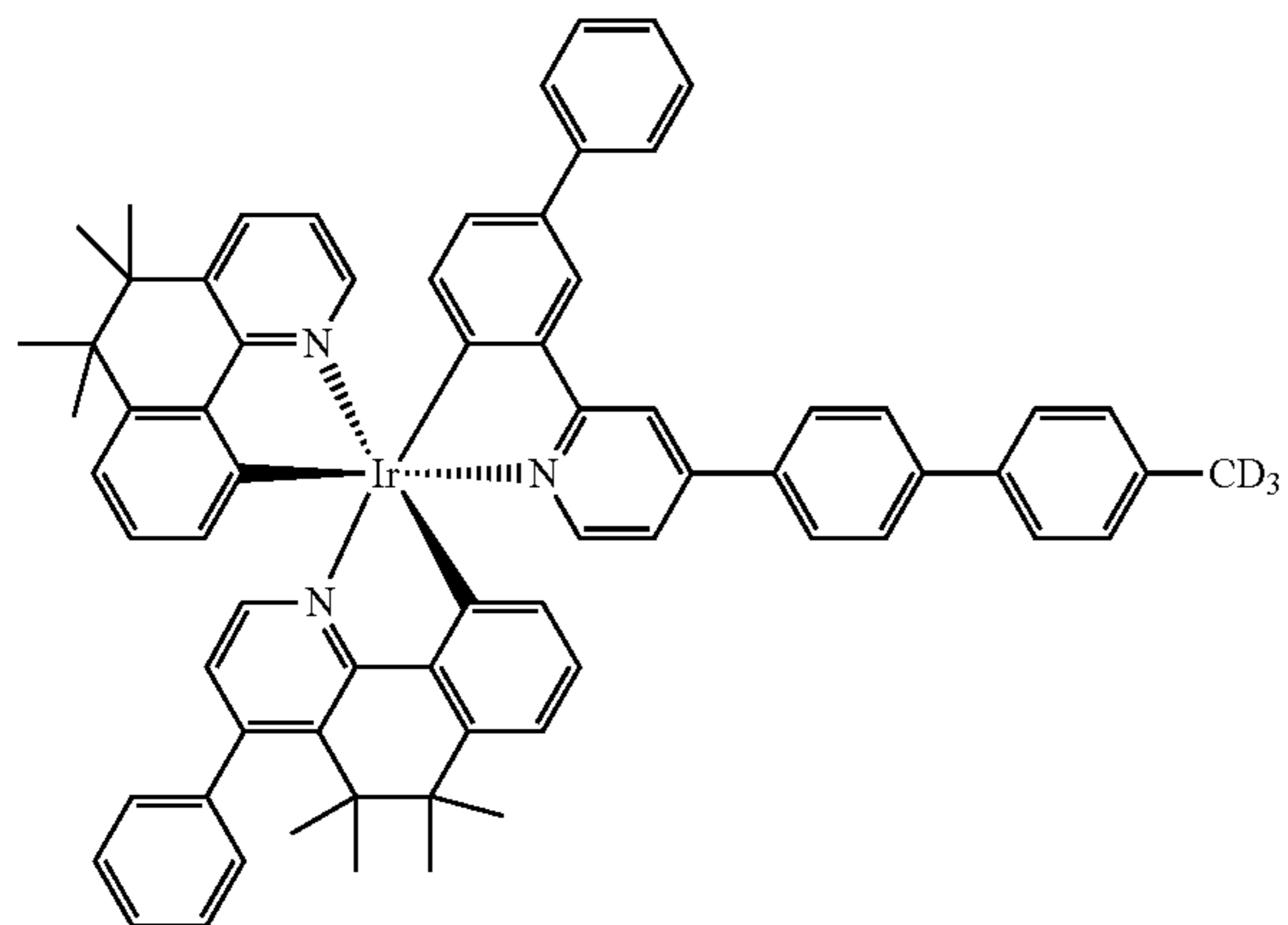
Compound 128
