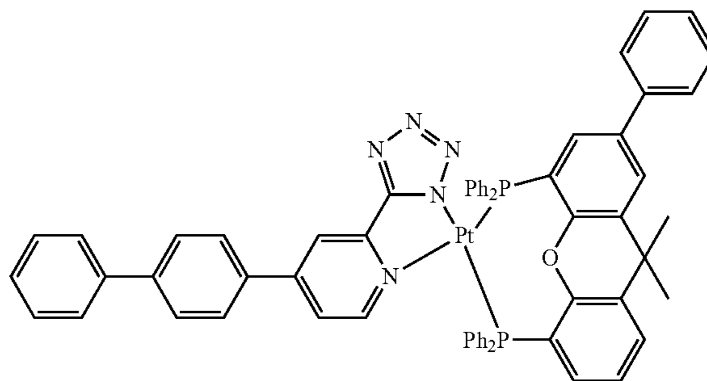
Compound 140
