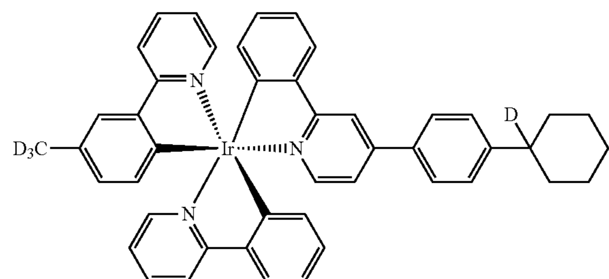
Compound 10
