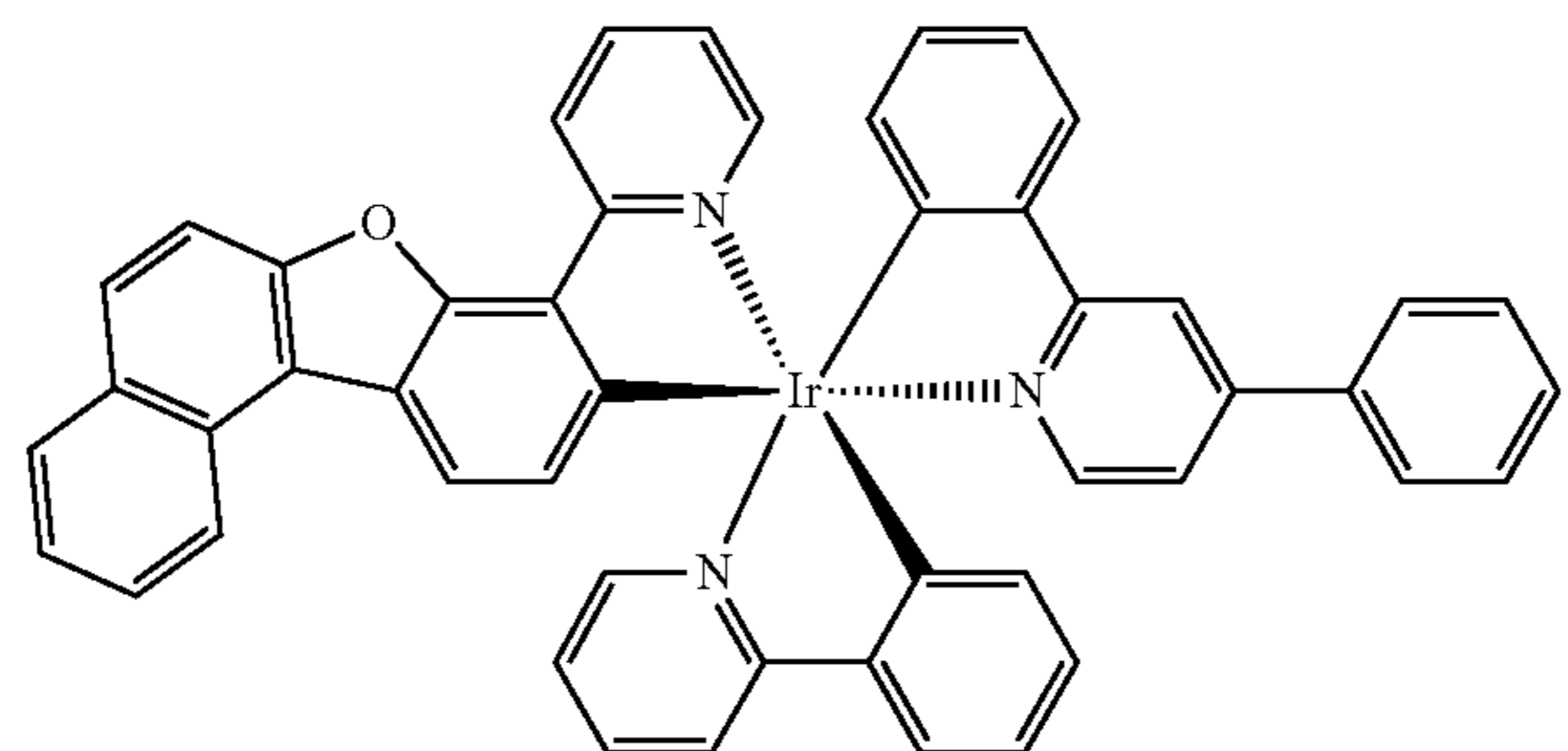
Compound 125
