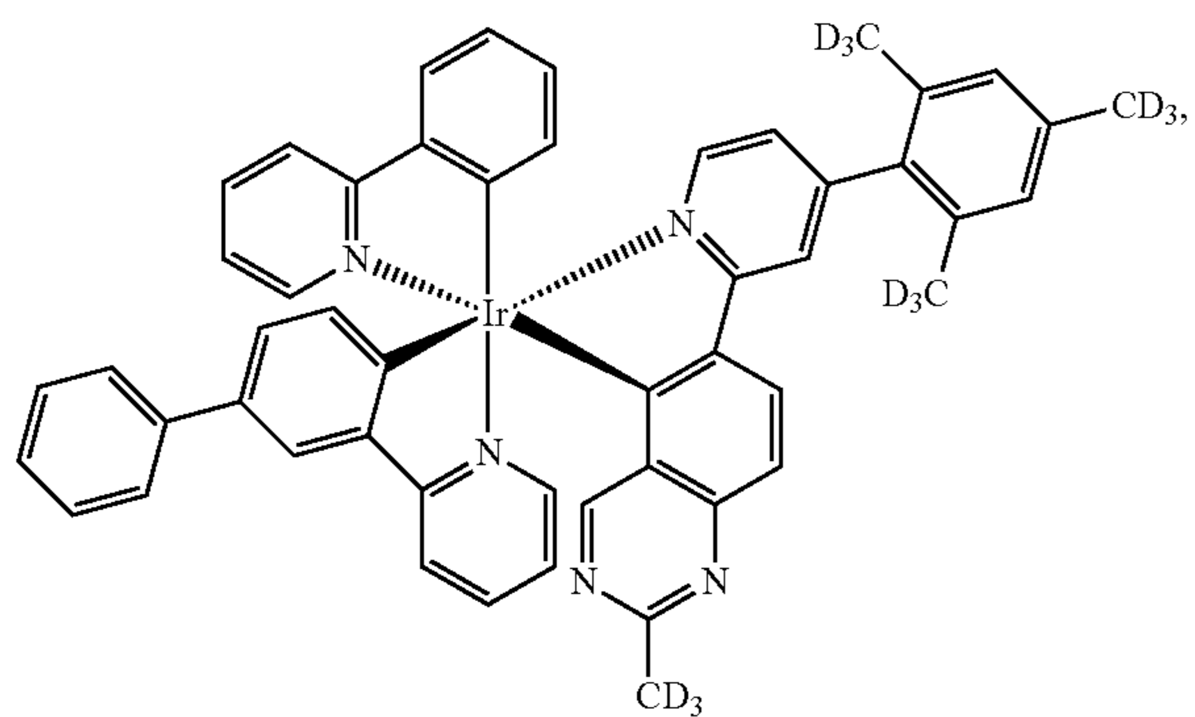
Compound 74
