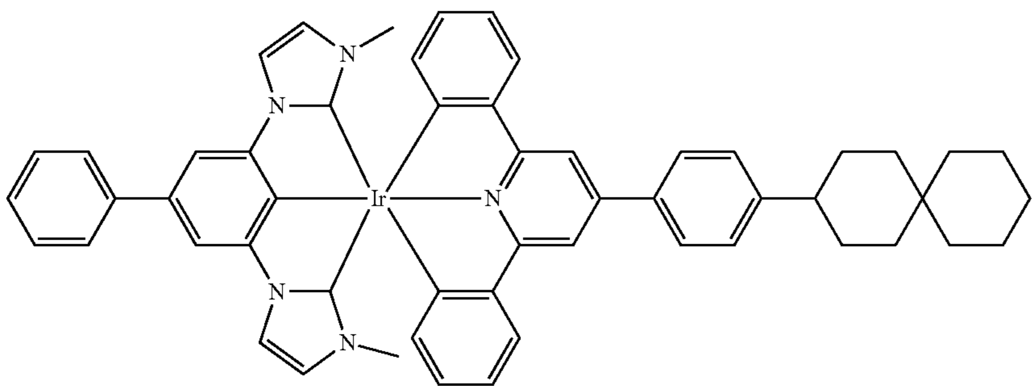
Compound 96
