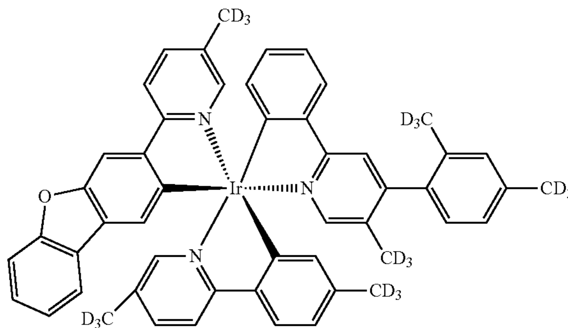
Compound 61
