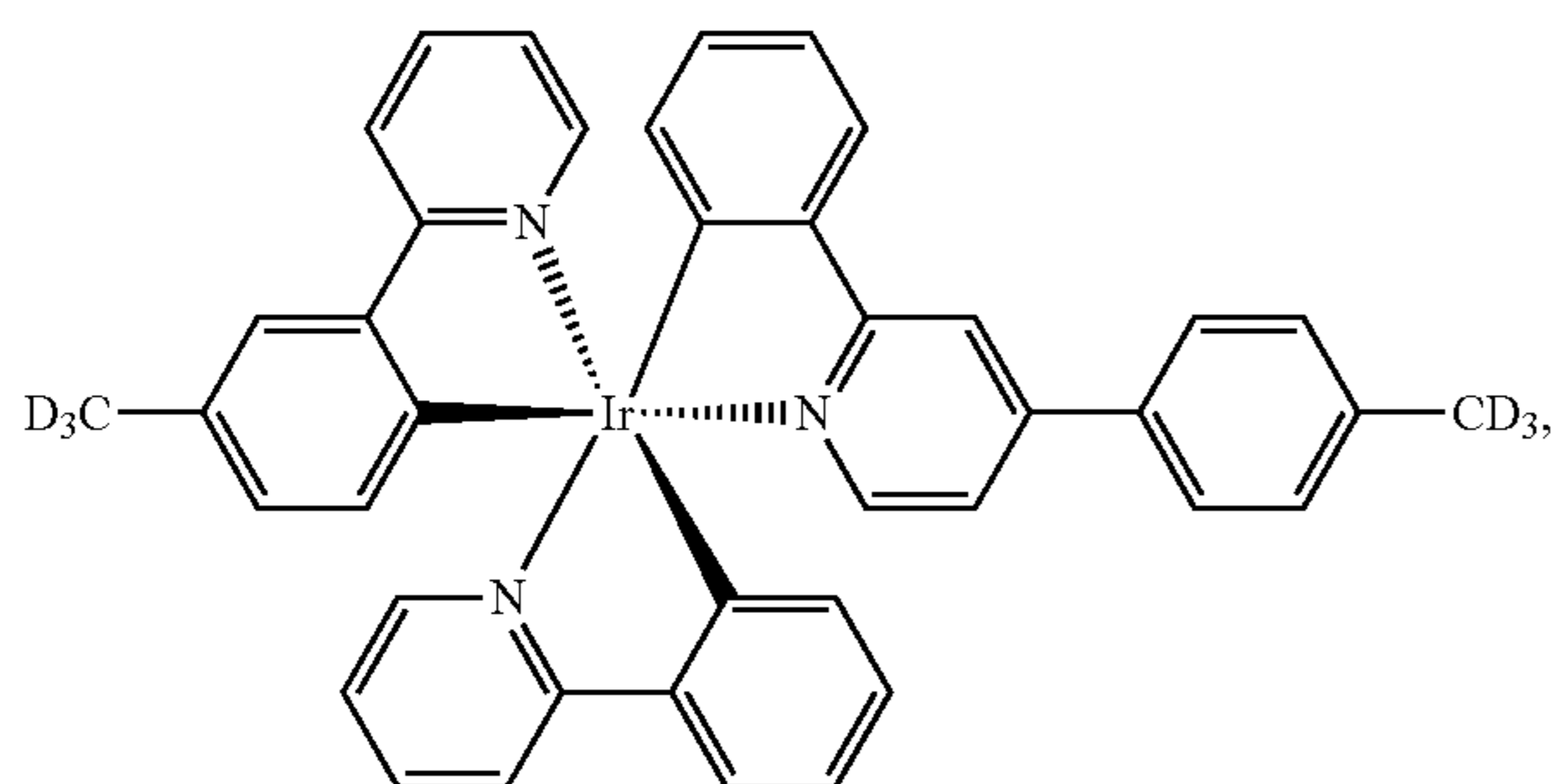
Compound 9
