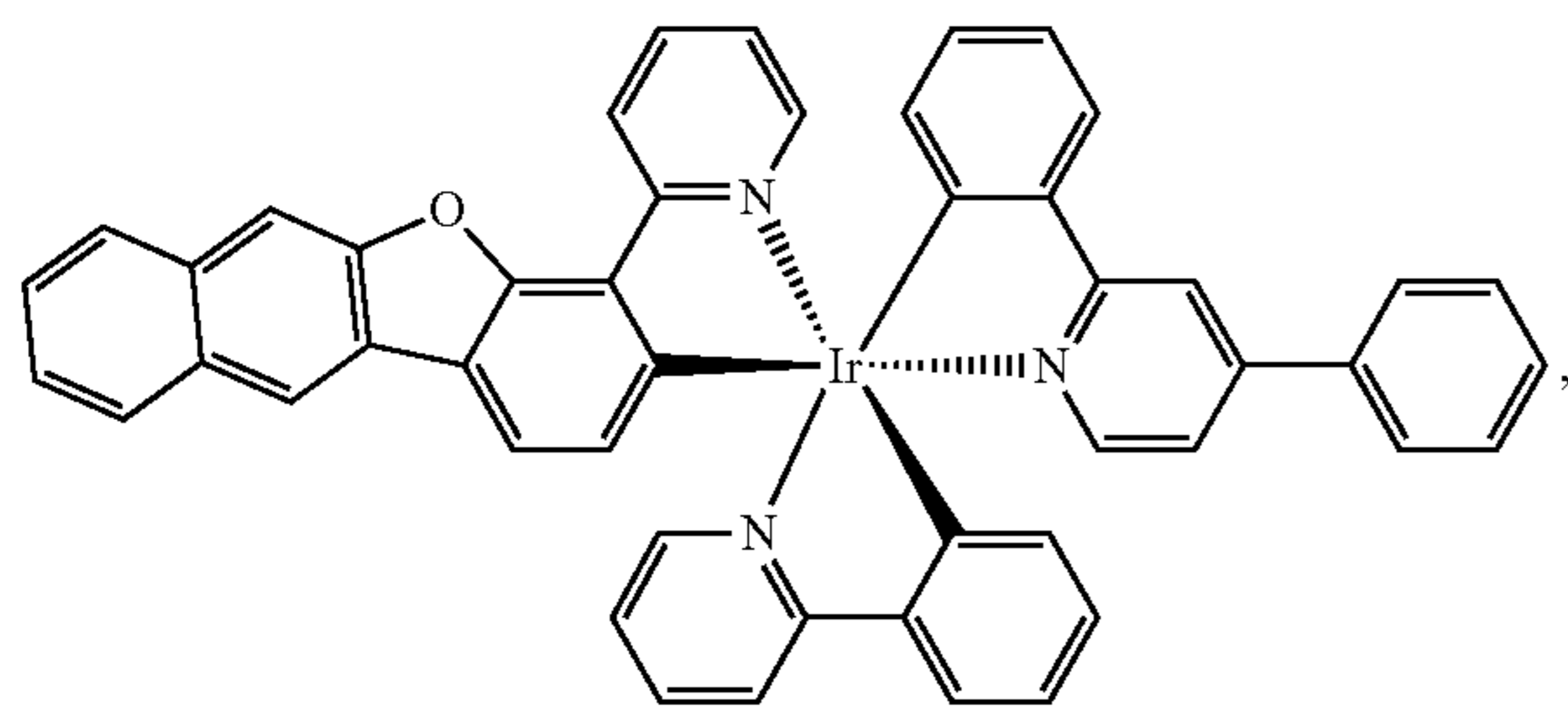
Compound 124
