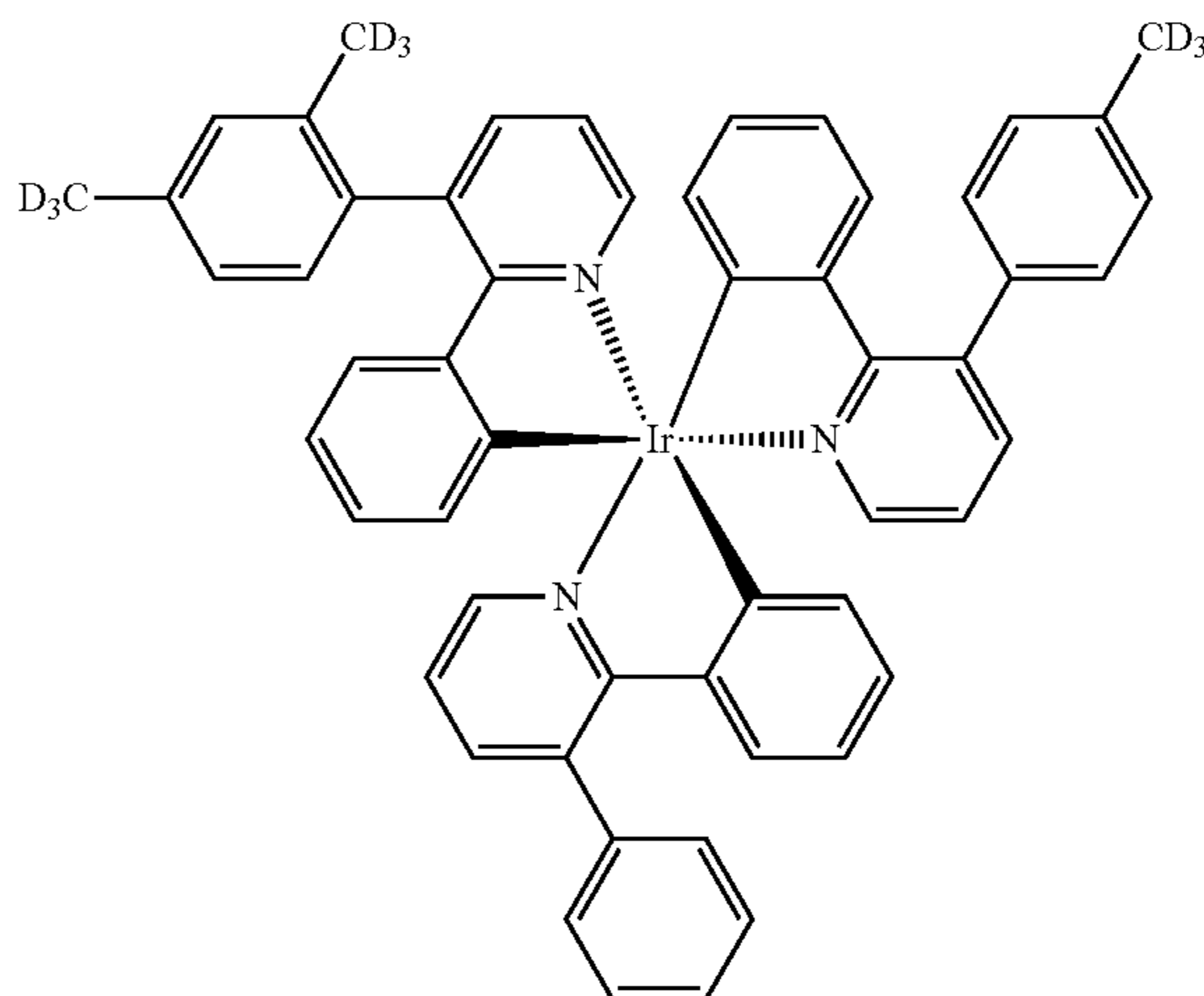
Compound 57
