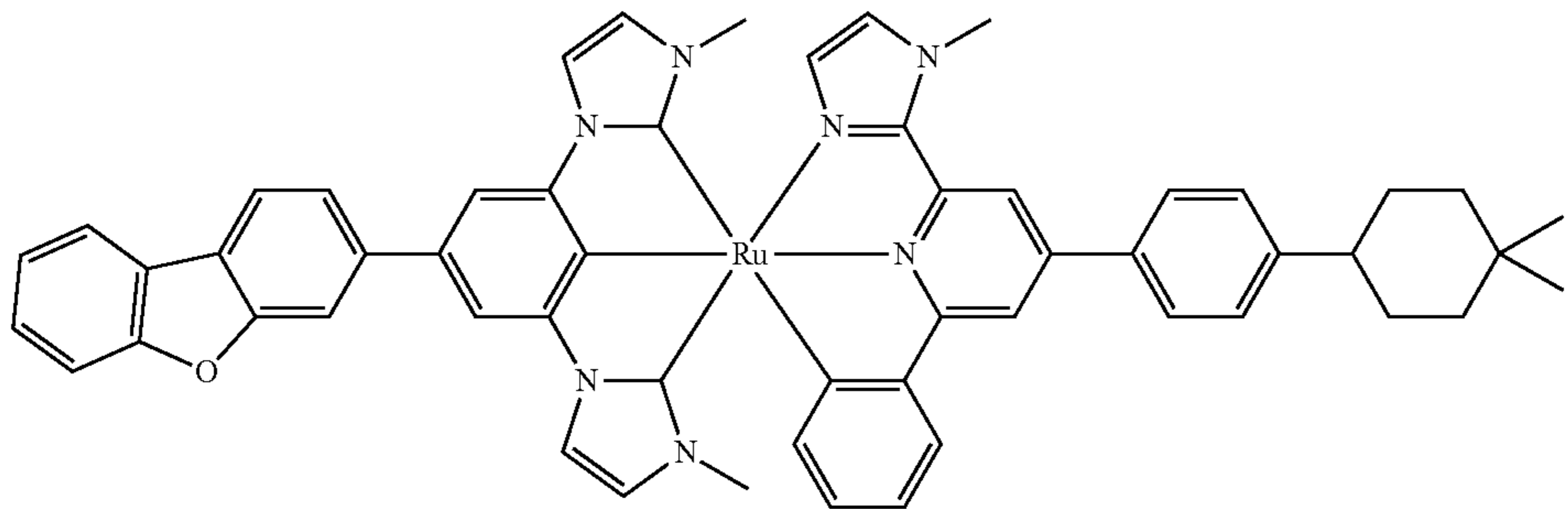
Compound 137
