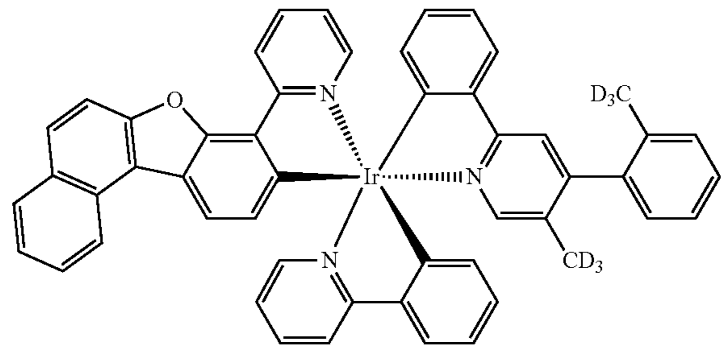
Compound 127
