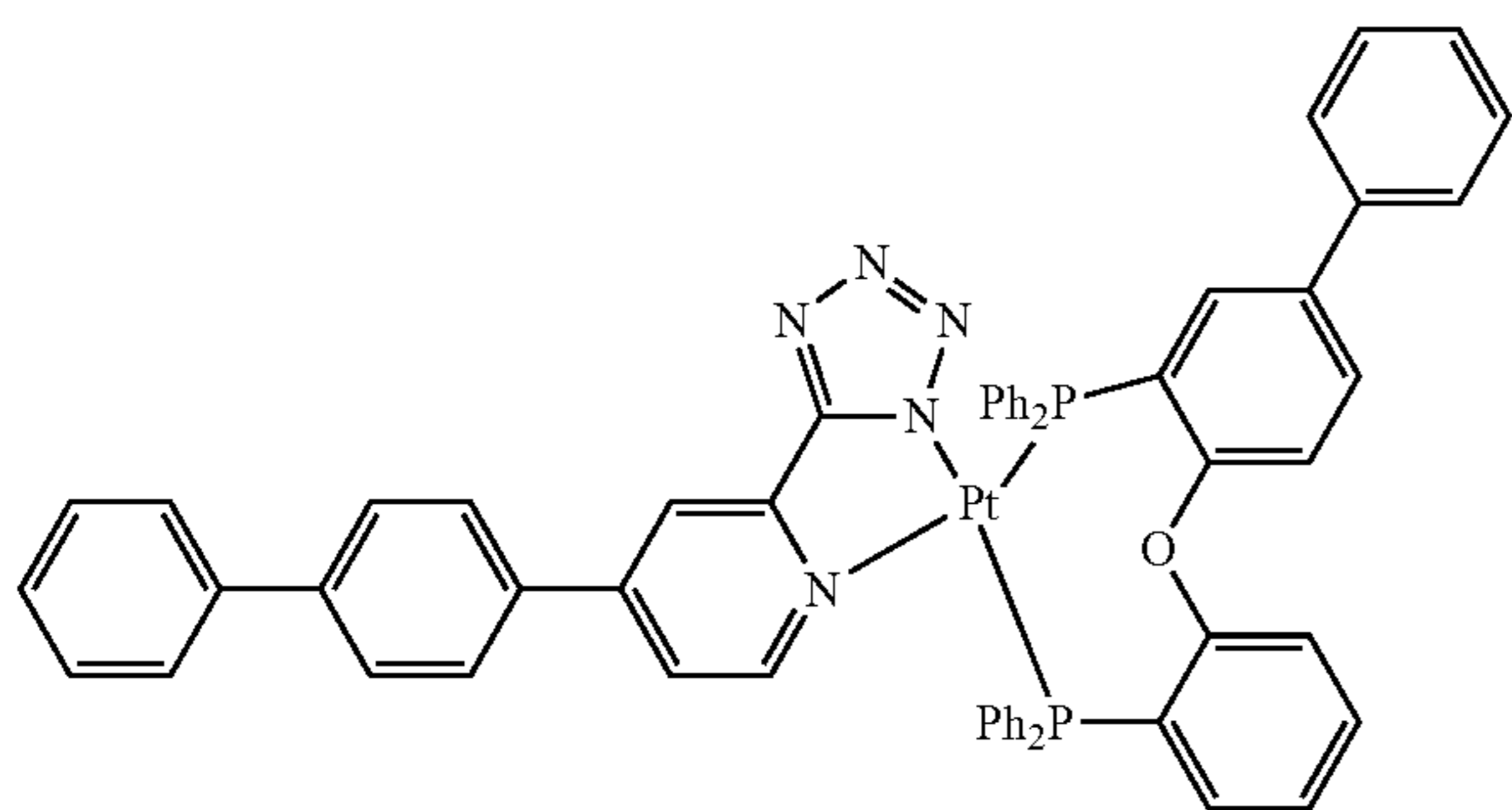
Compound 139
