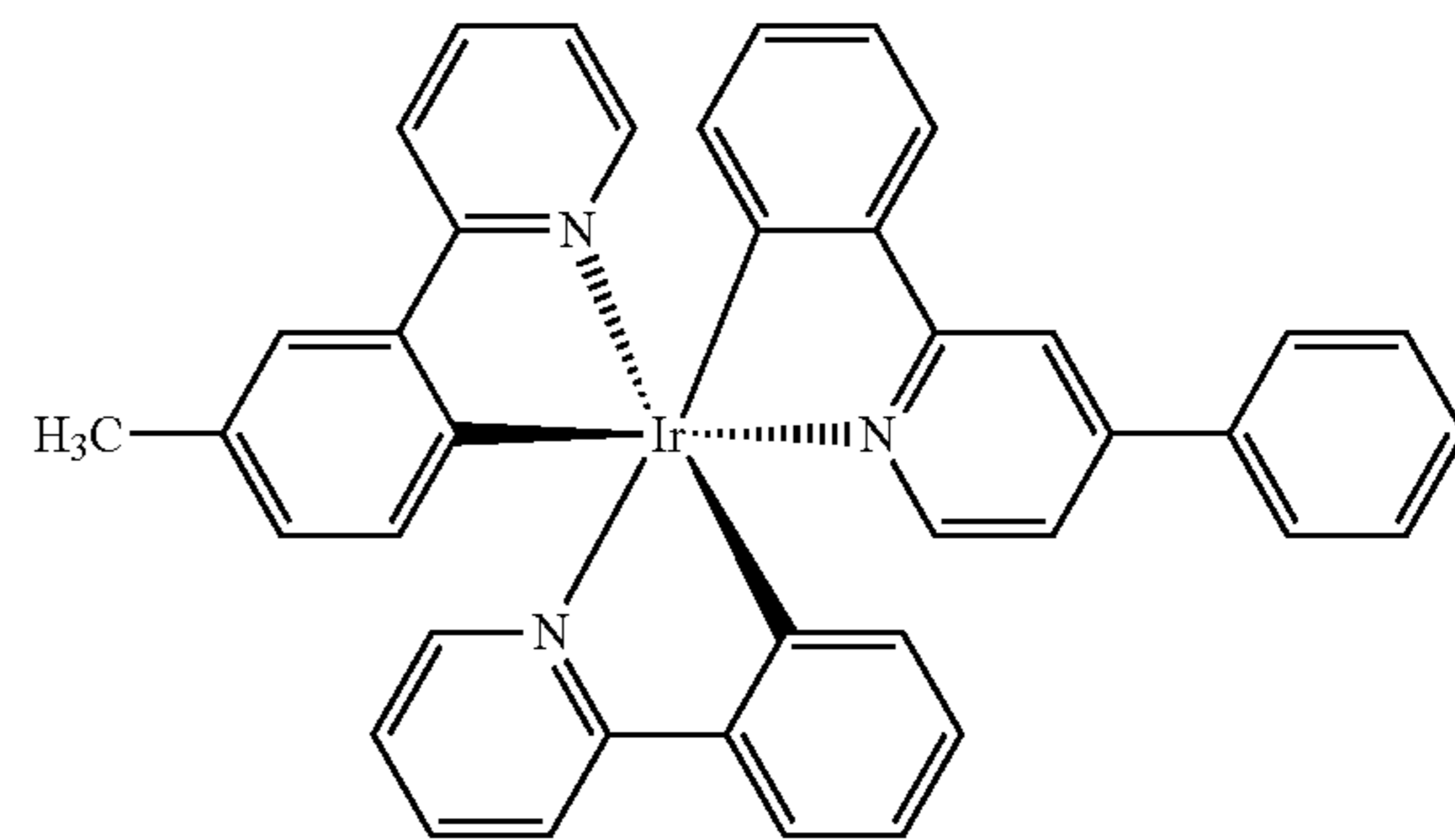
Compound 6
