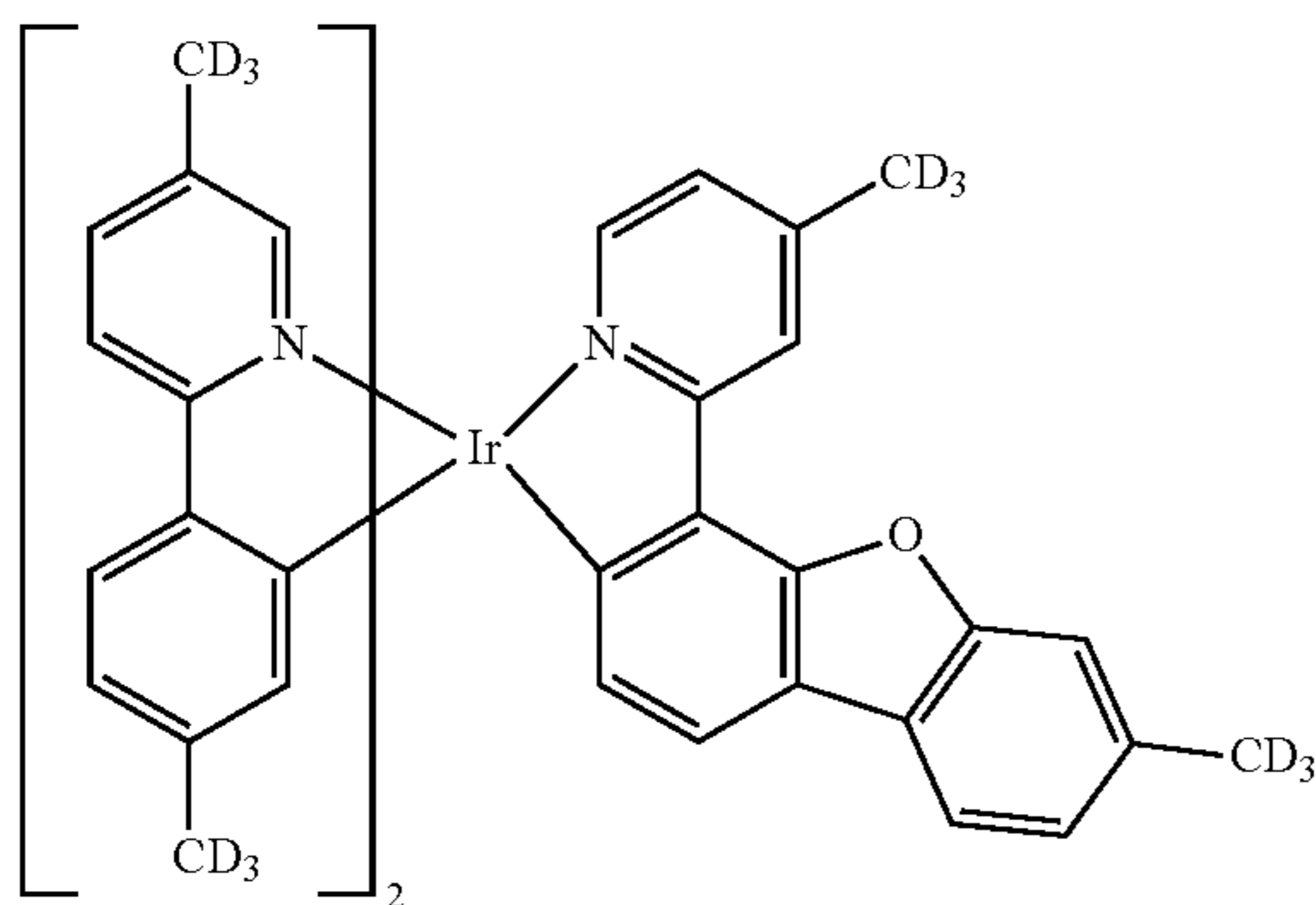
Compound A
