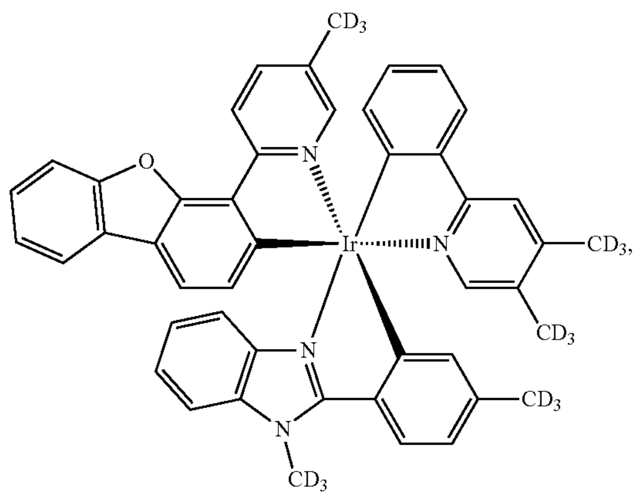
Compound 68
