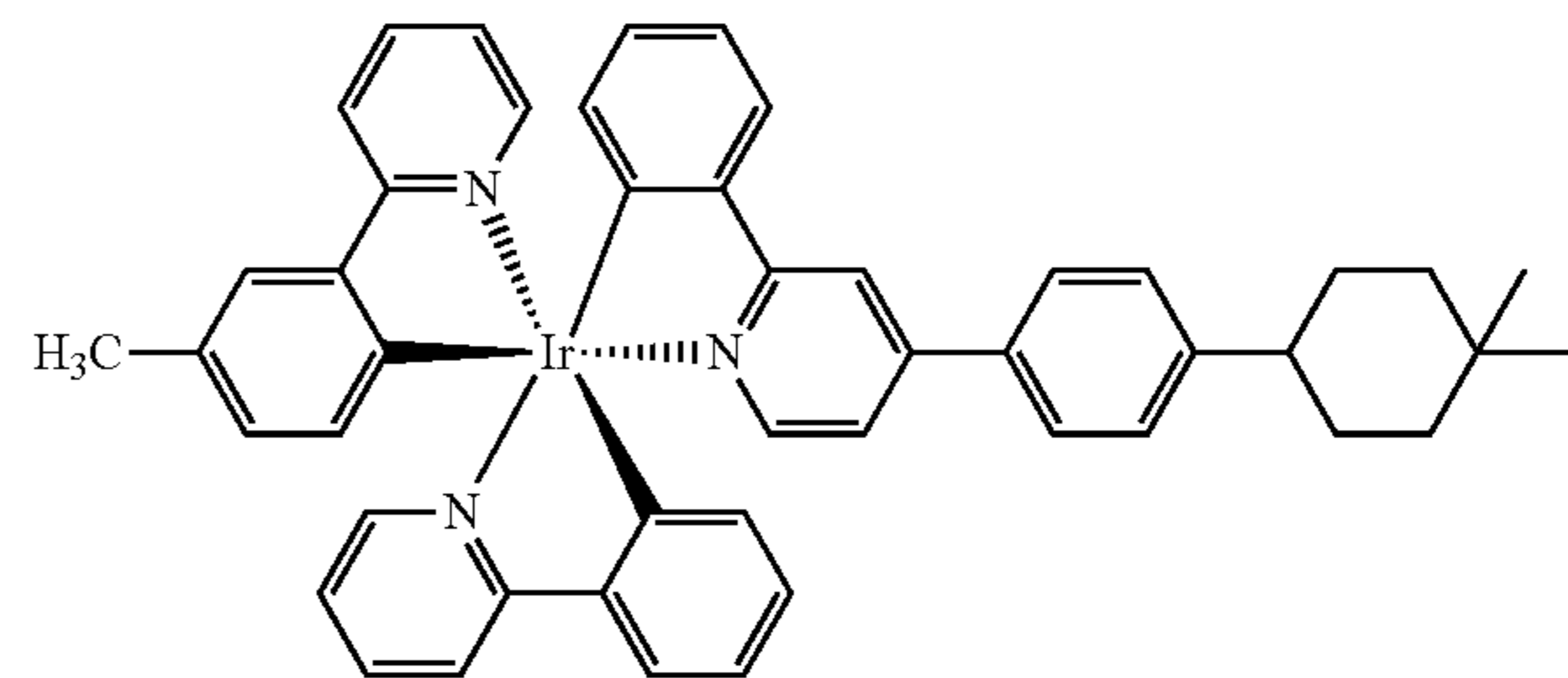
Compound 6
