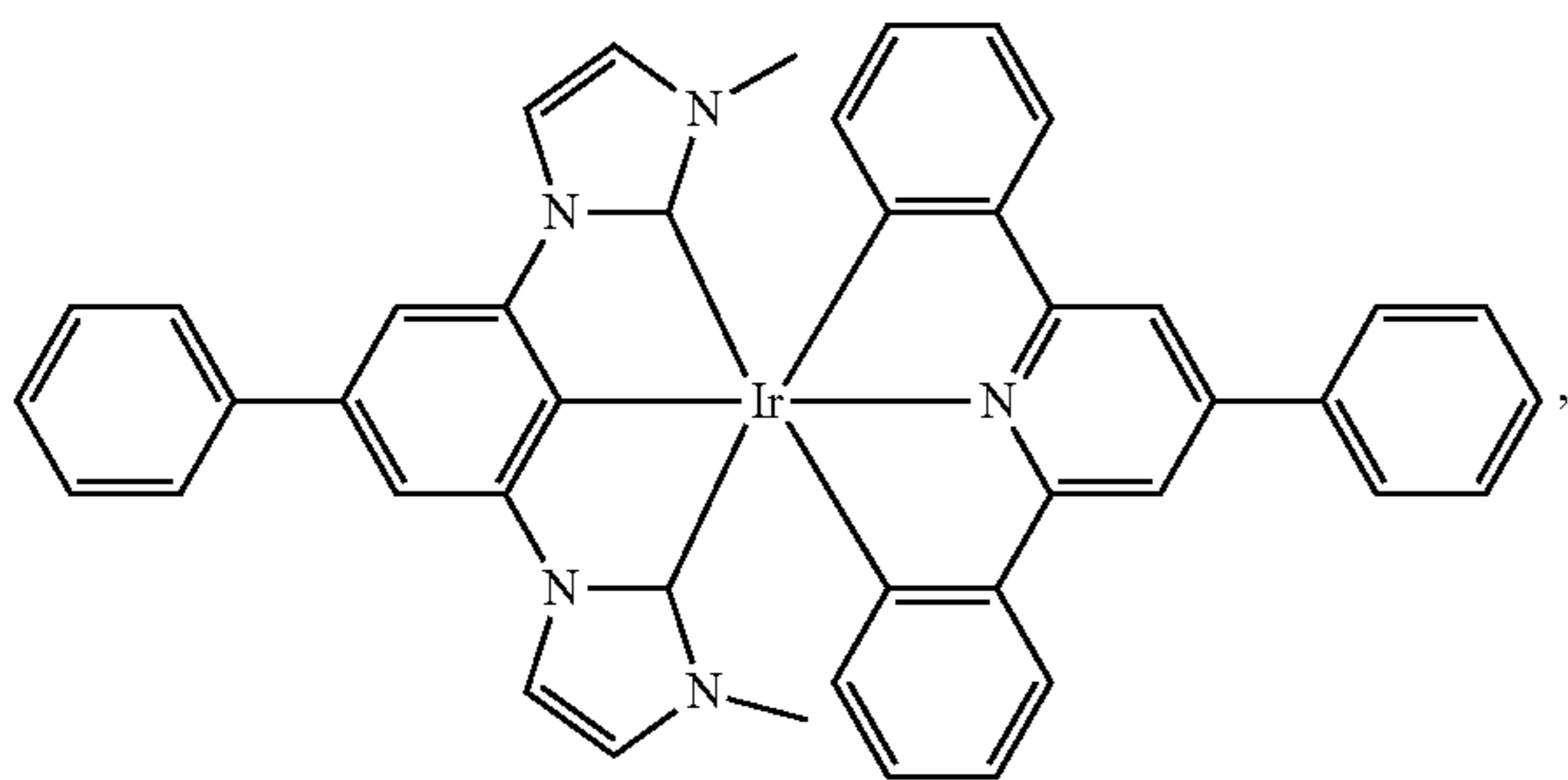
Compound 96
