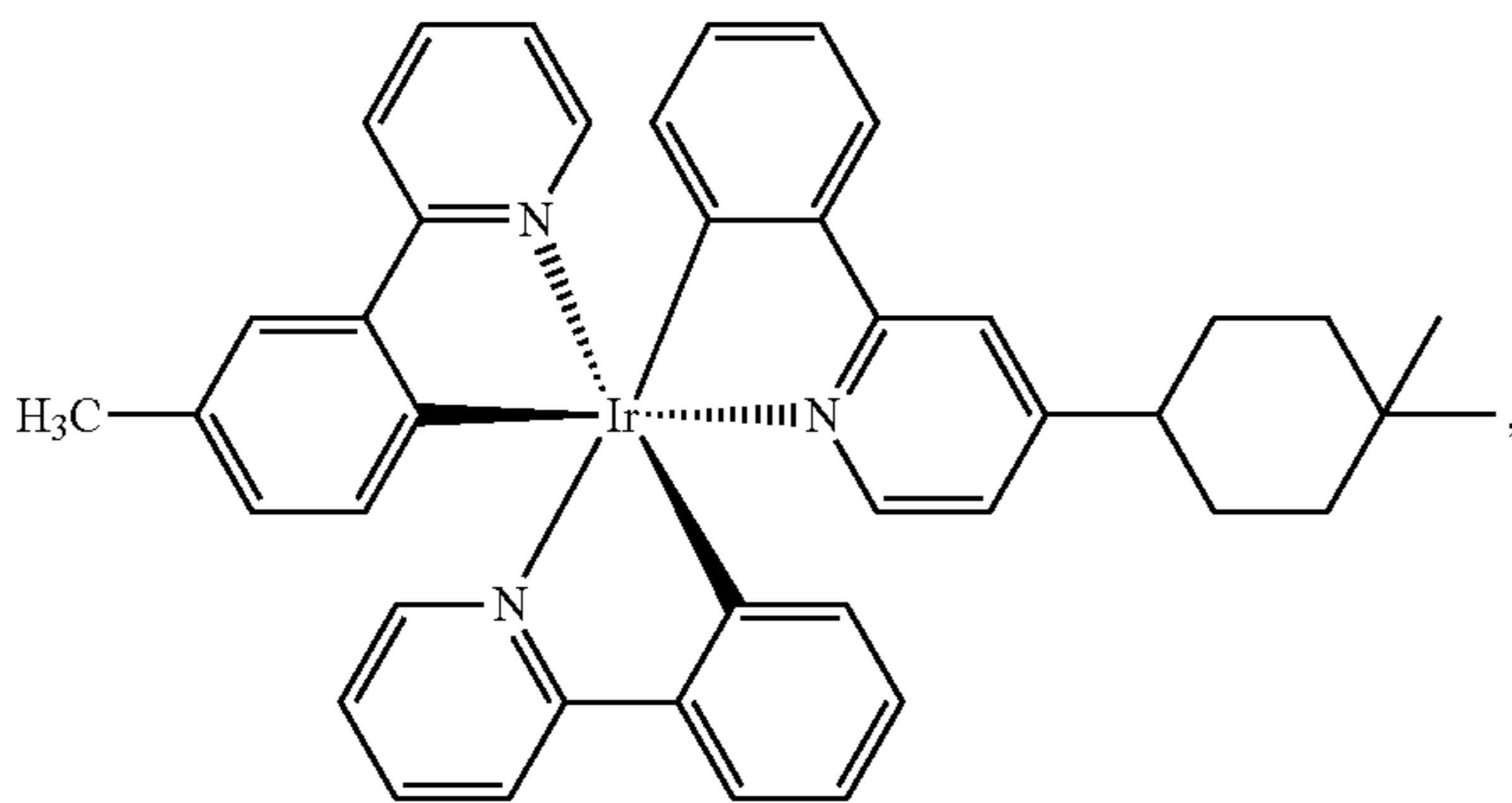
Compound 5
