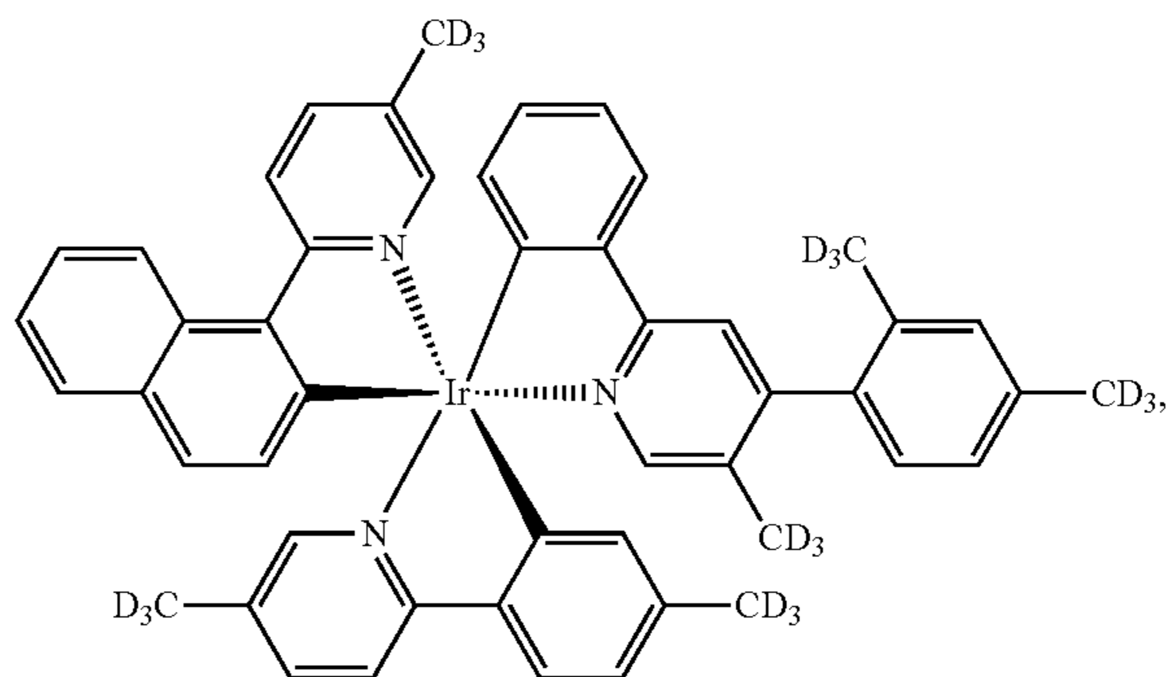
Compound 65
