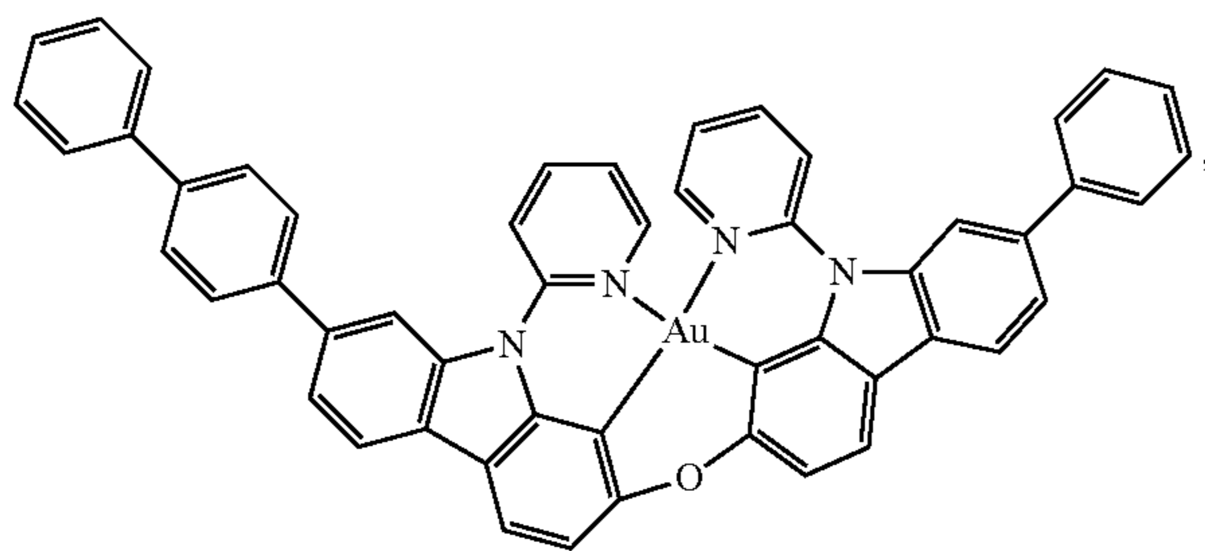
Compound 89
