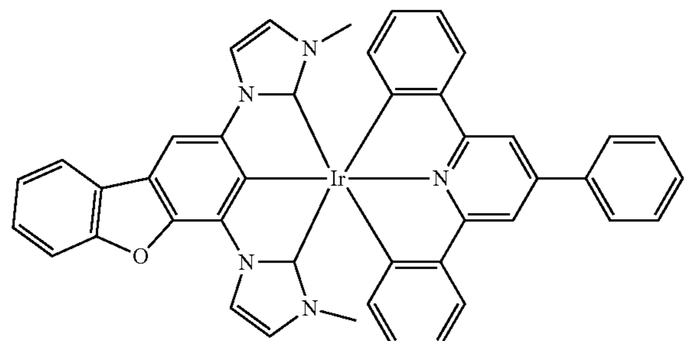
Compound 98
