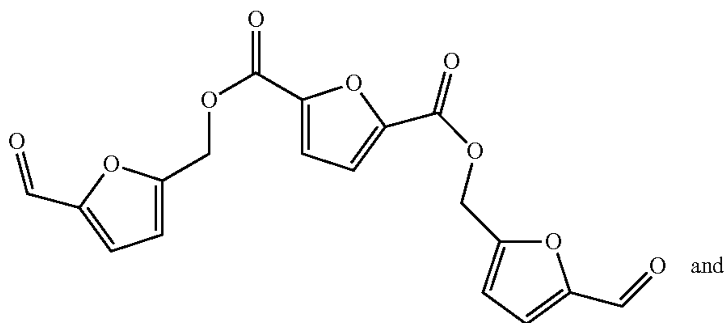
bis((5-formylfuran-2-yl)methyl) furan-2,5-dicarboxylate (FDCA-HMF)
