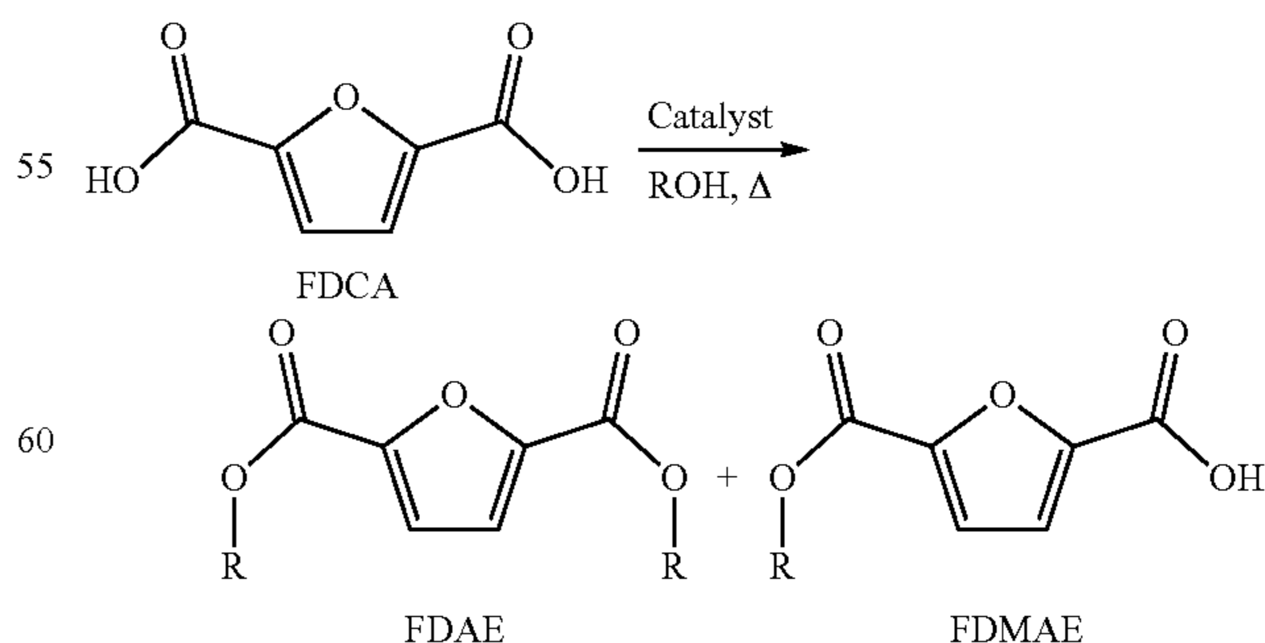
Scheme 1. Esterification of FDCA to FDMAE and FDAE
