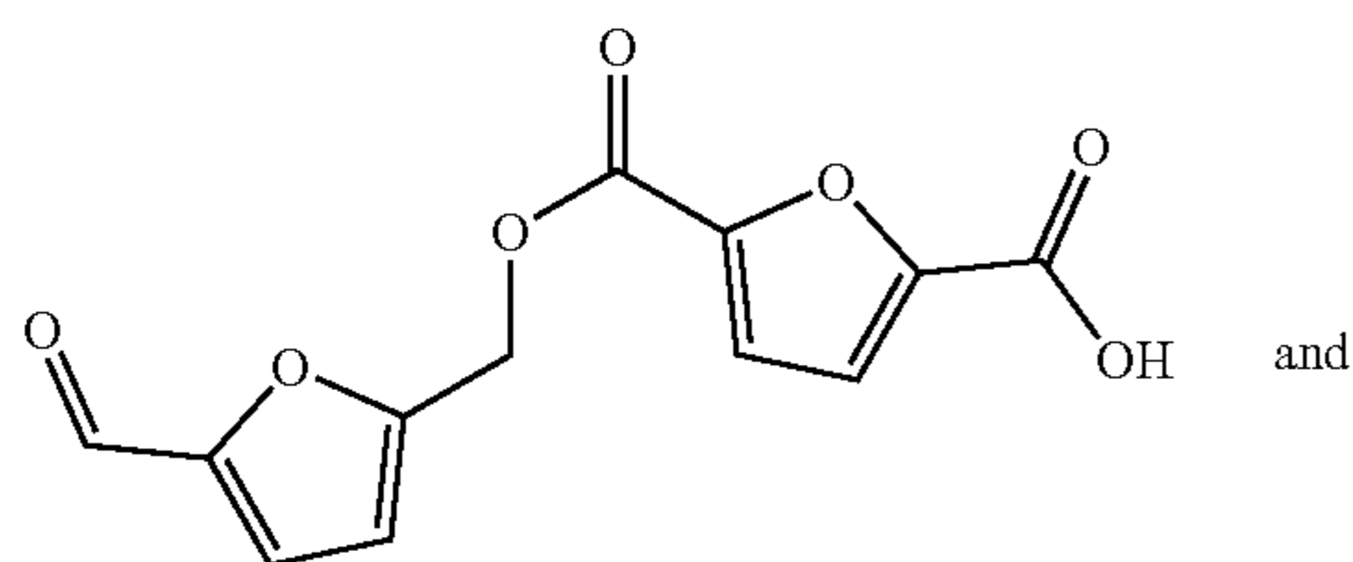
5-(((5-formylfuran-2-yl)methoxy)carbonyl)furan-2-carboxylic acid (FDCA-HMF)
