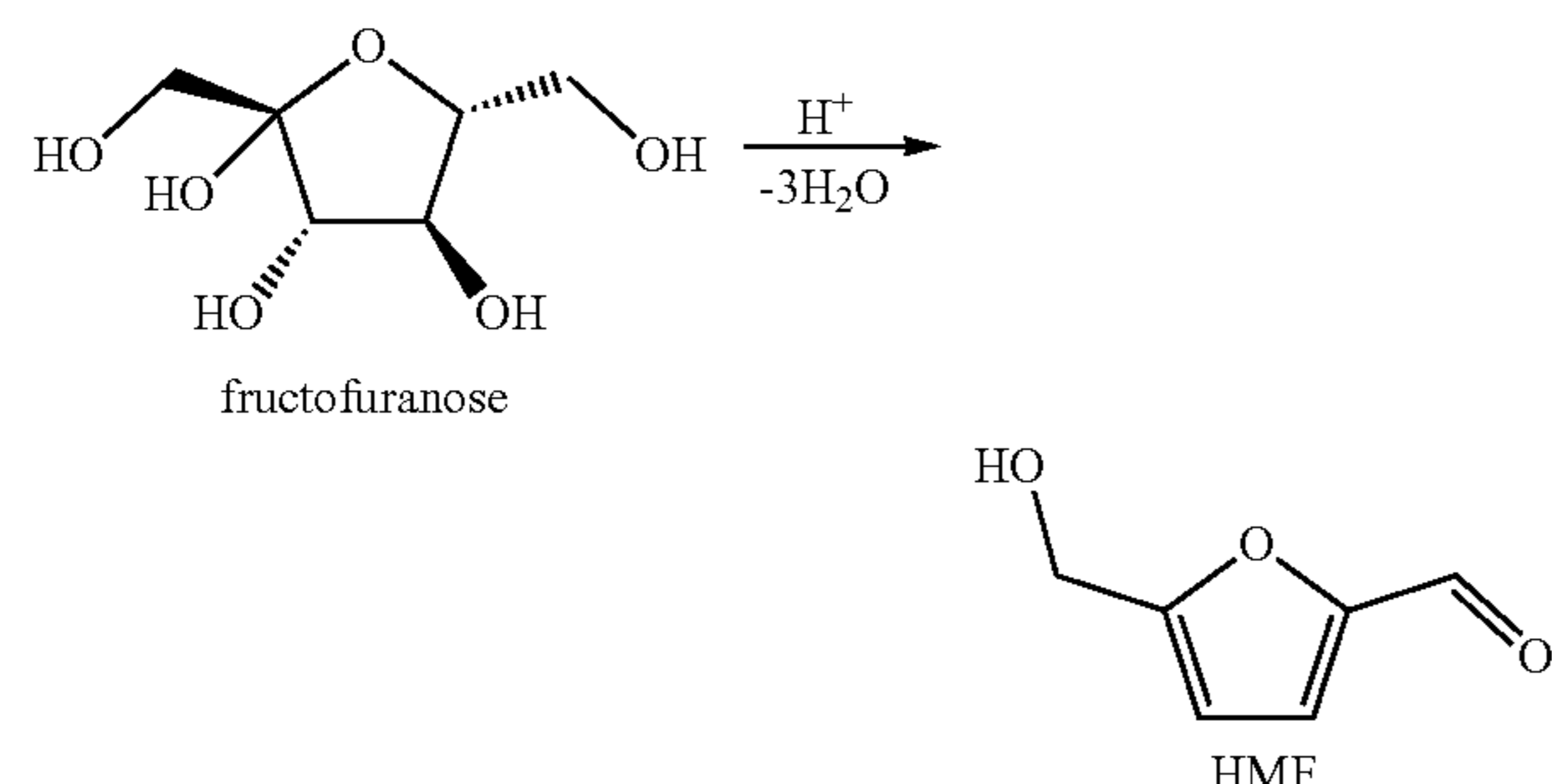
Scheme A. Catalytic dehydrative cyclization of fructose to HMF
