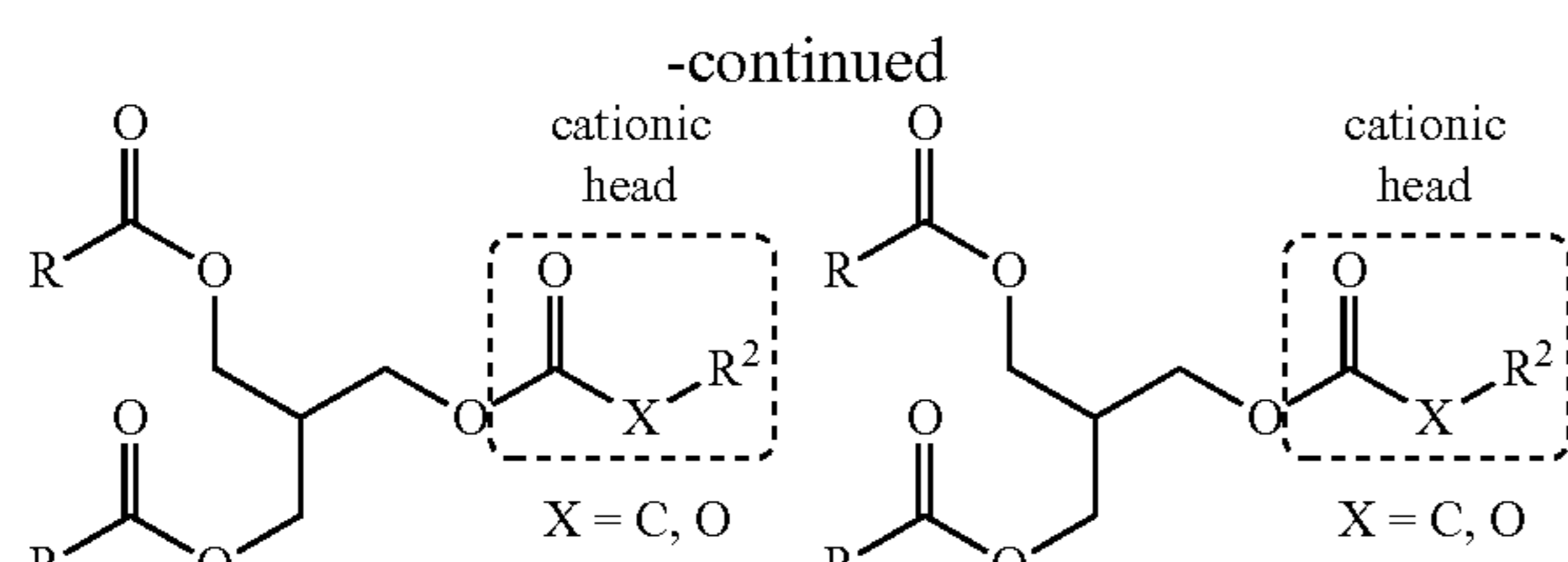
a) Selective bis-acylation for symmetric tail installation. b) Ester or carbonate cationic head coupling. c) Selective mono-acylation for asymmetric tail installation.
