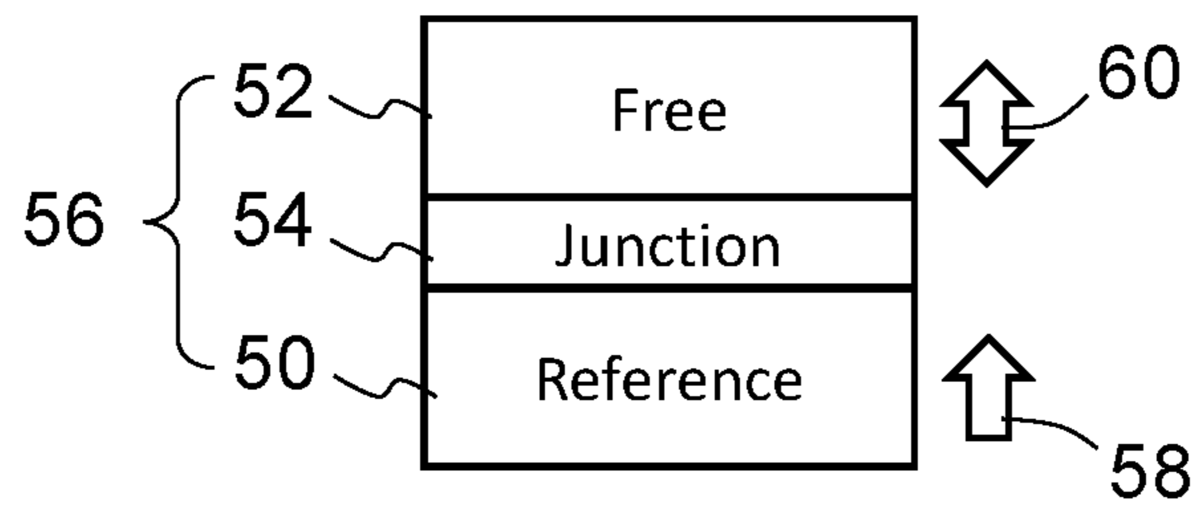
FIG. 2 PRIOR ART
