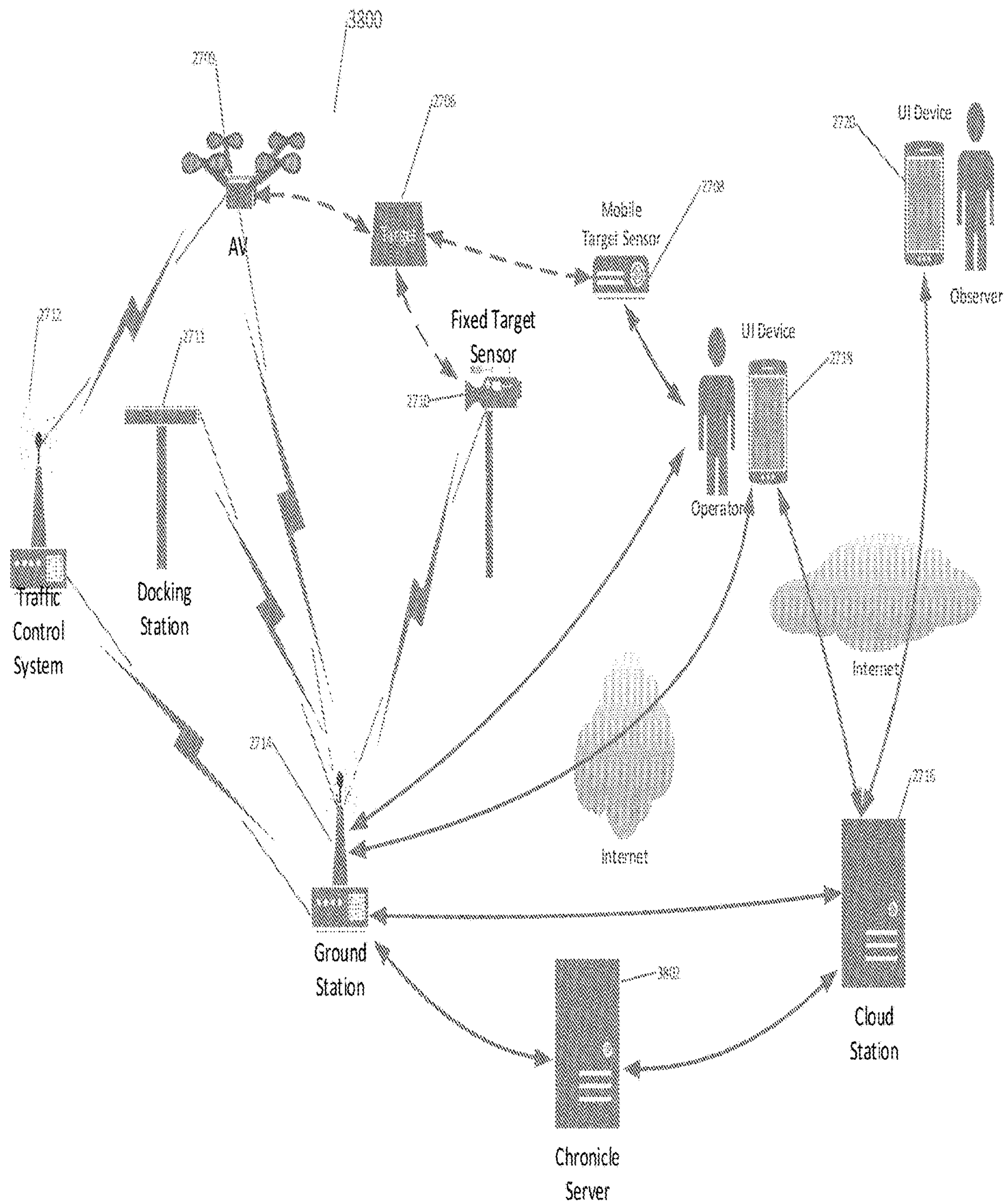
Figure 38. Main Architecture with Chronicle Server
