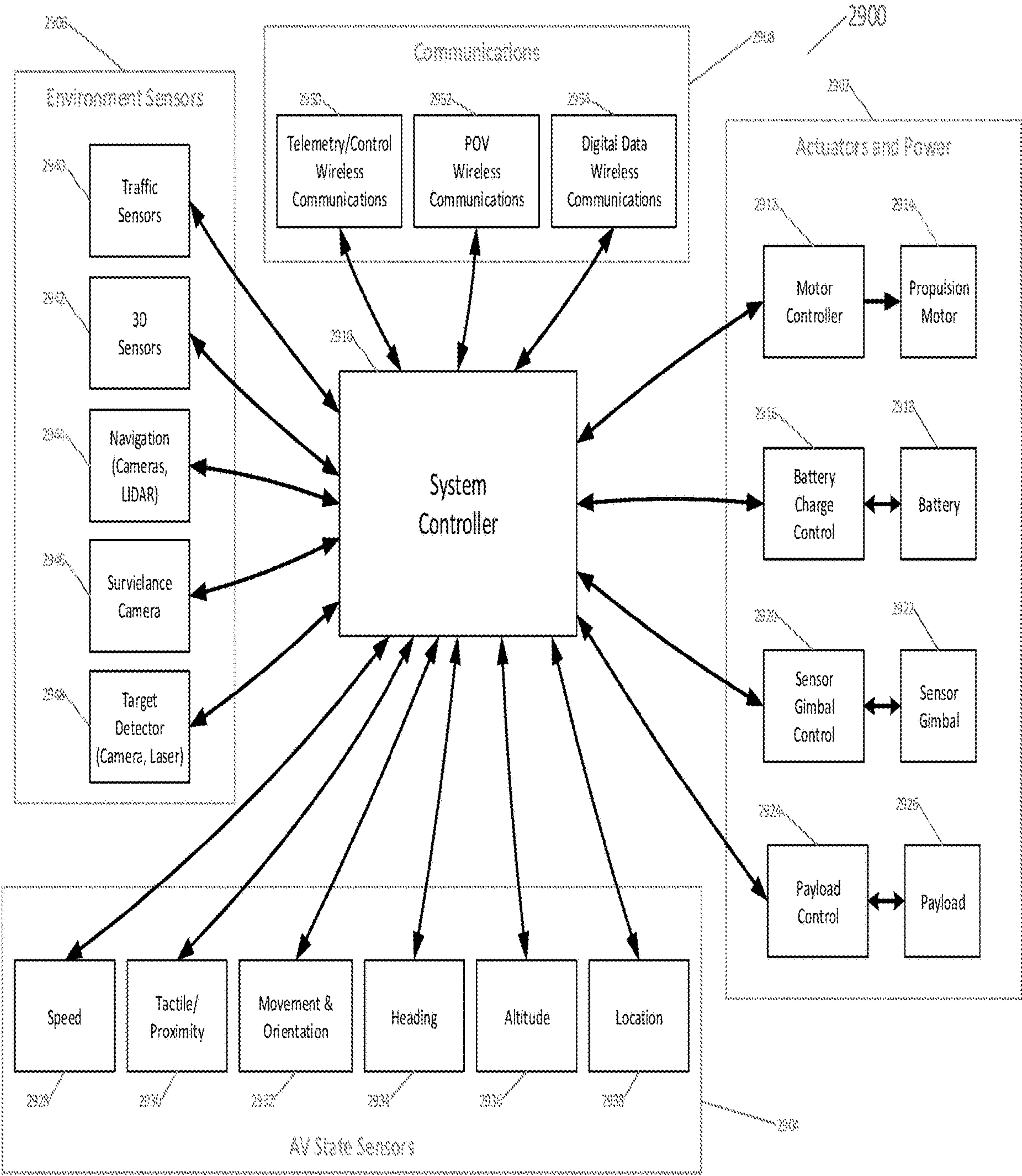
Figure 29. Automated Vehicle Subsystems
