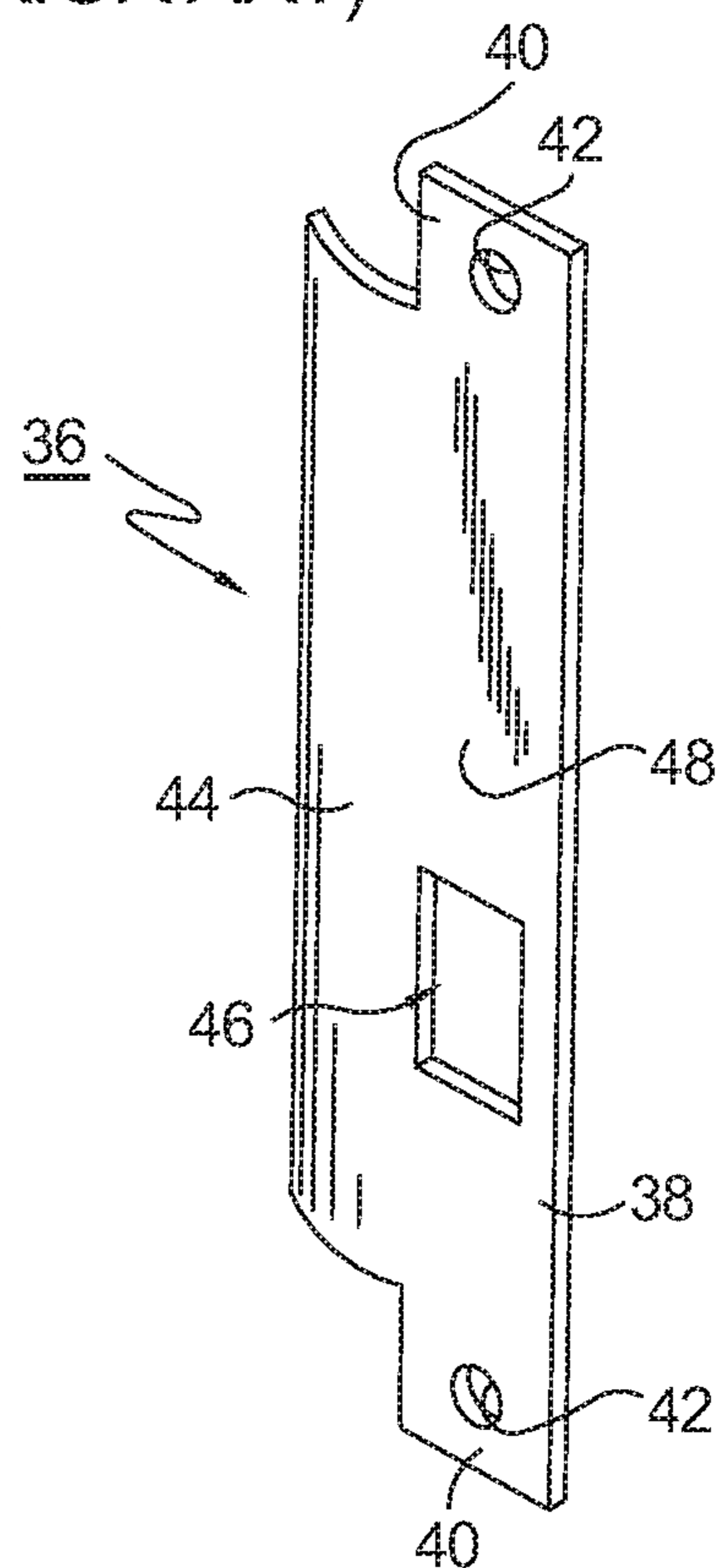
FIG. 3. (PRIOR ART)
