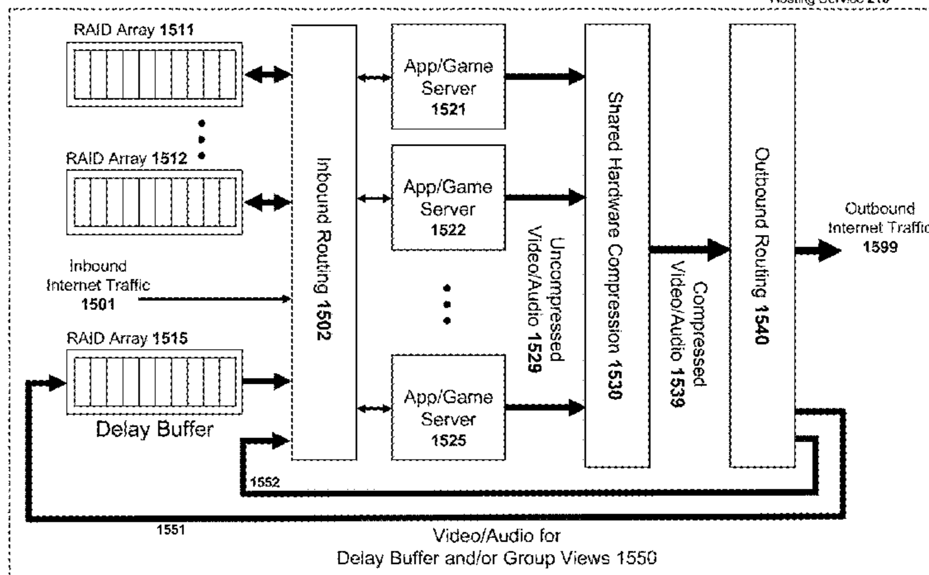
Server Center Embodiment of Hosting Service 210
