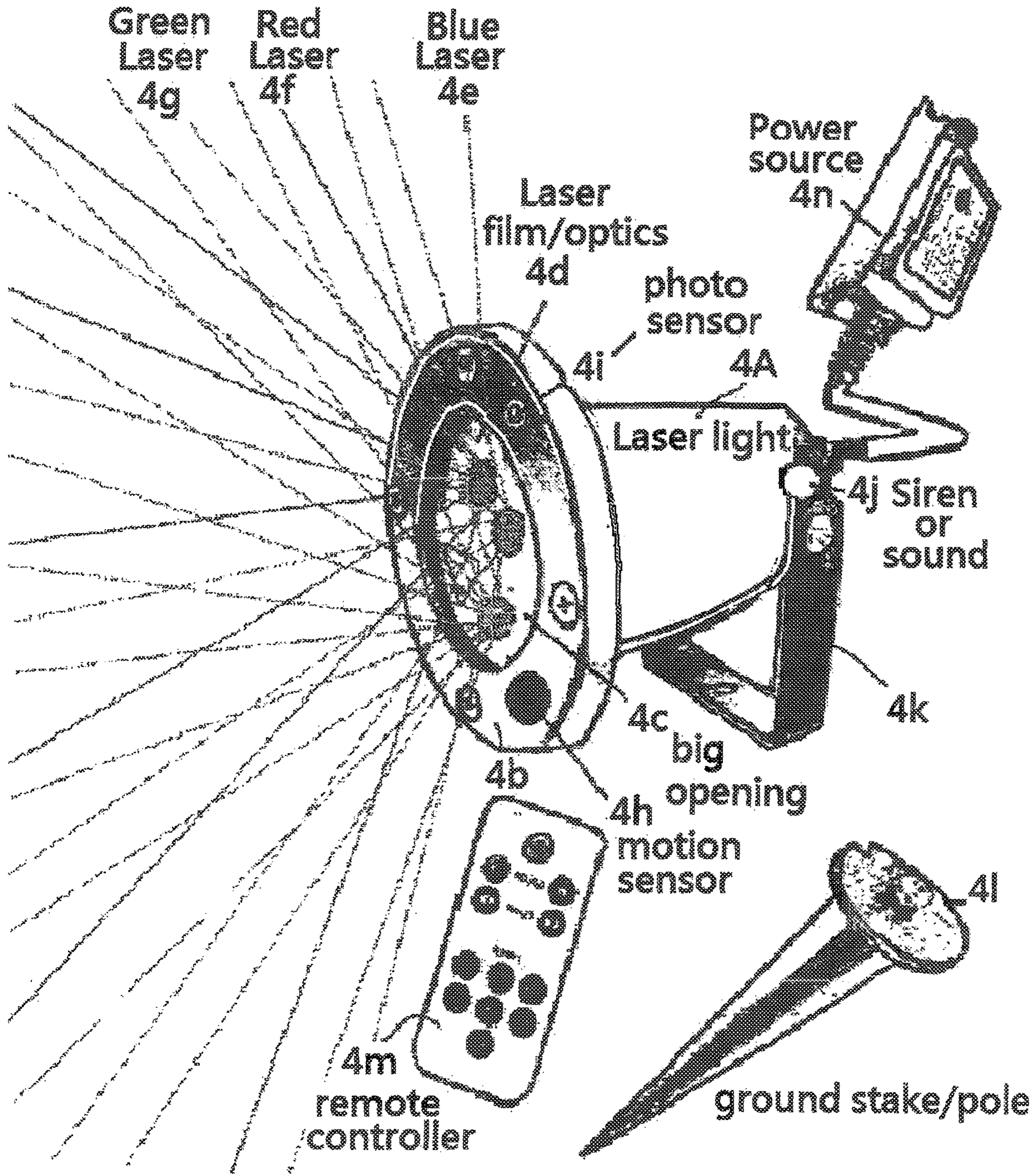
Garden light applicadtion with ground stake into soil
