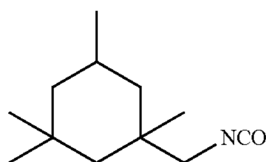
Isophorone diisocyanate
