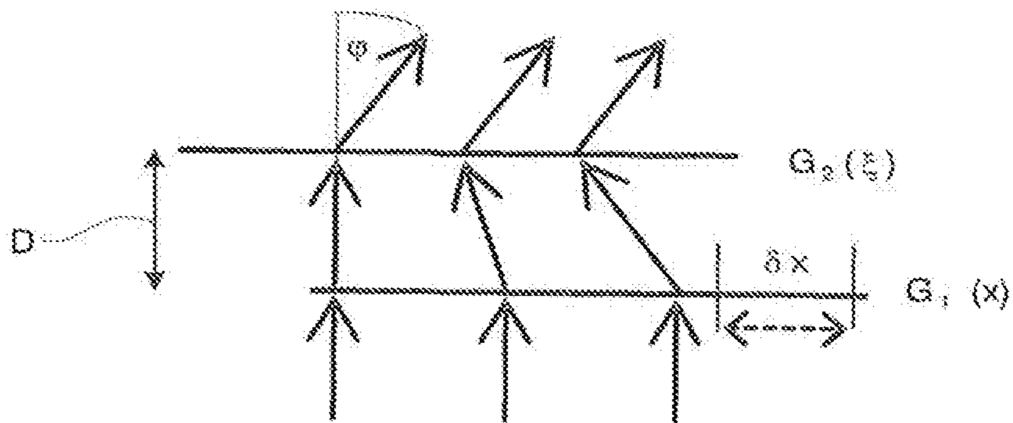
Fig 1C (Prior Art)
