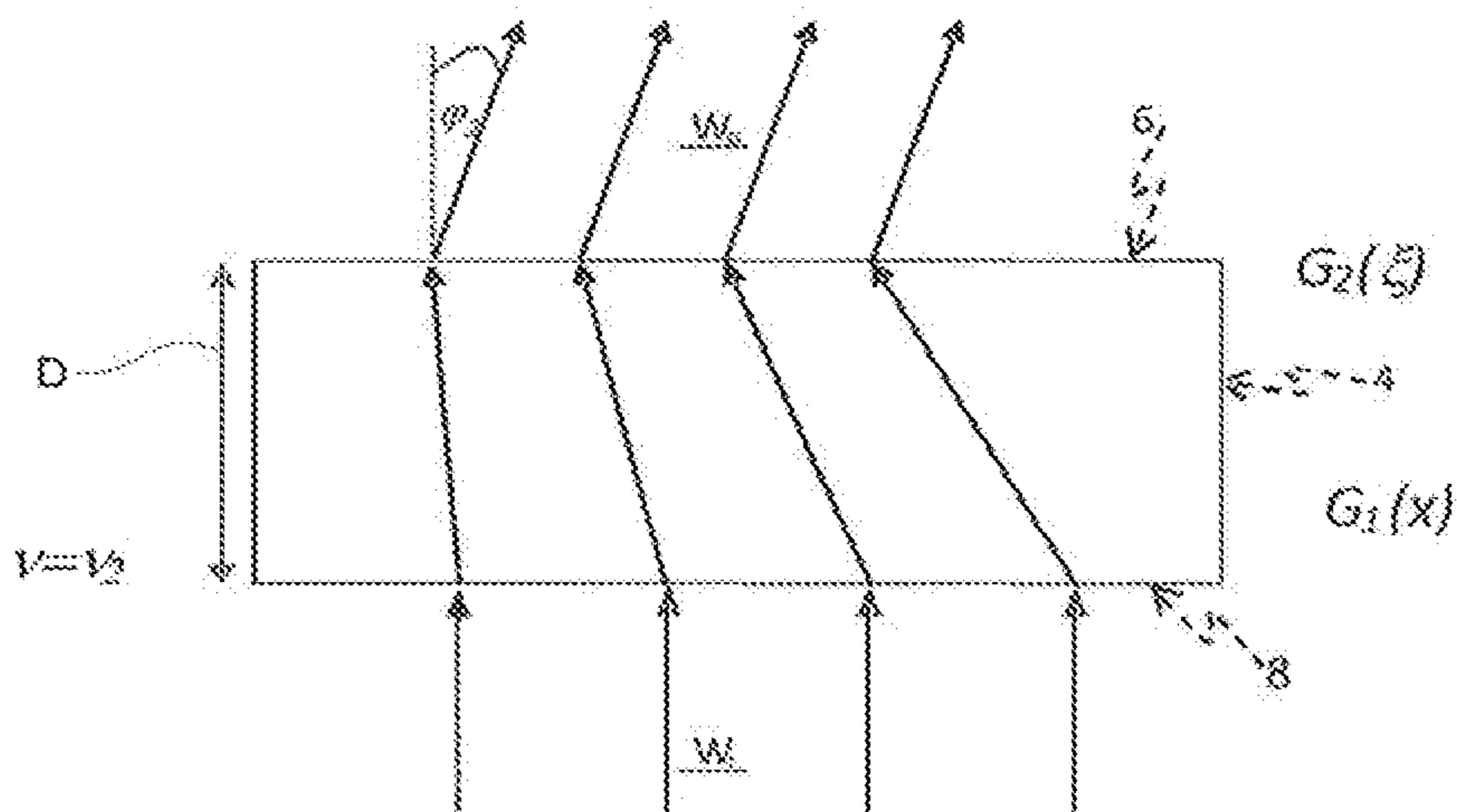
Fig. 2C (prior art)
