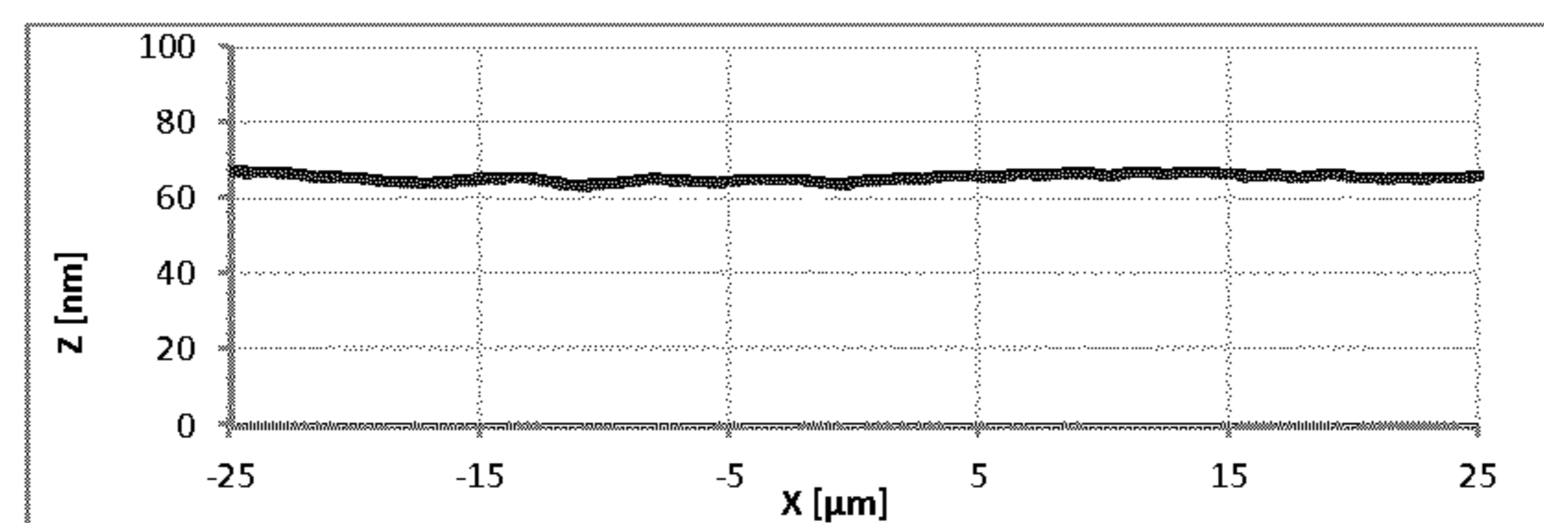
Film profile of the film of Example 2
