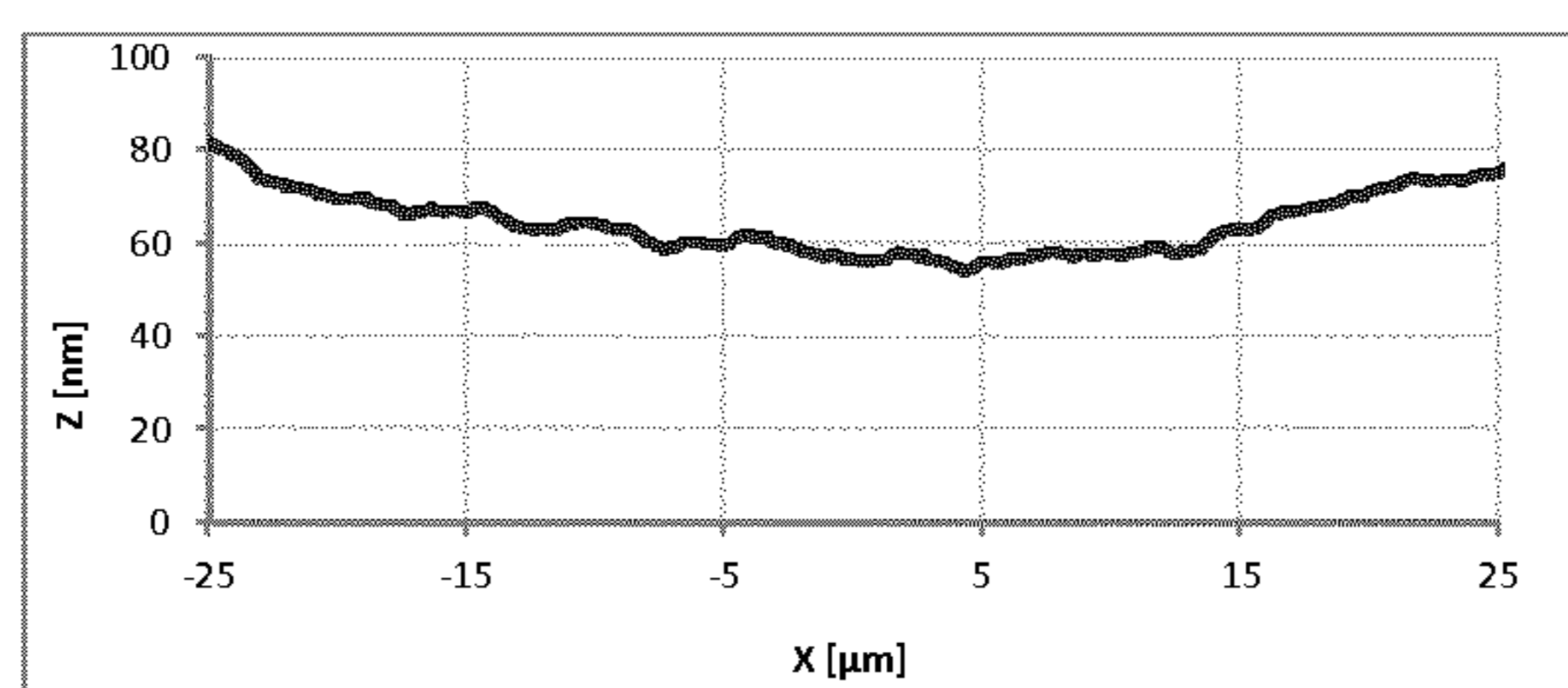
Film profile of the film of Reference Example
