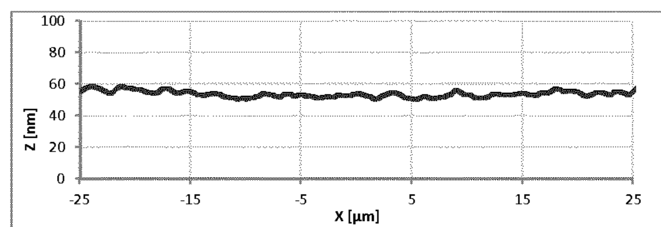
Film profile of the film of Example 3
