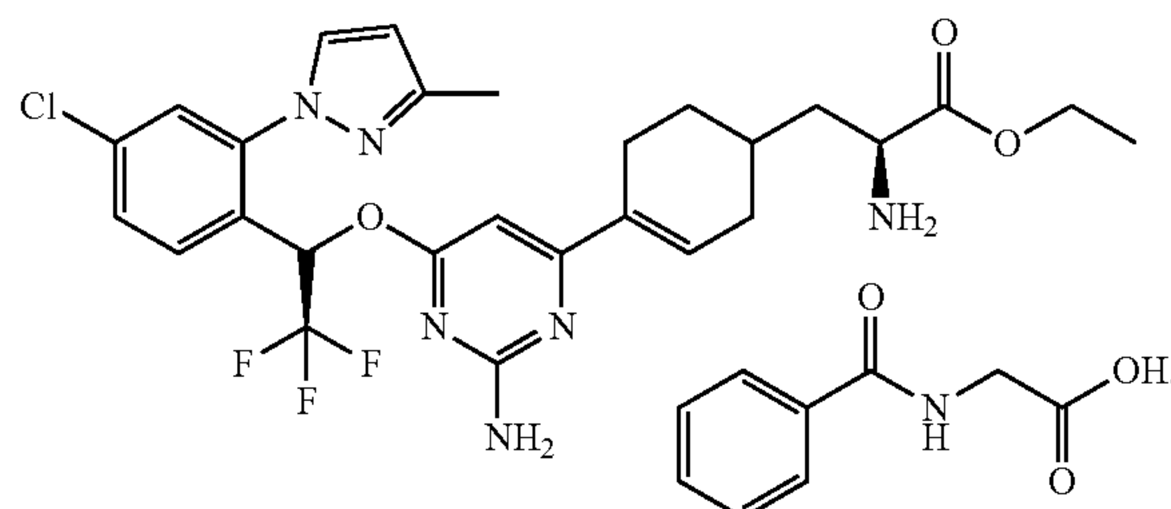
[Formula 53]
