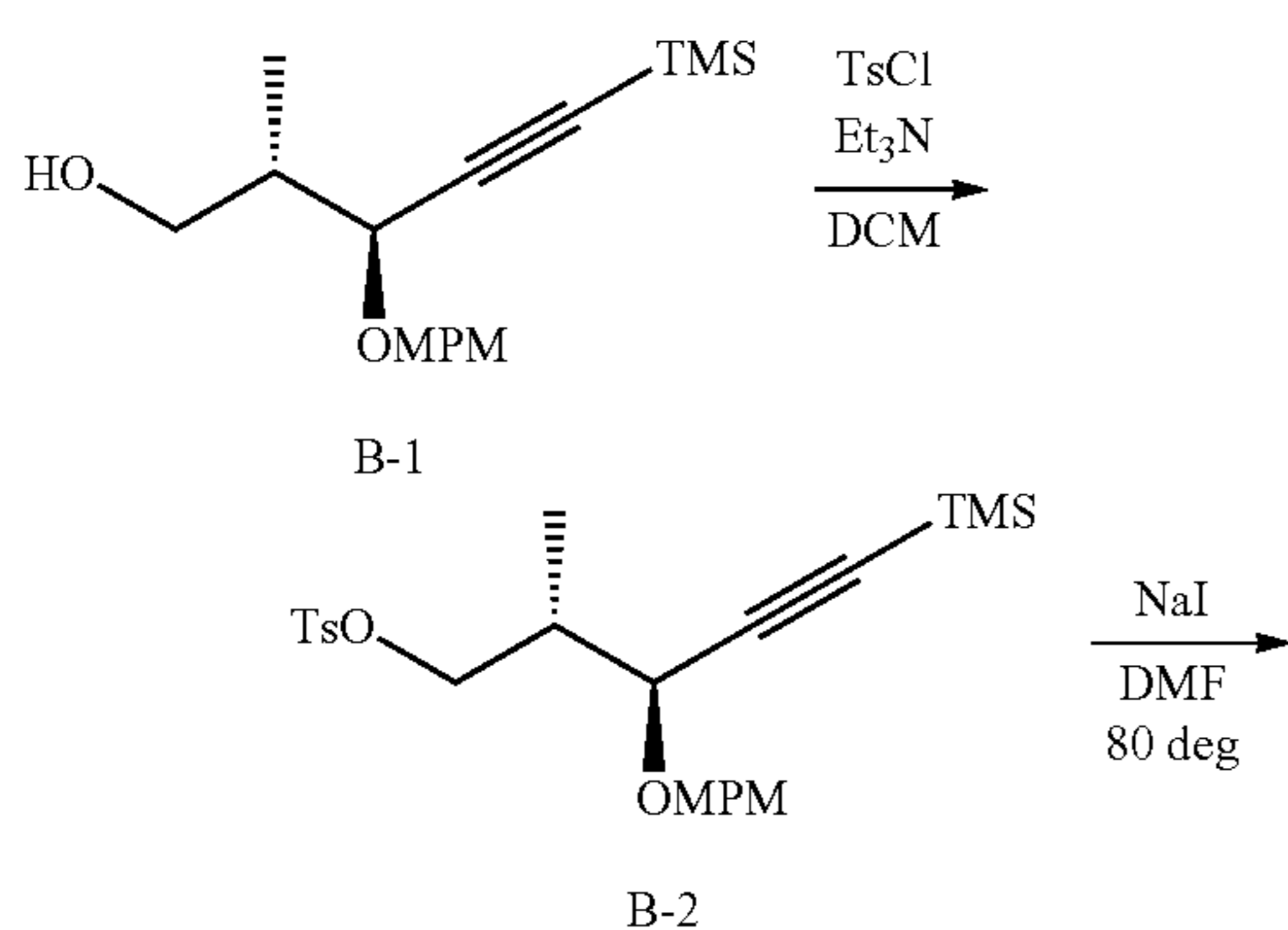
Scheme B; Preparation of Compound B-3
