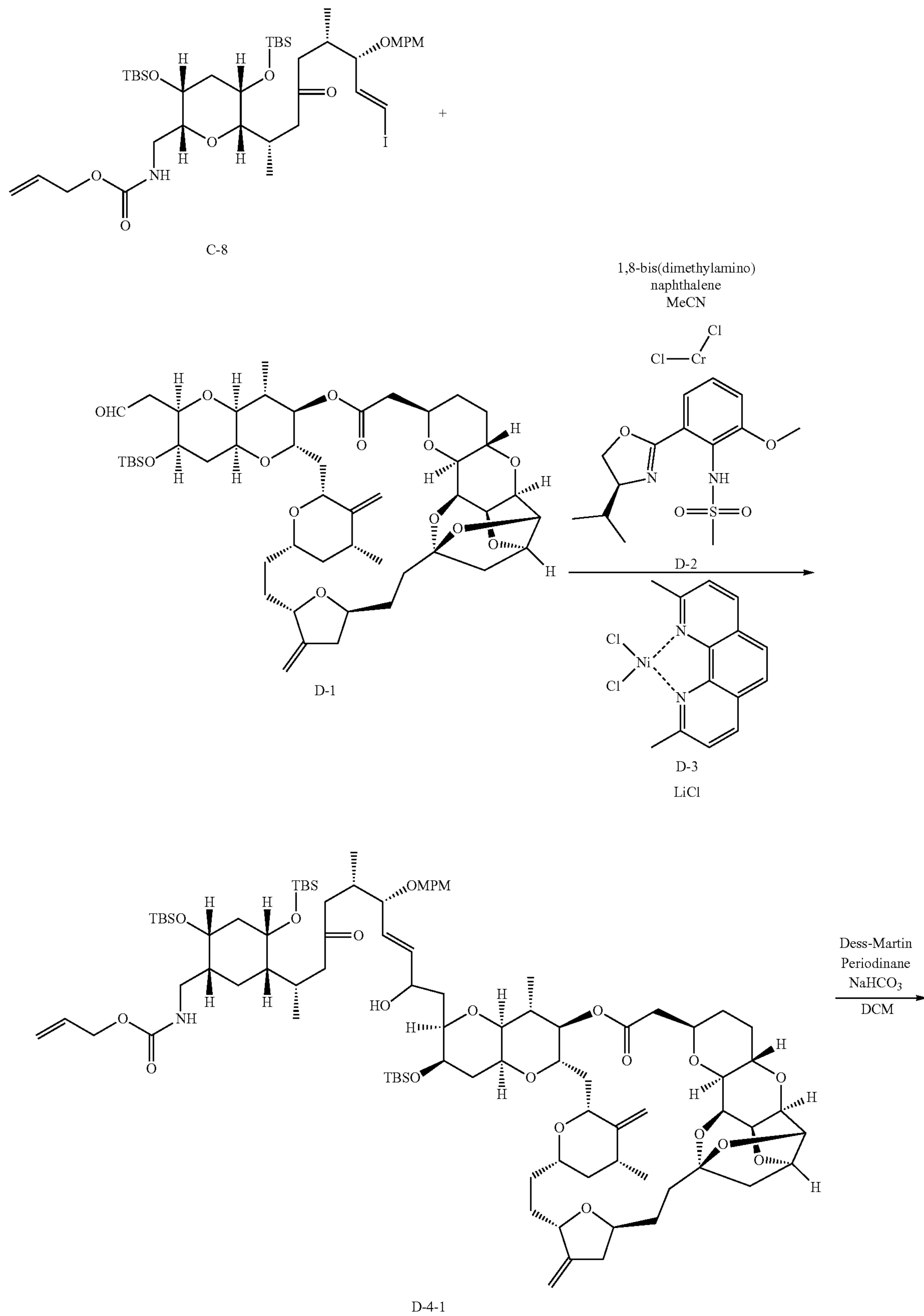
Scheme D-1; Preparation of Compound D-7-1
