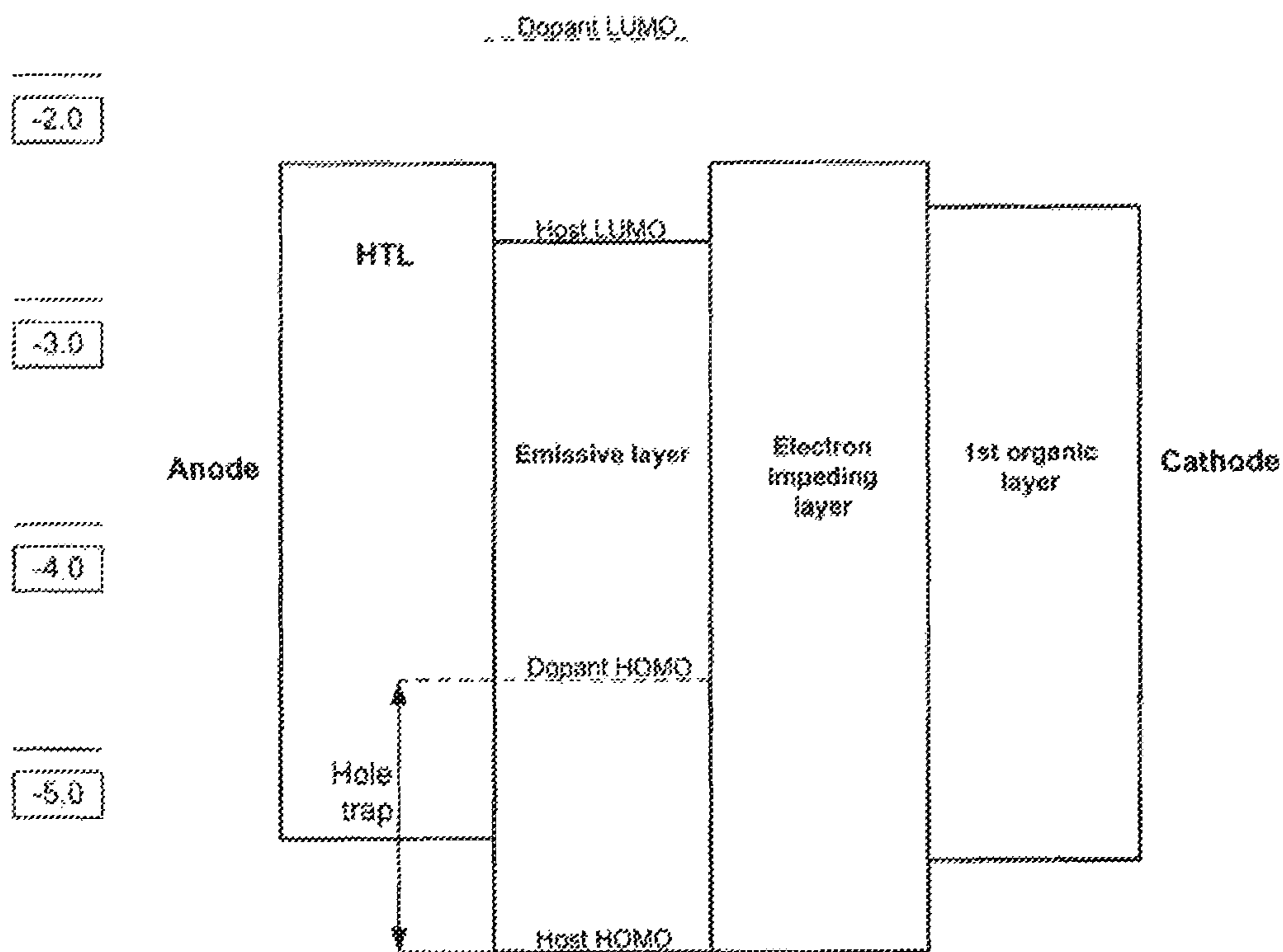
Figure 63b: Energy Level Diagram for a Device Having an Electron Impeding Layer
