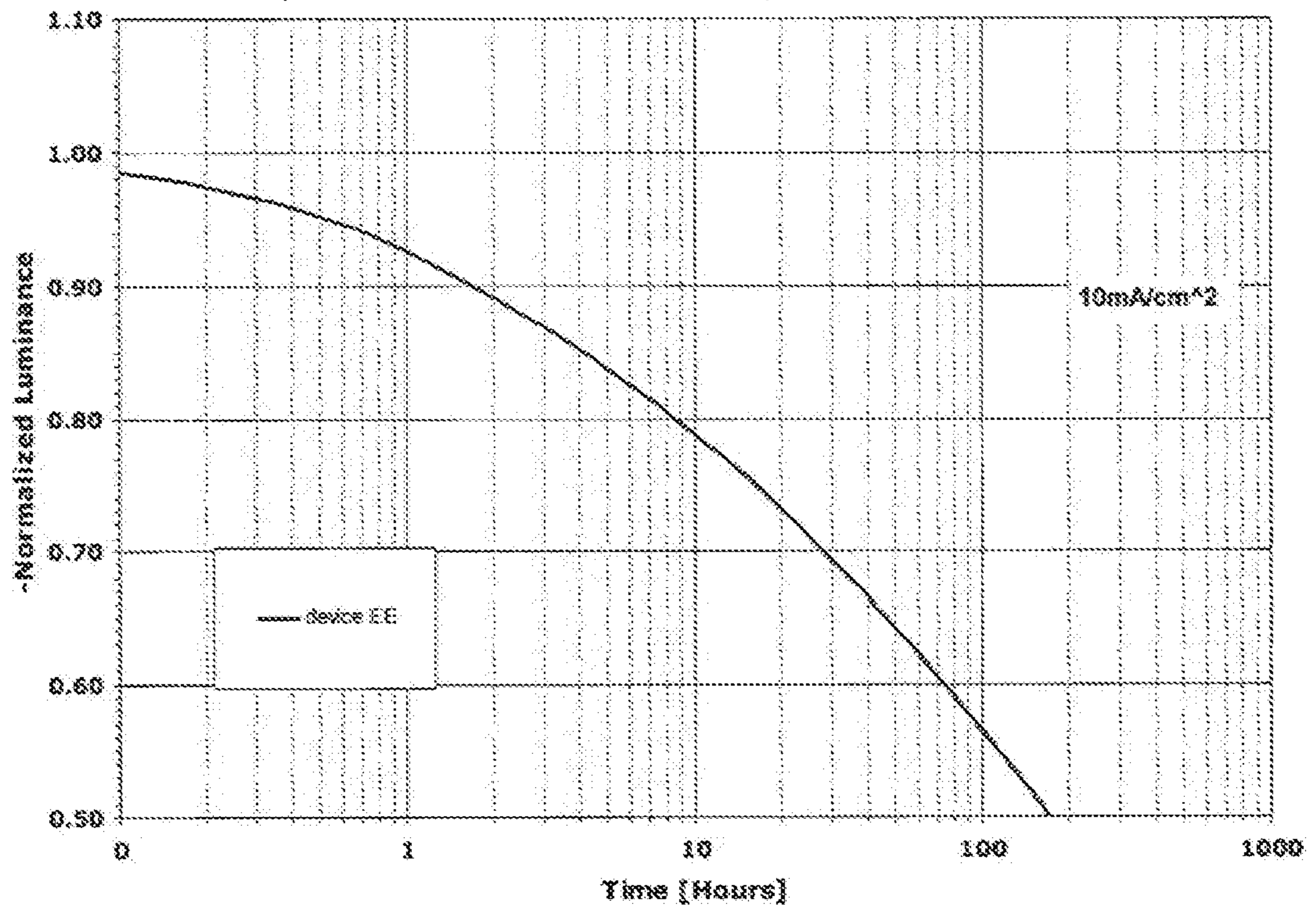
Figure 27 Lifetime (Device EE)
