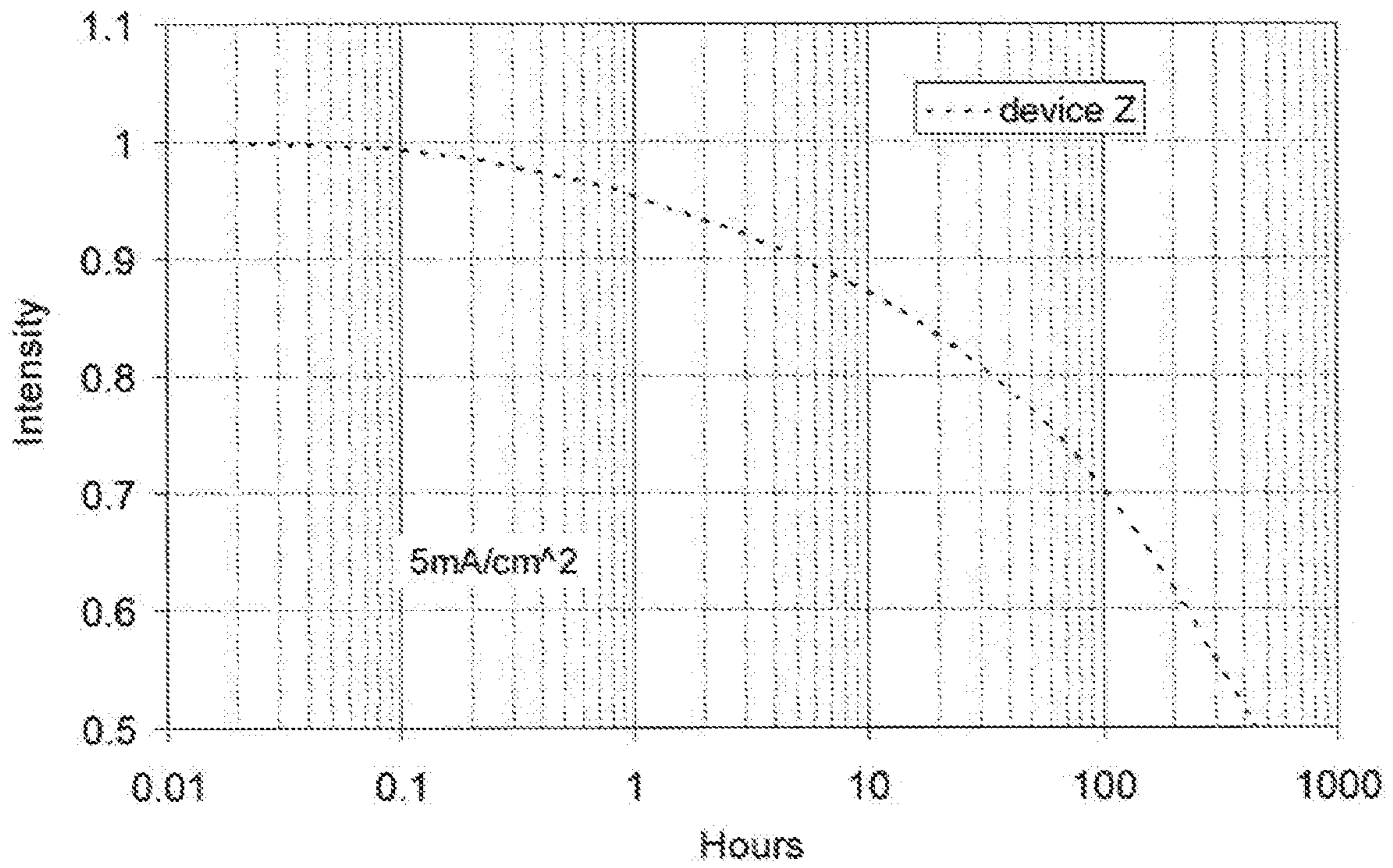
Figure 28 Lifetime (Device Z)
