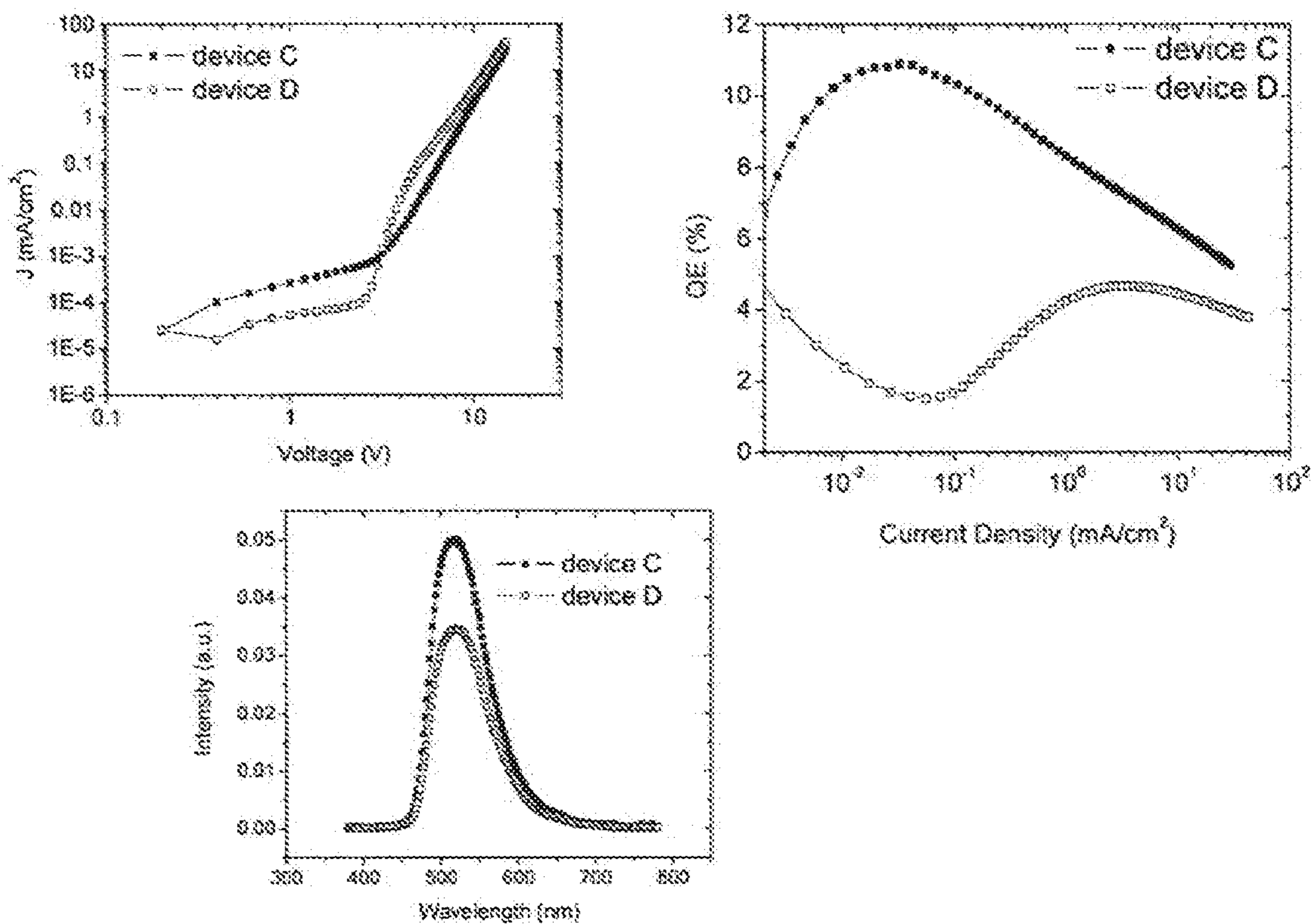
Figure 11 Devices C and D IV, QE vs. J and spectral data
