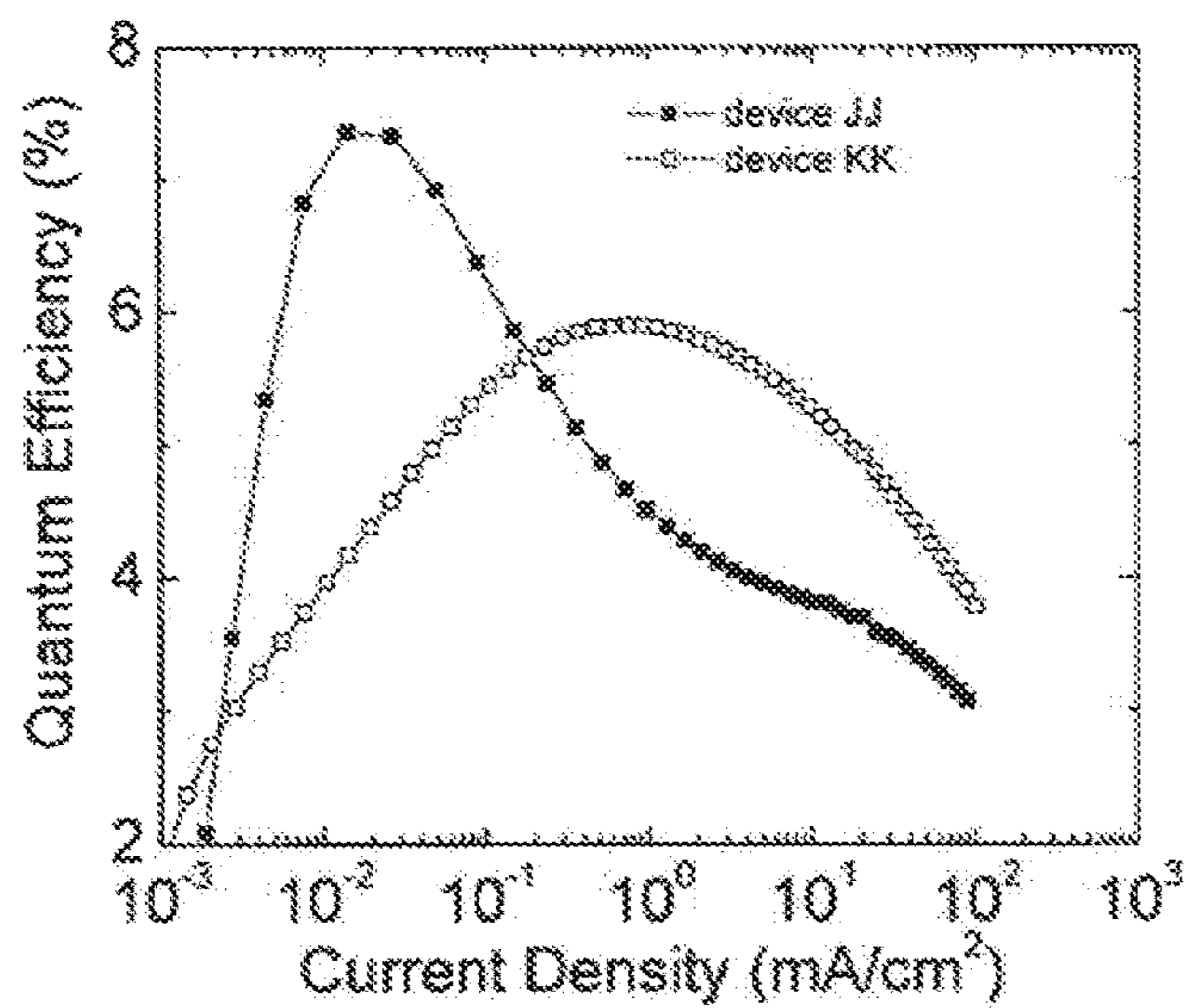
Figure 32 Devices JJ and KK IV, QE vs. J and spectral data
