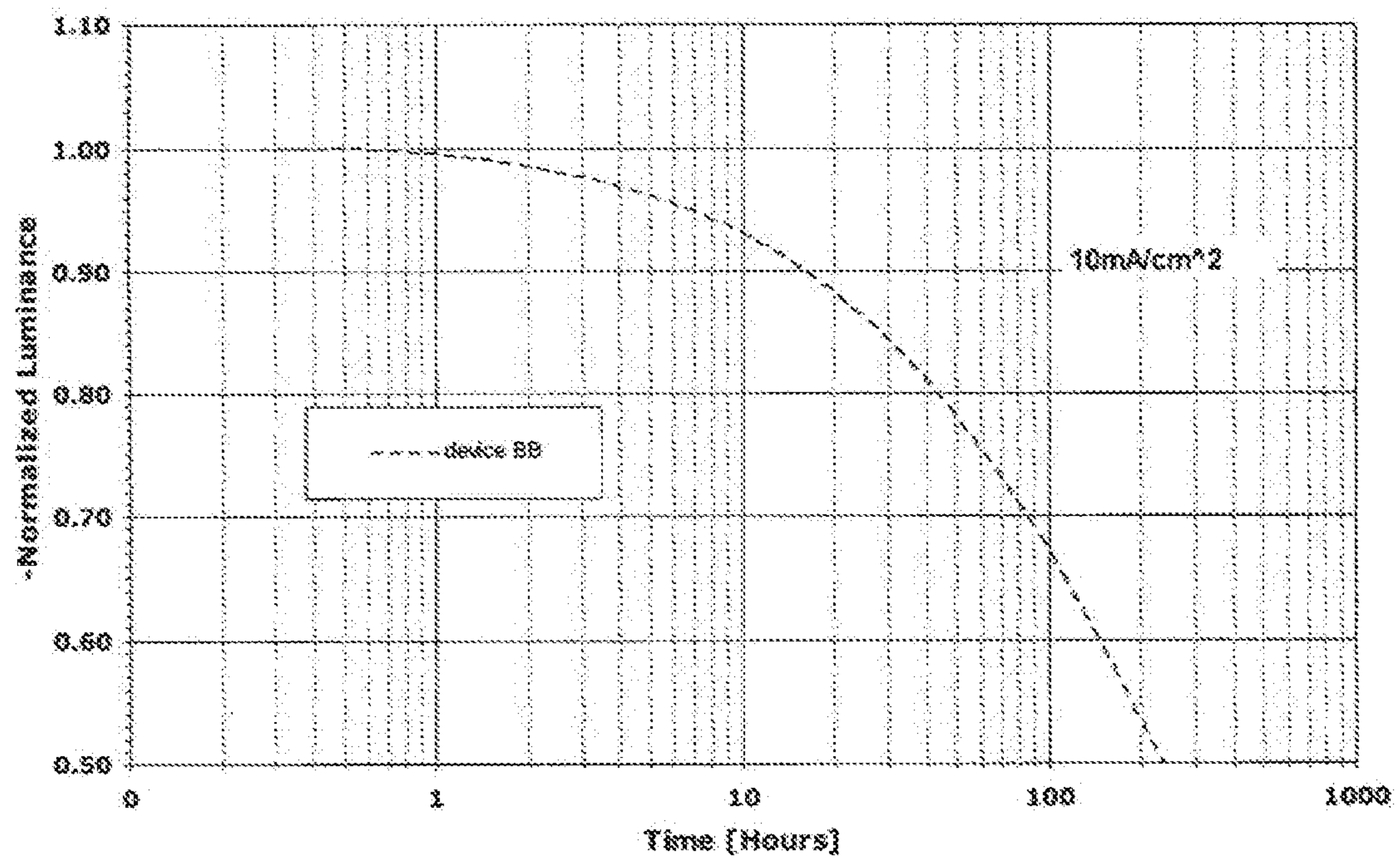
Figure 26 Lifetime (Device BB)
