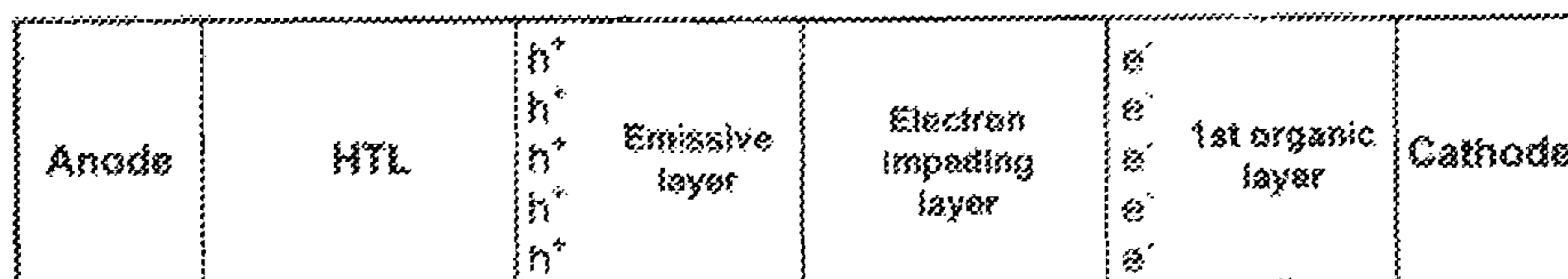
Figure 63a: Device Having an Electron Impeding Layer
