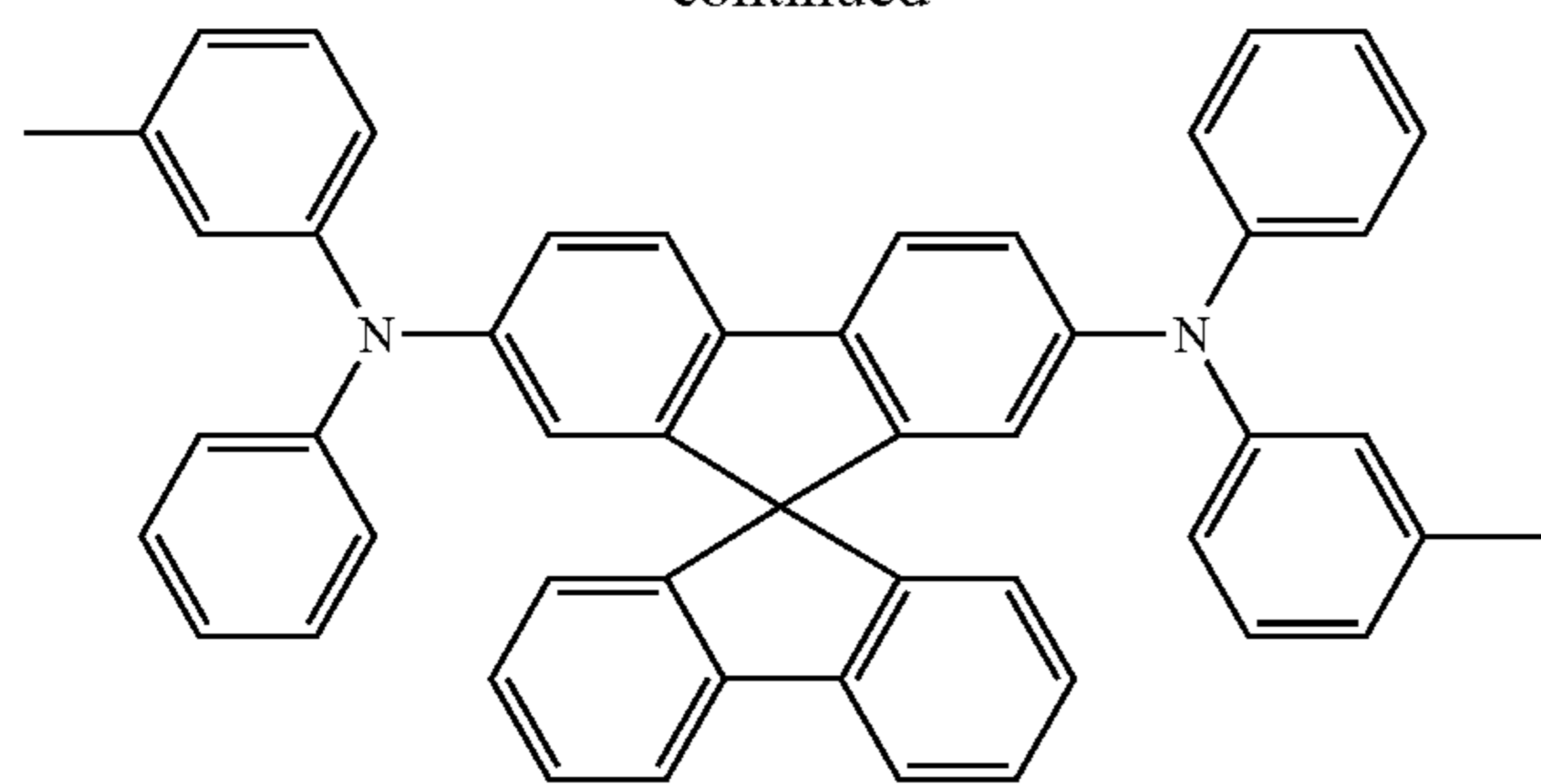
Spiro-TPD
