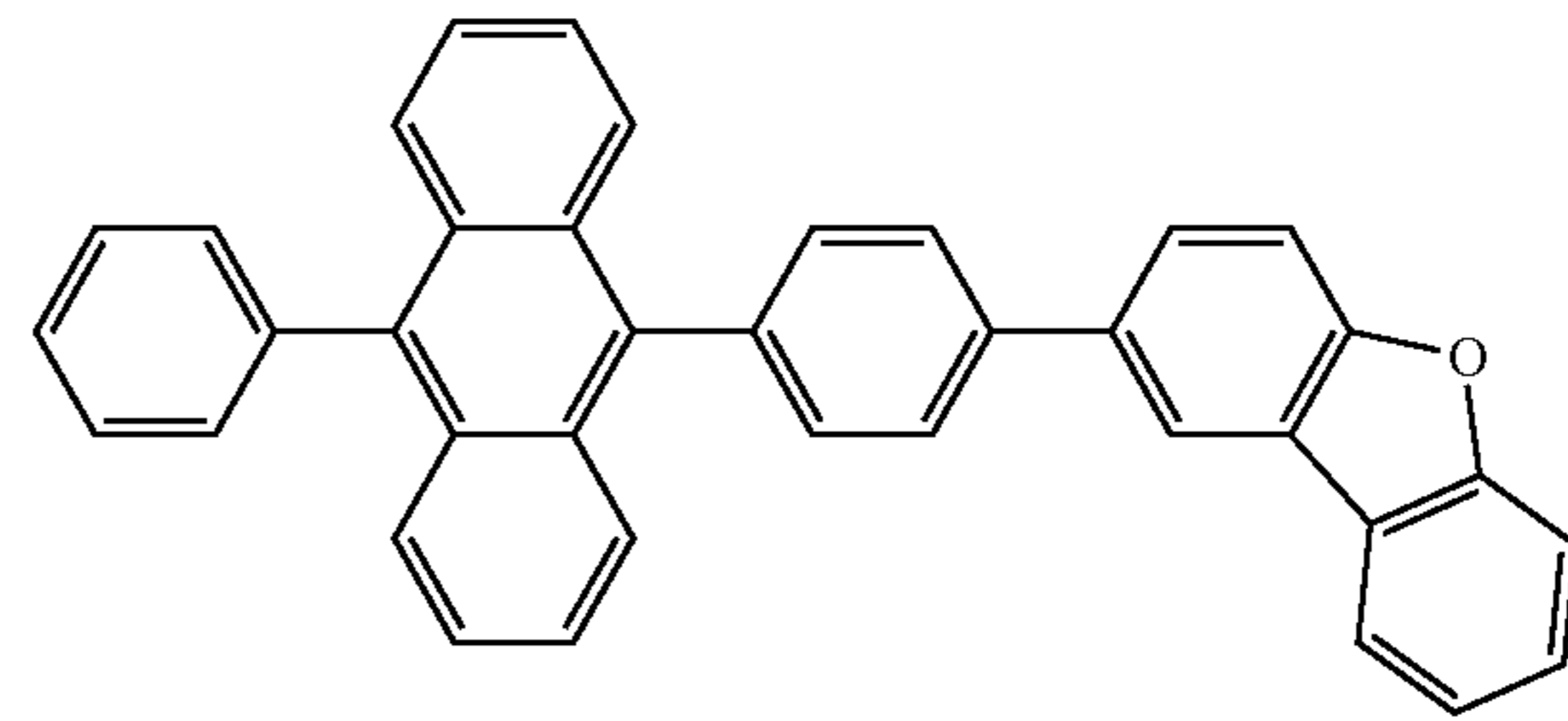
Compound 2-20
