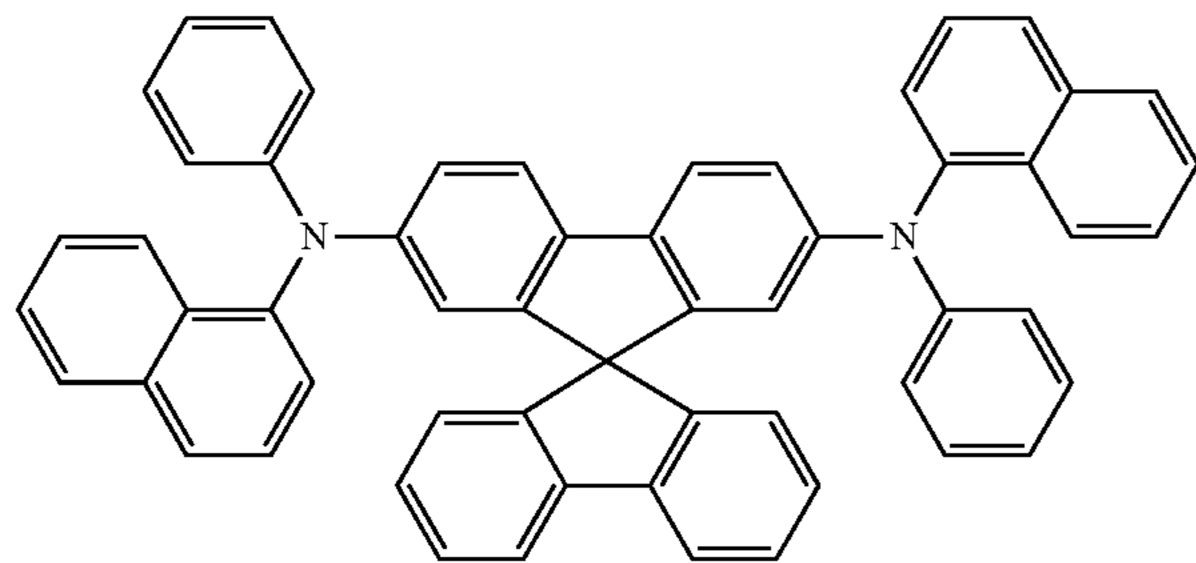
Spiro-NPB
