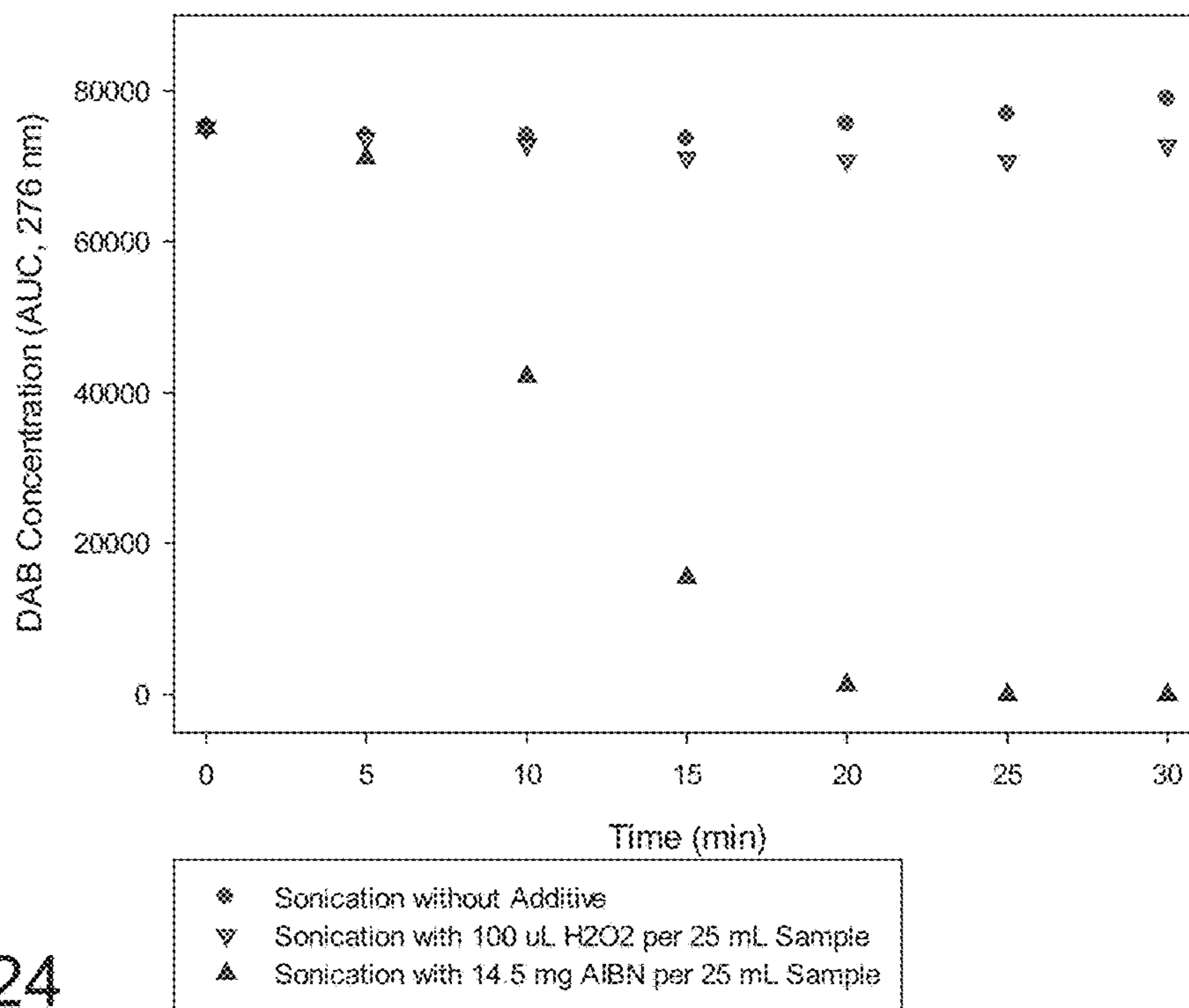
DAB Radical Oxidation Sonication with Additive (25 mL)
