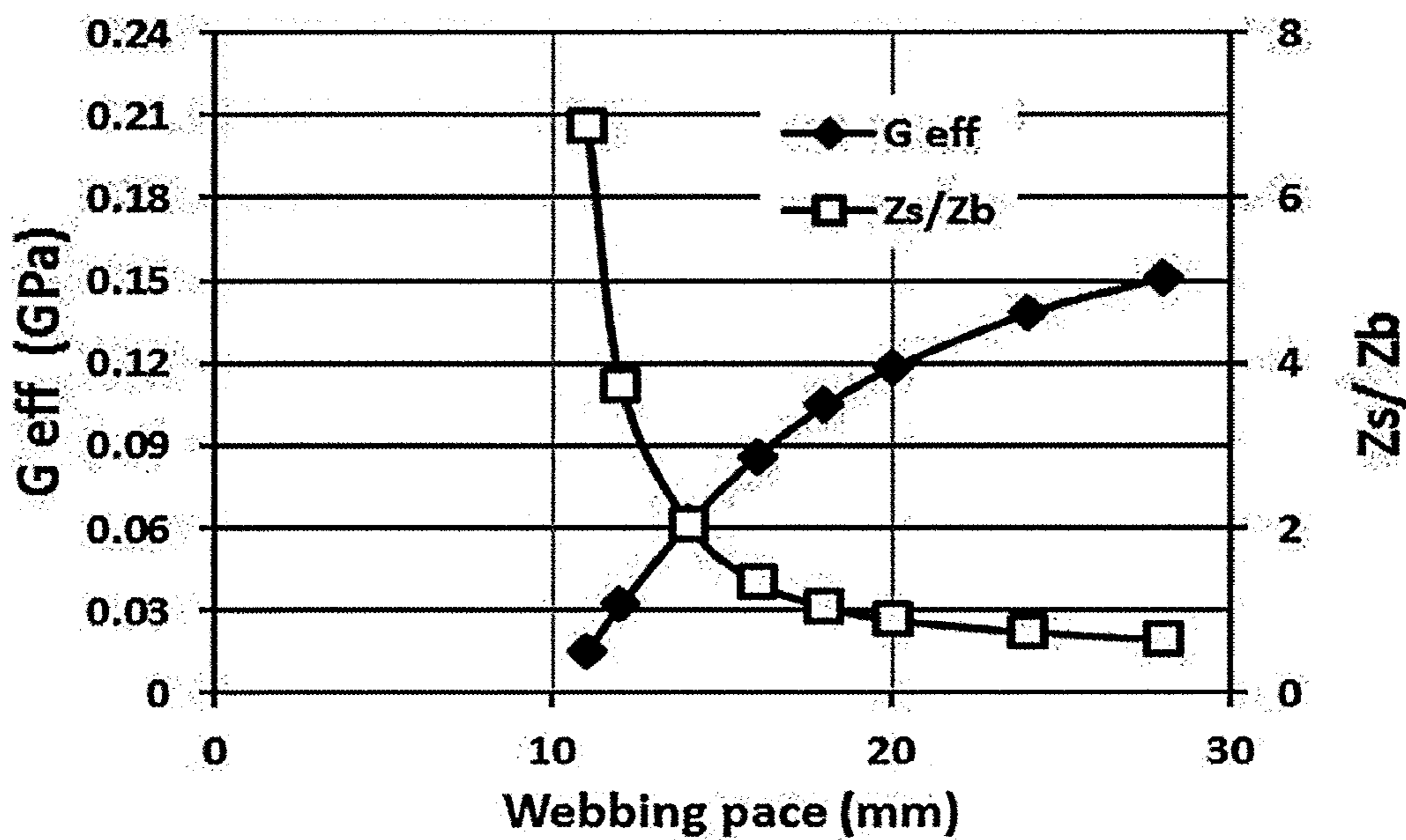
Fig. 17 – FEA results, with L = 60 mm, E = 1, ν = 0.45, Rc = 10 mm, t = 2 mm
