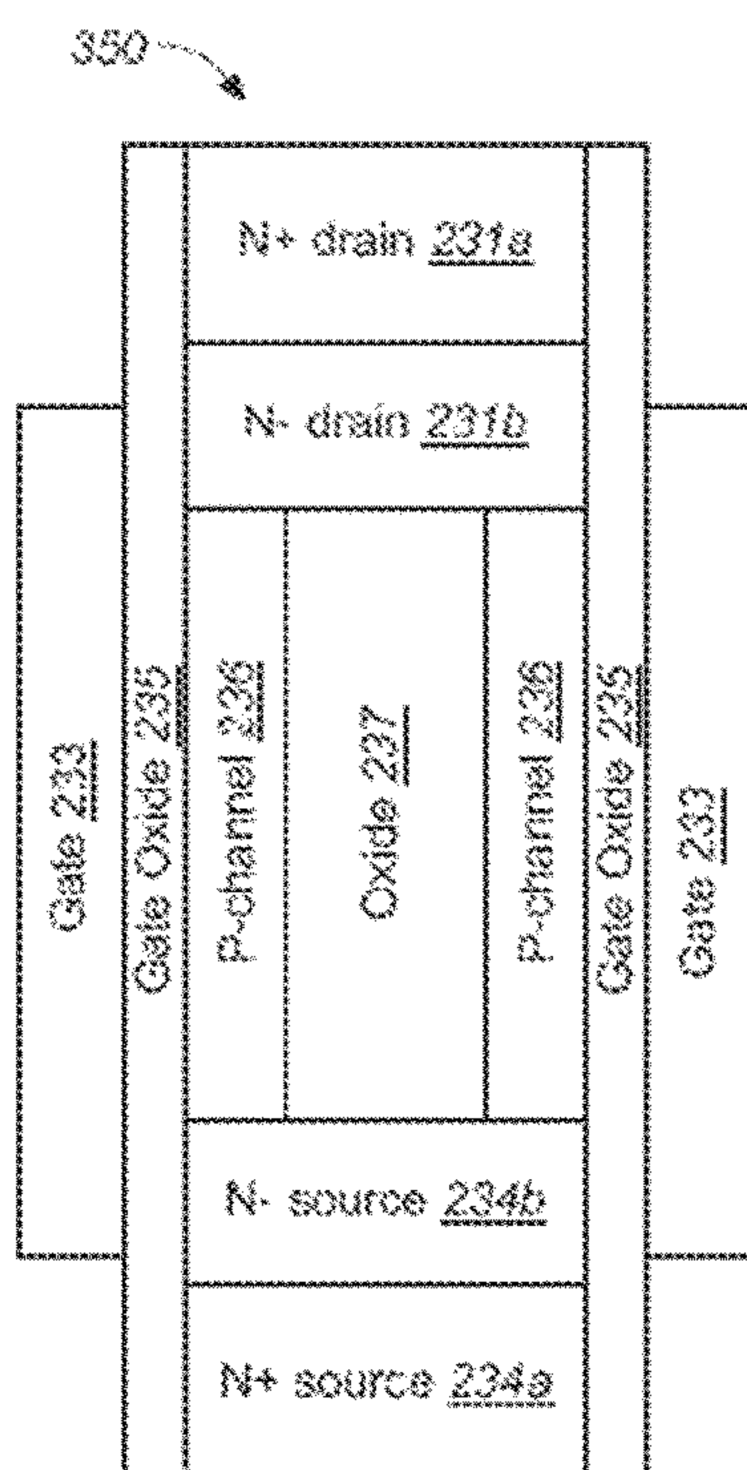
Thin Channel FIG. 2c
