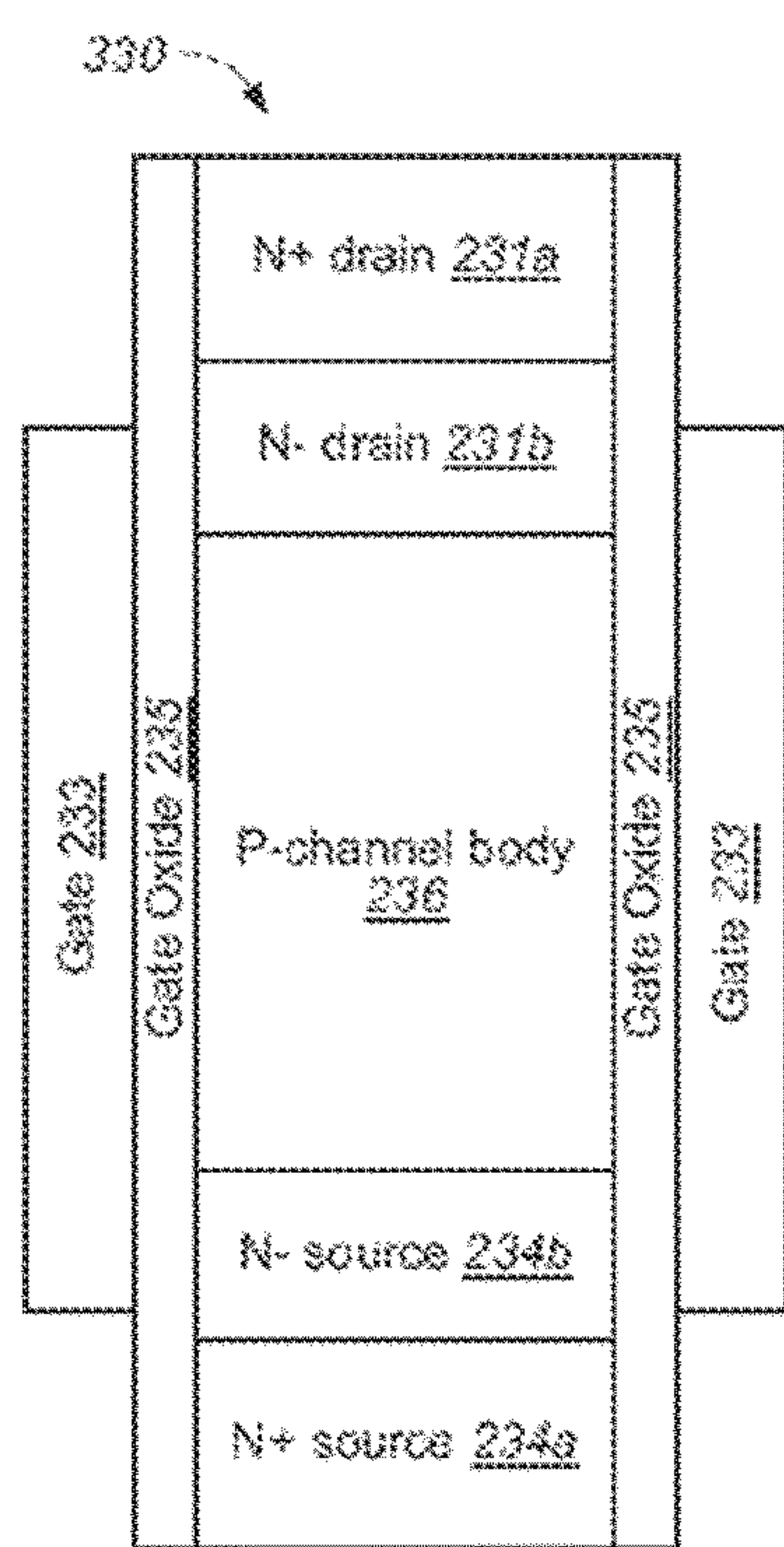
Full poly body FIG. 2b
