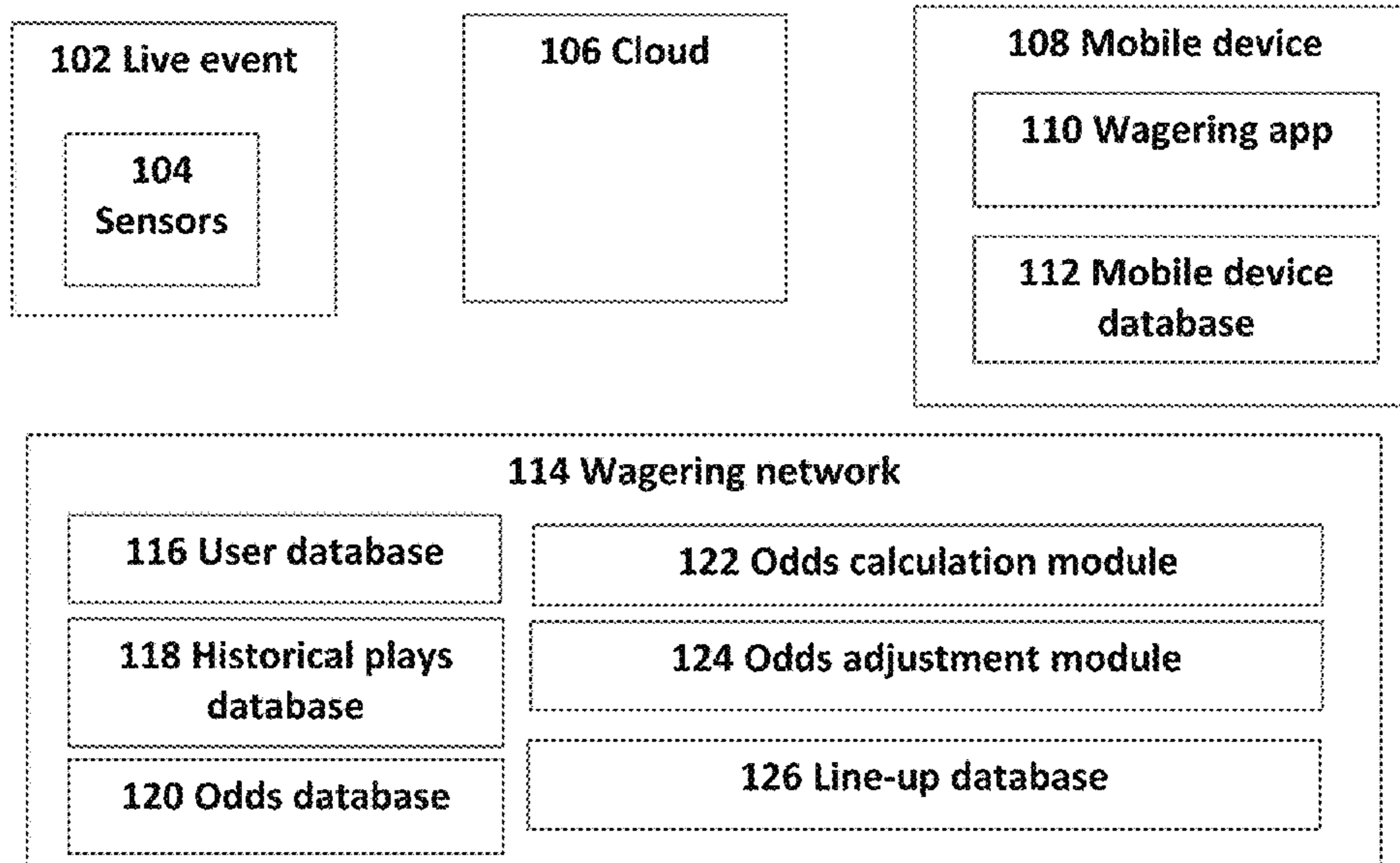
A system for lineup-based odds adjustment
