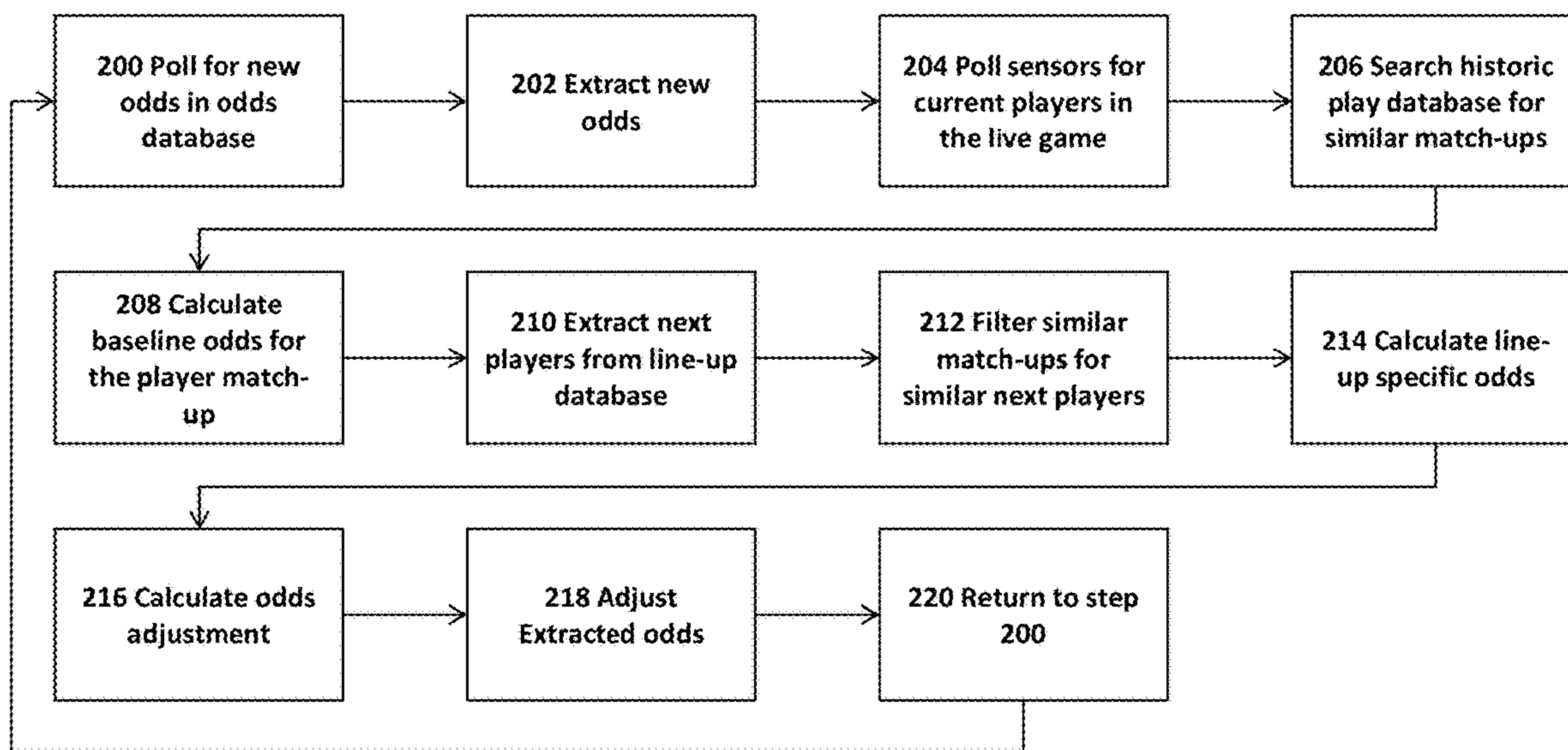
Fig.2 Odds adjustment module
