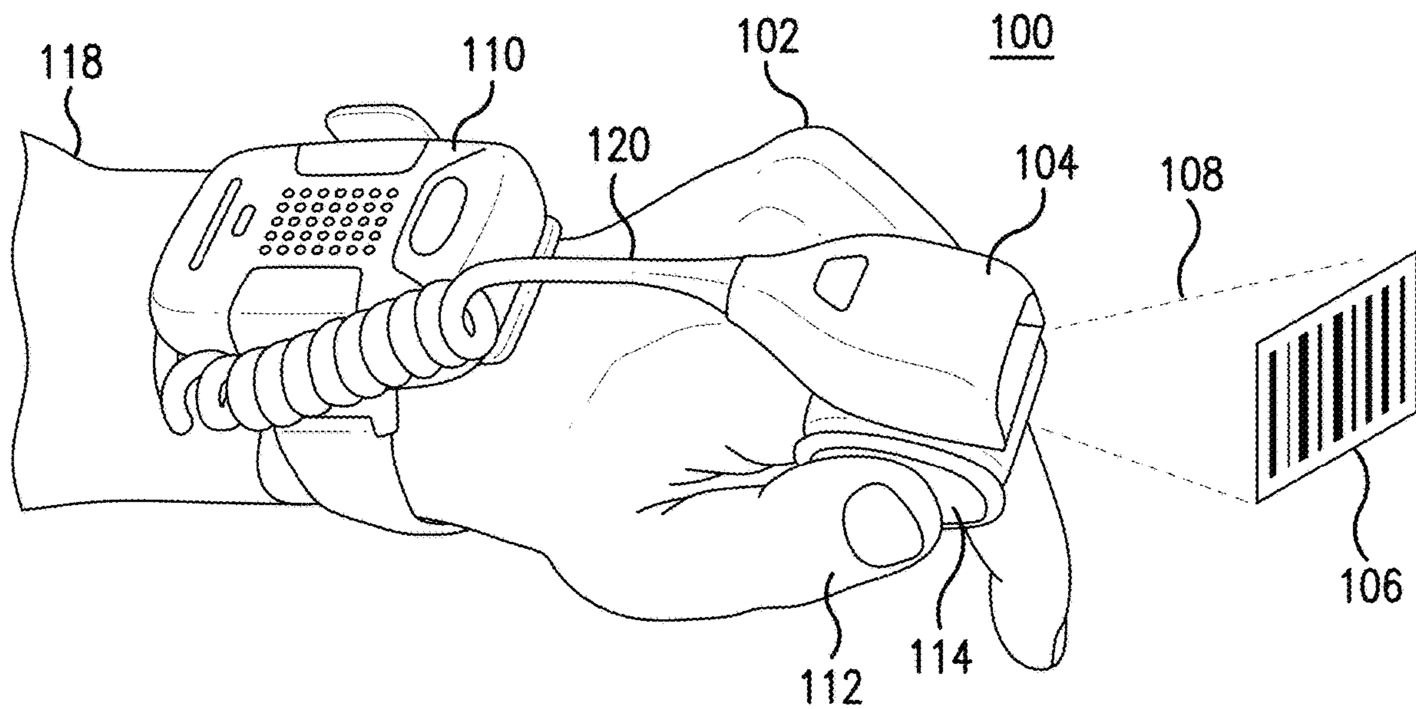
FIG. 1 (PRIOR ART)
