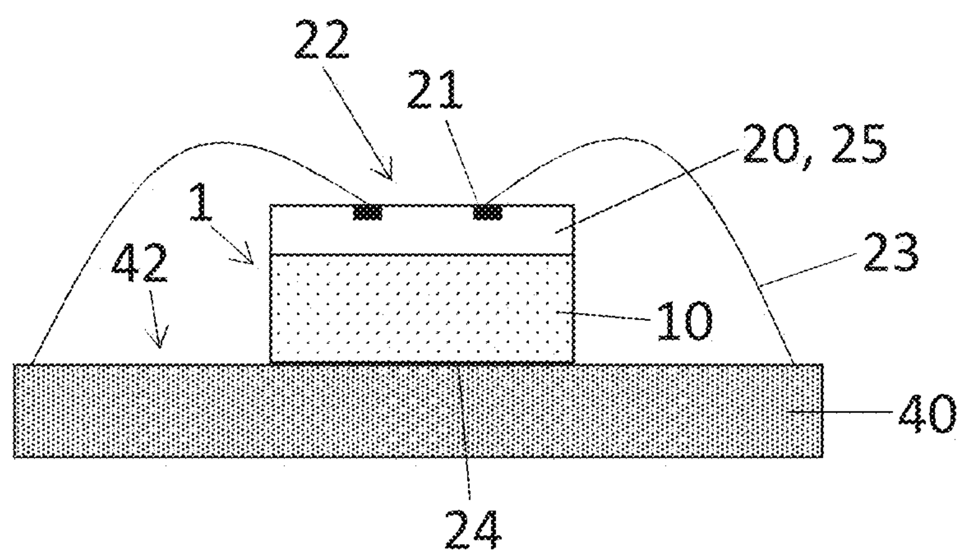
Fig. 5 (prior art)
