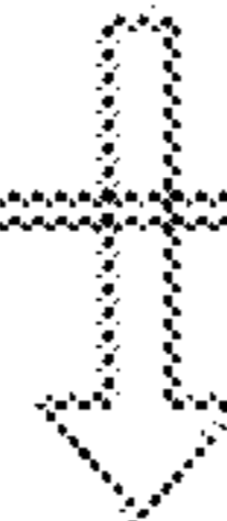
CSR representation
