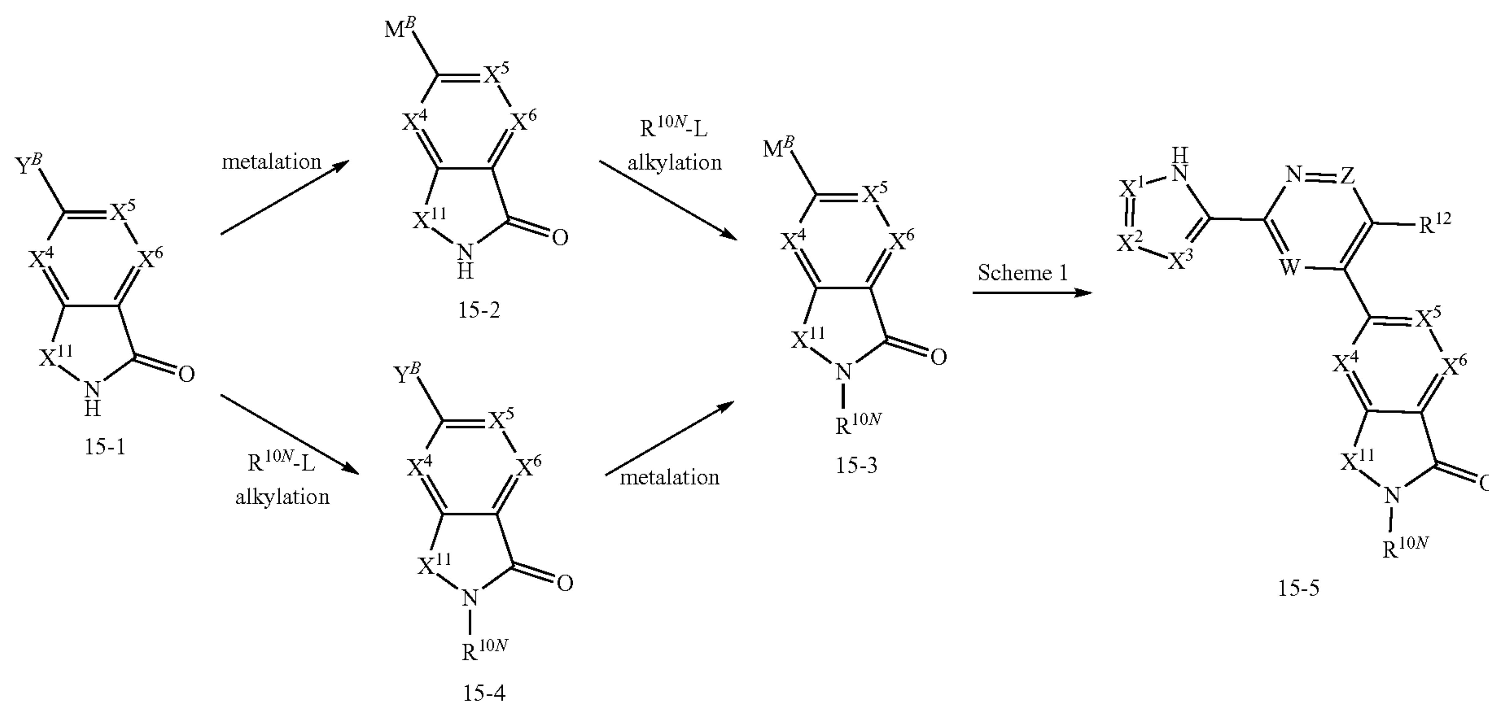
Scheme 15.
