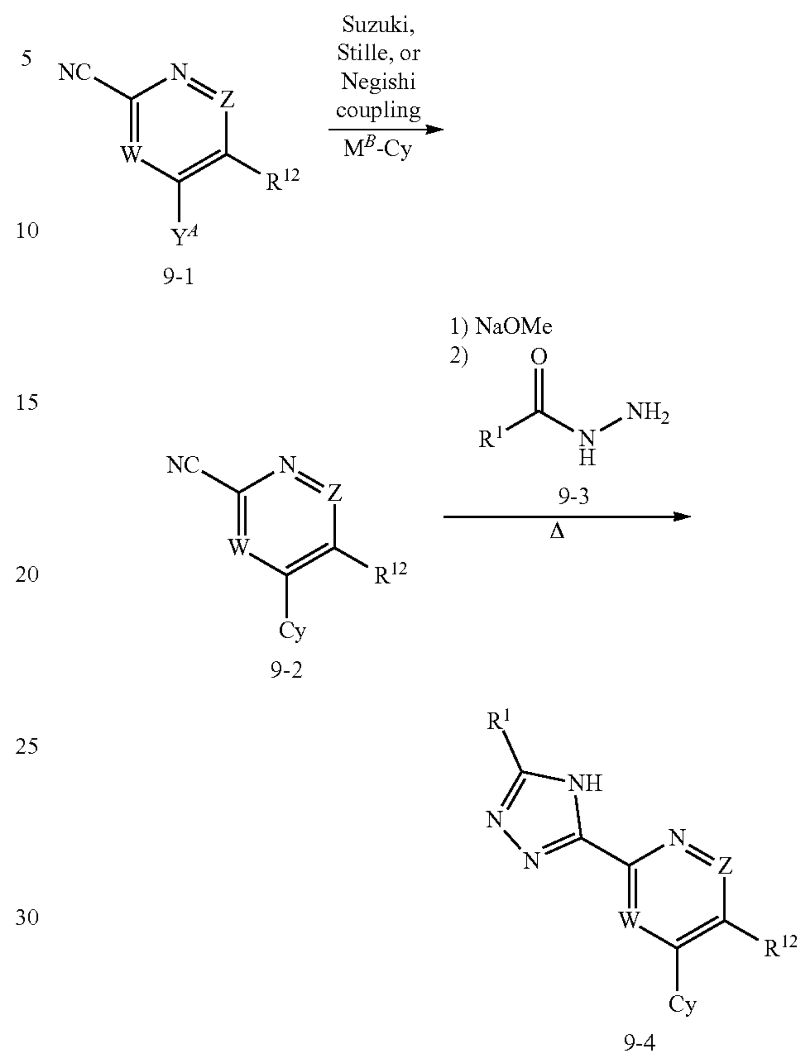
Scheme 9.
