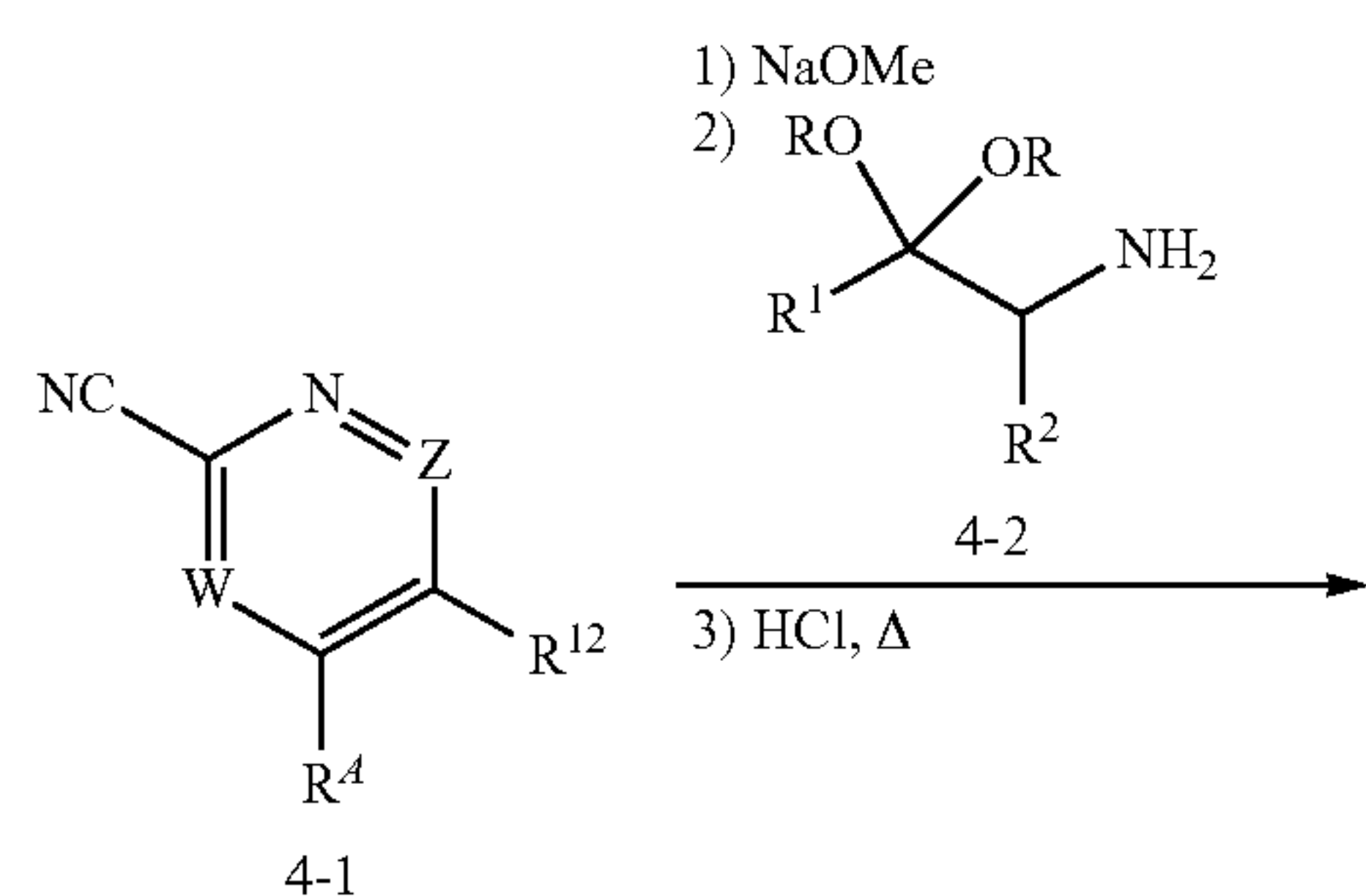
Scheme 4.
