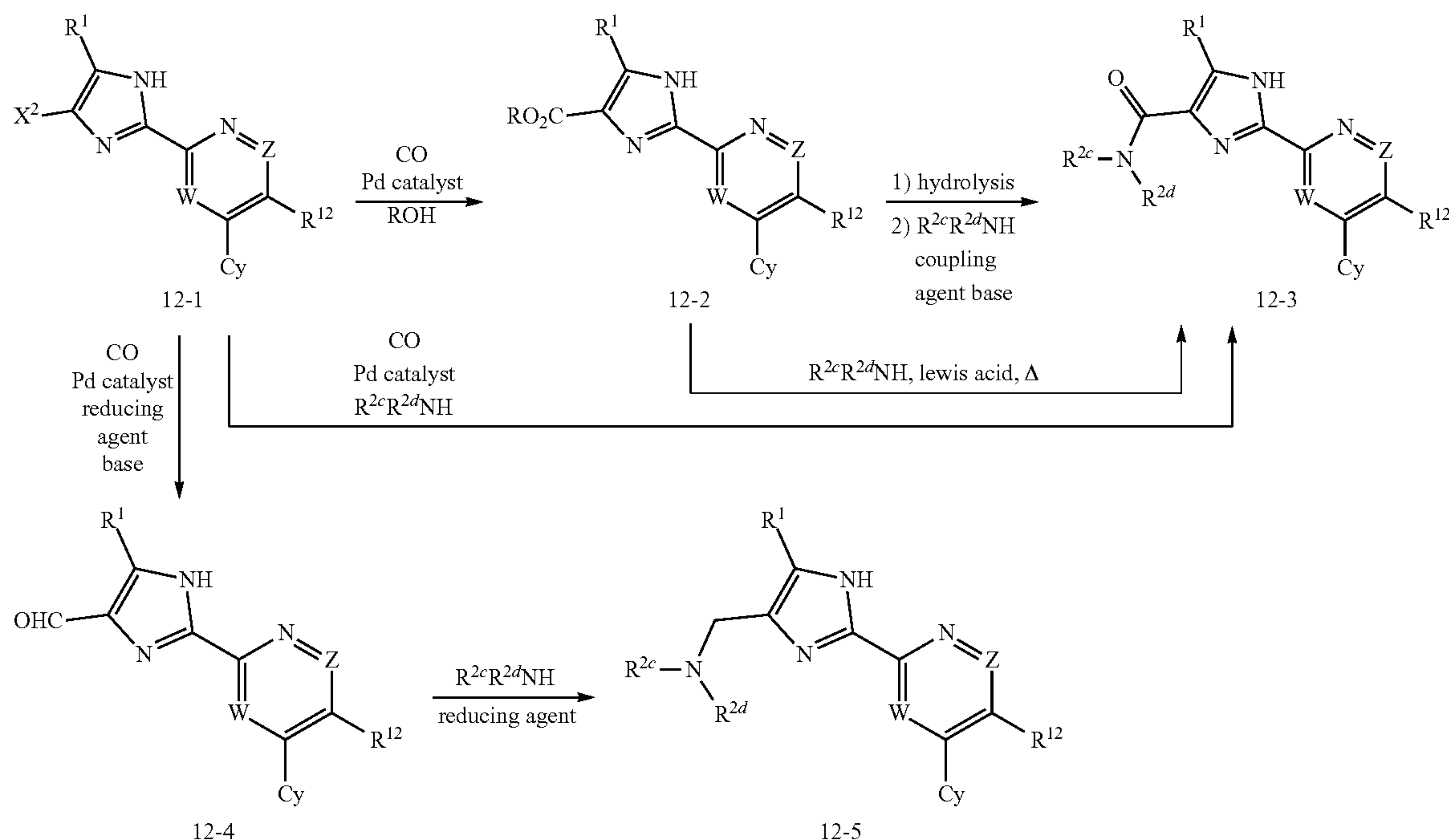
Scheme 12.
