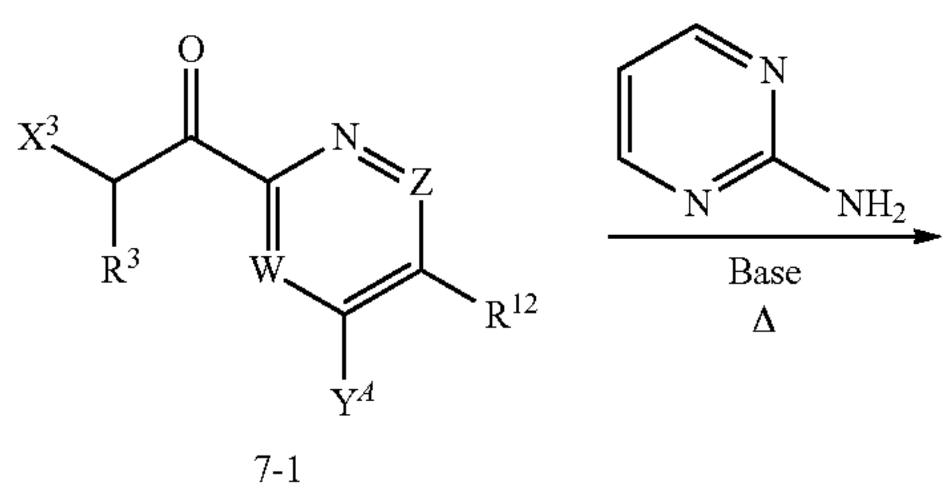
Scheme 7.
