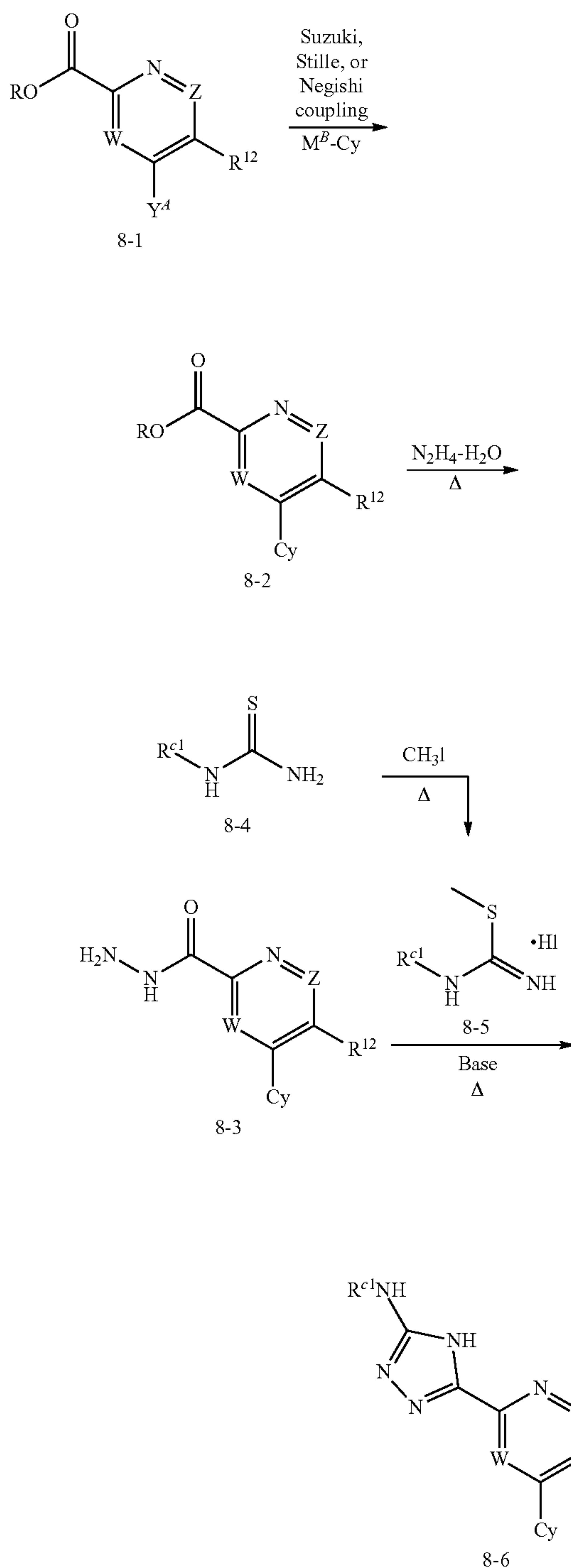
Scheme 8.
