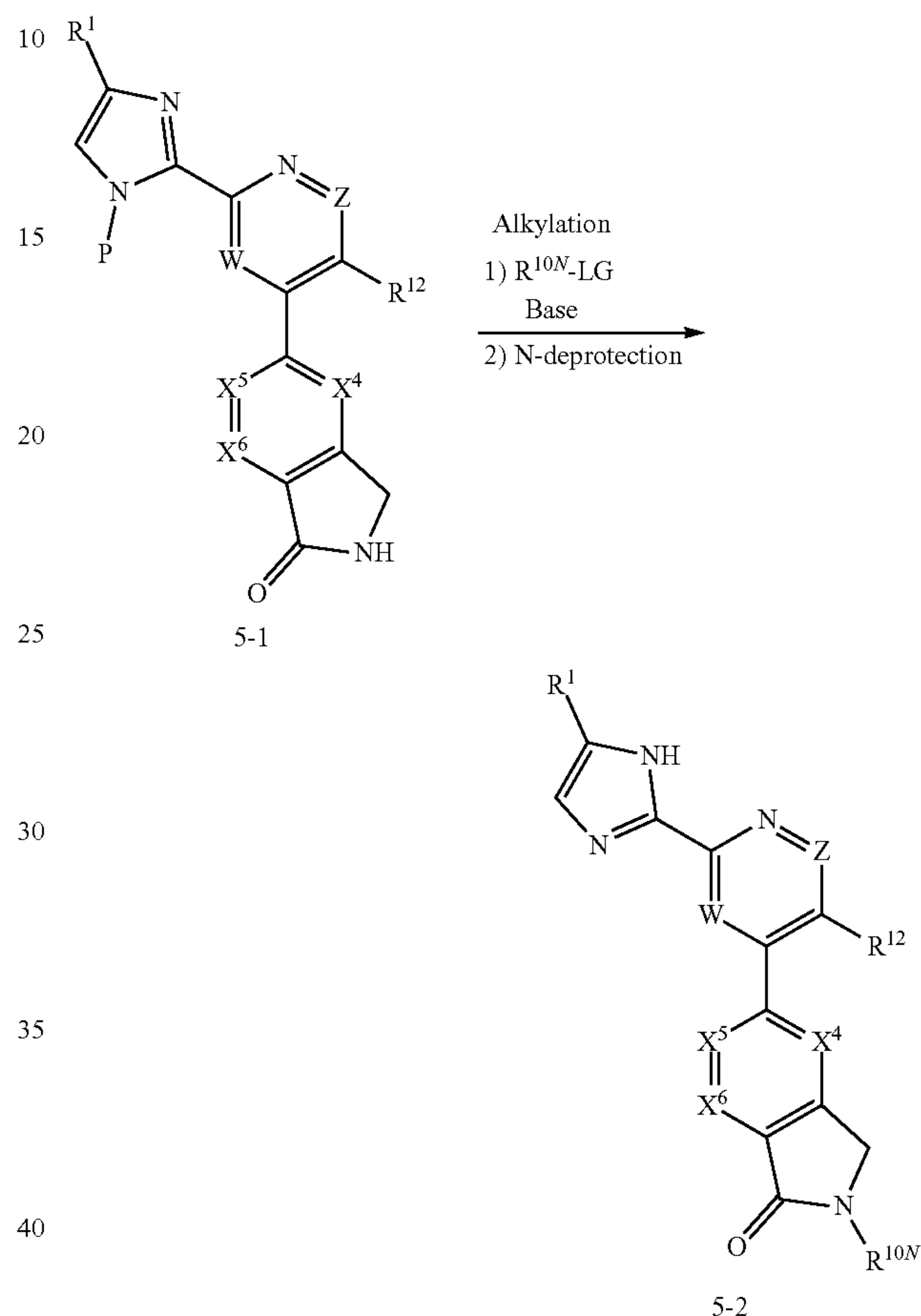
Scheme 5.
