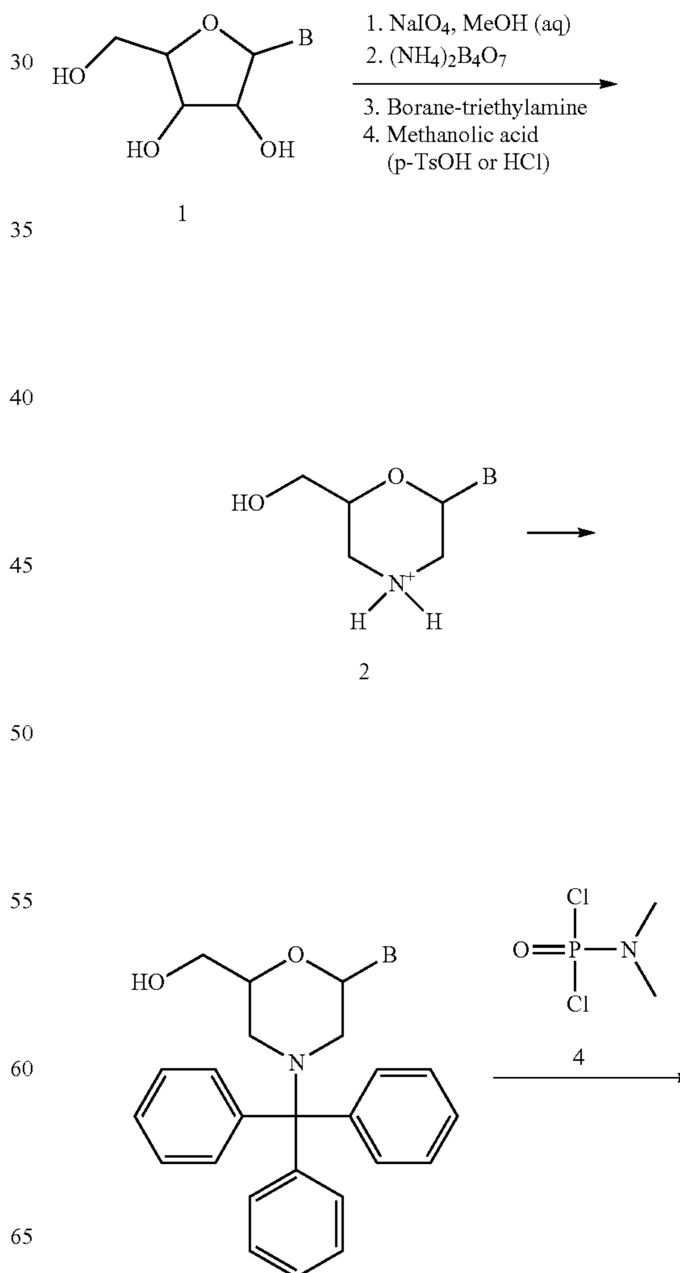
Scheme 1: General synthetic route to PMO Subunits
