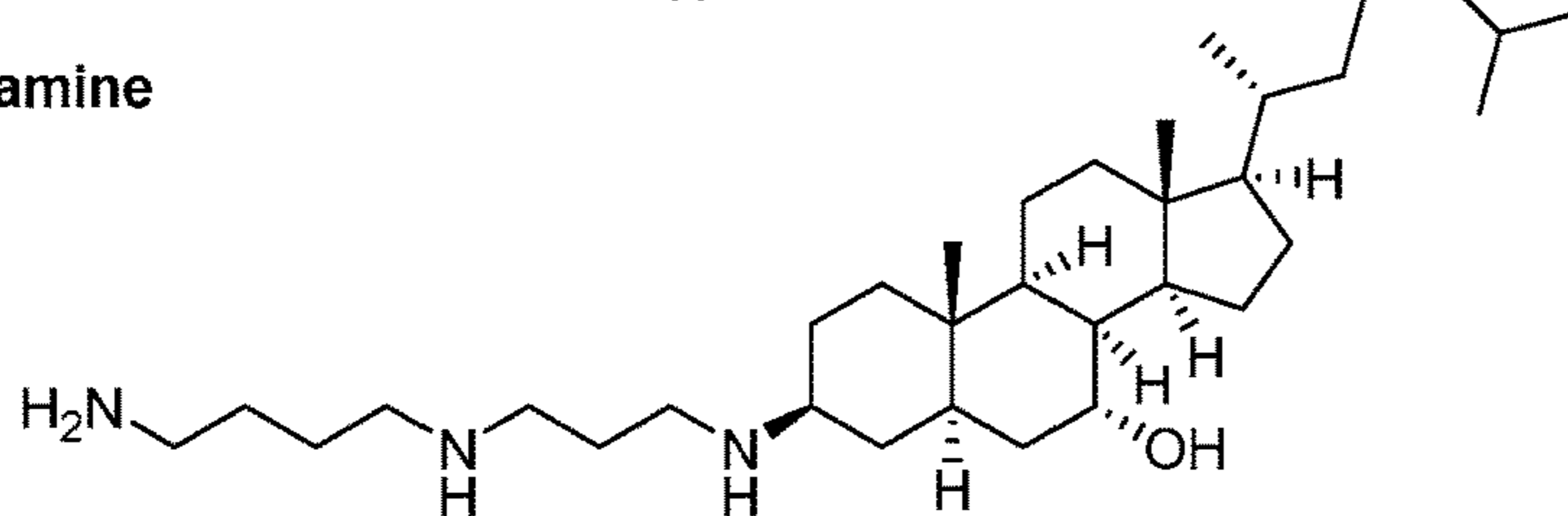
Deoxyspergualin
