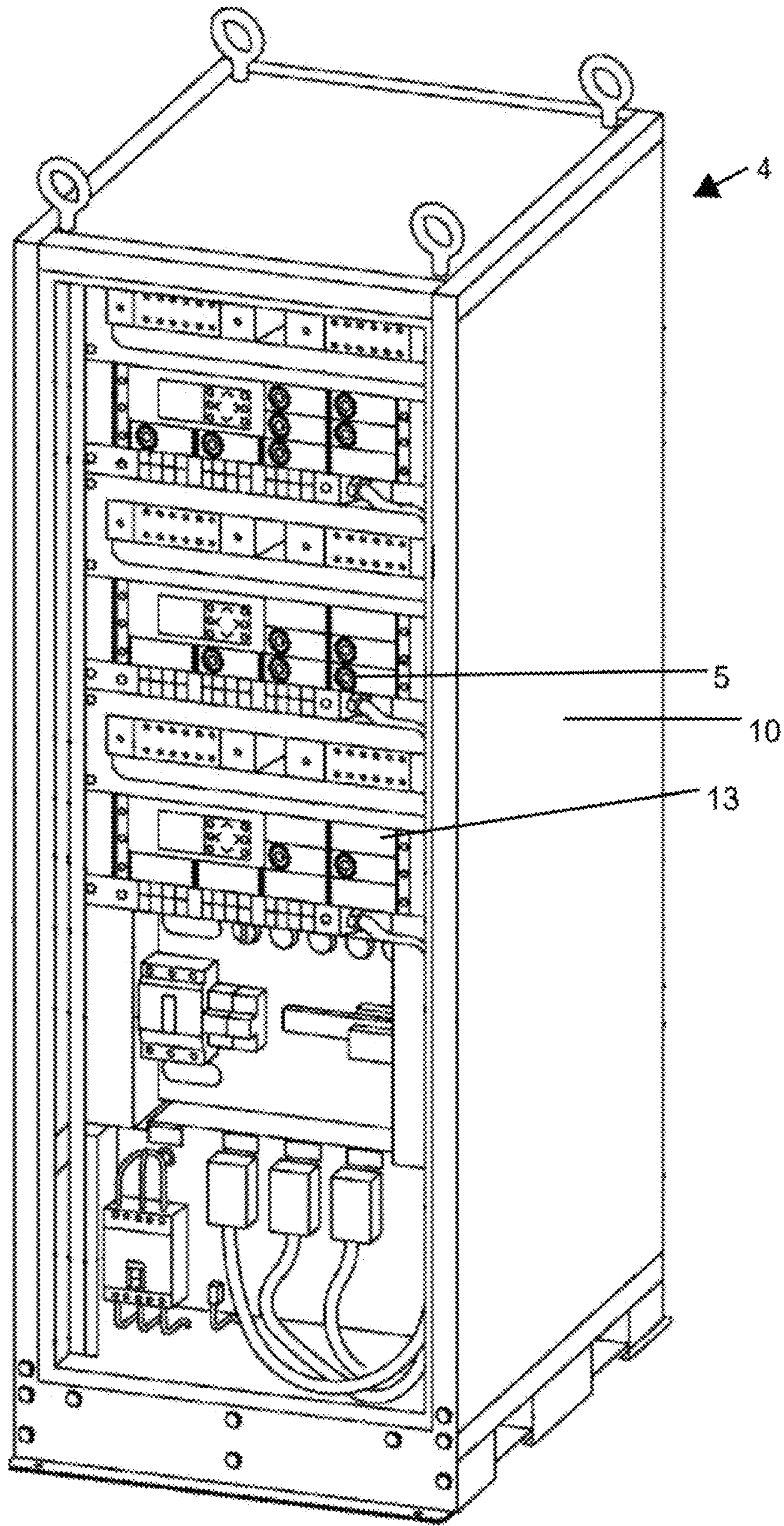
Figure 17 (prior art)
