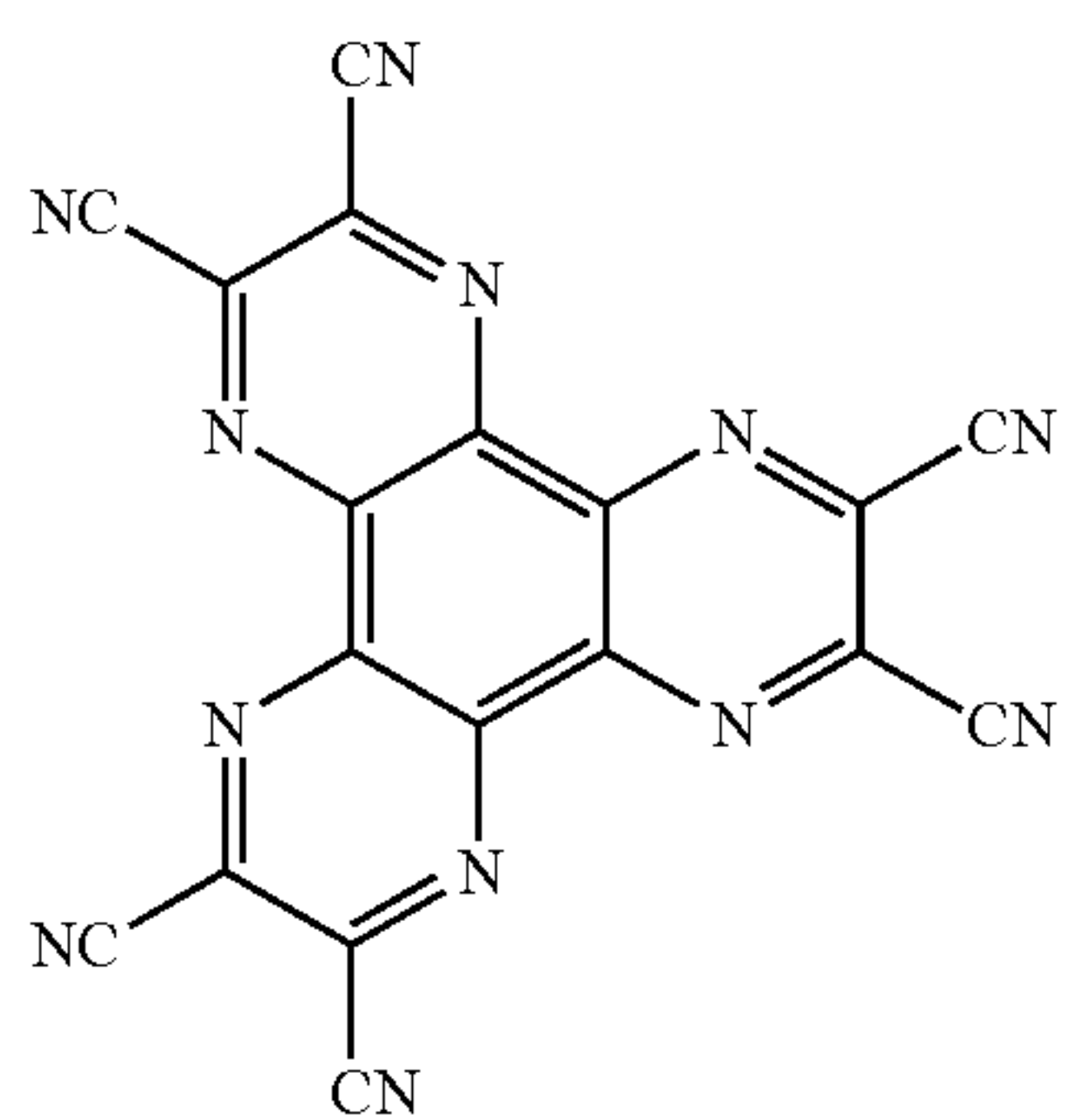
HATCN
