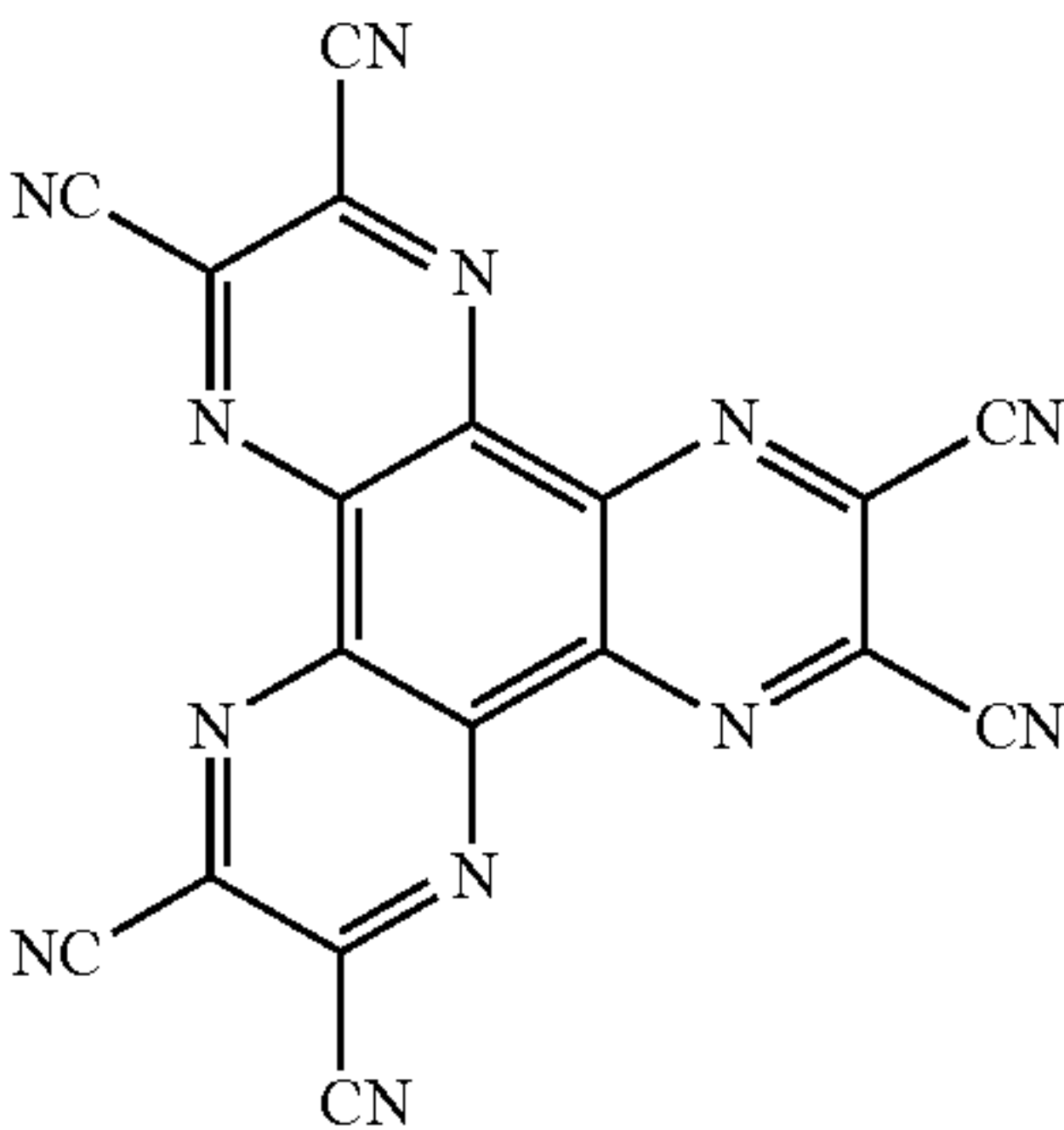
HAT-CN
