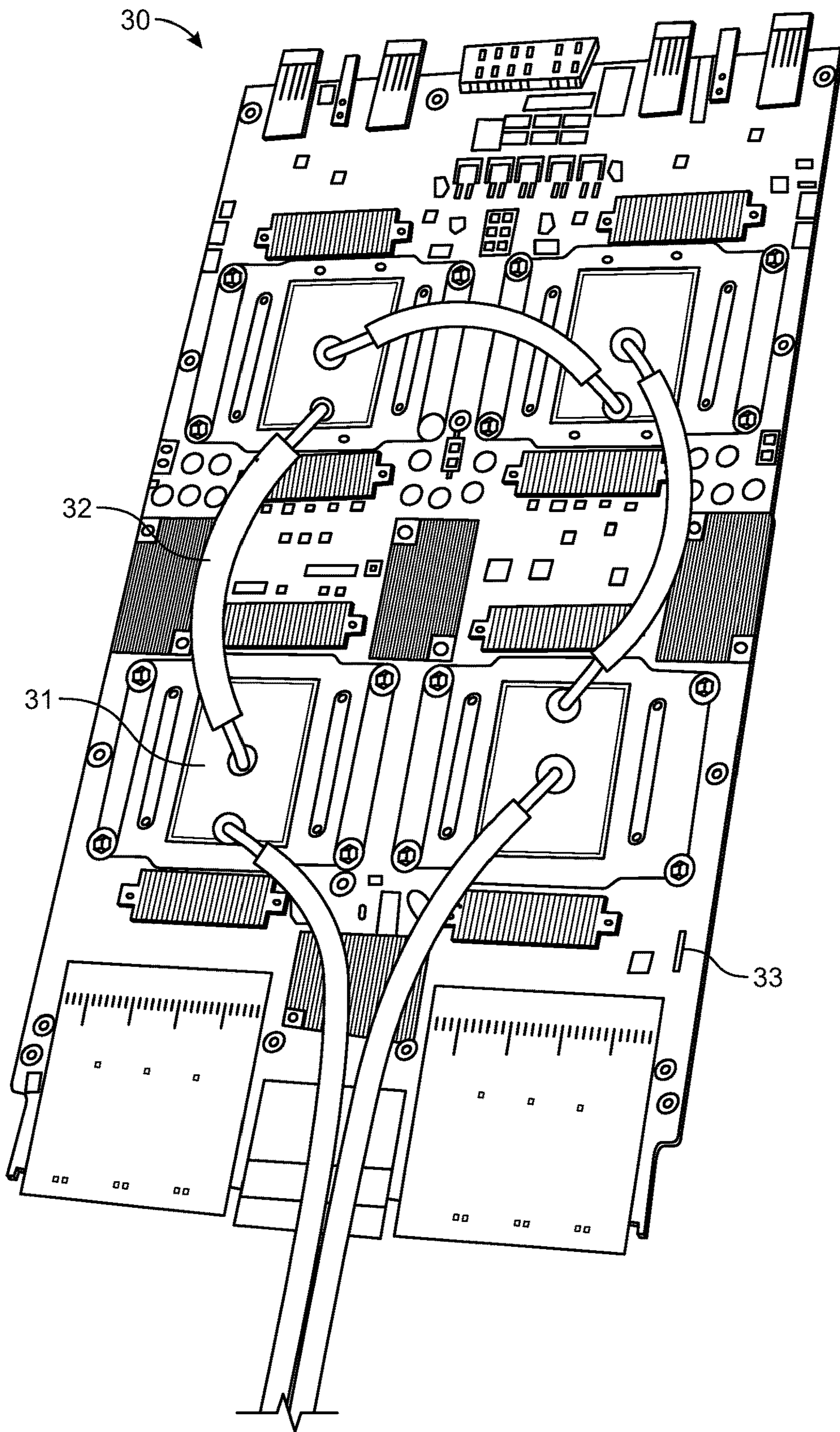
FIG. 3 (PRIOR ART)
