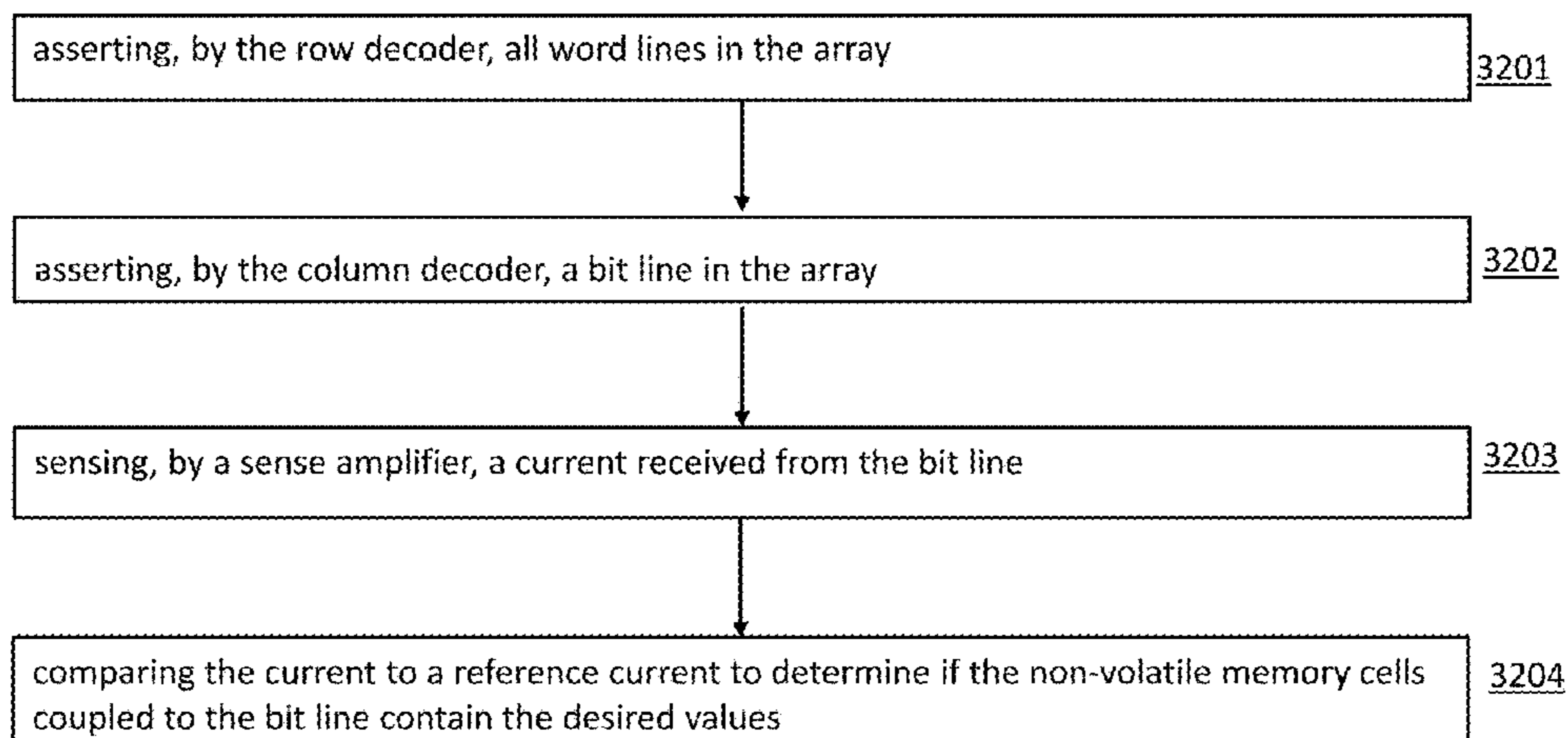
Bitline Neural Read 3101
