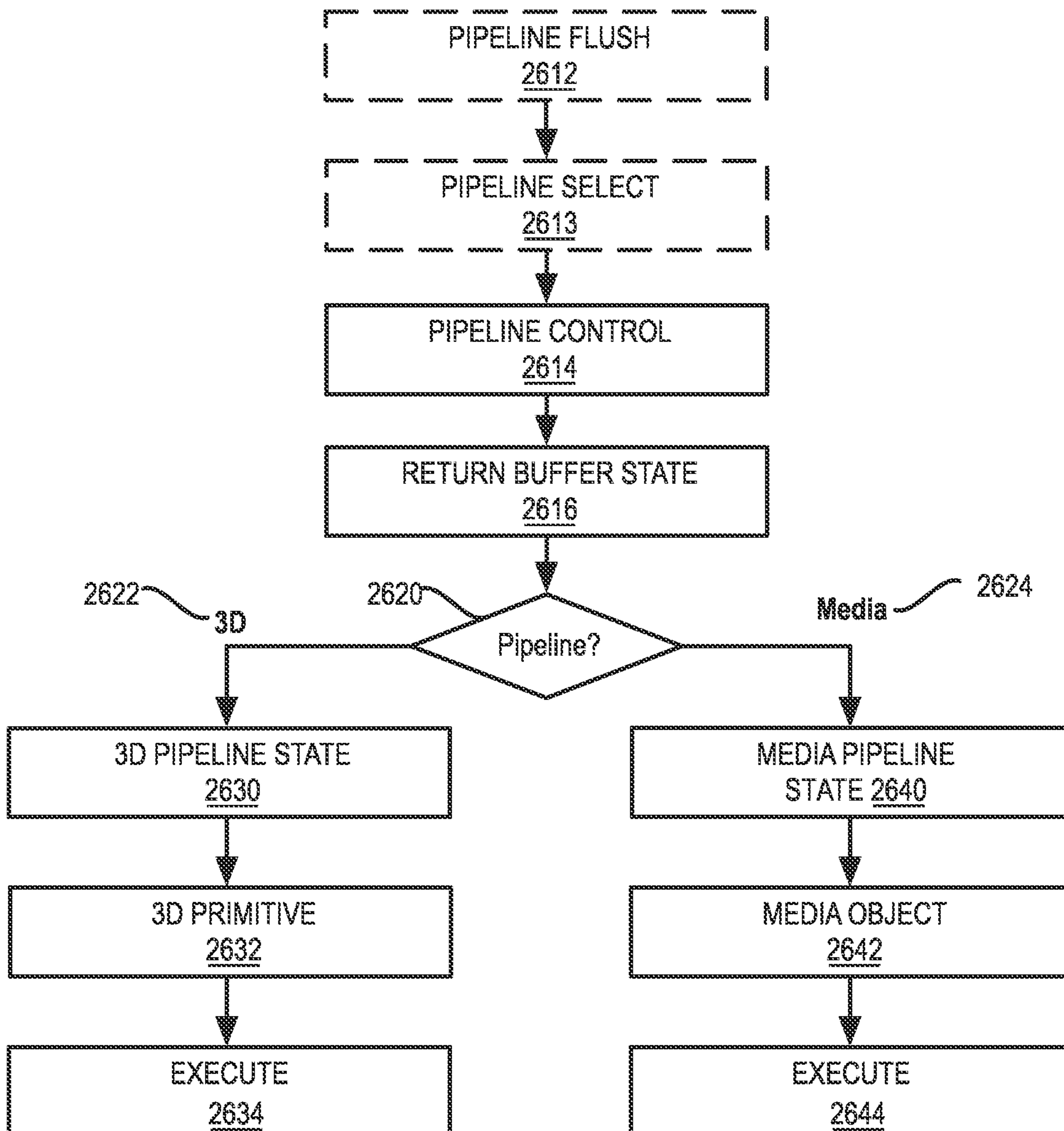
GRAPHICS PROCESSOR COMMAND SEQUENCE 2610
