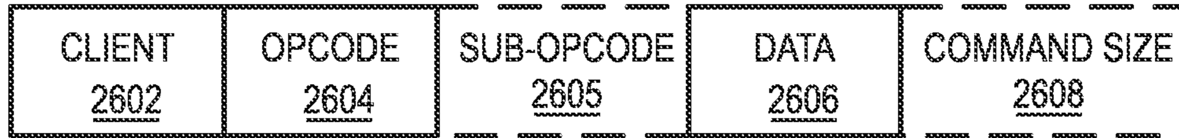
GRAPHICS PROCESSOR COMMAND FORMAT 2600
