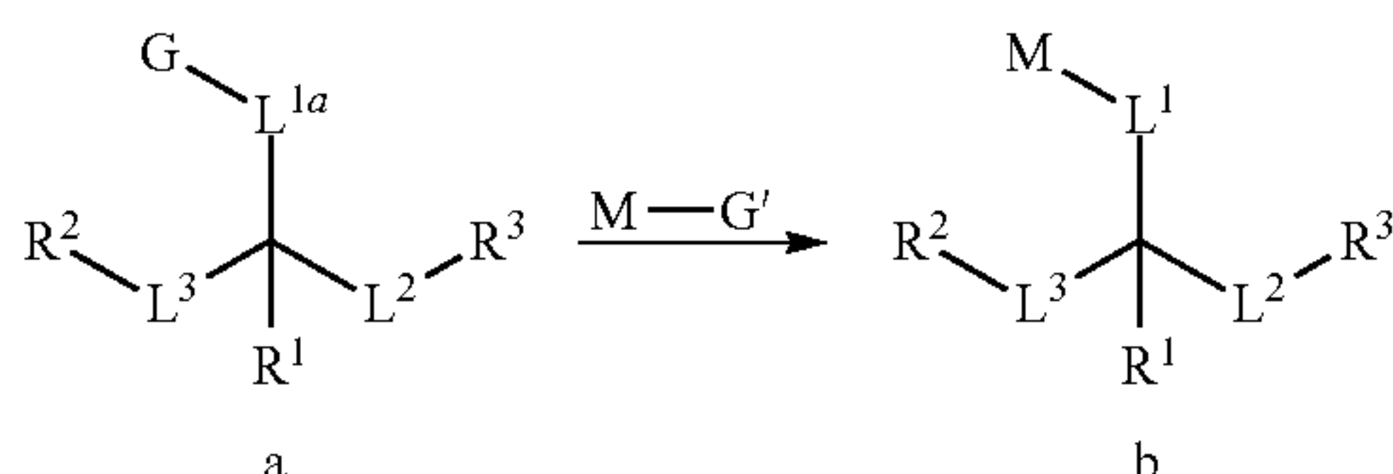
Reaction Scheme II
