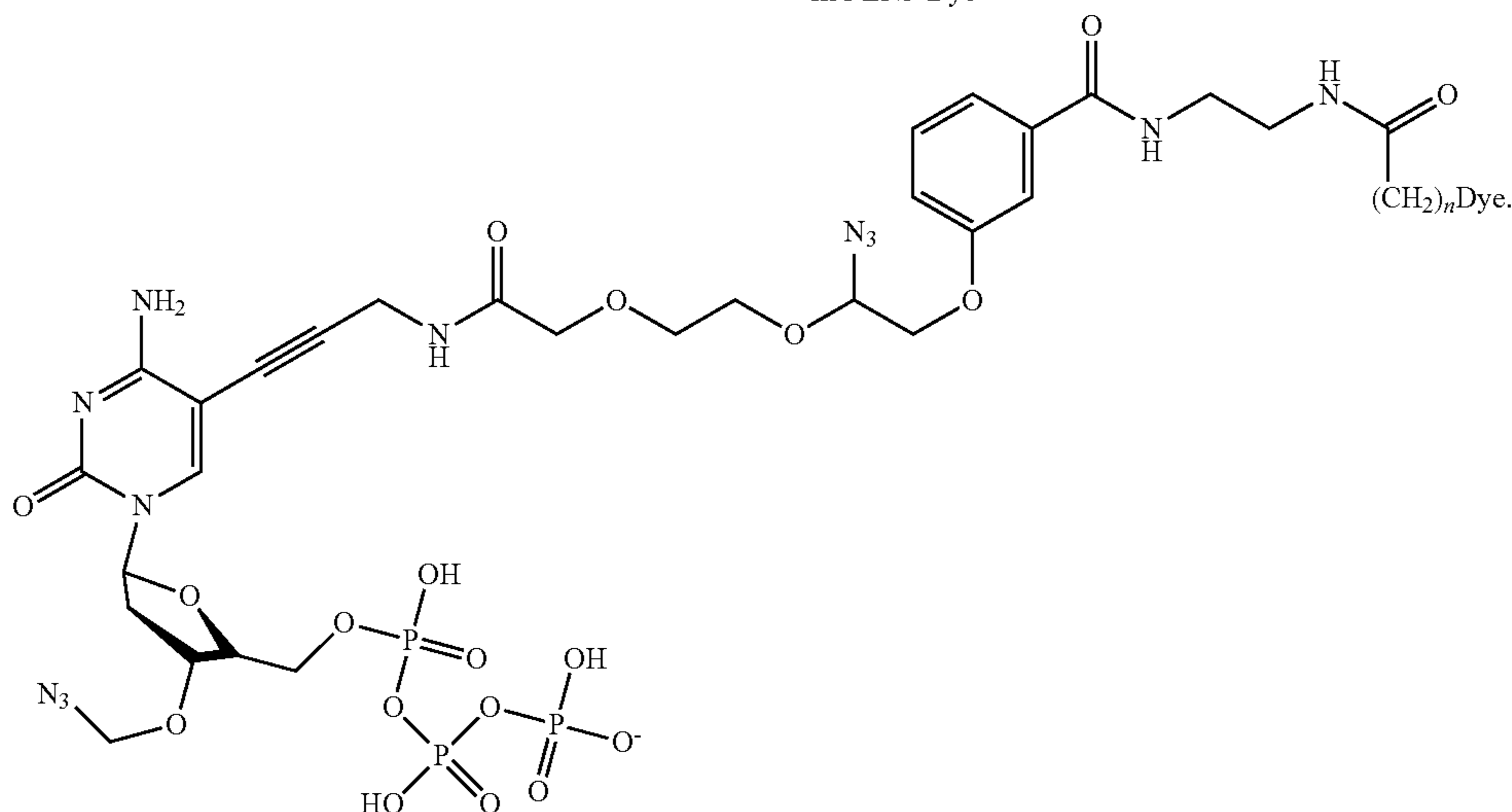
ffC-LN3-Dye
