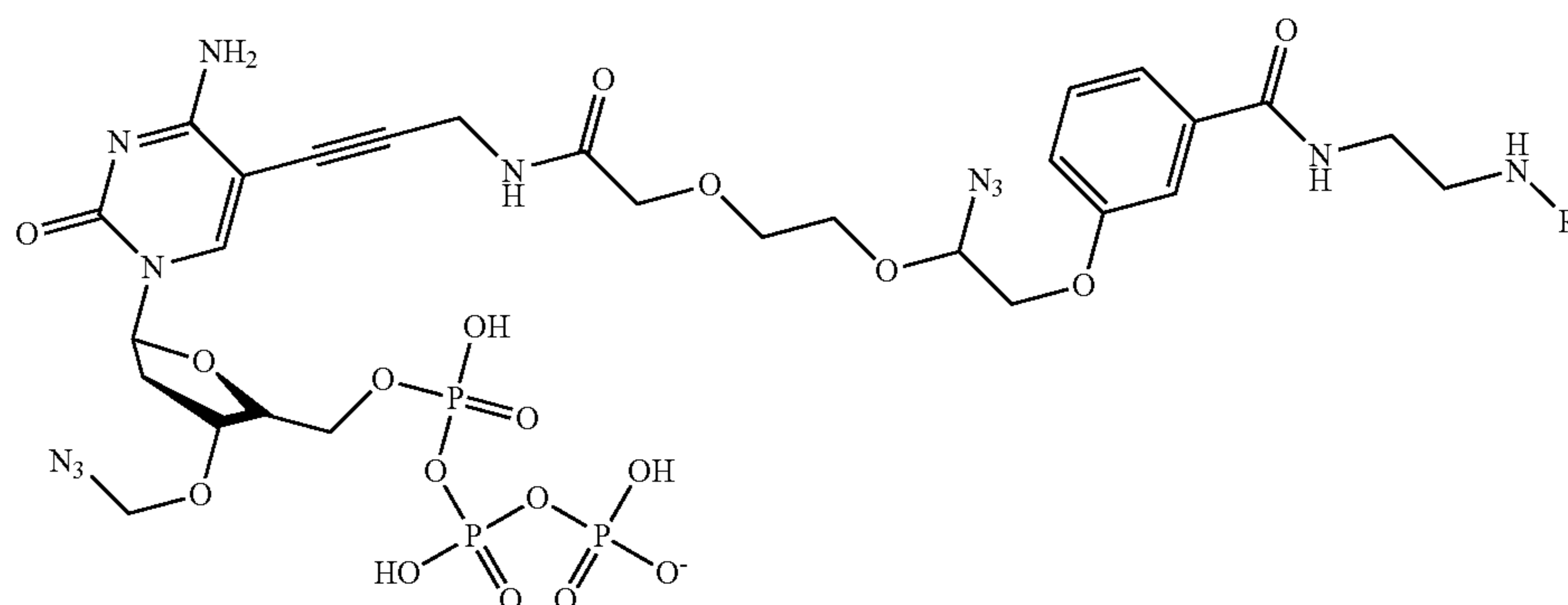
ffC-LN3-Dye
