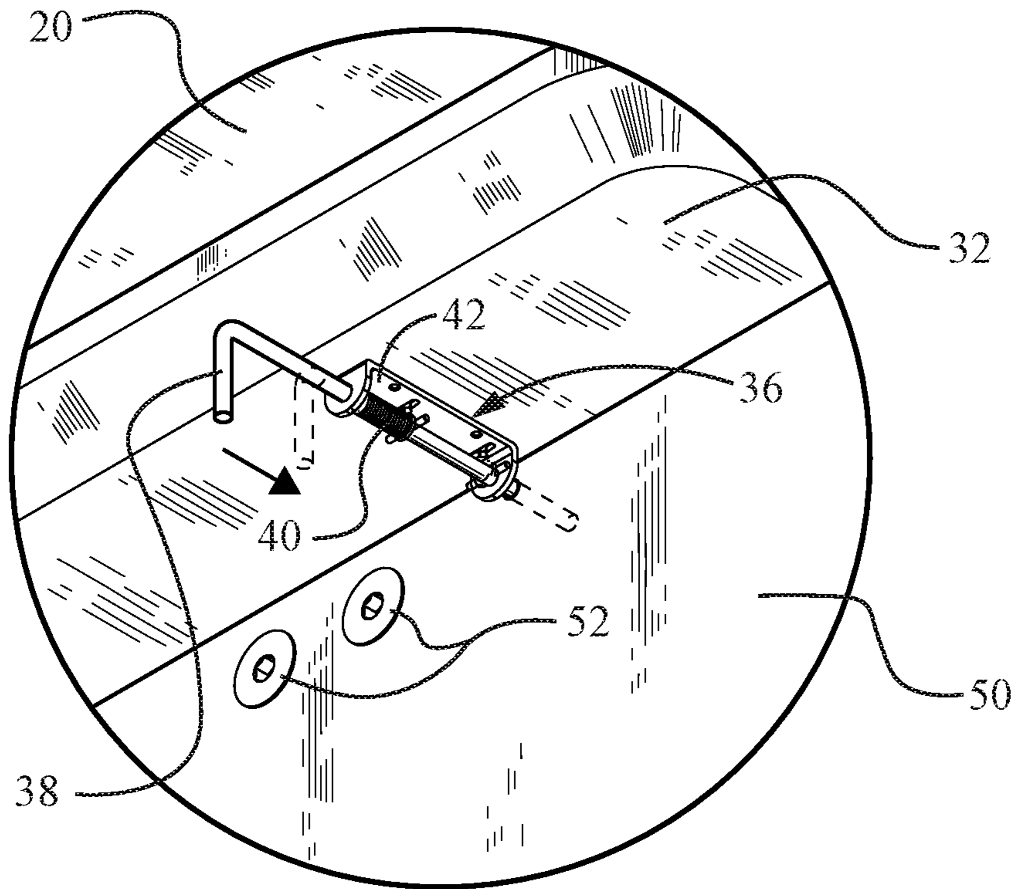
Detail A FIG. 6
