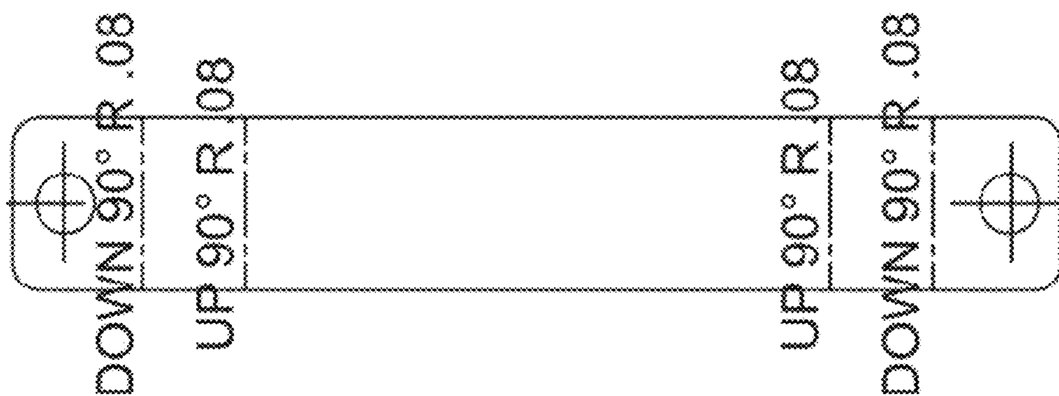
FLAT PATTERN
