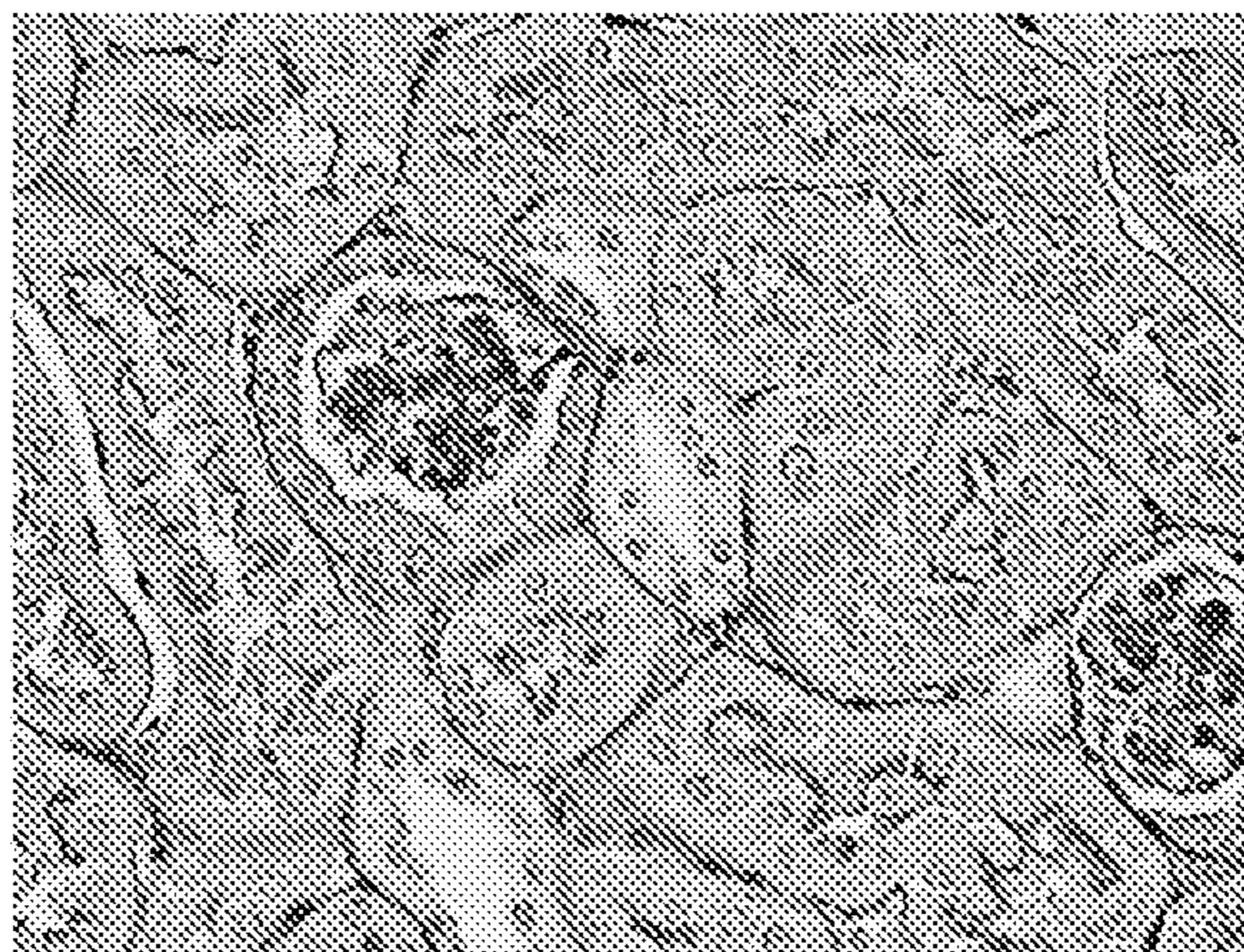
Compound 1
