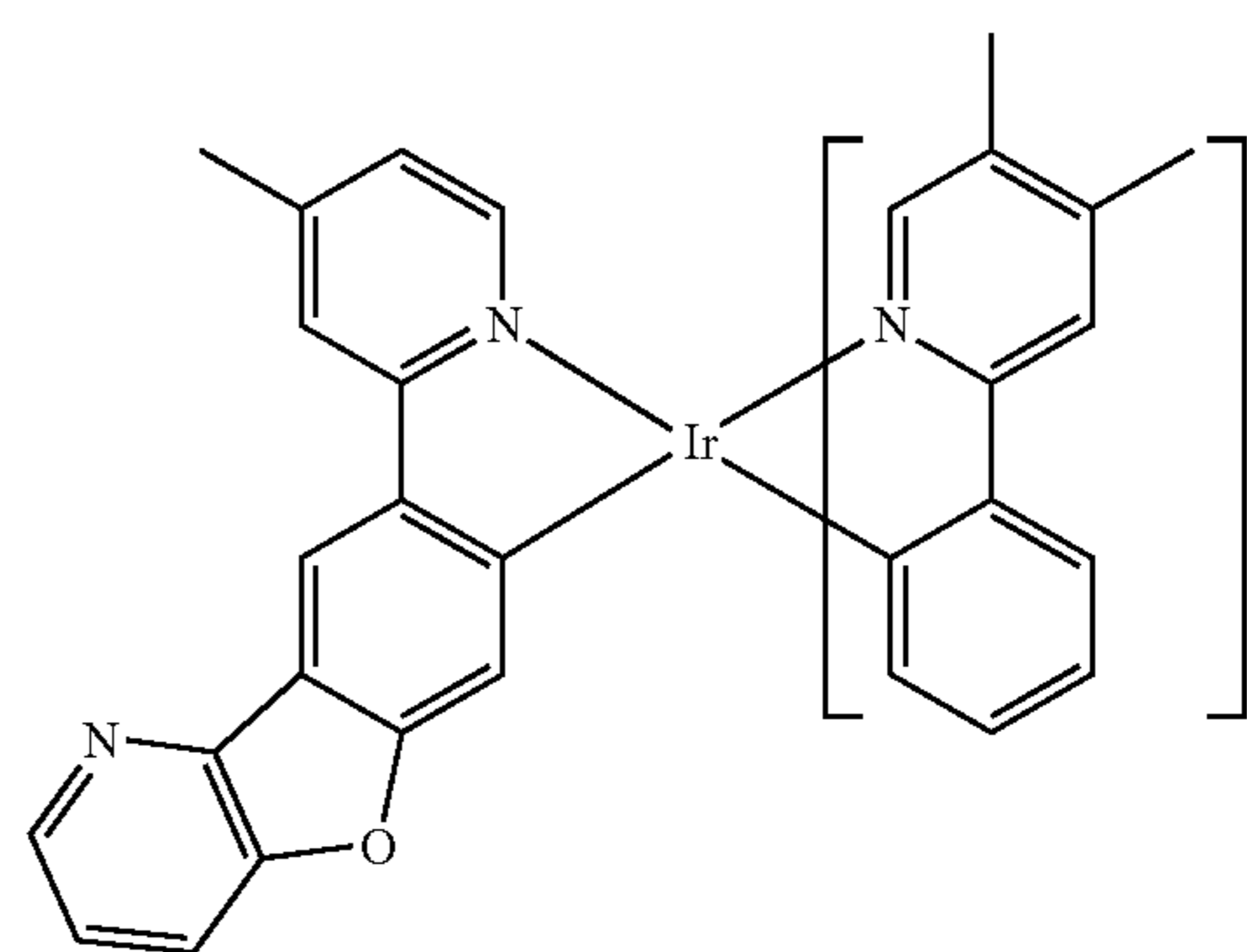
Compound 706
