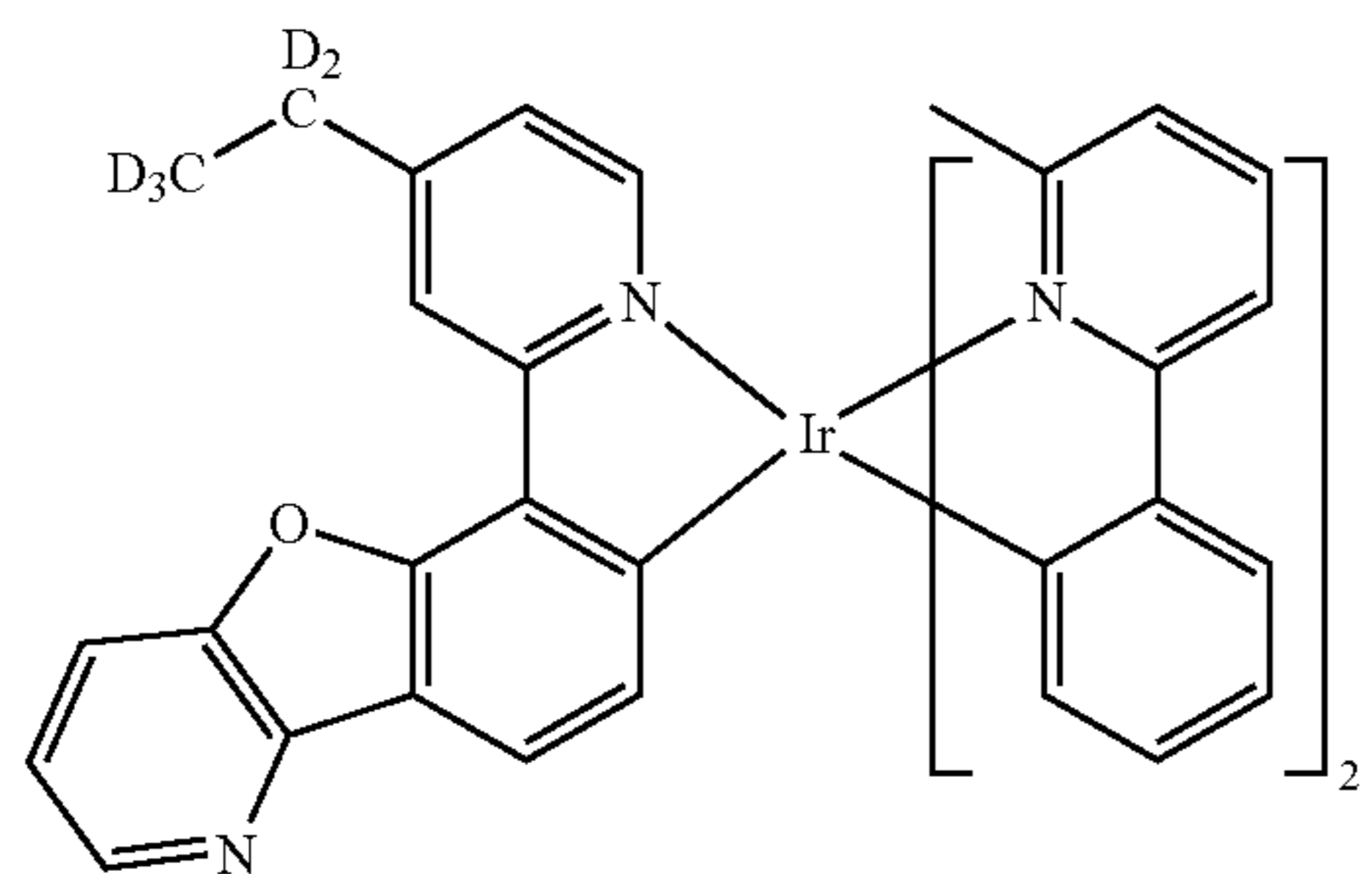
Compound 144
