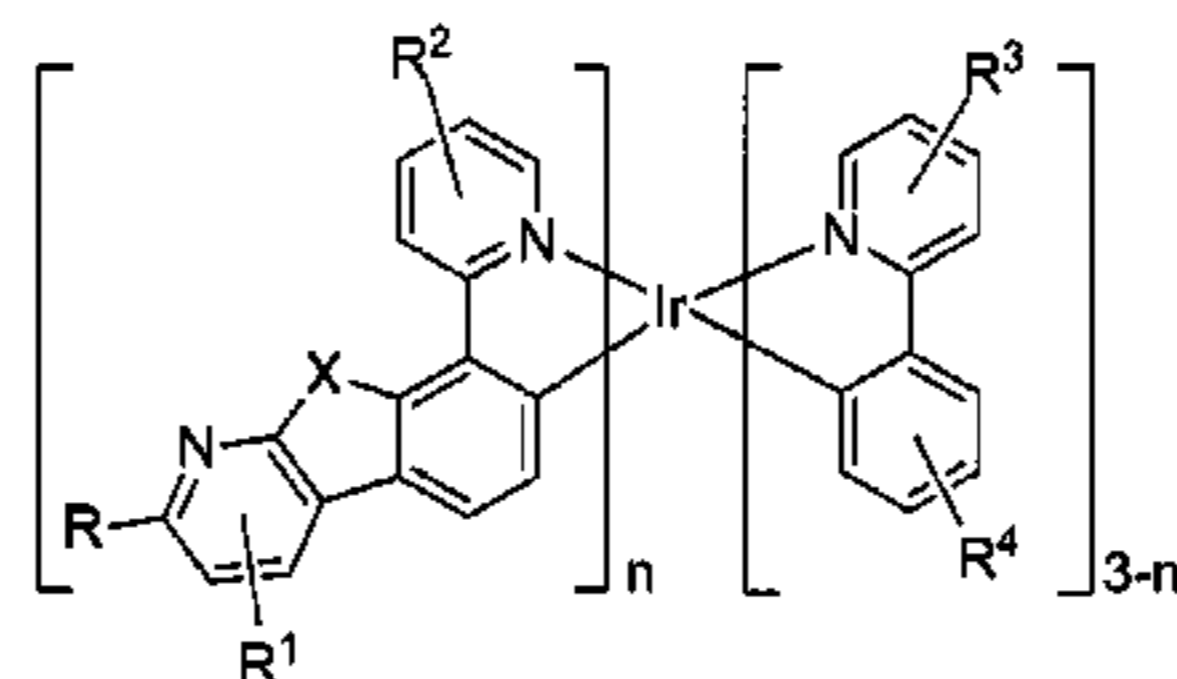
Formula III
