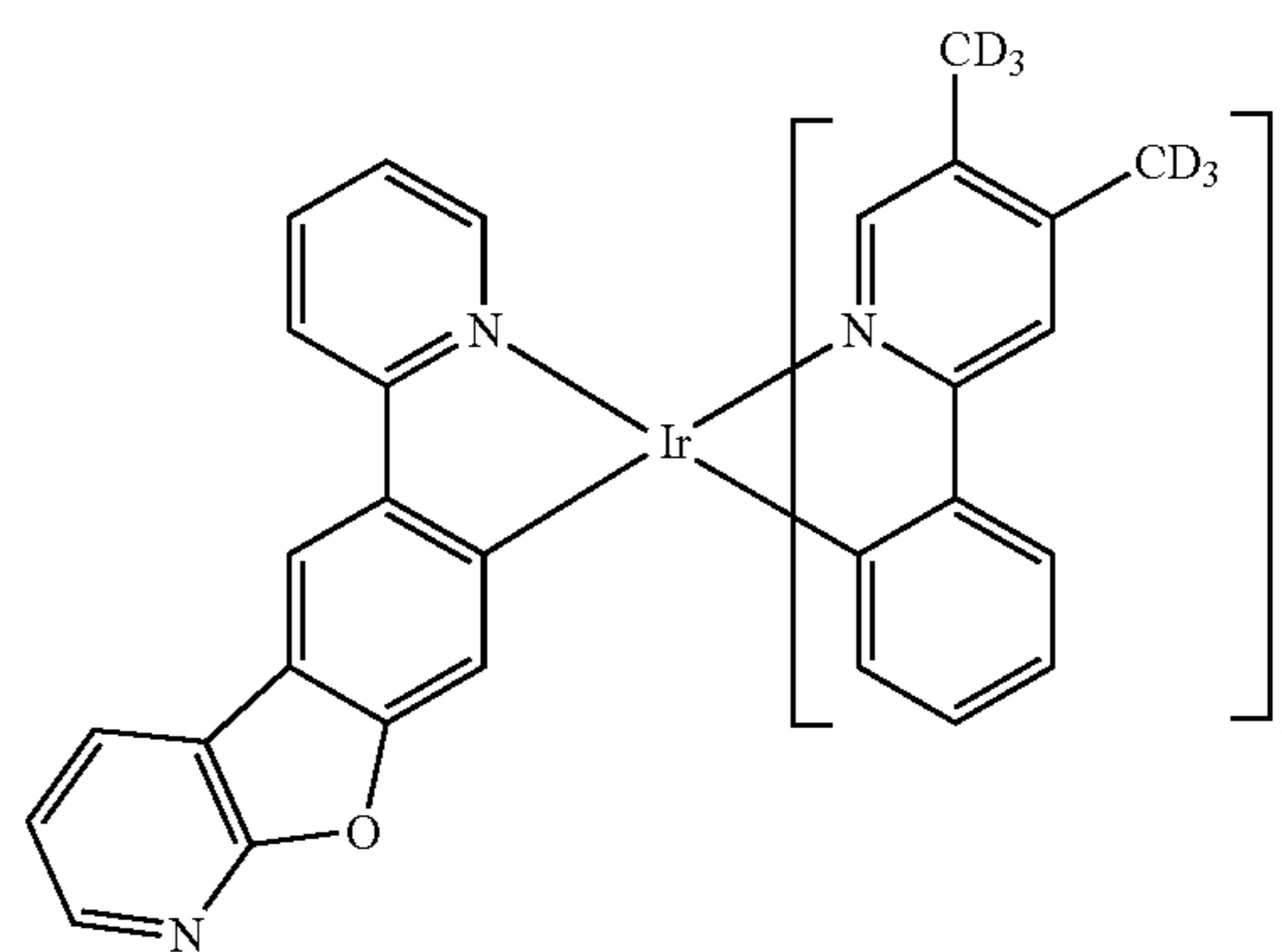
Compound 1649
