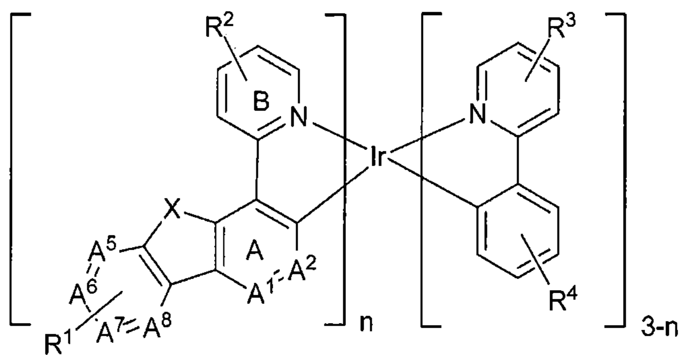
Formula II
