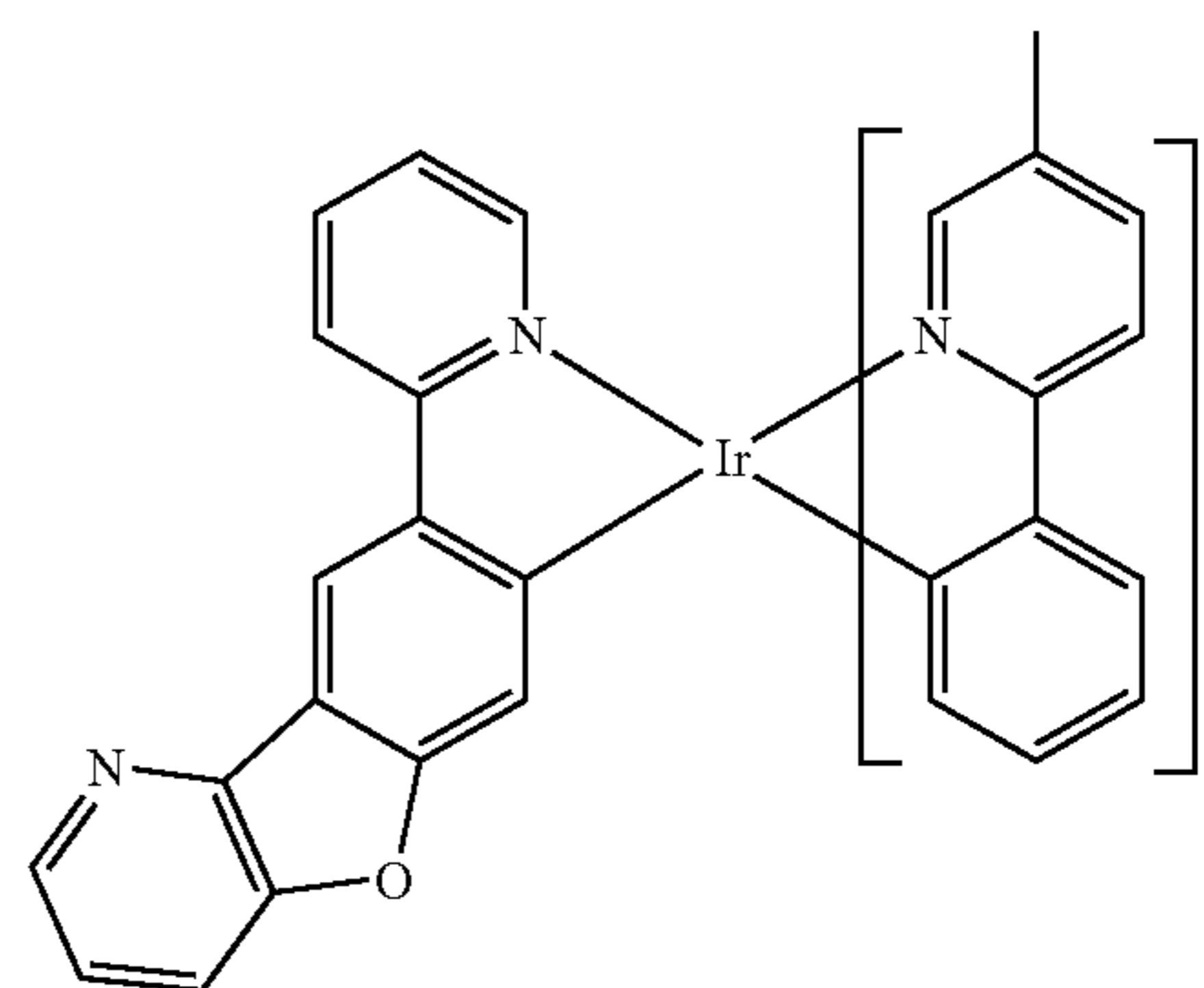
Compound 343
