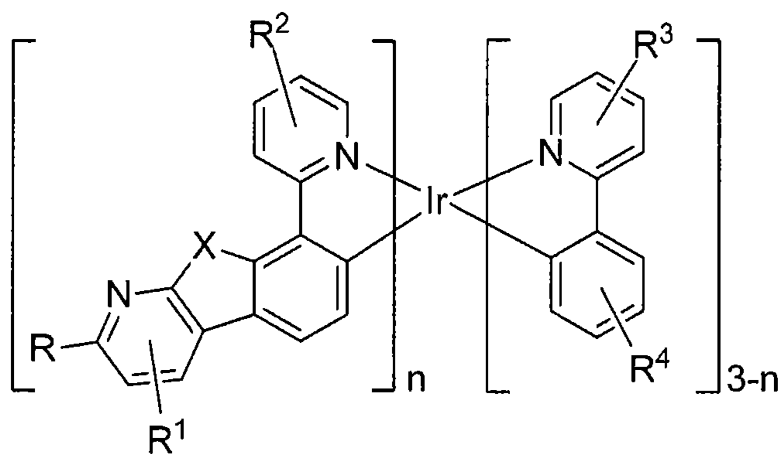
Formula III
