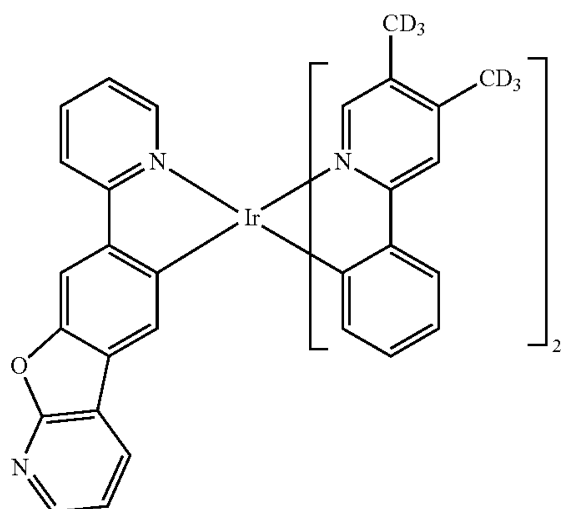
Compound 1664
