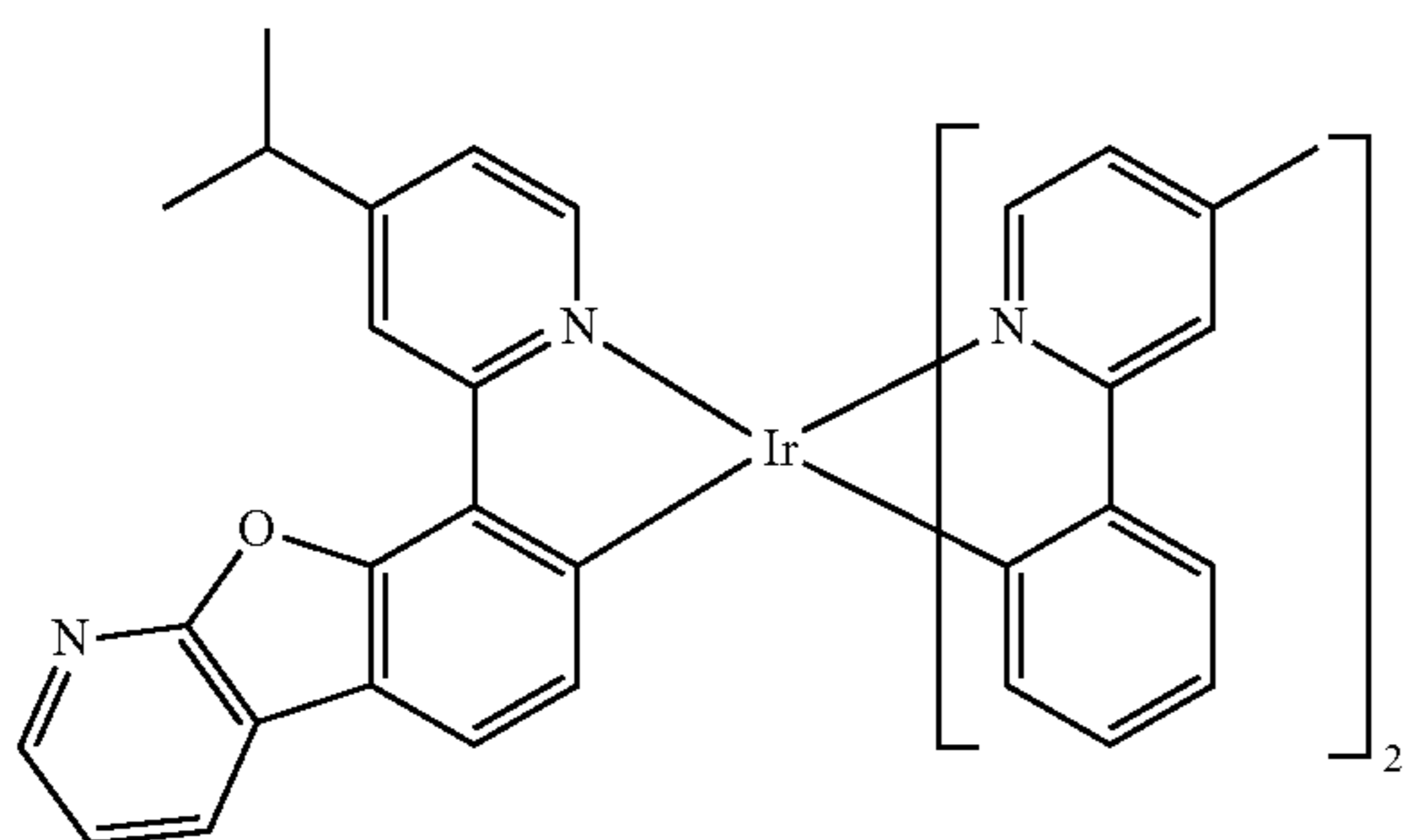
Compound 272
