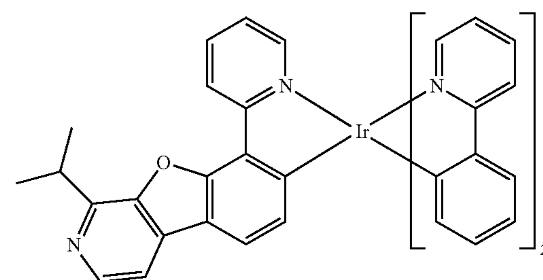
Compound 81
