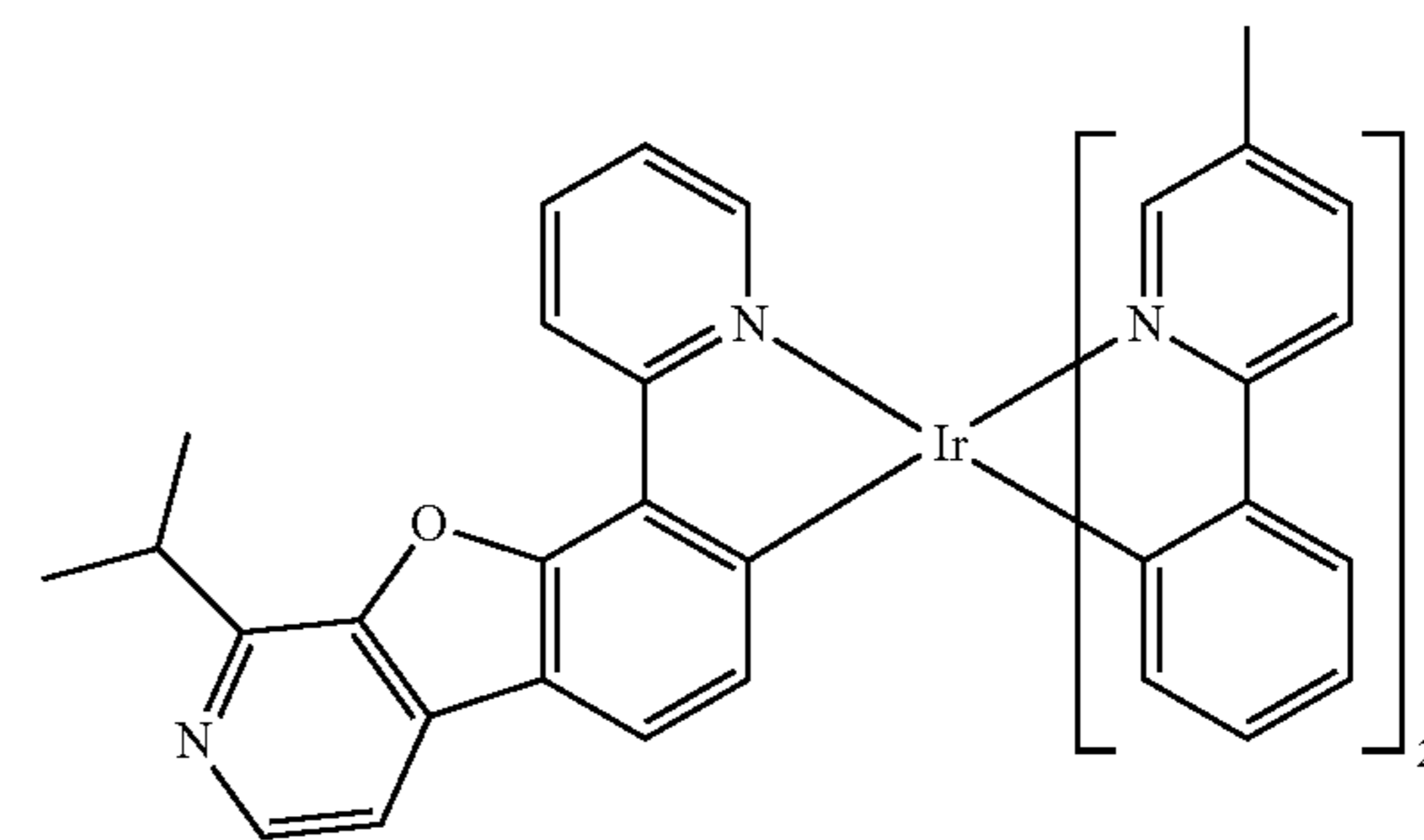
Compound 319
