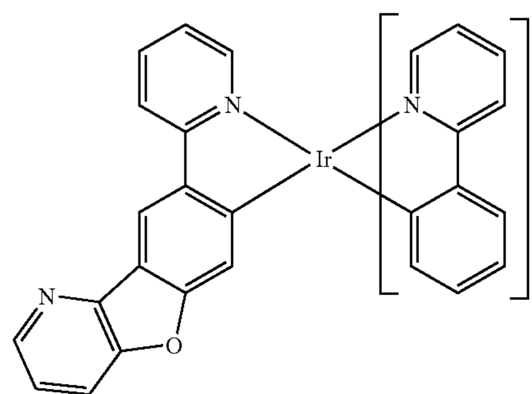
Compound 105
