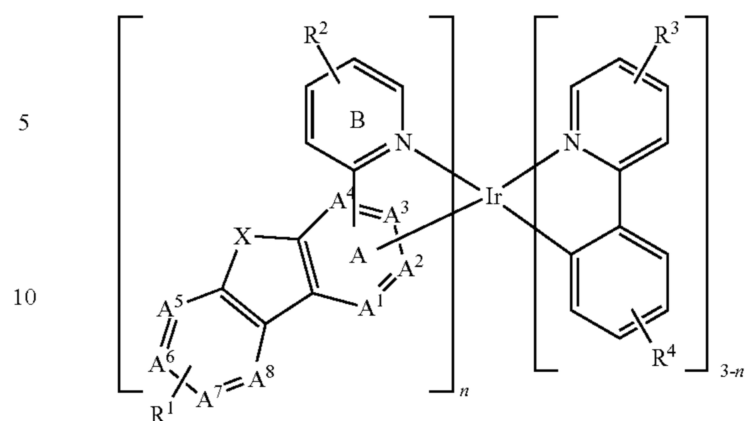
Compound 1304
