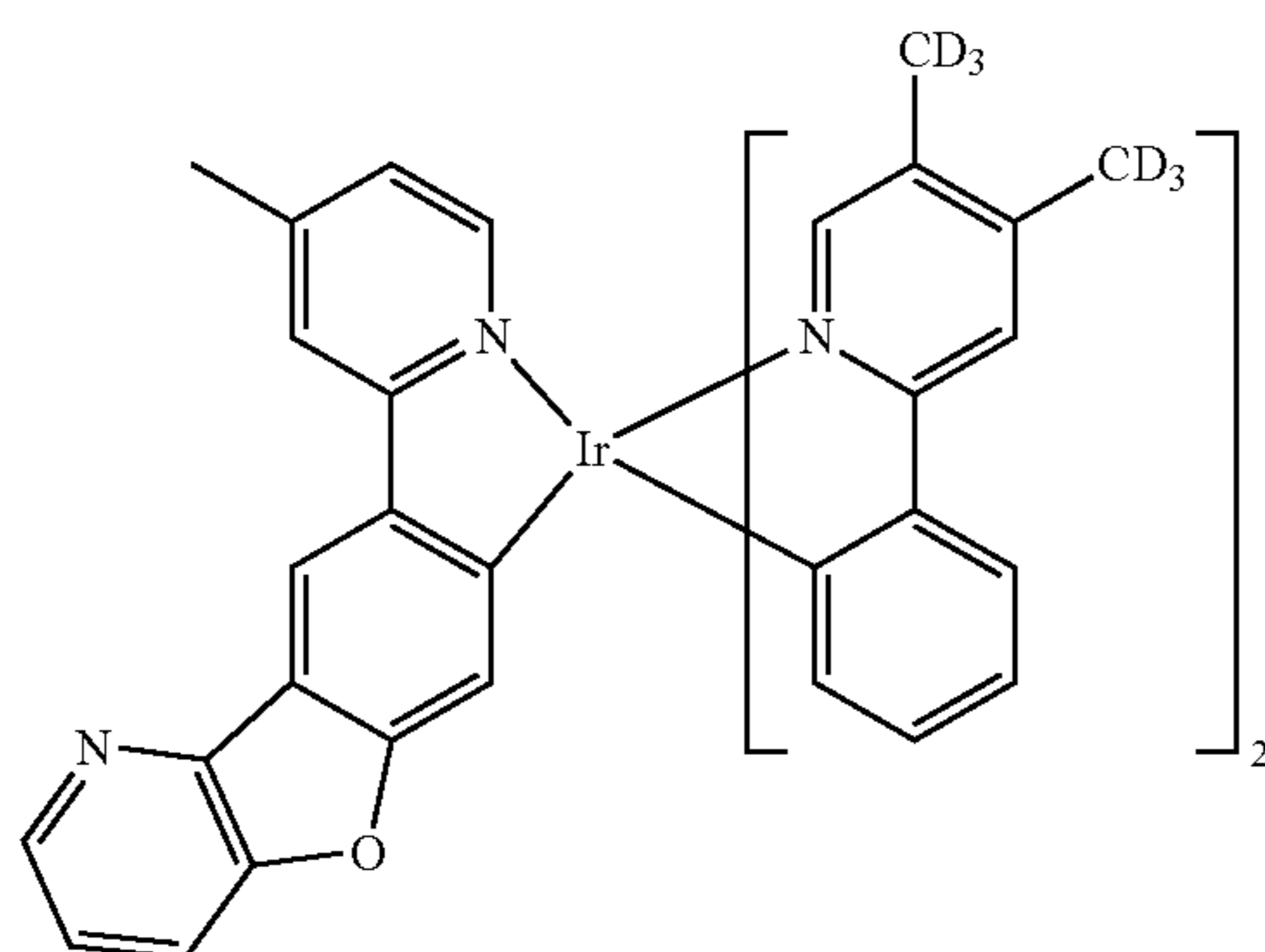
Compound 2134
