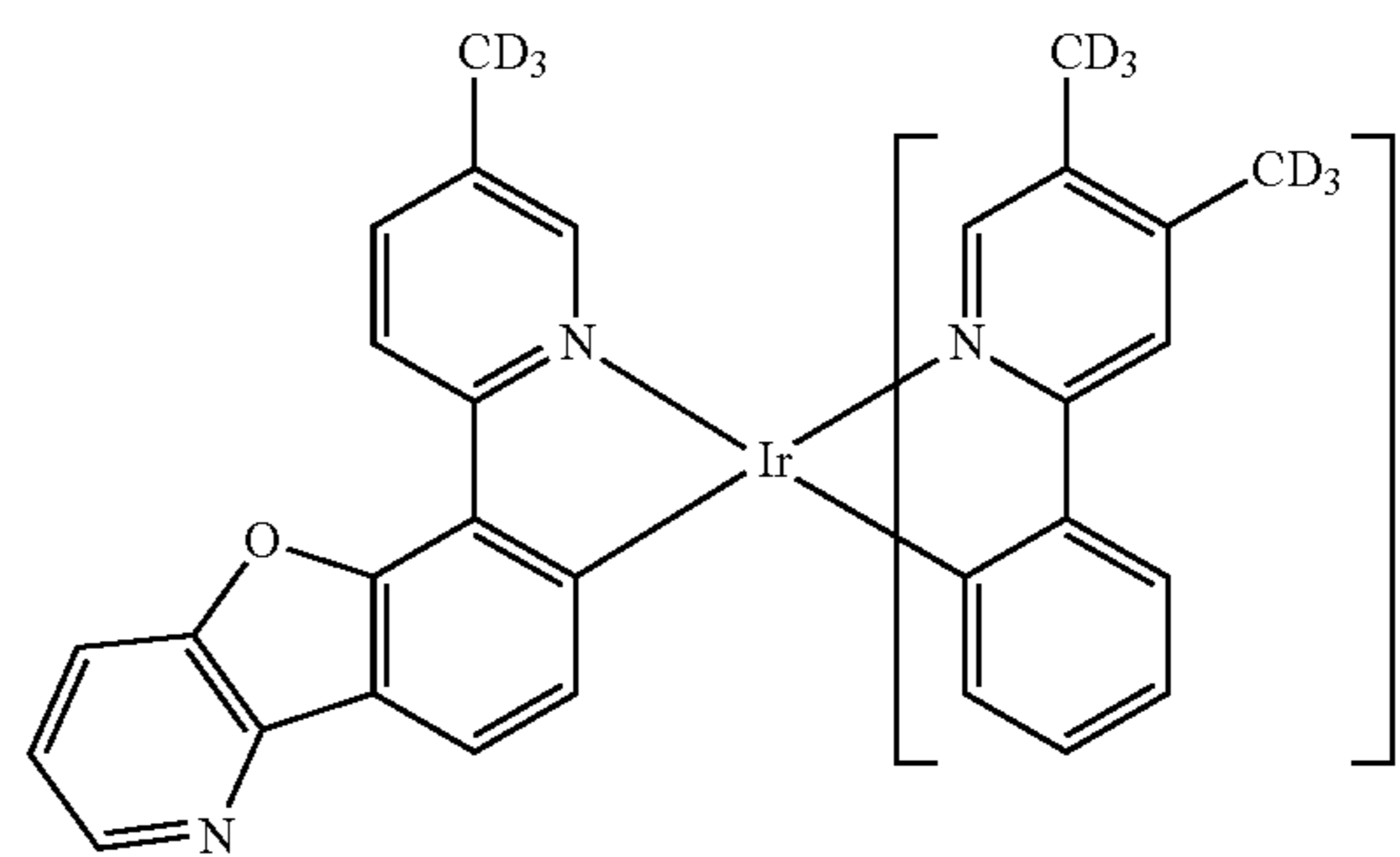
Compound 2072
