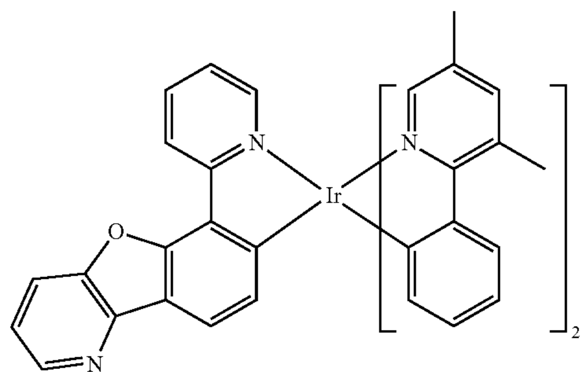
Compound 715
