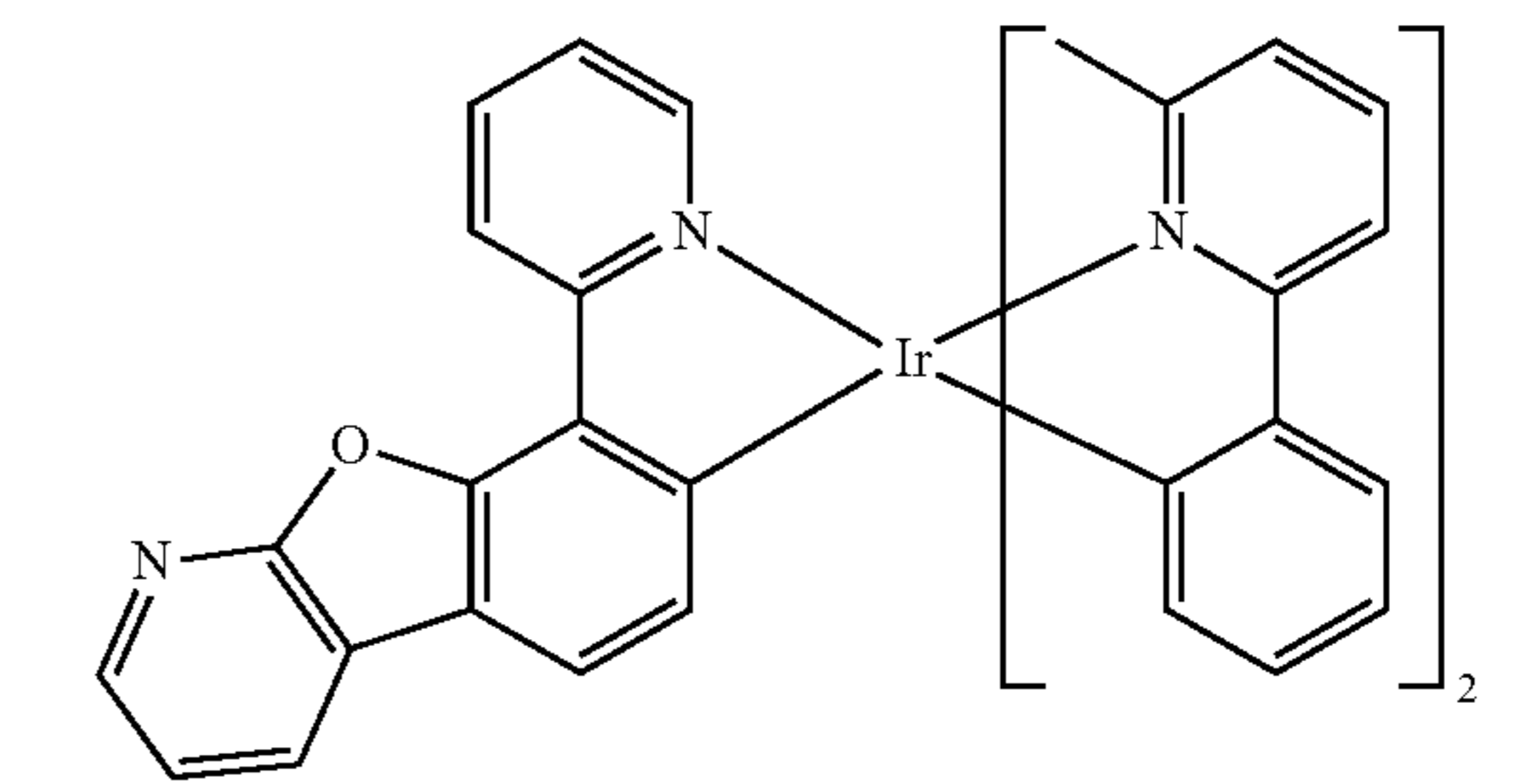
Compound 123
