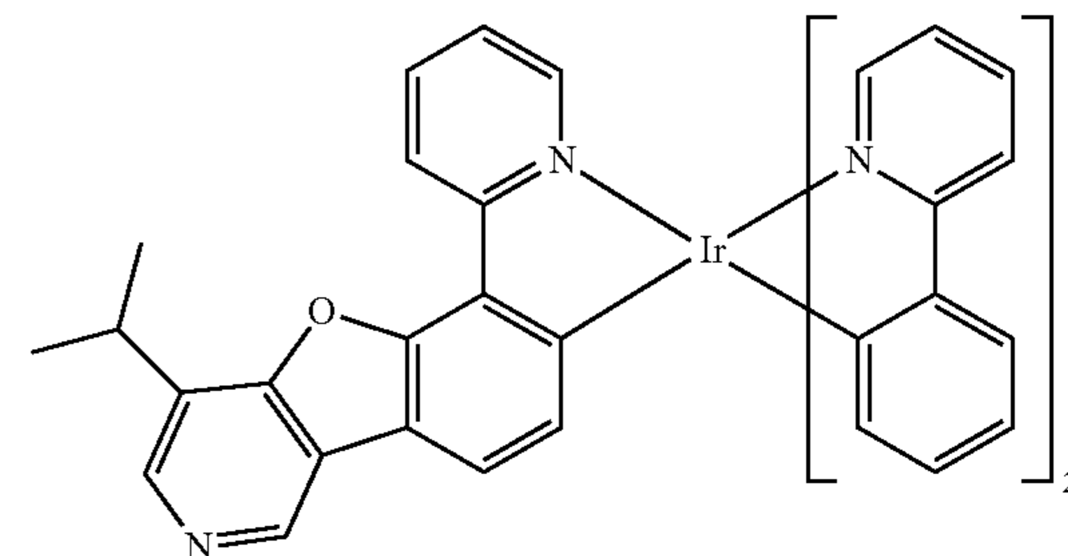
Compound 123
