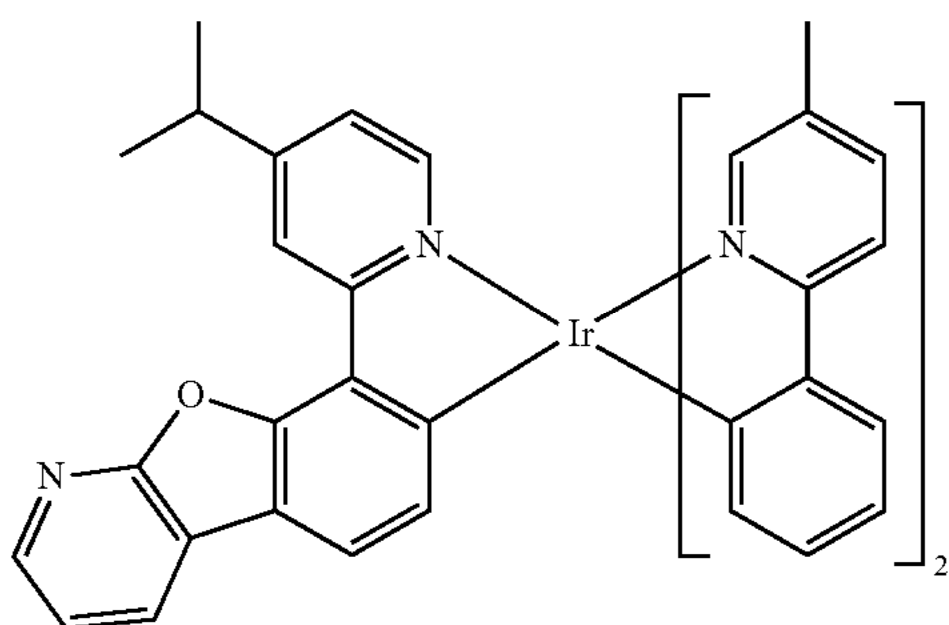
Compound 102
