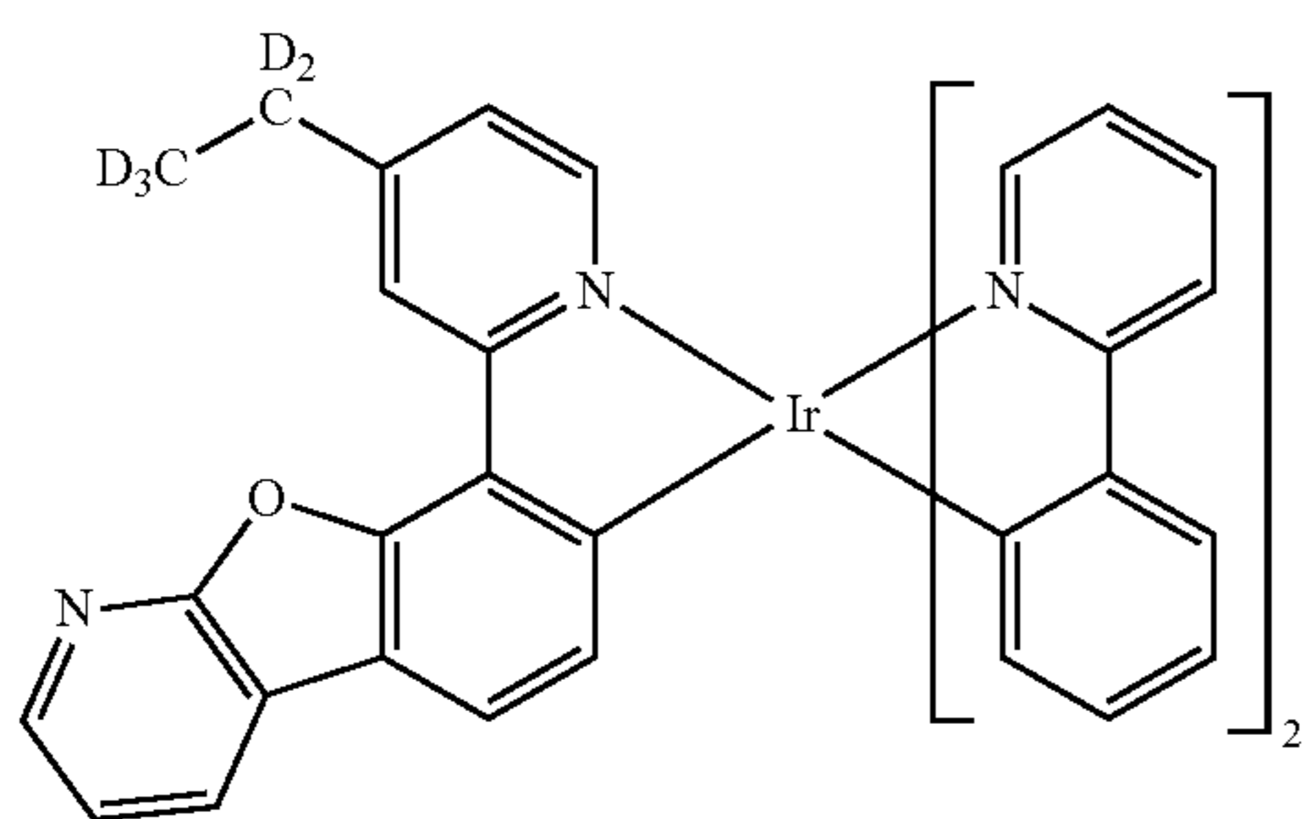
Compound 391
