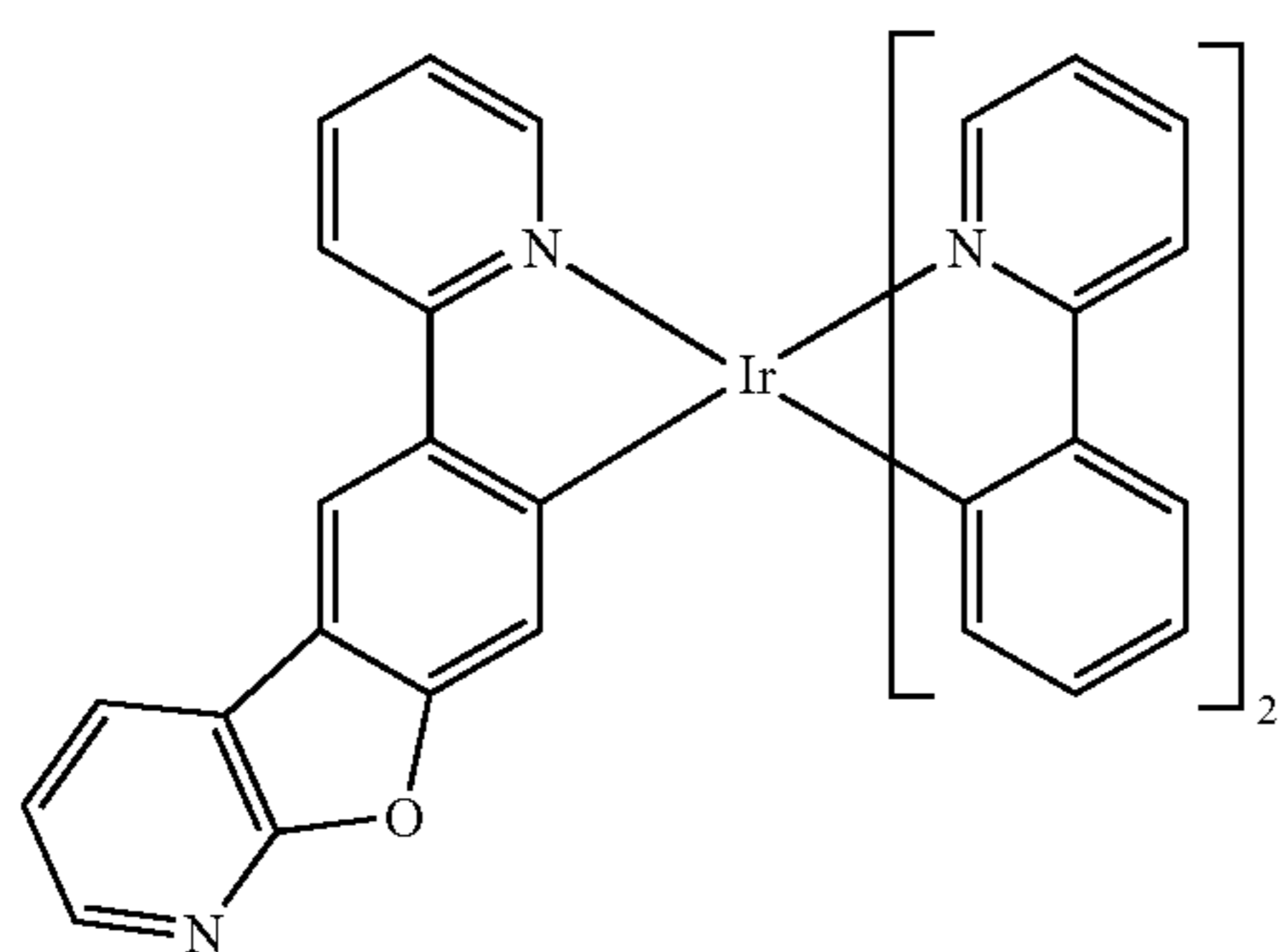
Compound 102
