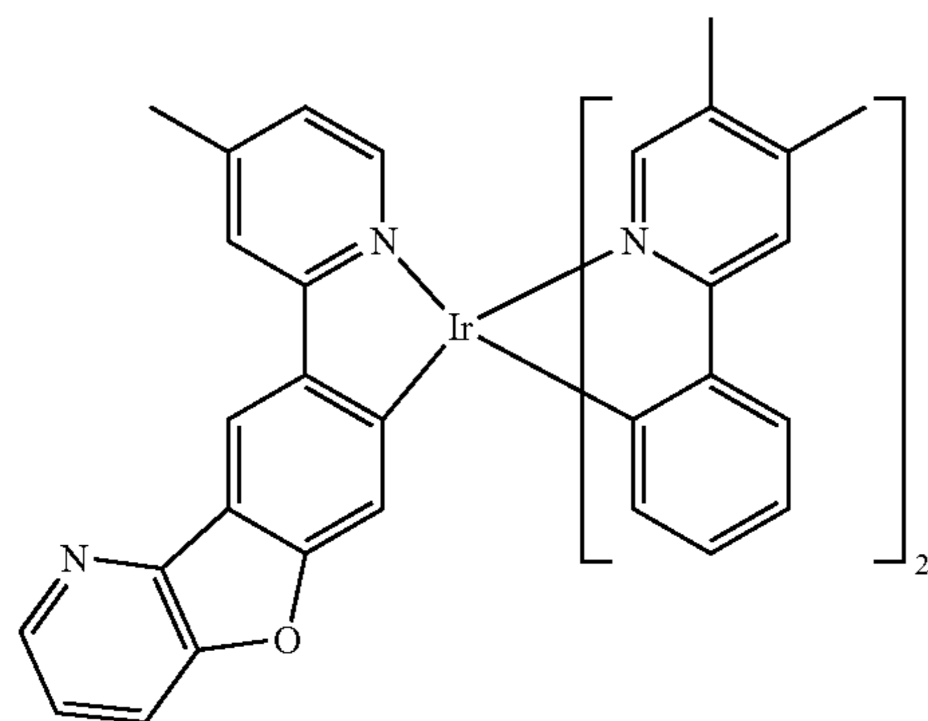
Compound 706
