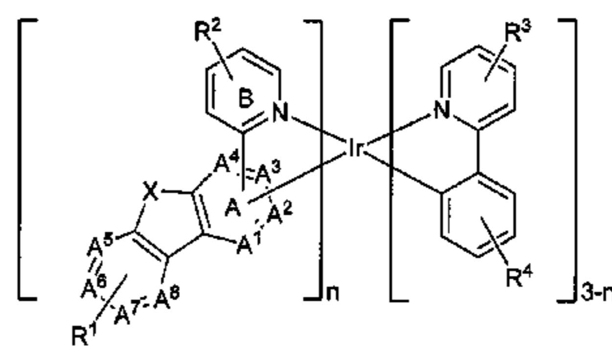
Formula I
