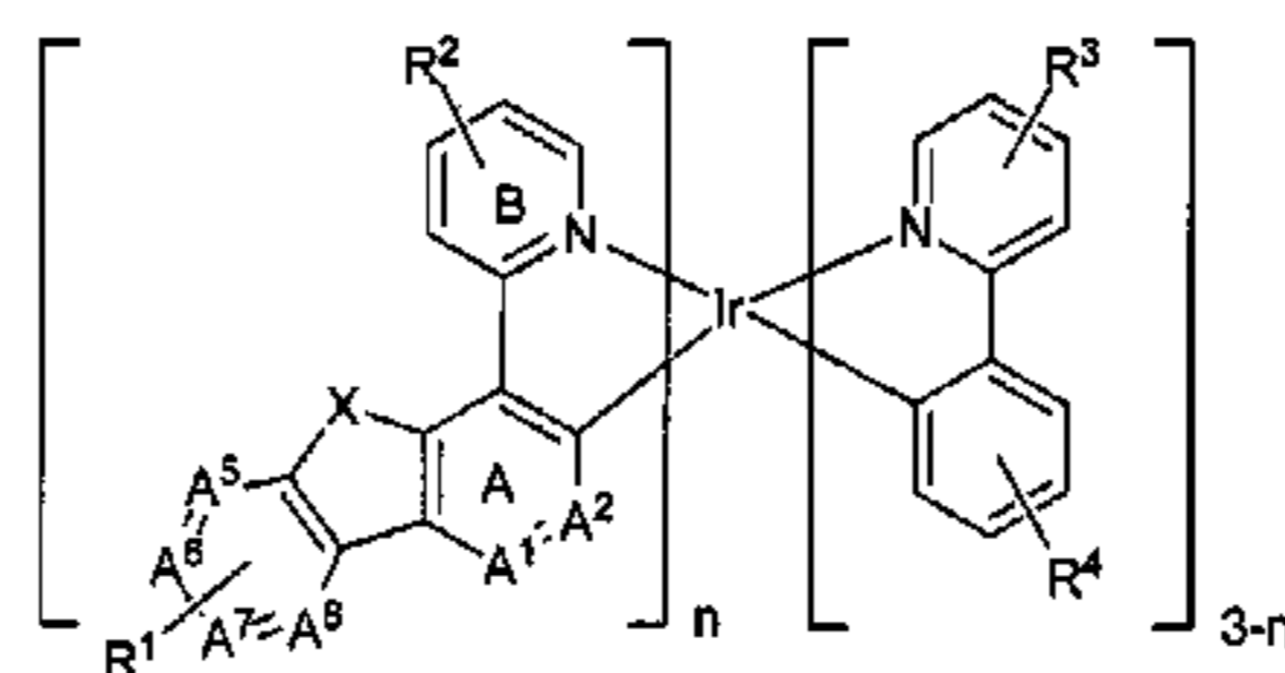
Formula II
