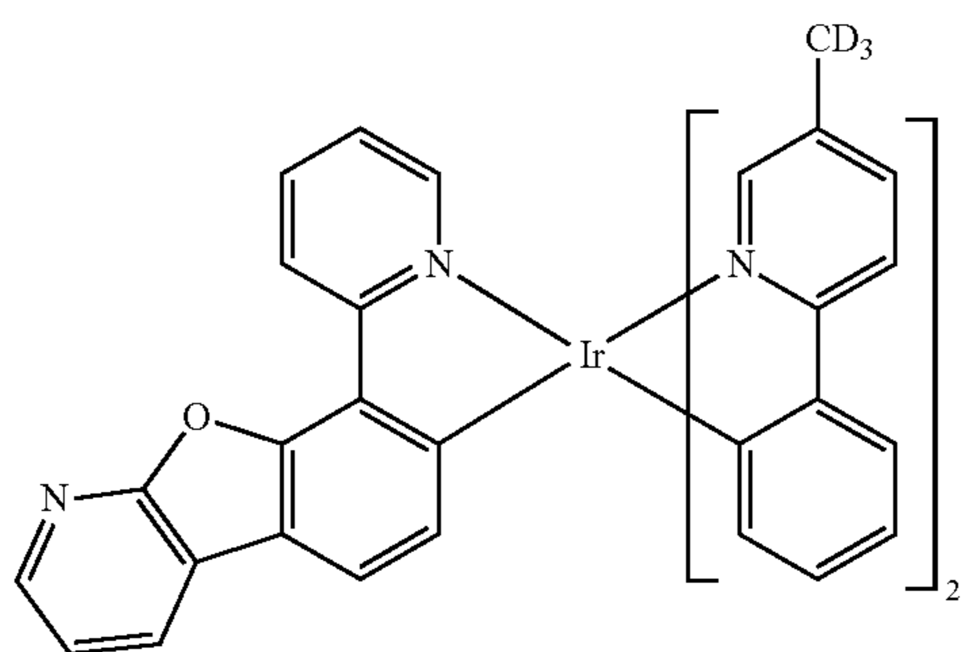
Compound 28
