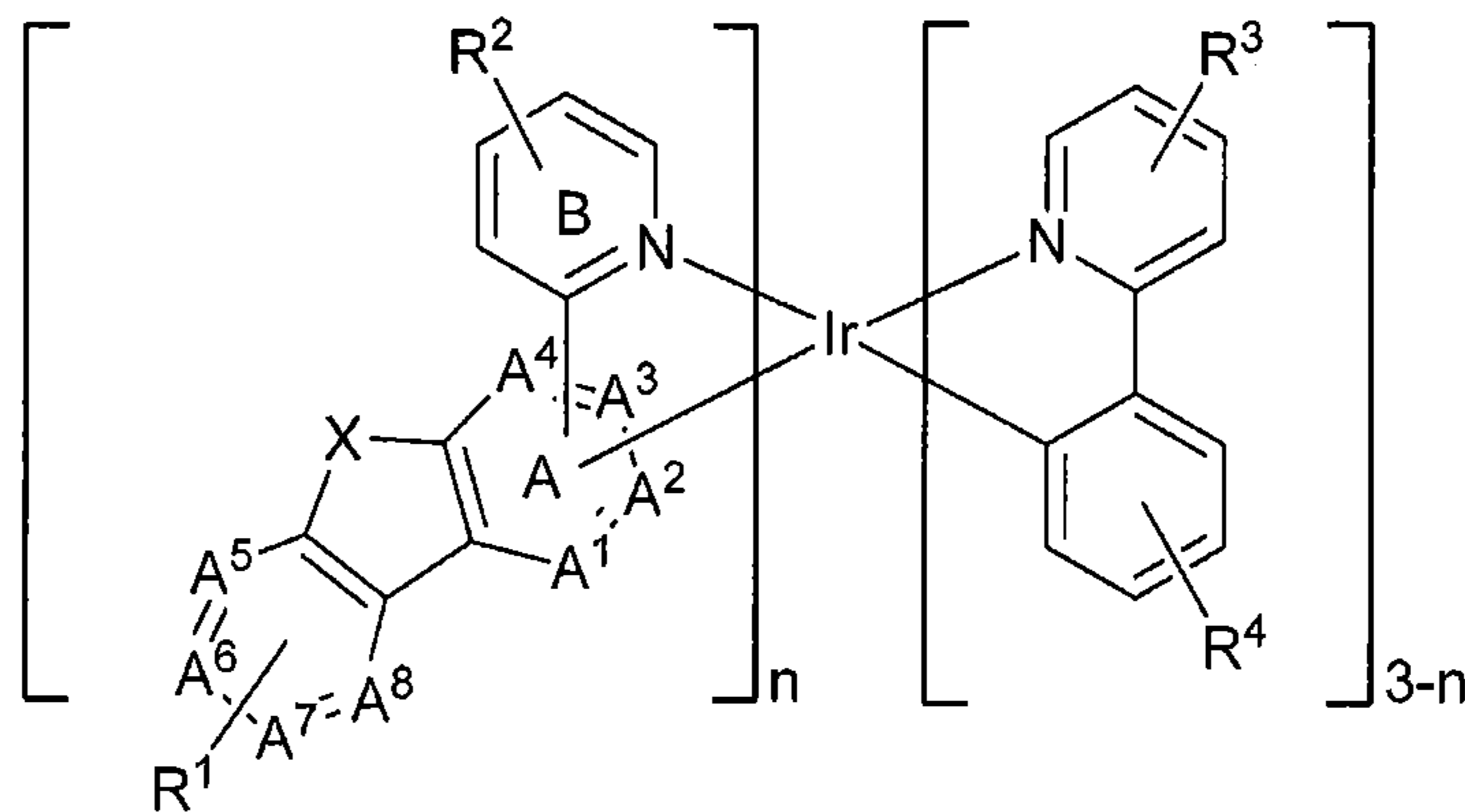
Formula I
