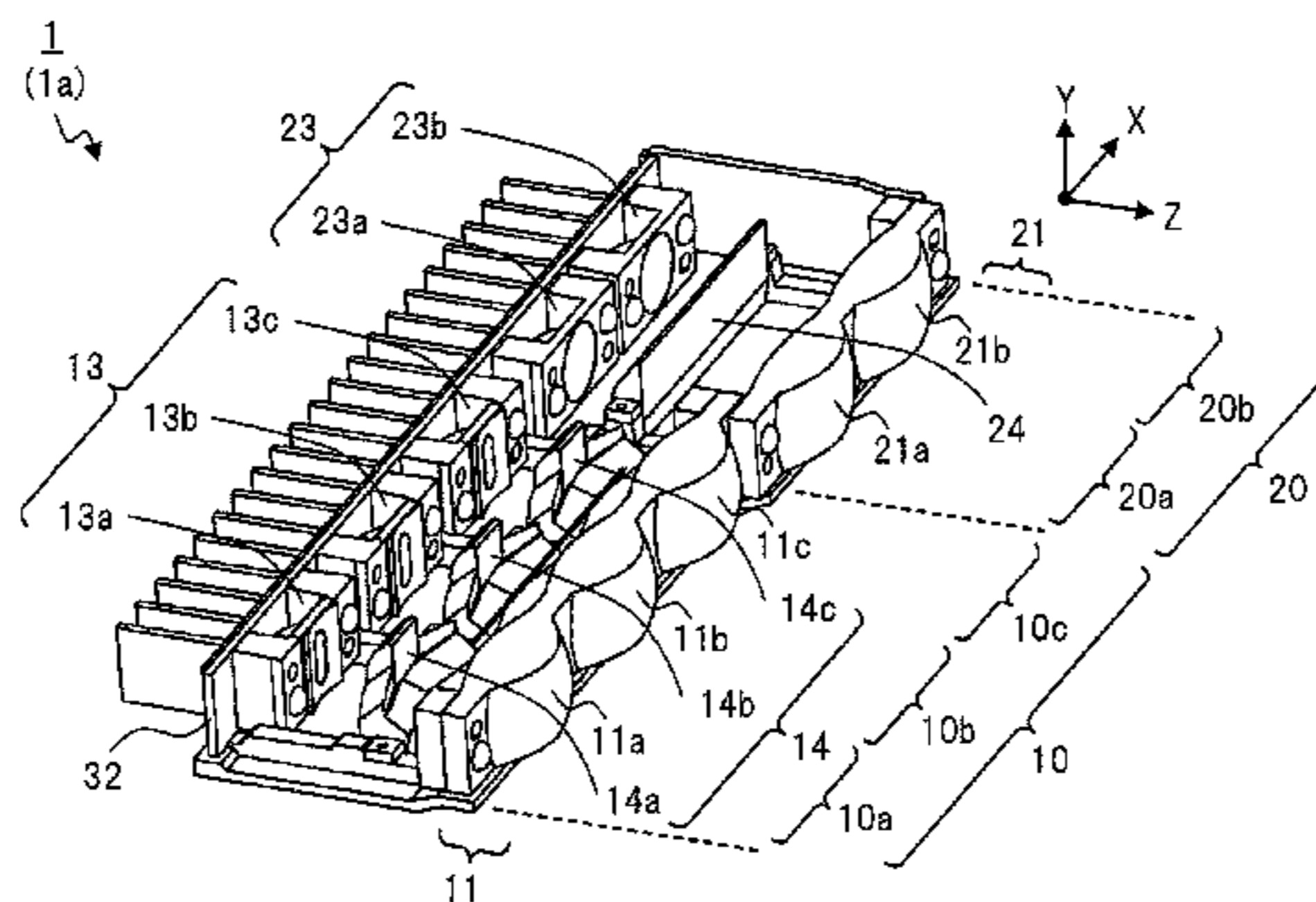
1 (1a): HEADLIGHT APPARATUS 10: LOW BEAM HEADLIGHT 20: HIGH BEAM HEADLIGHT 10a, 10b, 10c: LOW BEAM UNIT 20a, 20b: HIGH BEAM UNIT 11, 21: PROJECTOR LENS 13, 23: LED COLLIMATOR 14, 24: LIGHT GUIDE 32: LED SUBSTRATE
