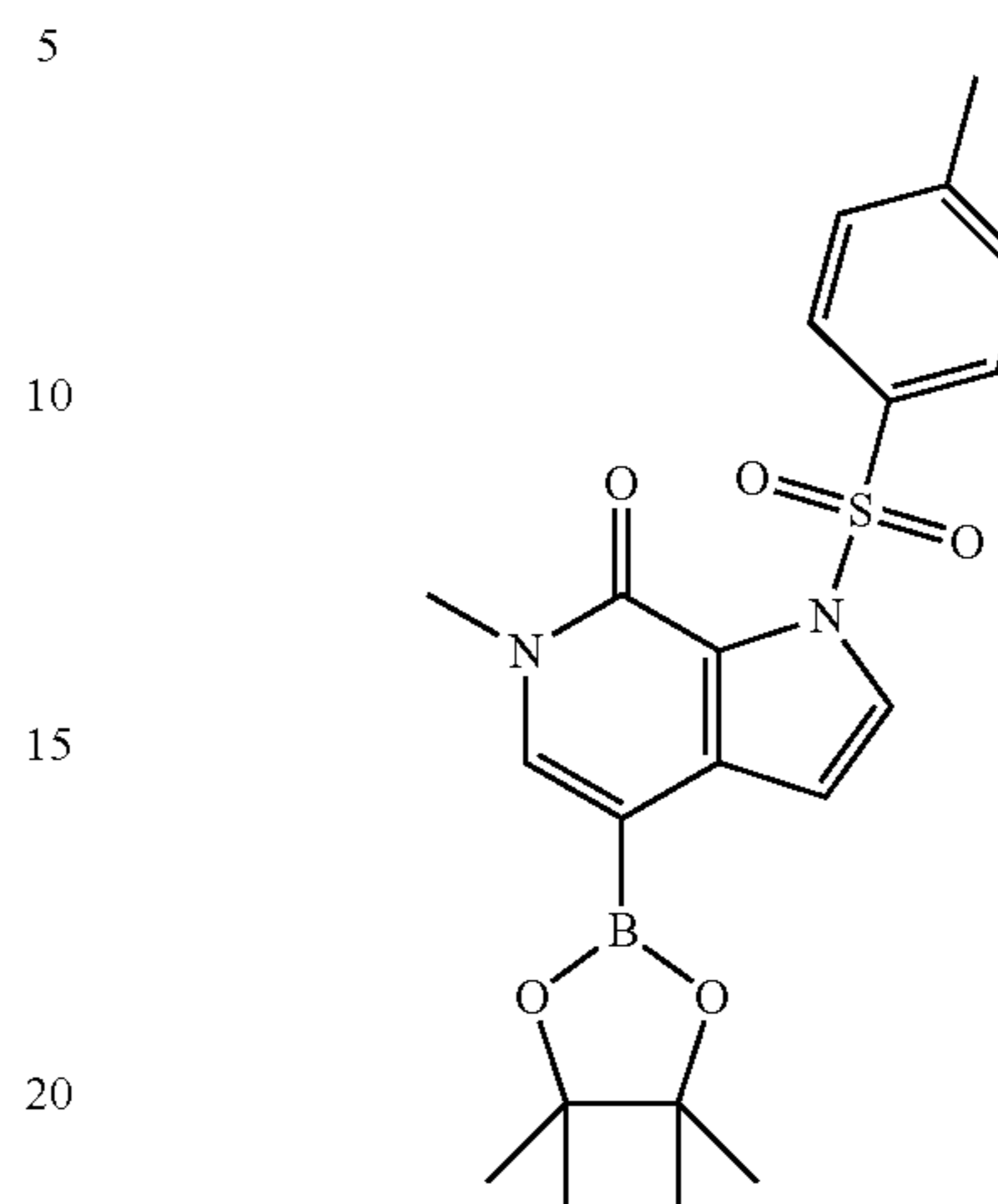
5 Compound 6
