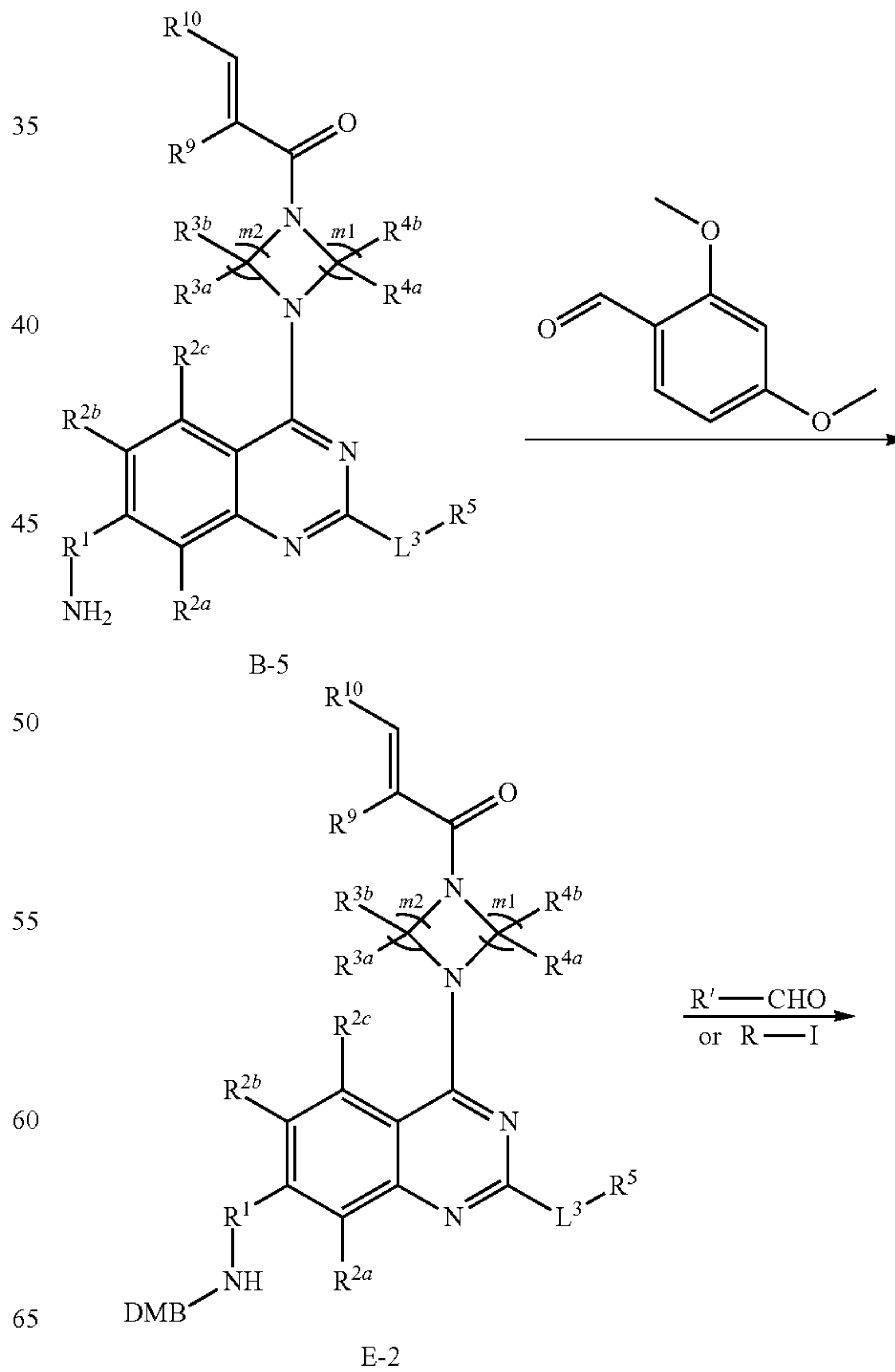
General Reaction Scheme 5
