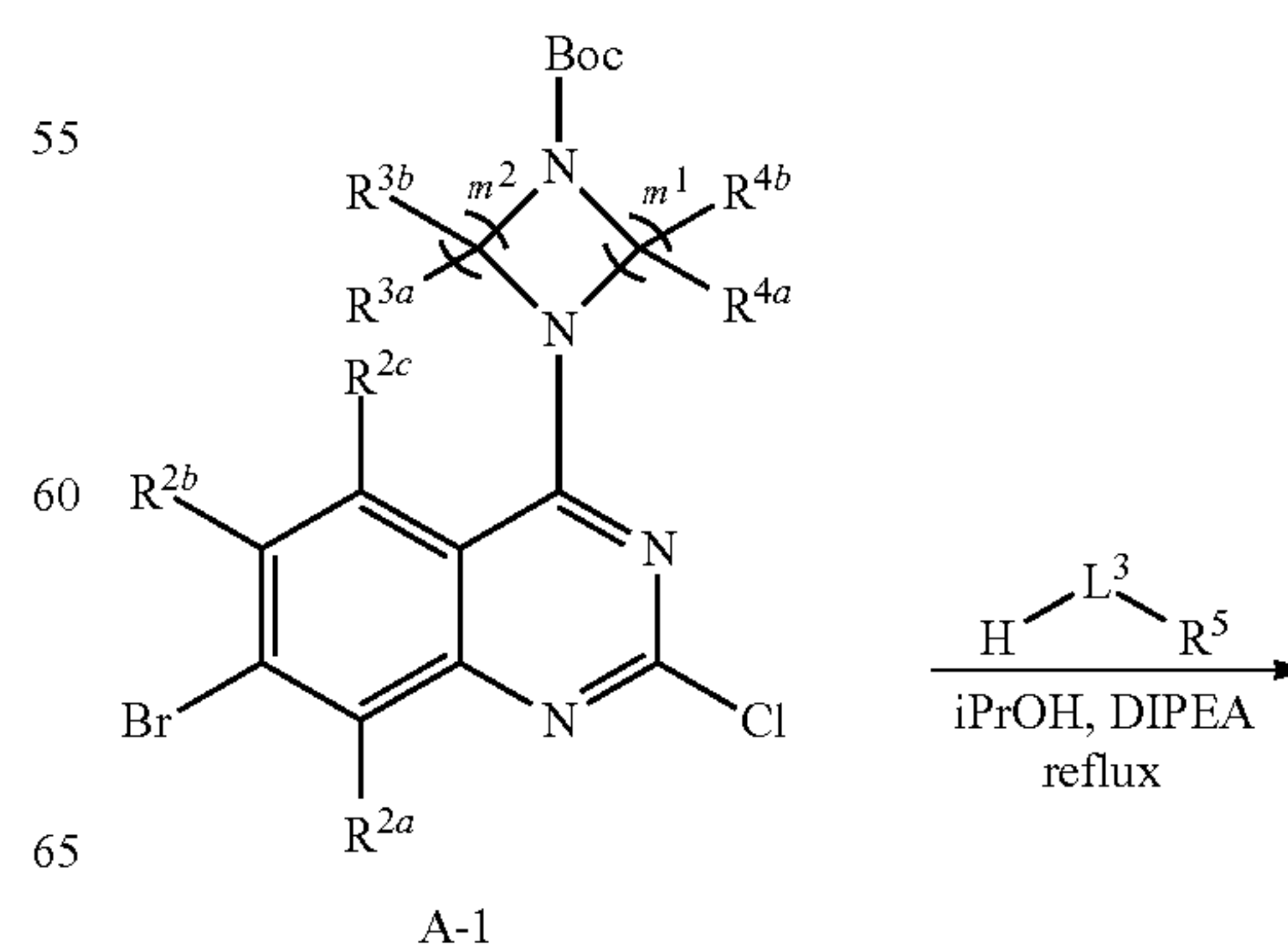
General Reaction Scheme 1
