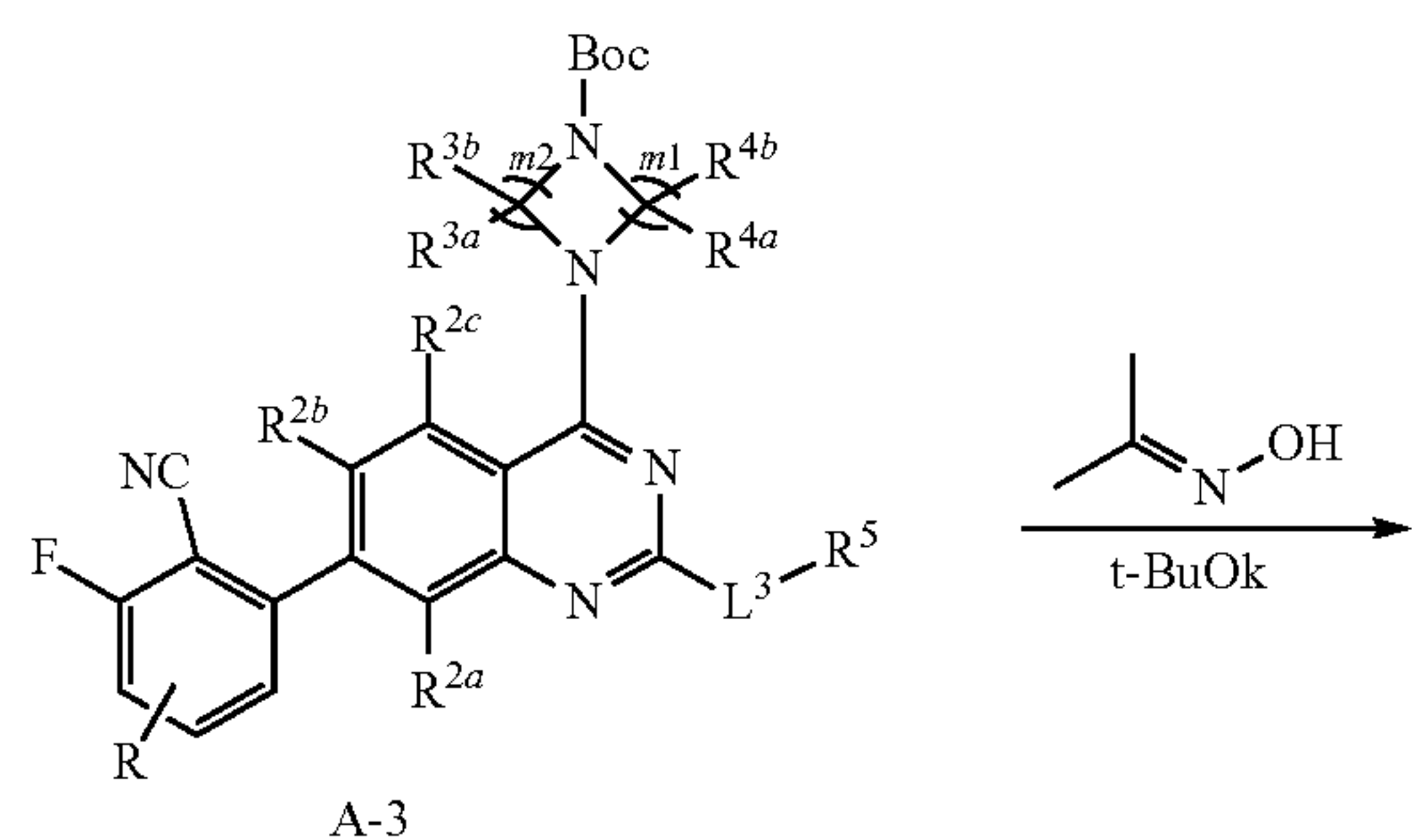
General Reaction Scheme 6
