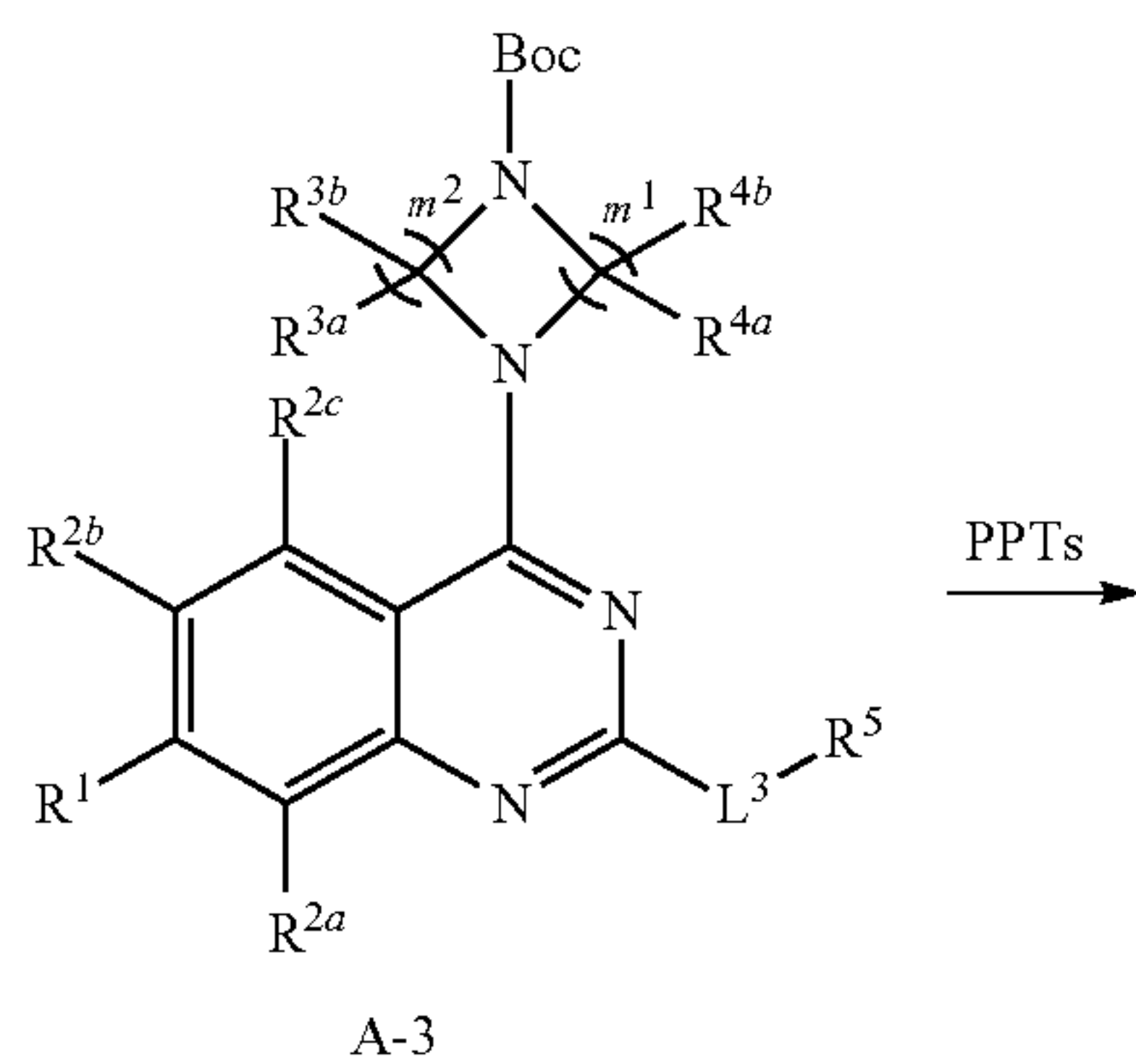
General Reaction Scheme 4
