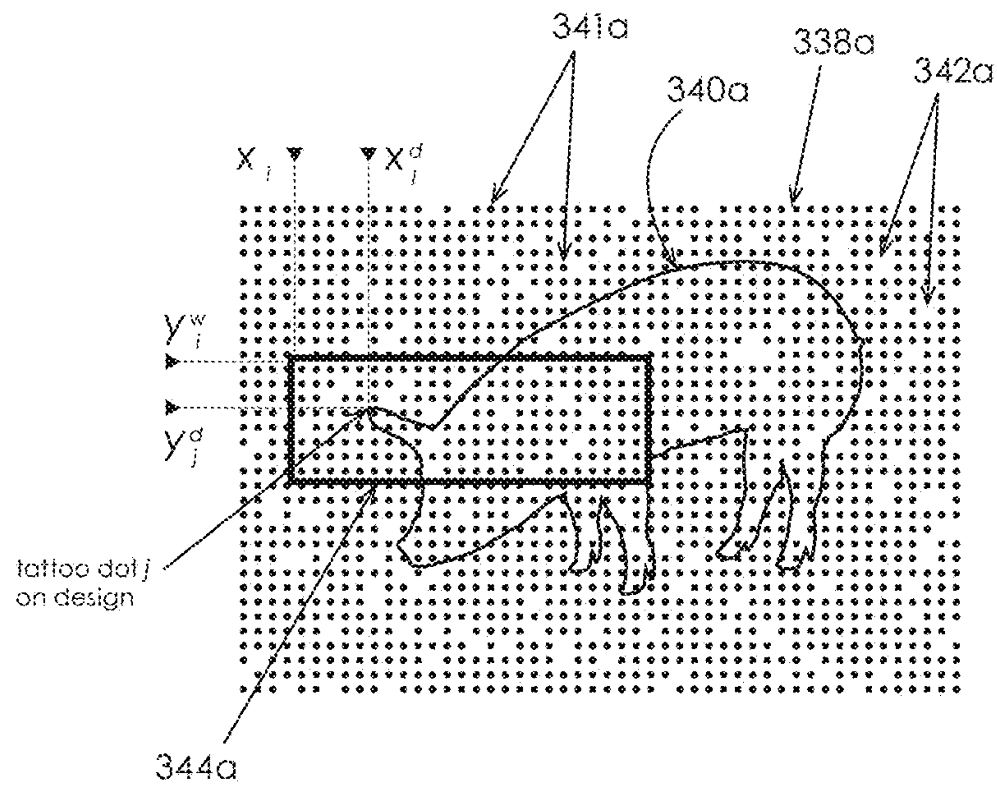
Digital Representation
