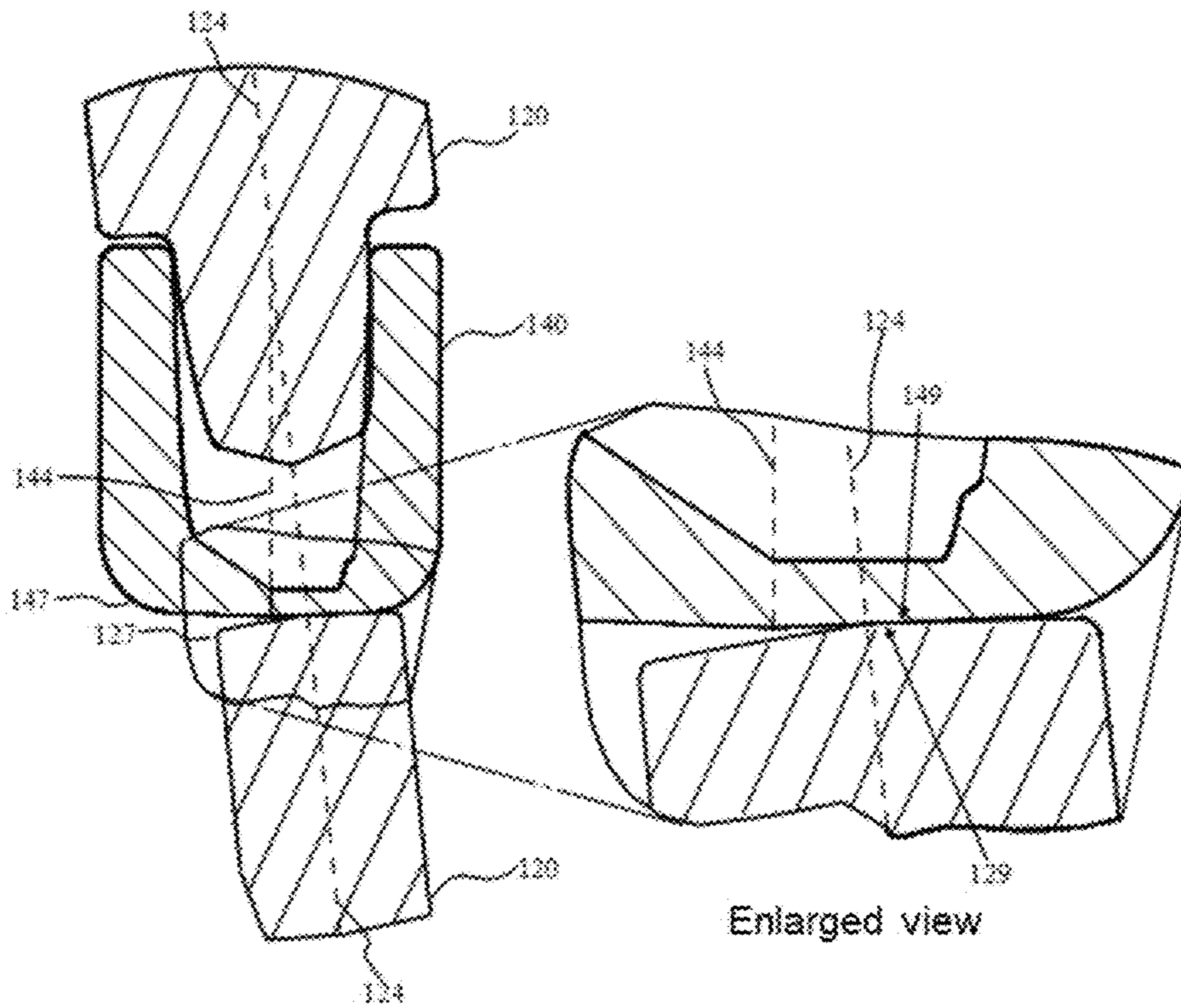
Partial cross-sectional view taken along line C-C'
