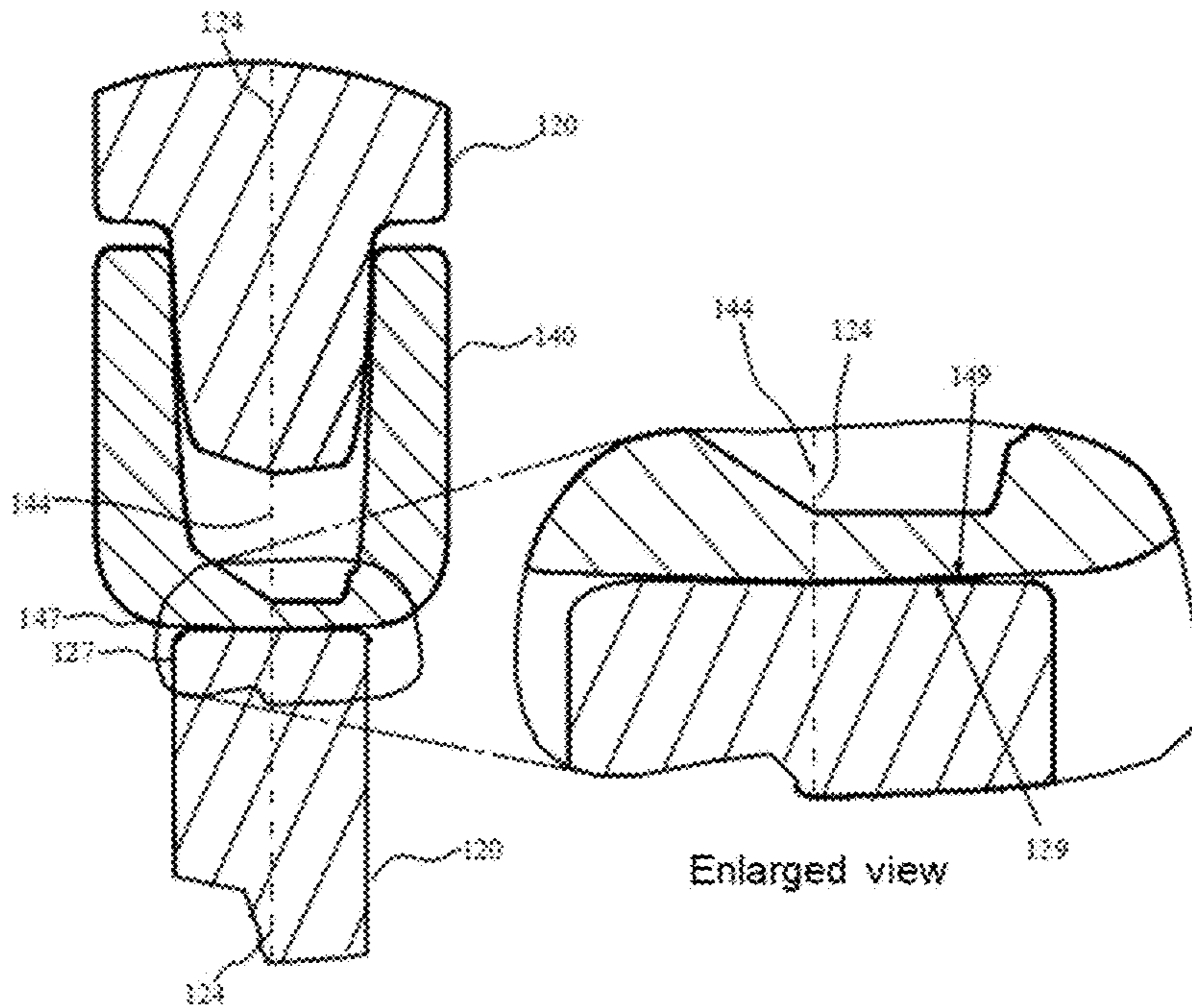
Partial cross-sectional view taken along line A-A'
