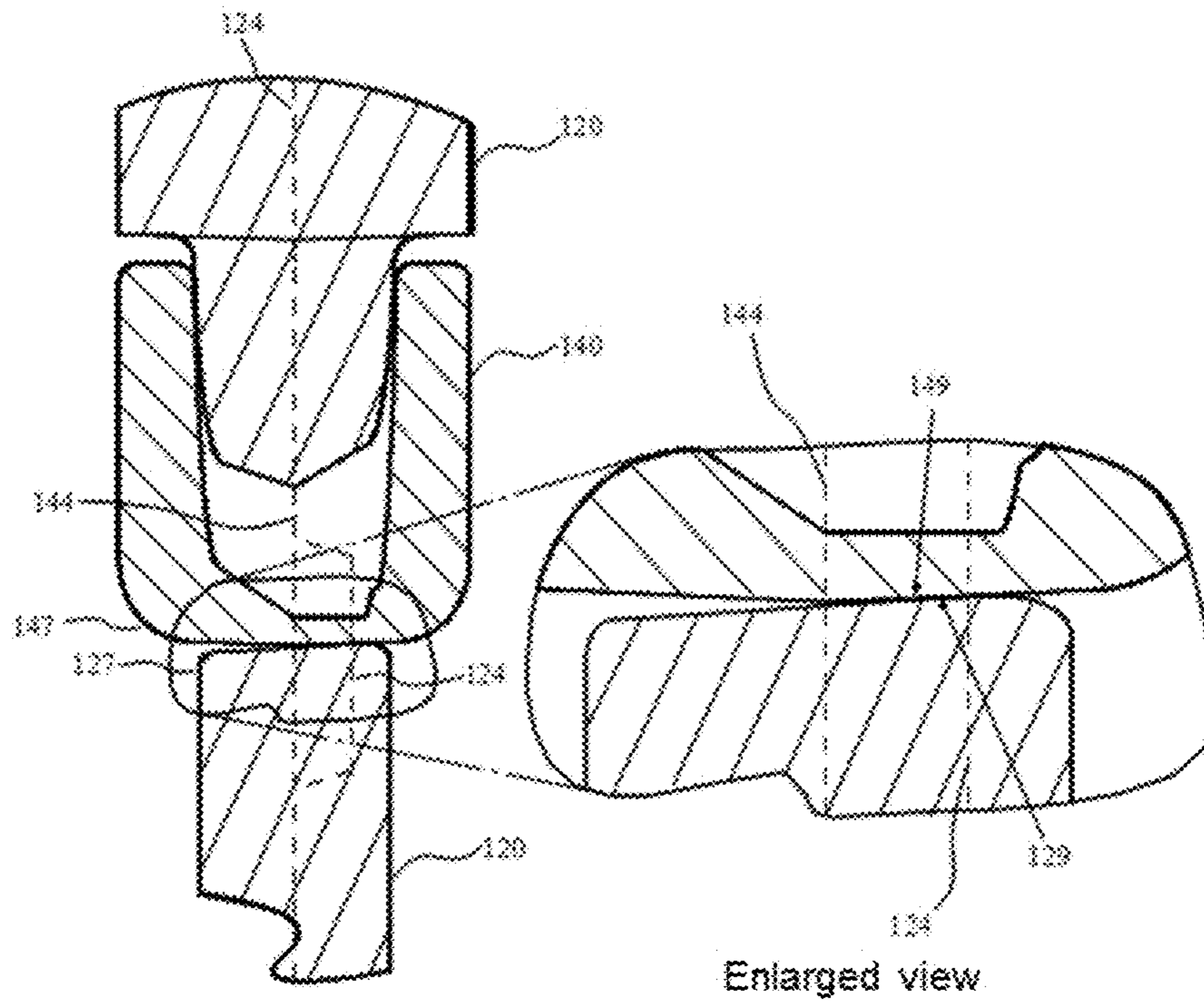
Partial cross-sectional view taken along line B-B'
