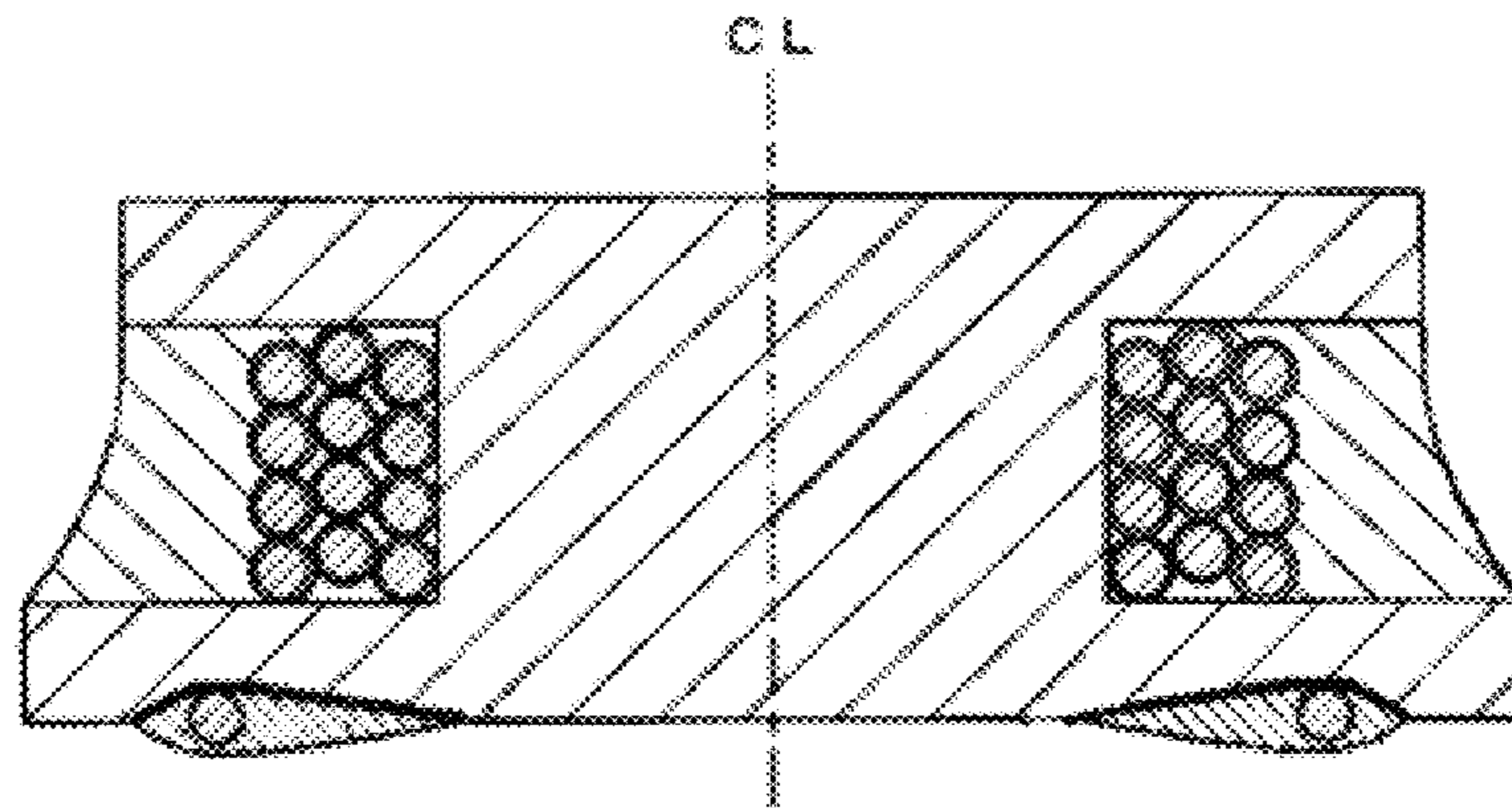
Cross-Section A-A
