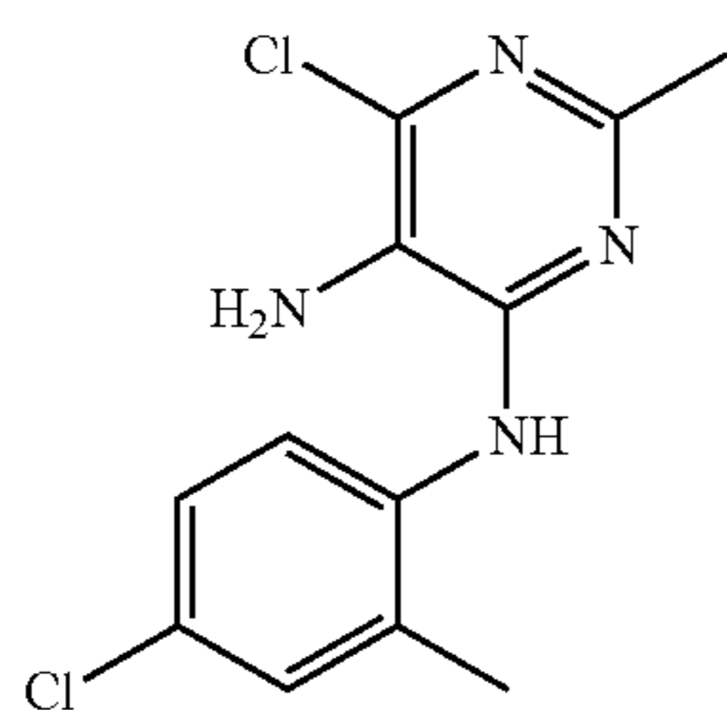
6-Chloro-N4-(4-chloro-2-methylphenyl)-2-methylpyrimidine-4,5-diamine (3)
