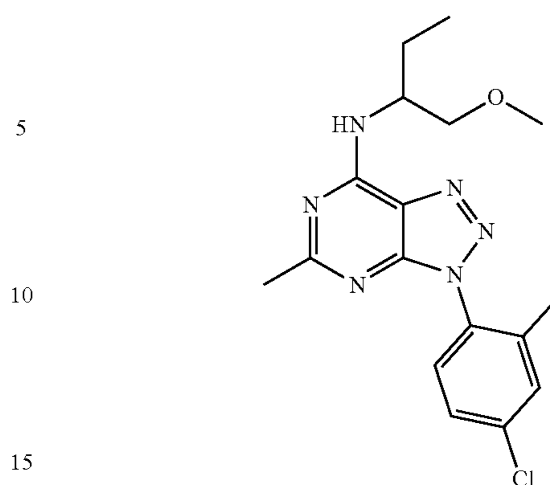
3-(4-Chloro-2-methylphenyl)-N-(1-methoxybutan-2-yl)-5-methyl-3H-[1,2,3]triazolo[4,5-d]pyrimidin-7-amine (6)
