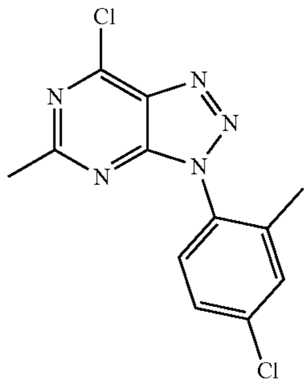
7-Chloro-3-(4-chloro-2-methylphenyl)-5-methyl-3H-[1,2,3]triazolo[4,5-d]pyrimidine (4)
