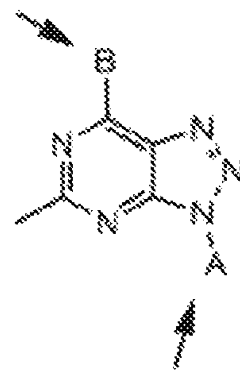
Triazolopyrimidine (J17)
